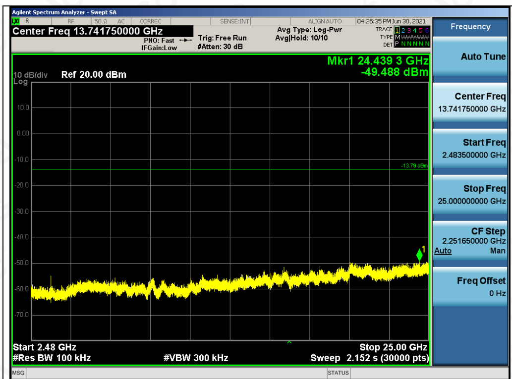
Test_Graph_LE1M_ANT1_2402_1Mbps_High Band Emissions
