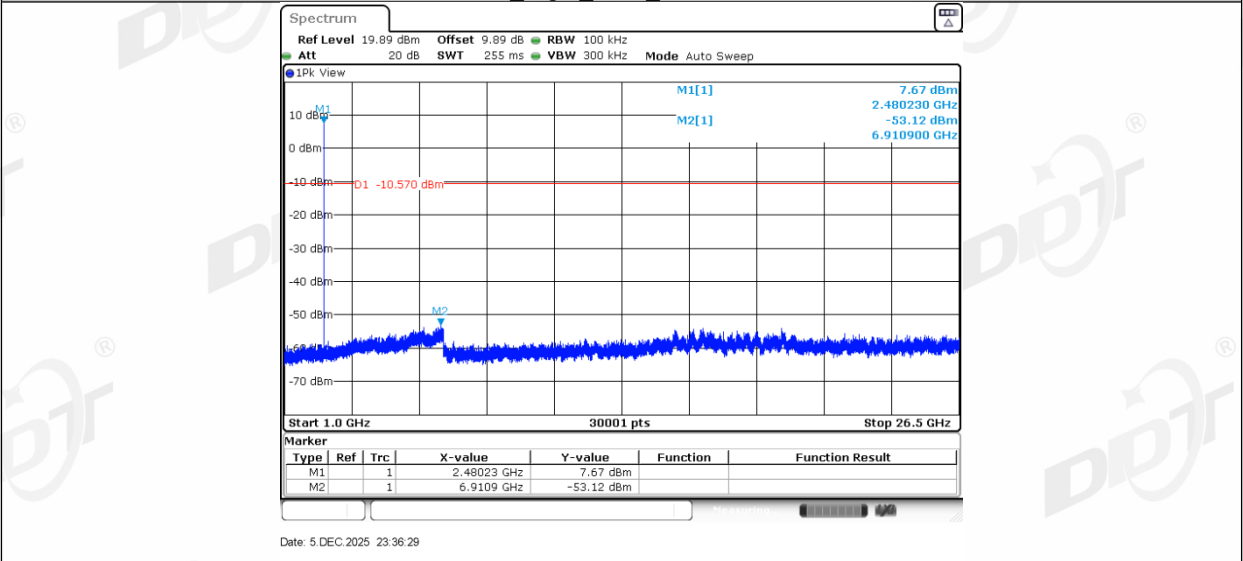
3DH5_Right_2480_1000~26500
