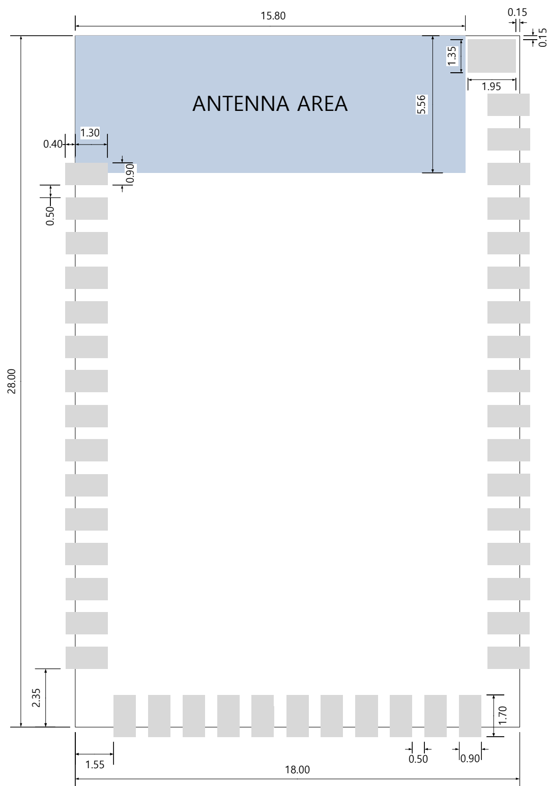
Land Pattern
