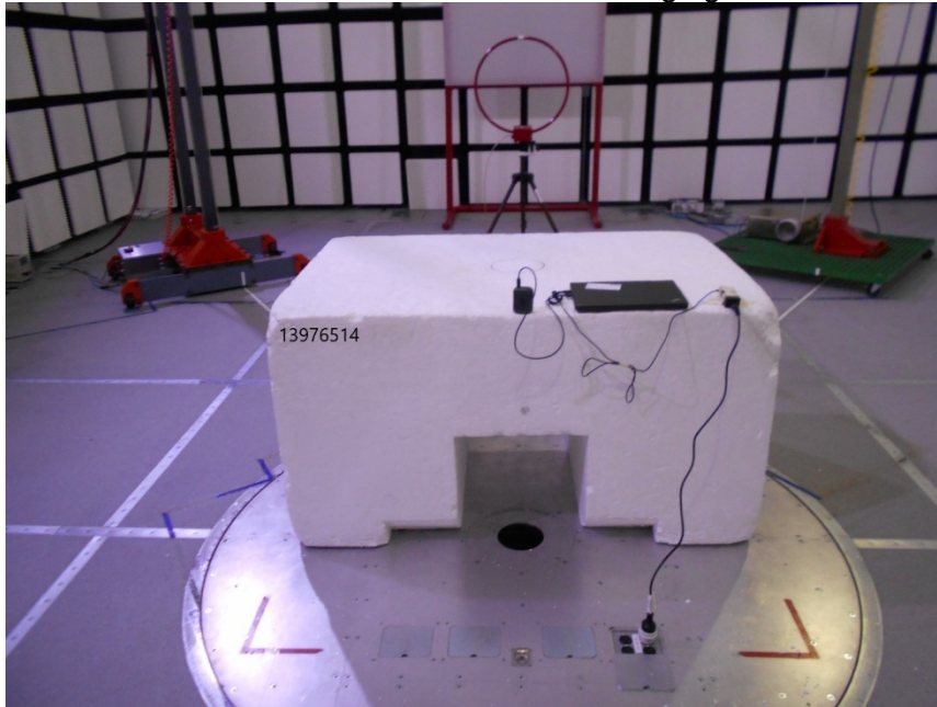
<30 MHz Face On Antenna Orientation - Charging Case
