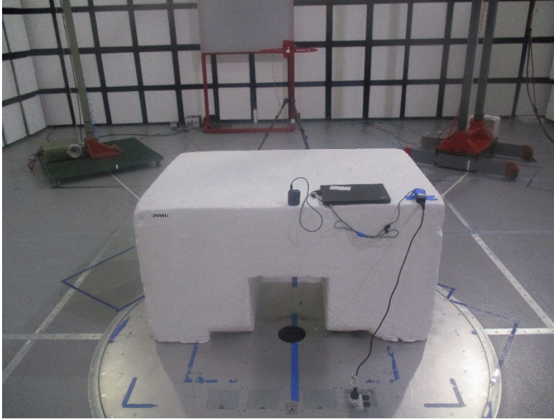
<30MHz Ground-Parallel Antenna Orientation - Charging Case
