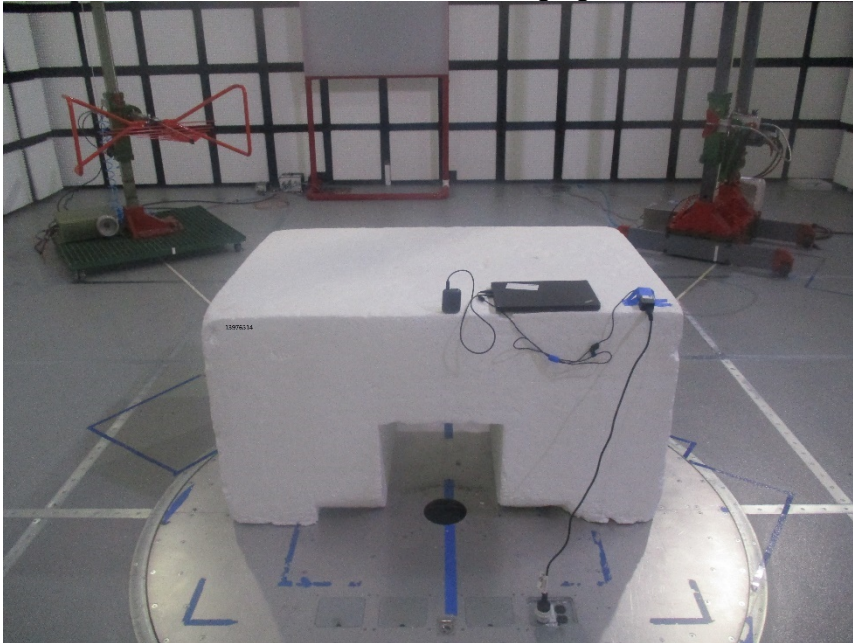
RADIATED PHOTO 30-1000MHz – Charging Case
