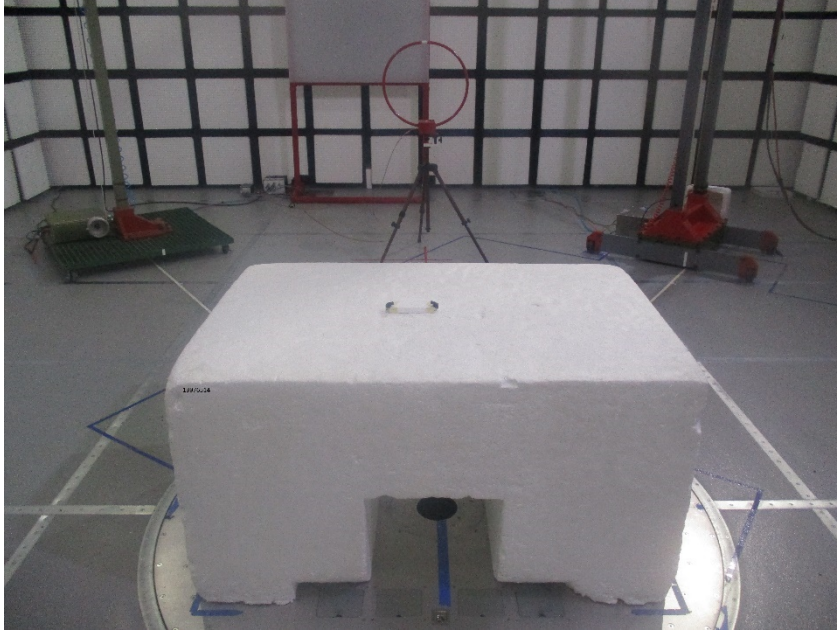
<30 MHz Face On Antenna Orientation
