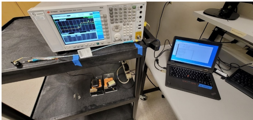
ANTENNA PORT CONDUCTED SETUP
