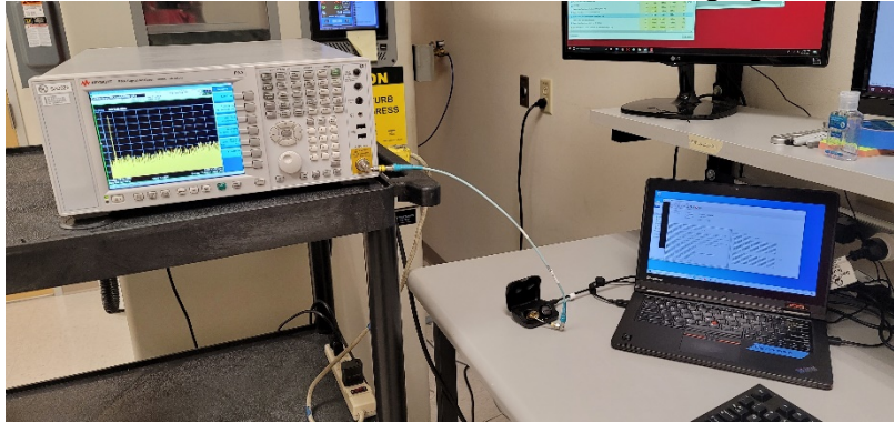
ANTENNA PORT CONDUCTED SETUP – Charging Case
