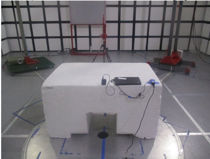
<30MHz Perpendicular Antenna Orientation - Charging Case
