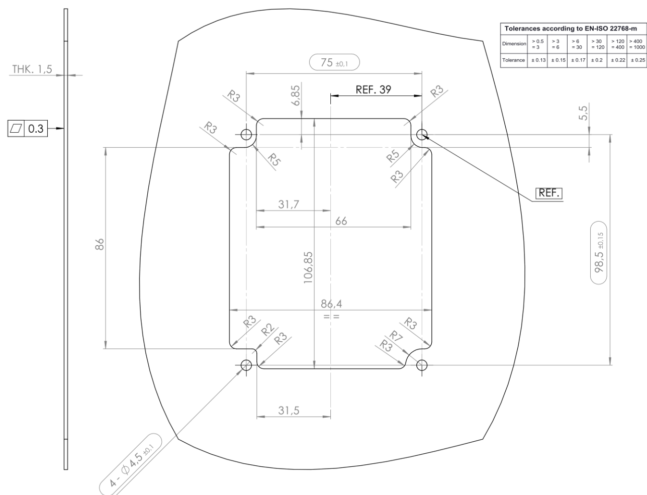
FIGURE 7 – Panel drilling of BV1000GTV
