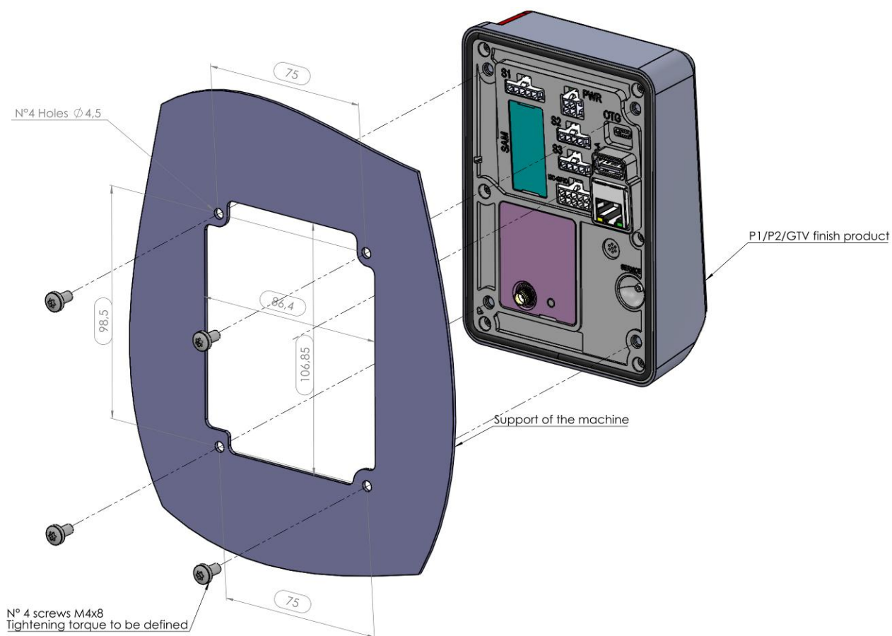
FIGURE 8 – Panel Fixing for BV1000GTV
