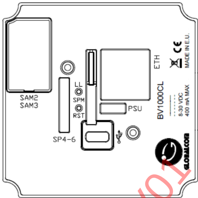
FIGURE 1 – Connector View of the BV1000CL
