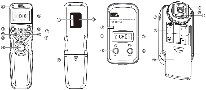
TW-283 Transmitter
