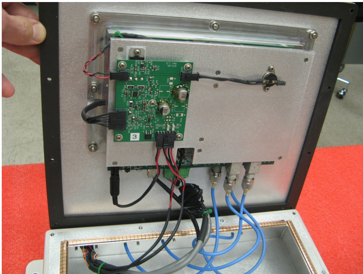
ID6204 Chassis Interior
