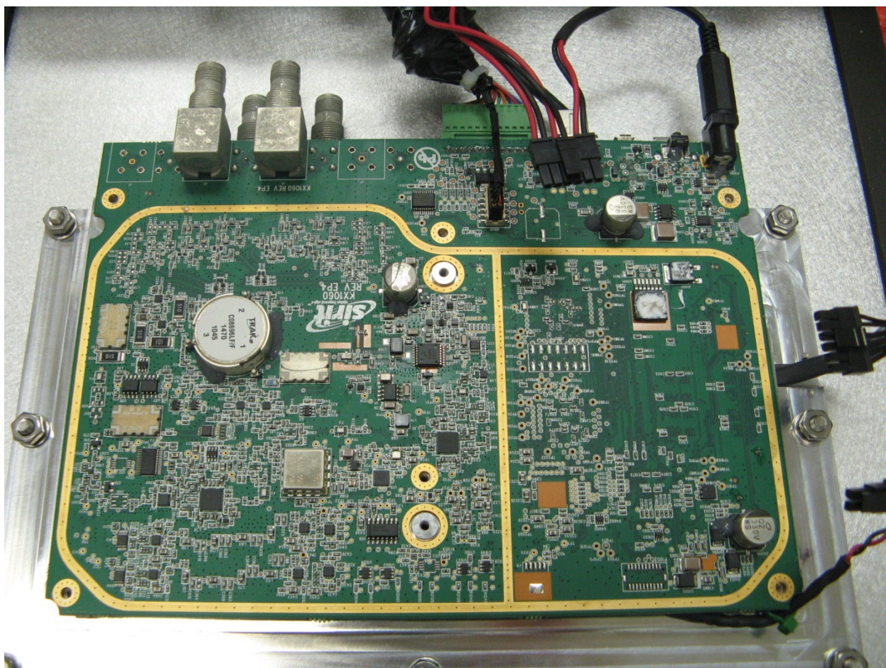
ID6204 PCB Bottom (Bottom Shield Cover Removed)
