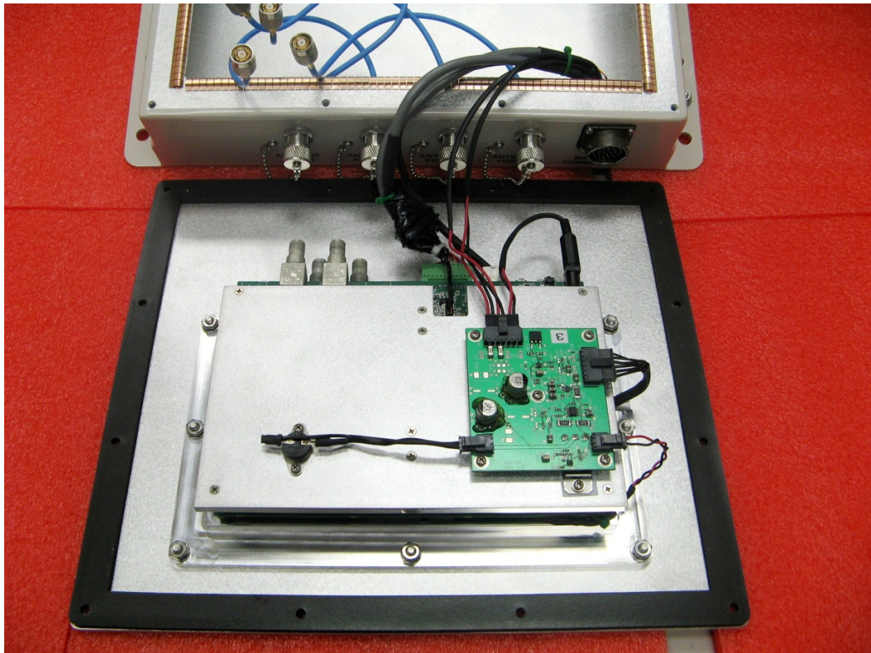
ID6204 Bottom Shield Cover, Heater Control PCB, Thermostat & Interconnect Wiring
