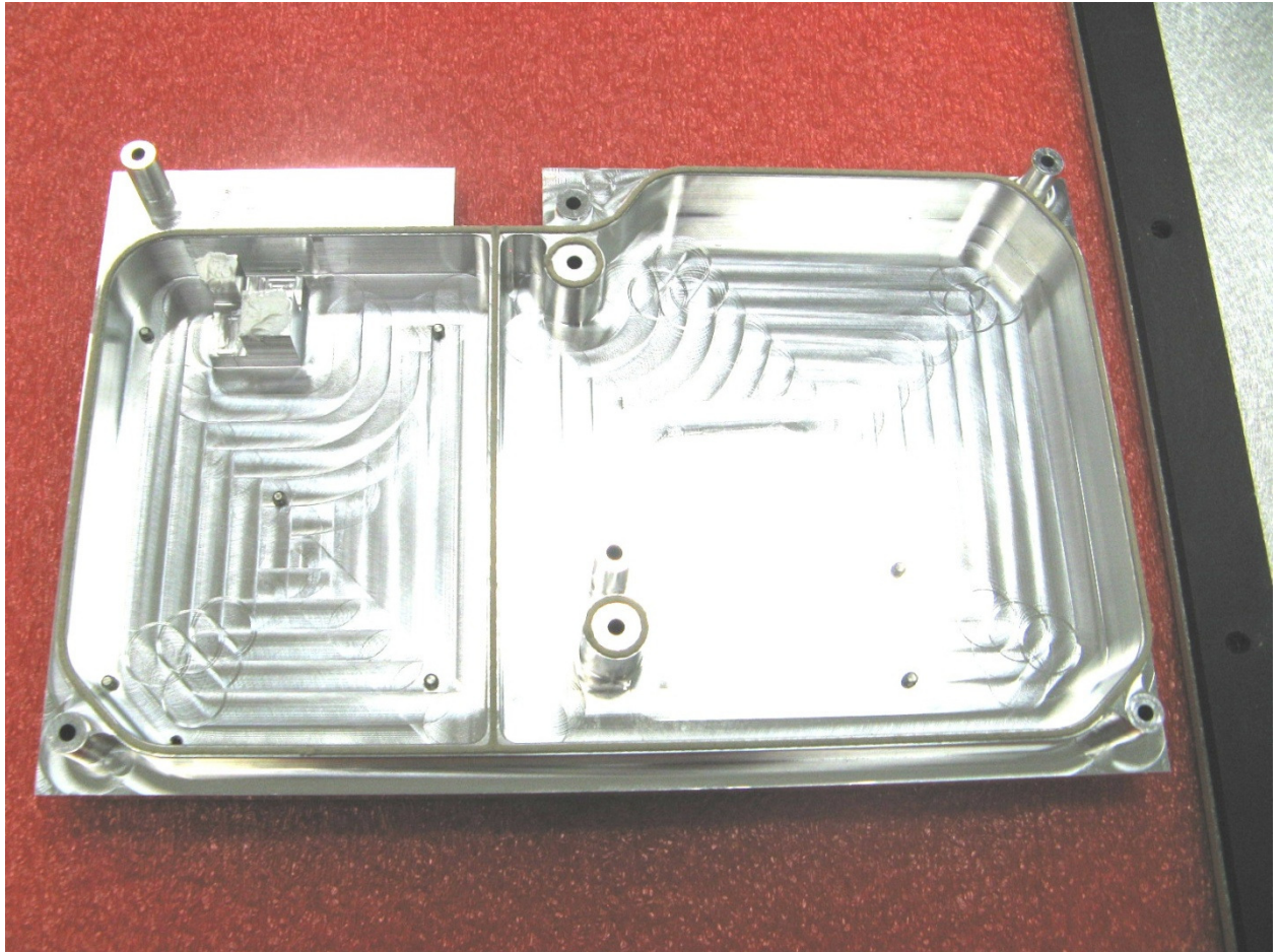
ID6204 Bottom Shield Cover Interior
