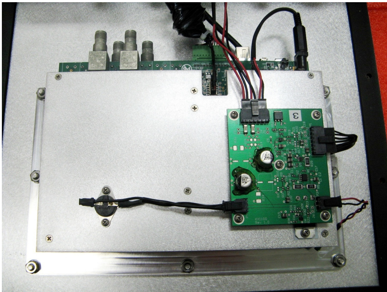
ID6204 Bottom Shield Cover, Close Up
