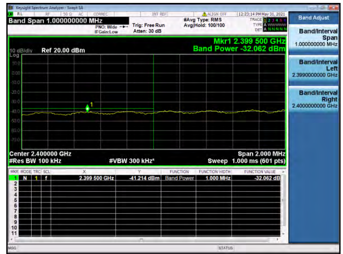
802.11g CHANNEL 2, Reference level
