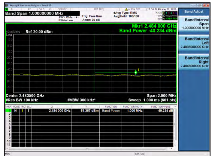
802.11g CHANNEL 10, Reference level
