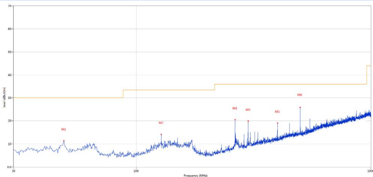
30 MHz to 1 GHz, ANT H
