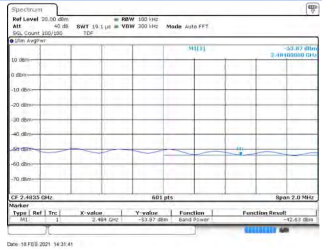
802.11g HIGH CHANNEL, Reference level
