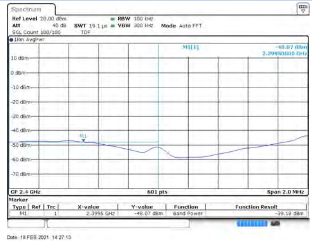
802.11b LOW CHANNEL, Reference level
