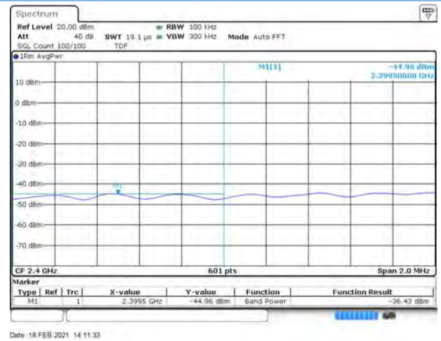
802.11n-20 MHz LOW CHANNEL, Reference level
