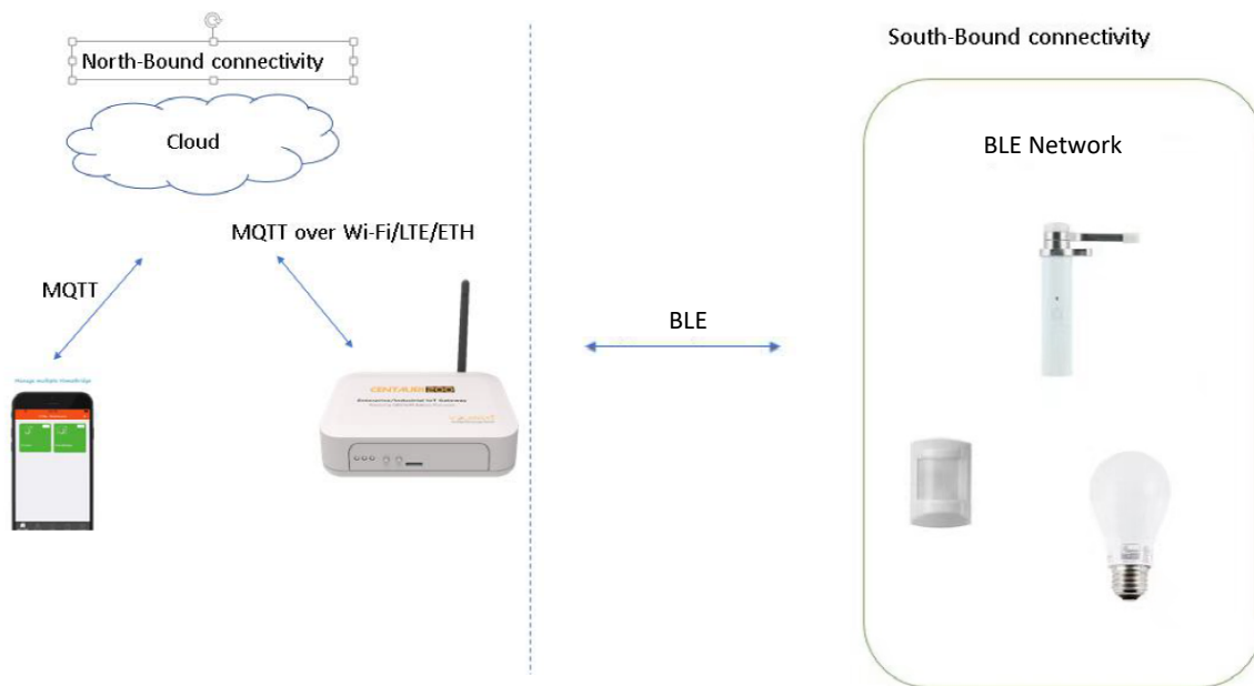
Figure 1-1 Gateway setup architecture
