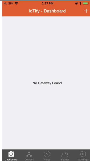
Figure 4- 2 IoTify Dashboard
