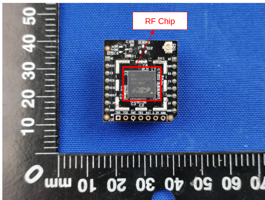
ZWAVE MODULE TOP VIEW --- 1# circuit (without saw filter)
