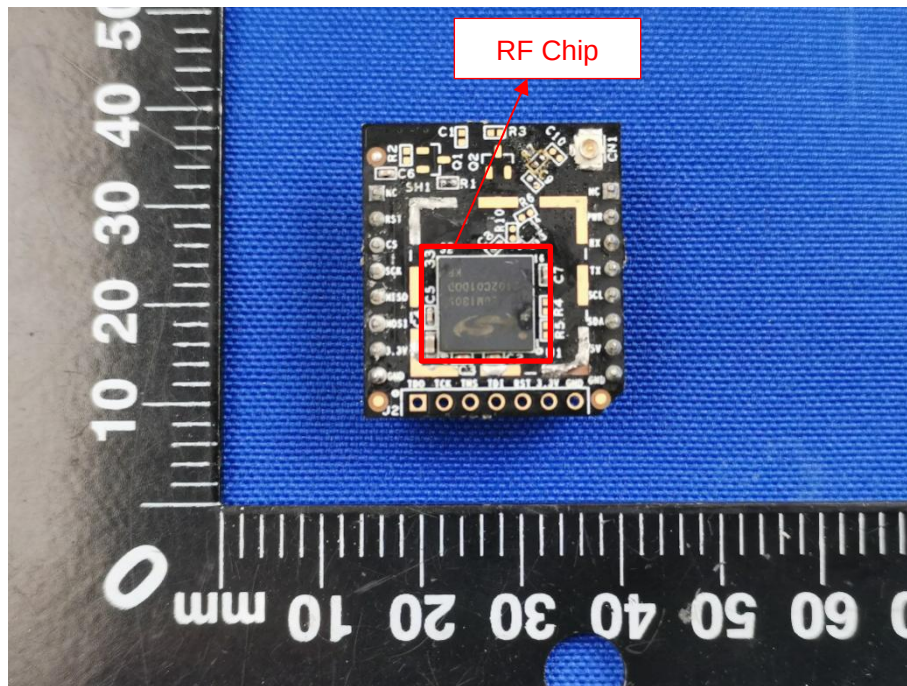
ZWAVE MODULE TOP VIEW --- 1# circuit (with saw filter)
