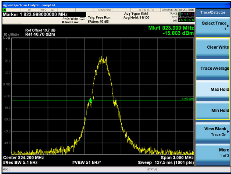
(Channel 128: 824.20MHz @ GPRS 850)
