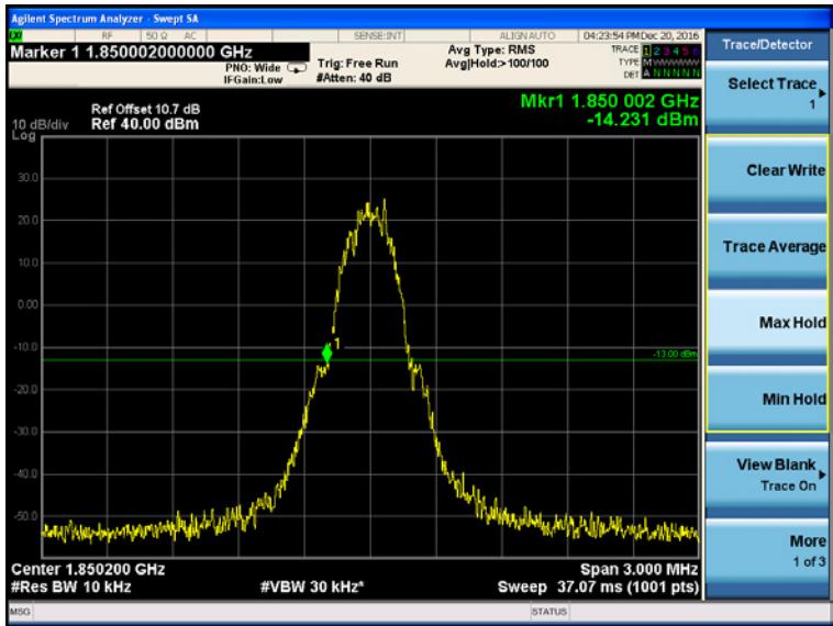
(Channel 512: 1850.20MHz @ GPRS 1900)
