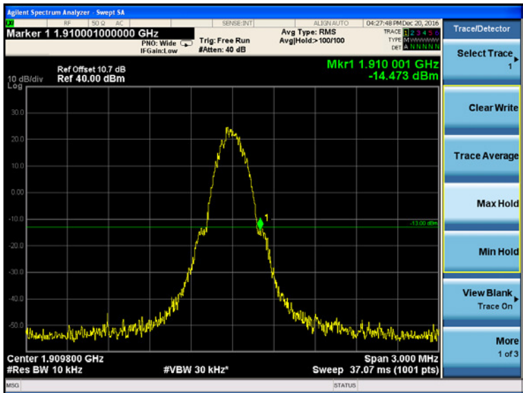
(Channel 810: 1909.80MHz @ GPRS 1900)
