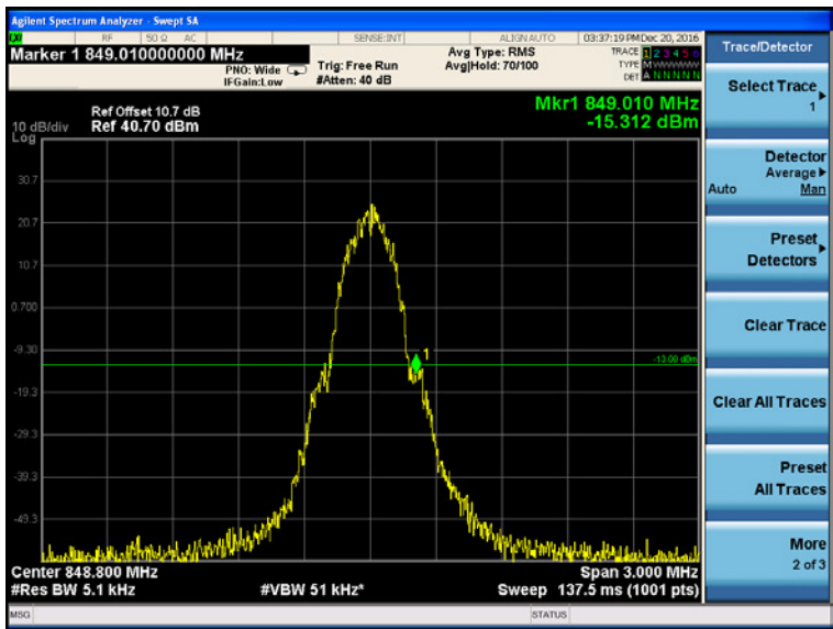
(Channel 251: 848.80MHz @ GPRS 850)
