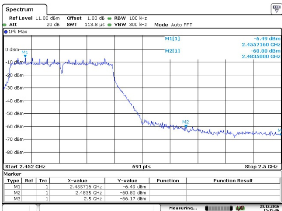
CH11-Bandedge
