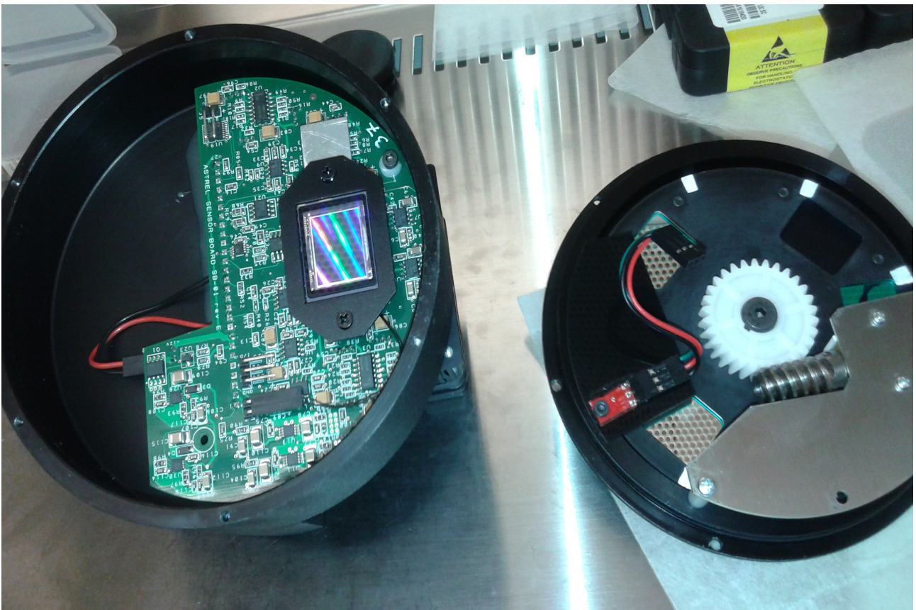
AST8300-B Sensor Unit Box and its Top Cover
