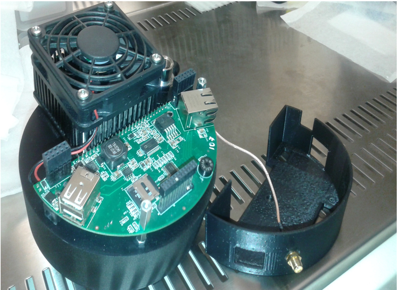
AST8300-B Processor Unit Box and its Bottom Cover
