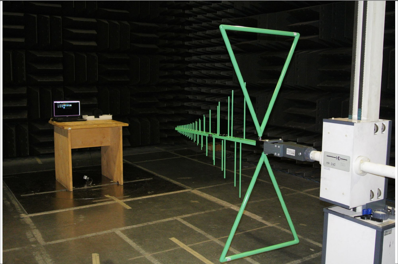
Fig. 6.2 Radiated Emissions Test Set-up
