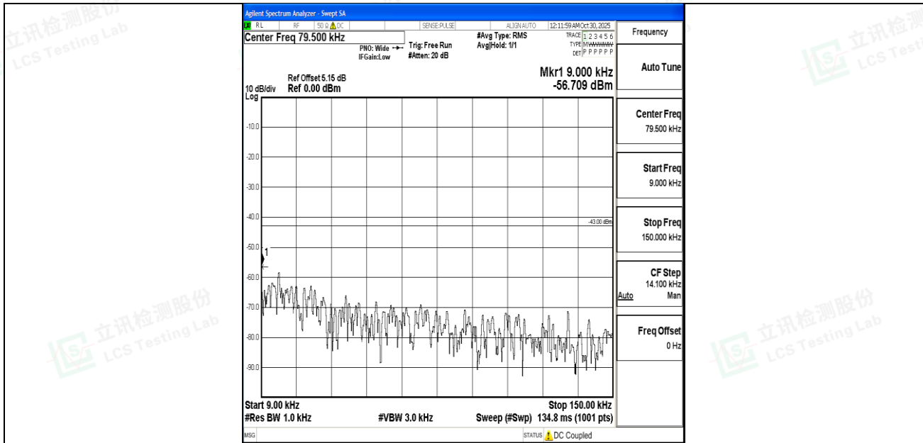
Band4_20MHz_QPSK_20050_1RB#0_0.009~0.15_0.009~0.15
