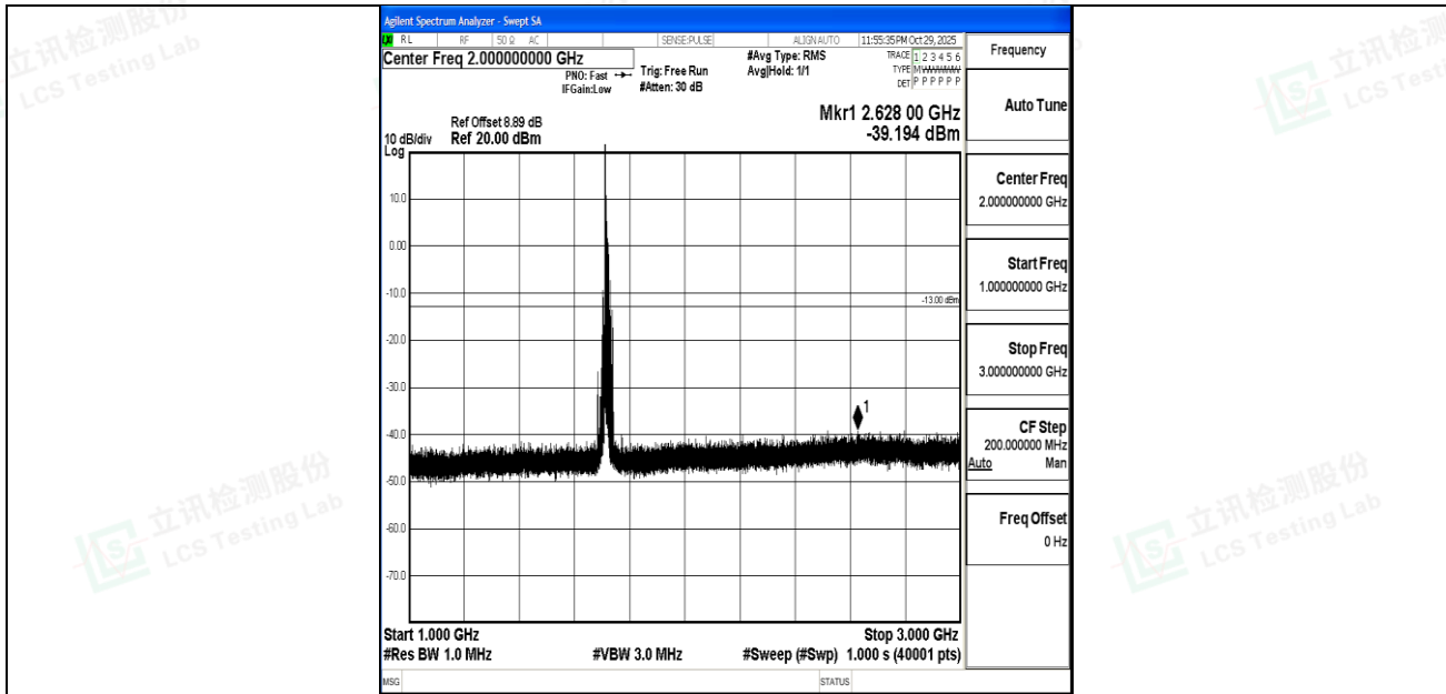
Band4_15MHz_16QAM_20025_1RB#0_1000~3000_1000~3000
