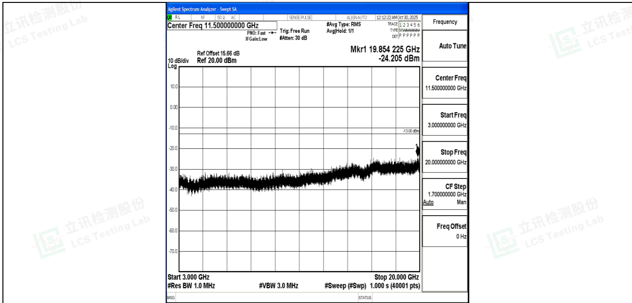
Band4_20MHz_QPSK_20050_1RB#0_3000~20000_3000~20000
