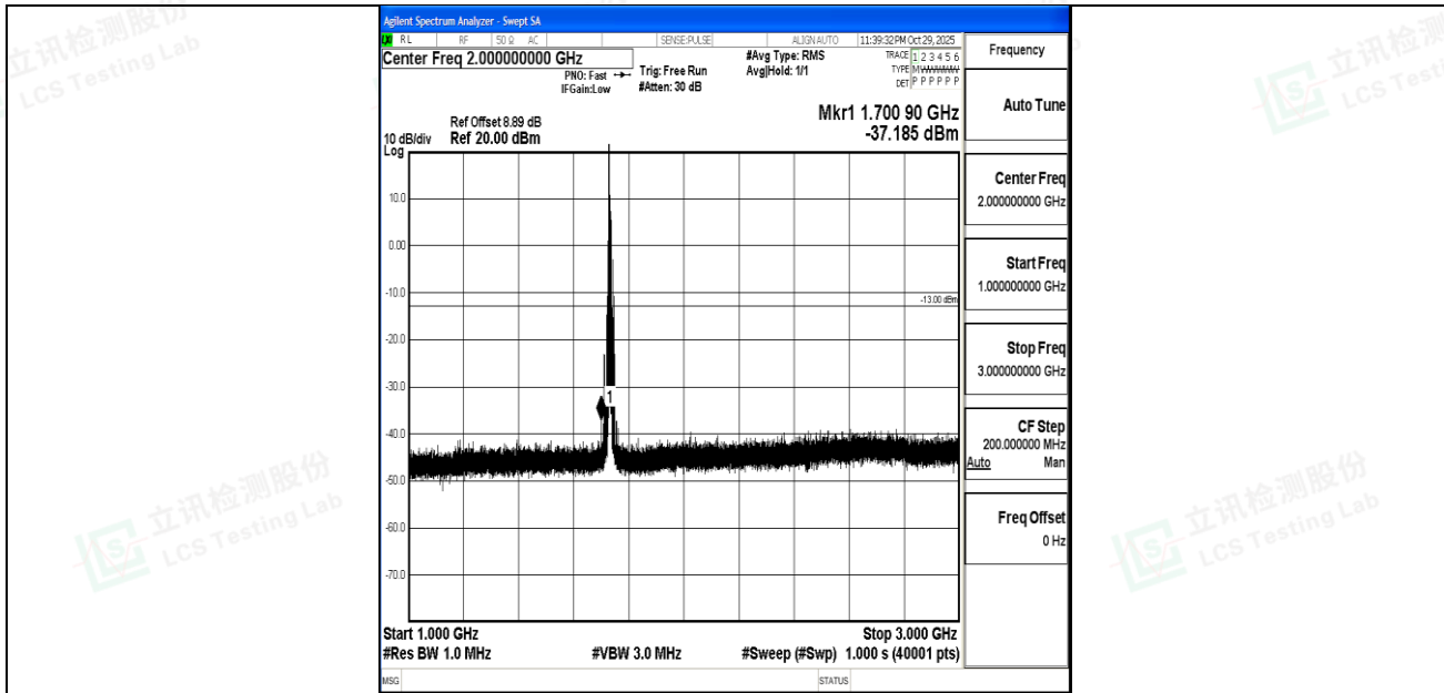
Band4_10MHz_16QAM_20175_1RB#0_1000~3000_1000~3000
