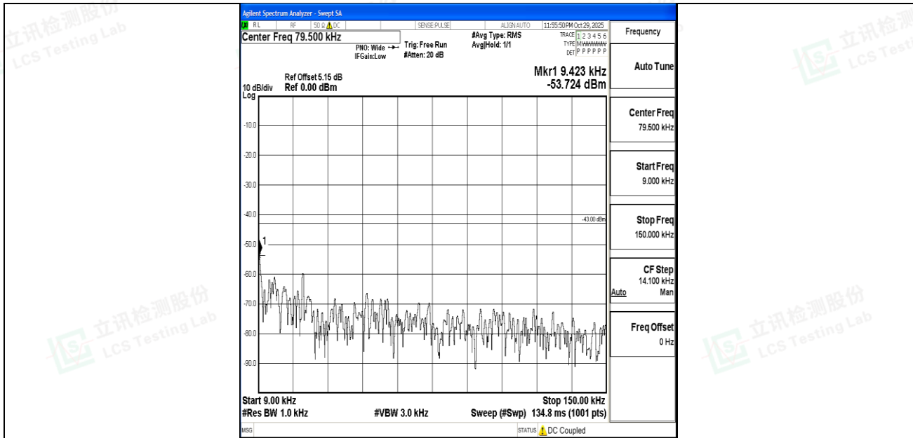
Band4_15MHz_QPSK_20175_1RB#0_0.009~0.15_0.009~0.15
