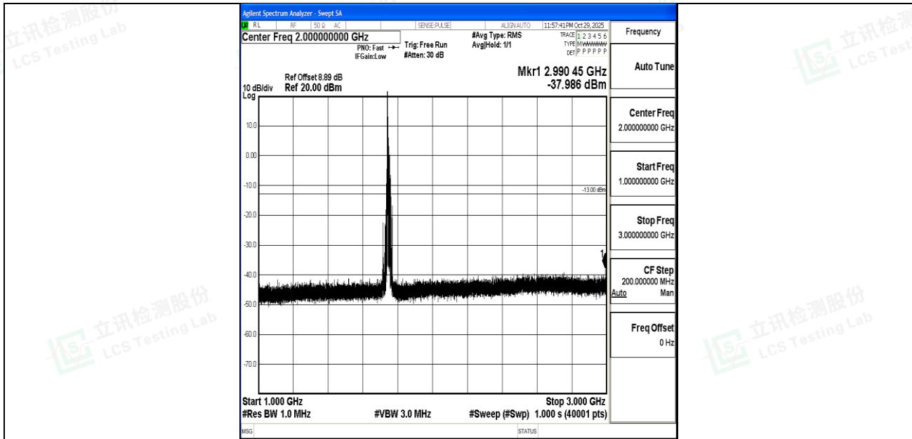
Band4_15MHz_16QAM_20325_1RB#0_1000~3000_1000~3000
