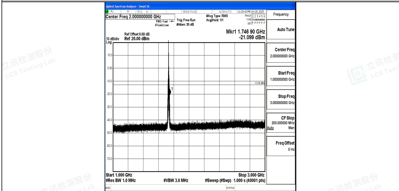
Band4_5MHz_QPSK_20175_1RB#0_1000~3000_1000~3000
