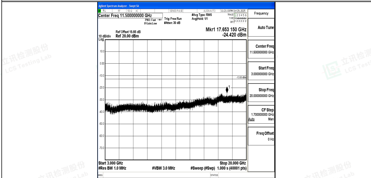
Band4_5MHz_16QAM_20175_1RB#0_3000~20000_3000~20000
