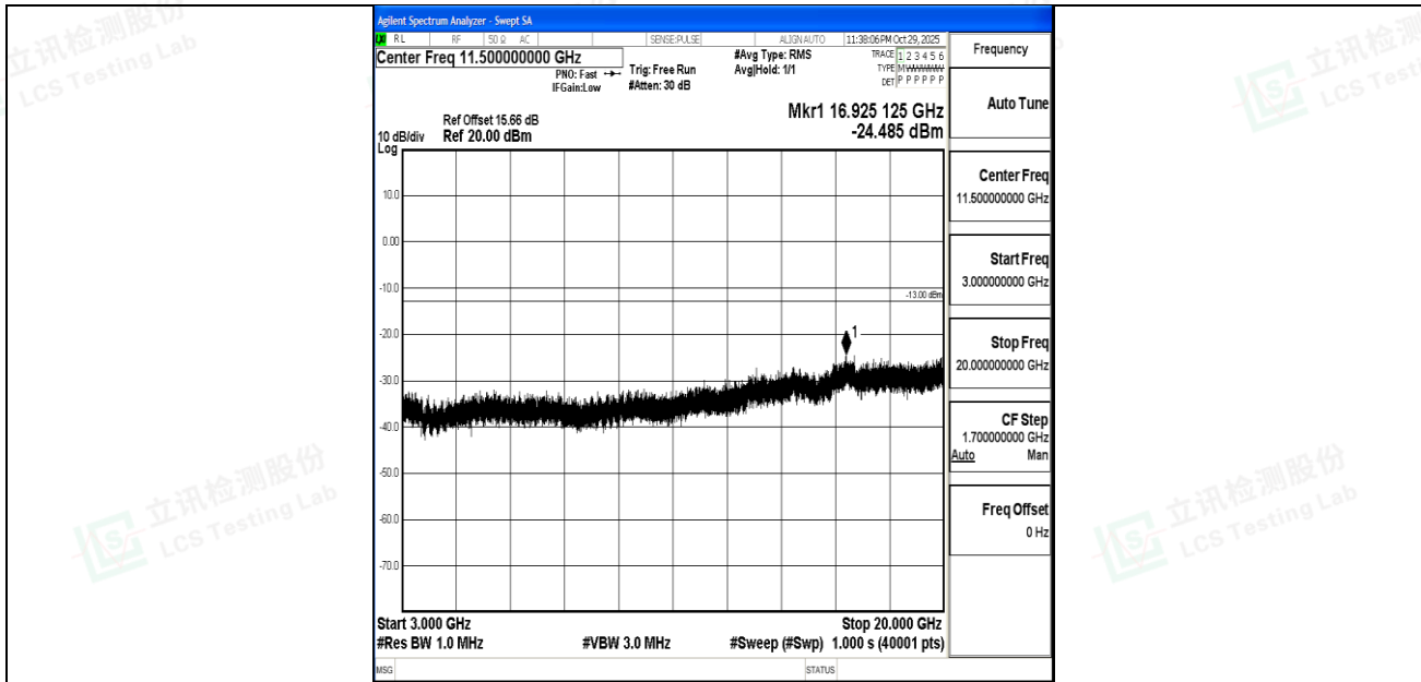
Band4_10MHz_QPSK_20000_1RB#0_3000~20000_3000~20000
