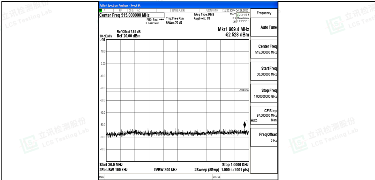
Band4_5MHz_QPSK_20175_1RB#0_30~1000_30~1000
