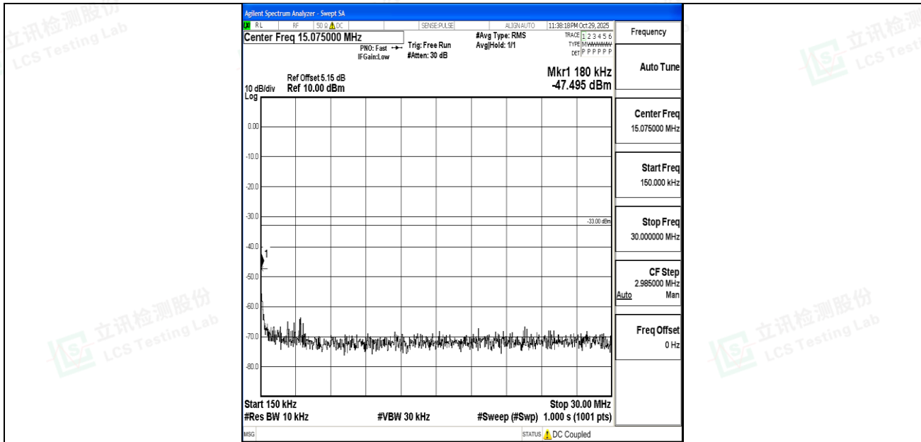
Band4_10MHz_16QAM_20000_1RB#0_0.15~30_0.15~30
