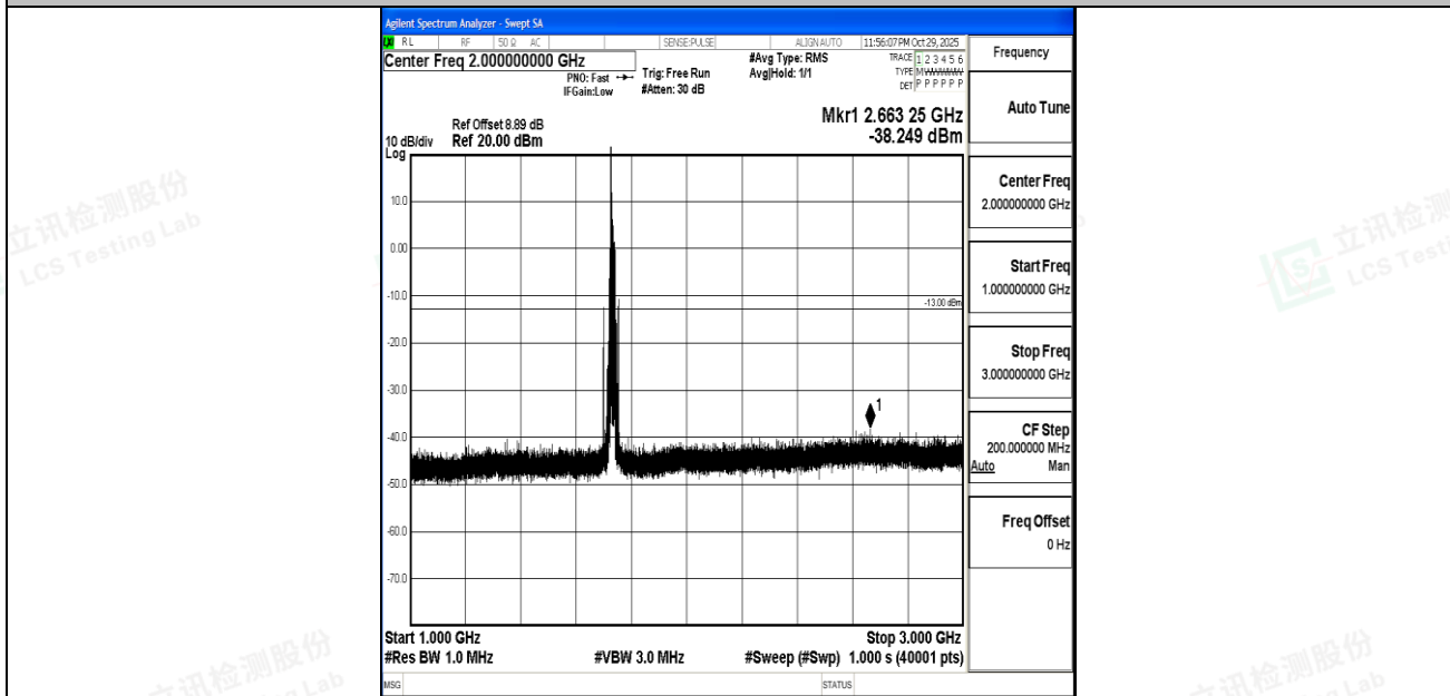
Band4_15MHz_QPSK_20175_1RB#0_1000~3000_1000~3000
