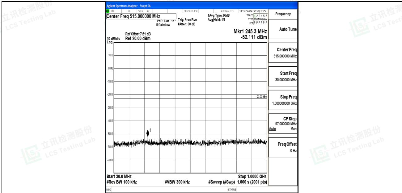
Band4_15MHz_QPSK_20025_1RB#0_30~1000_30~1000
