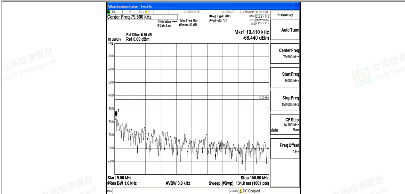
Band4_15MHz_16QAM_20025_1RB#0_0.009~0.15_0.009~0.15
