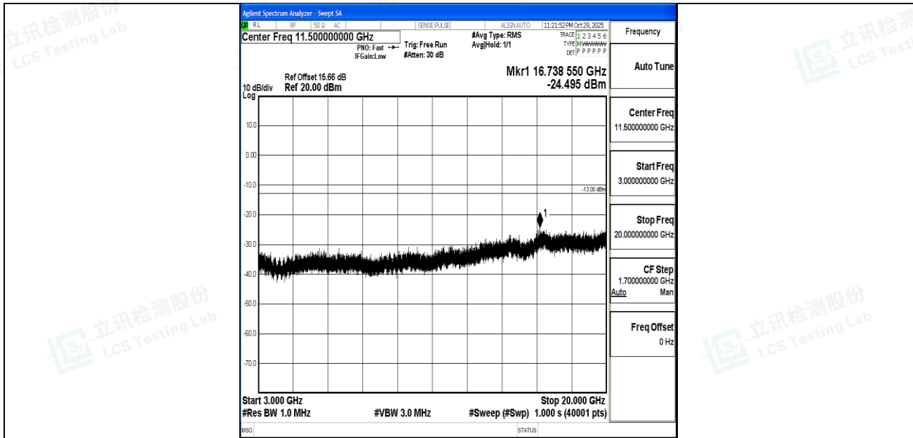
Band4_5MHz_QPSK_20375_1RB#0_3000~20000_3000~20000
