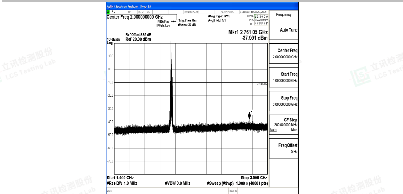
Band4_15MHz_QPSK_20325_1RB#0_1000~3000_1000~3000
