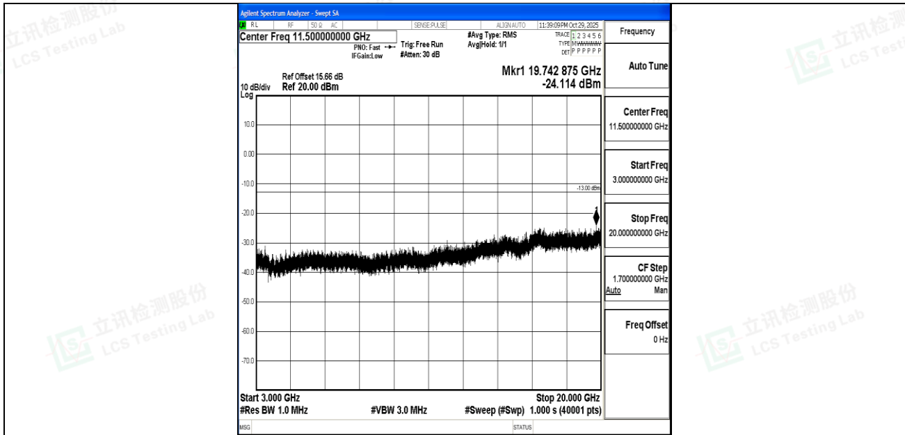
Band4_10MHz_QPSK_20175_1RB#0_3000~20000_3000~20000
