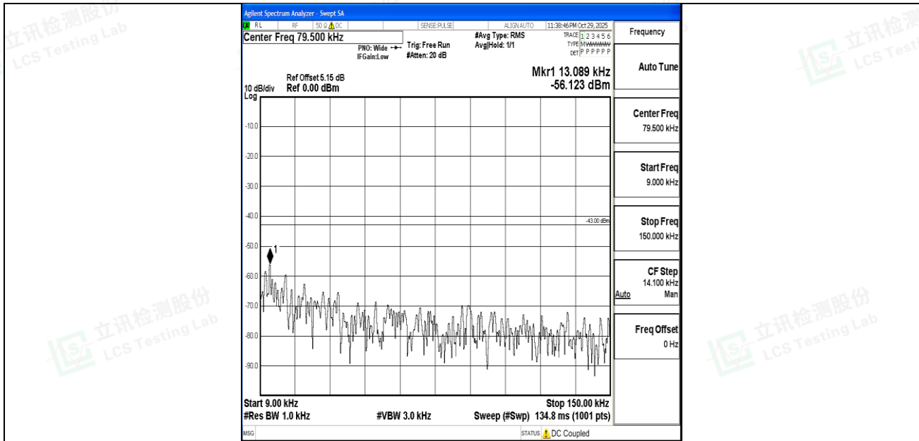
Band4_10MHz_QPSK_20175_1RB#0_0.009~0.15_0.009~0.15
