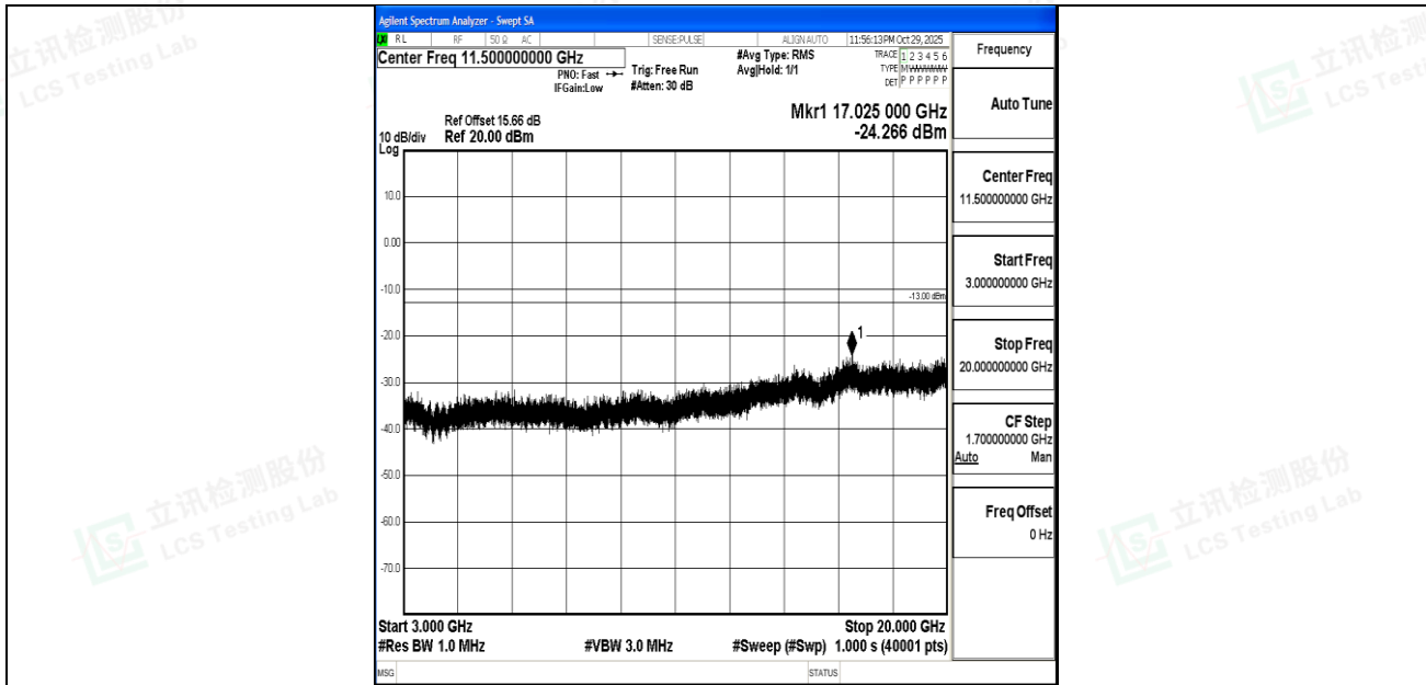
Band4_15MHz_QPSK_20175_1RB#0_3000~20000_3000~20000
