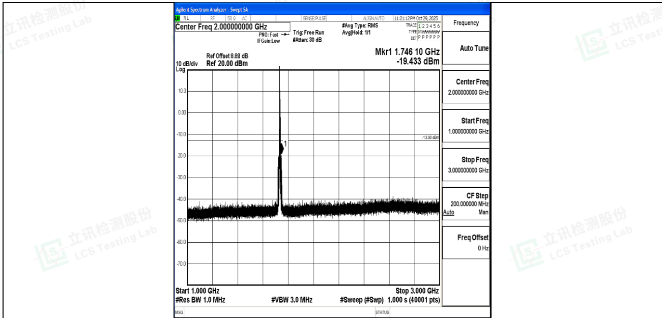
Band4_5MHz_16QAM_20175_1RB#0_1000~3000_1000~3000
