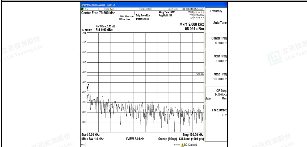
Band4_10MHz_16QAM_20350_1RB#0_0.009~0.15_0.009~0.15
