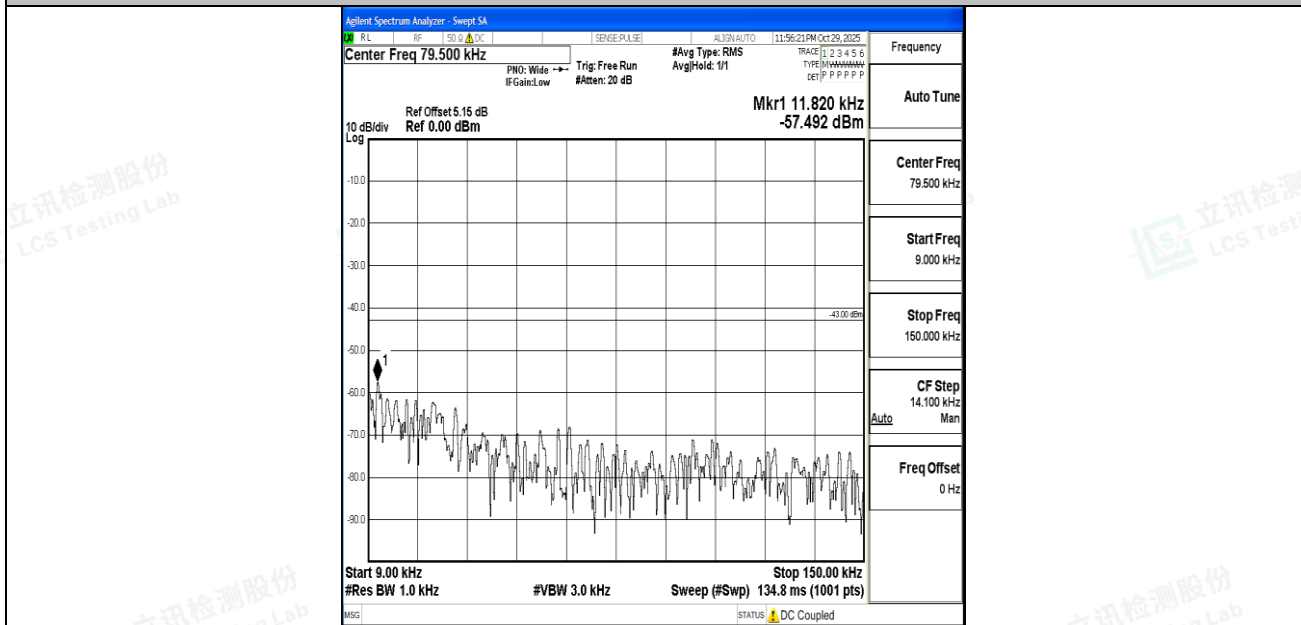
Band4_15MHz_16QAM_20175_1RB#0_0.009~0.15_0.009~0.15
