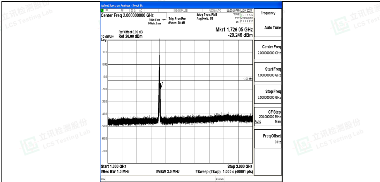
Band4_5MHz_16QAM_19975_1RB#0_1000~3000_1000~3000
