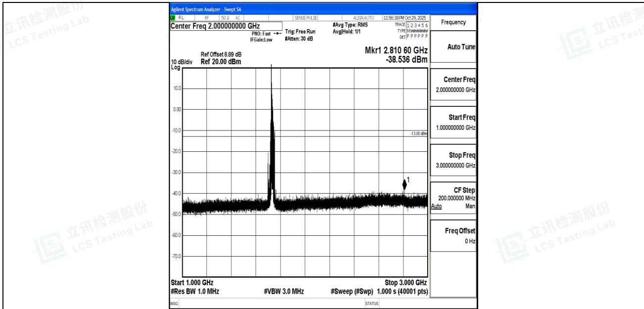
Band4_15MHz_16QAM_20175_1RB#0_1000~3000_1000~3000
