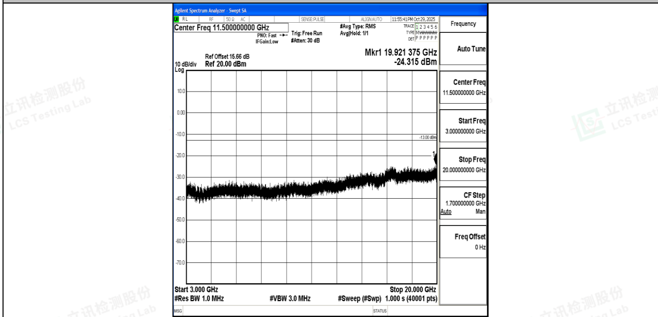
Band4_15MHz_16QAM_20025_1RB#0_3000~20000_3000~20000
