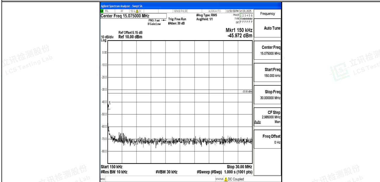
Band4_15MHz_QPSK_20325_1RB#0_0.15~30_0.15~30
