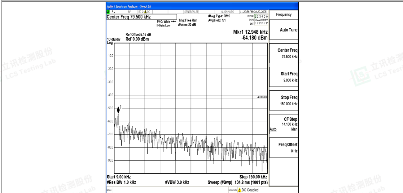
Band4_5MHz_16QAM_20175_1RB#0_0.009~0.15_0.009~0.15
