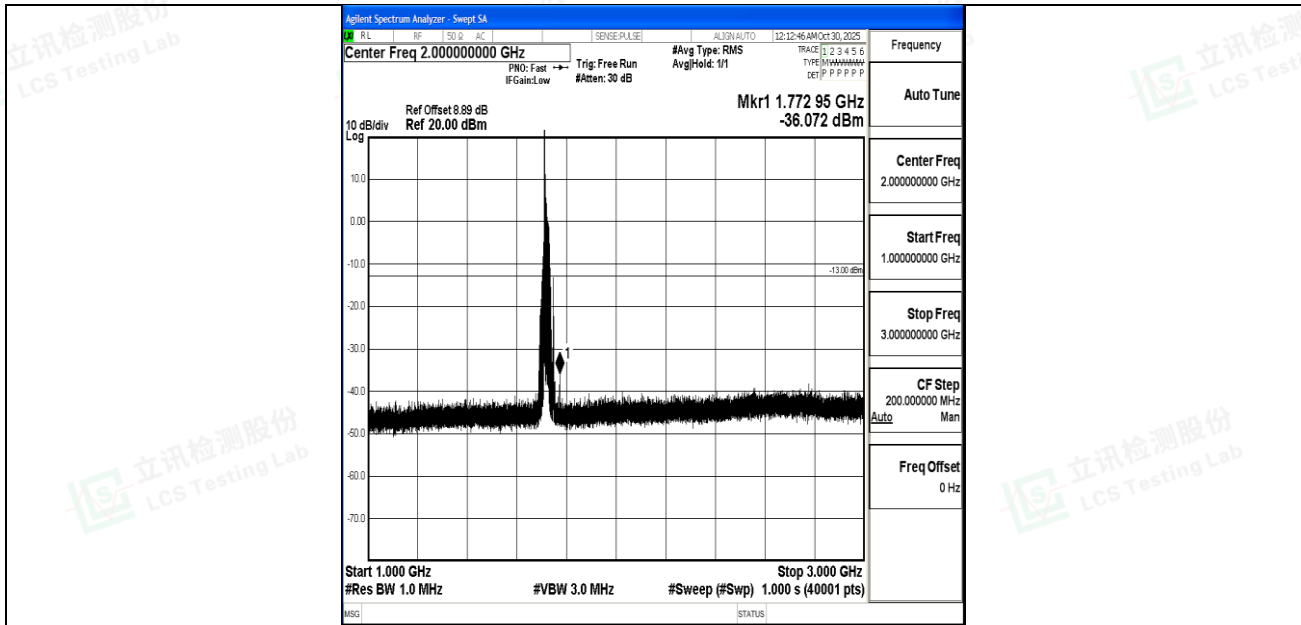
Band4_20MHz_16QAM_20050_1RB#0_1000~3000_1000~3000
