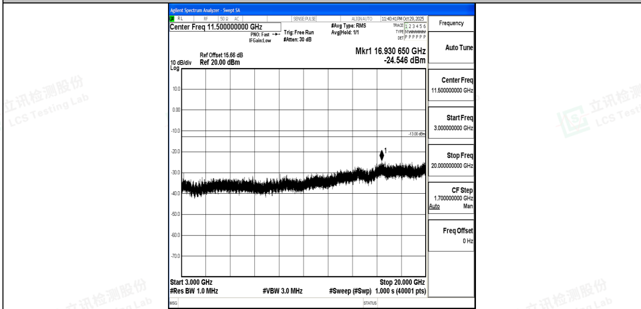
Band4_10MHz_16QAM_20350_1RB#0_3000~20000_3000~20000
