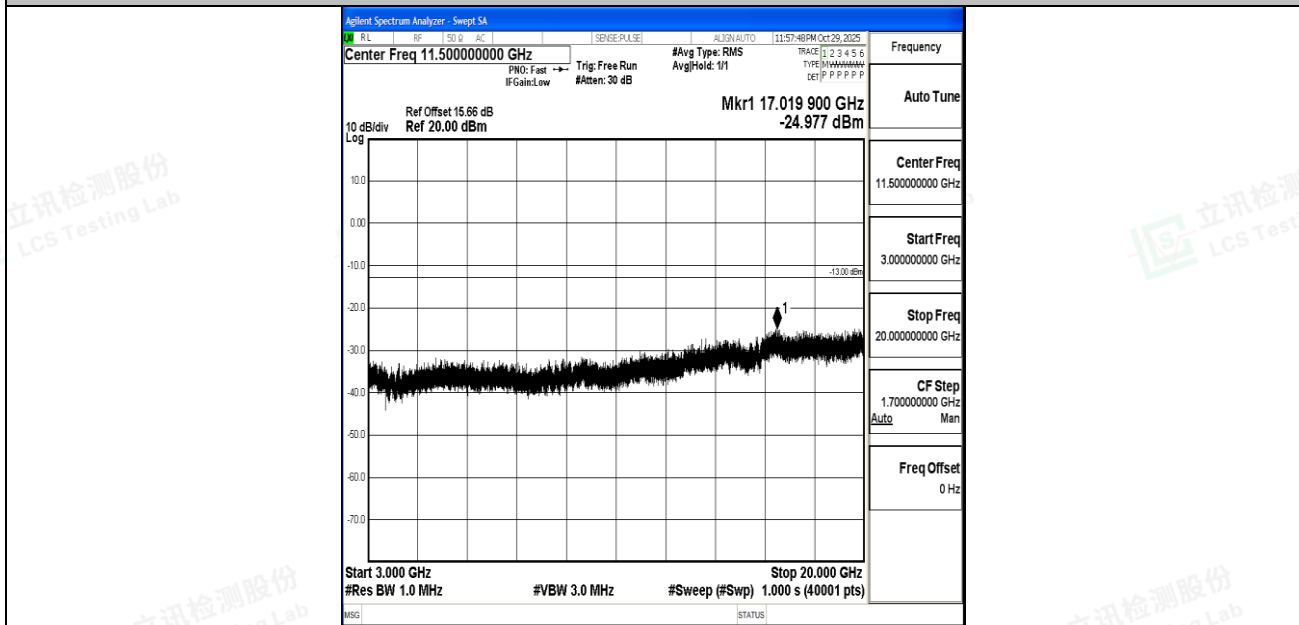
Band4_15MHz_16QAM_20325_1RB#0_3000~20000_3000~20000
