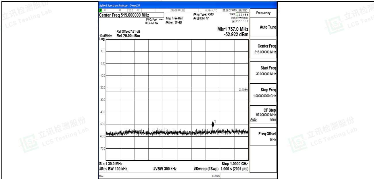
Band4_10MHz_QPSK_20350_1RB#0_30~1000_30~1000
