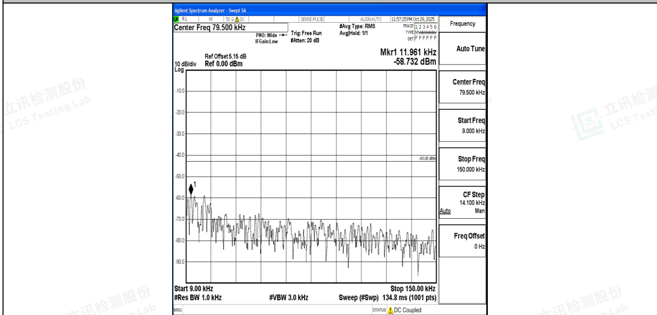
Band4_15MHz_16QAM_20325_1RB#0_0.009~0.15_0.009~0.15
