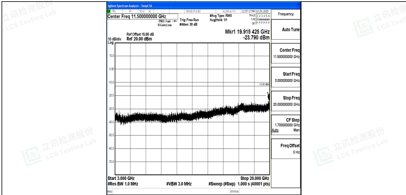
Band4_15MHz_QPSK_20325_1RB#0_3000~20000_3000~20000
