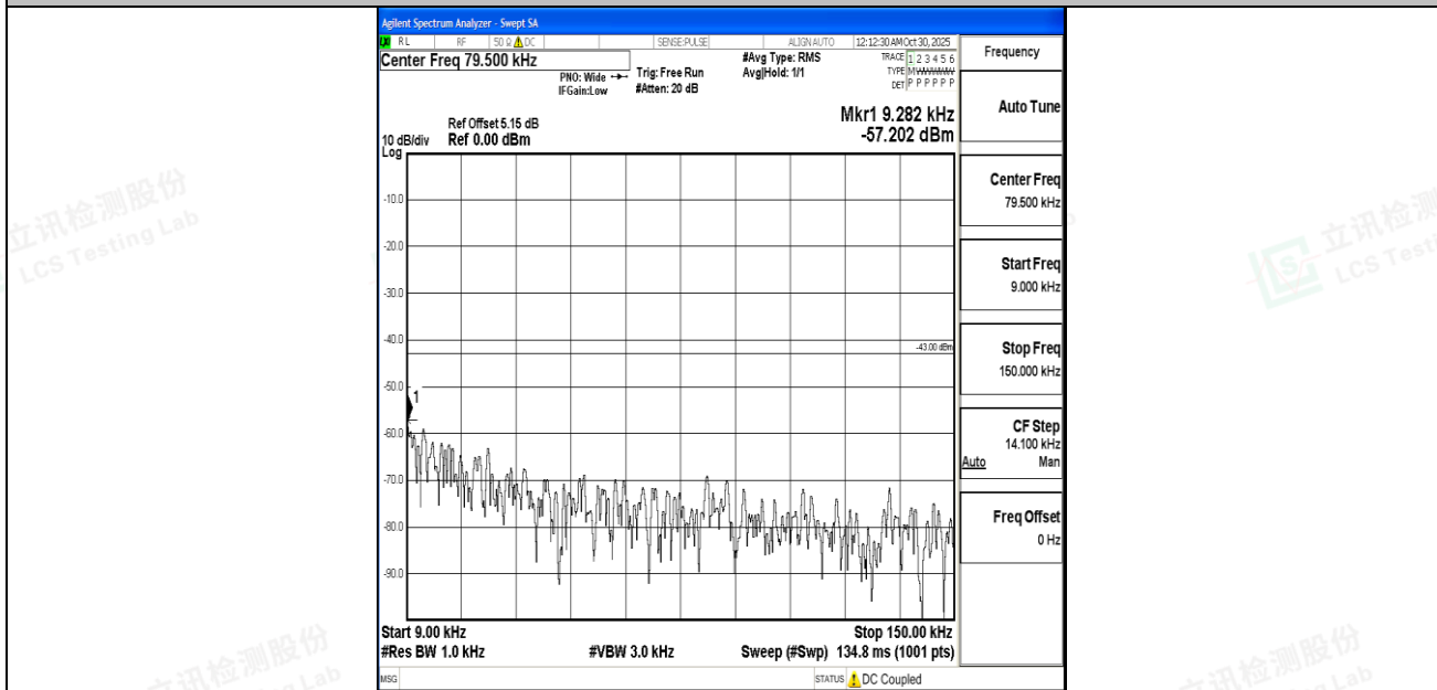
Band4_20MHz_16QAM_20050_1RB#0_0.009~0.15_0.009~0.15
