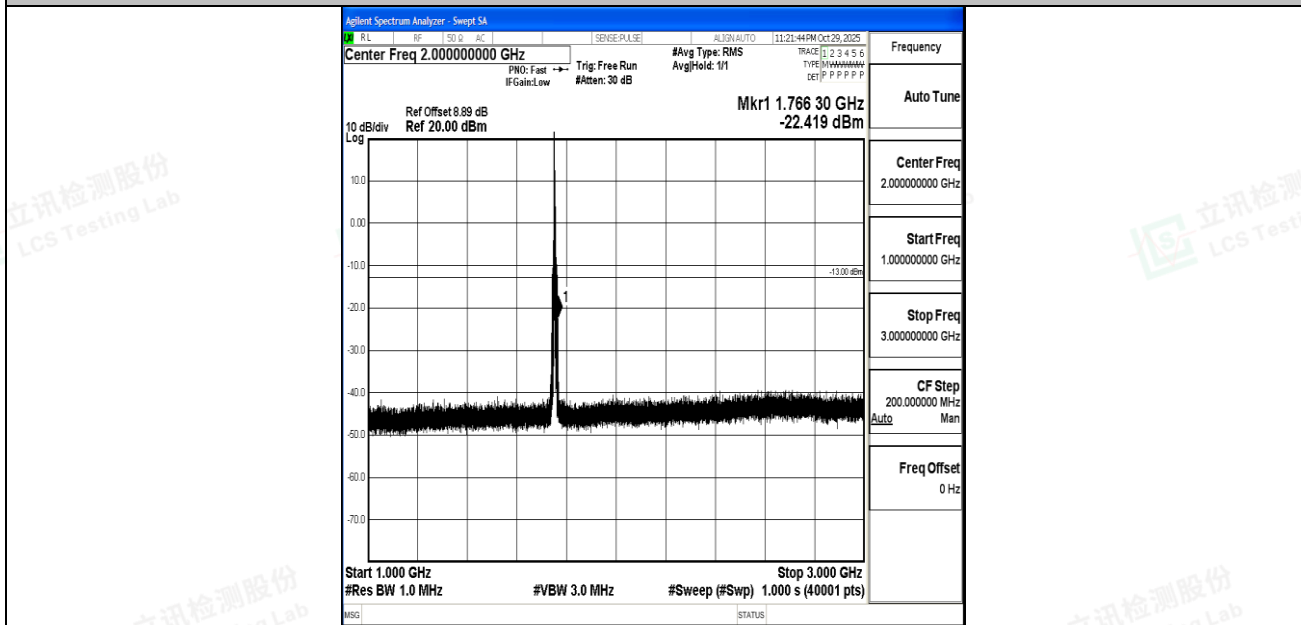
Band4_5MHz_QPSK_20375_1RB#0_1000~3000_1000~3000
