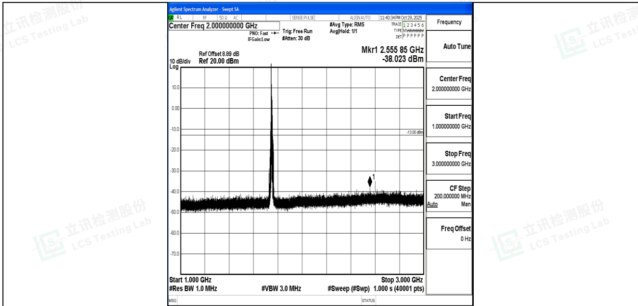
Band4_10MHz_16QAM_20350_1RB#0_1000~3000_1000~3000
