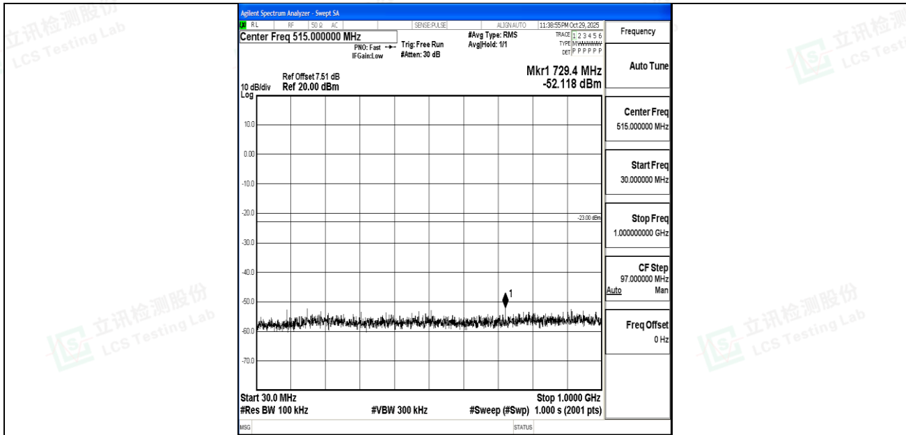
Band4_10MHz_QPSK_20175_1RB#0_30~1000_30~1000
