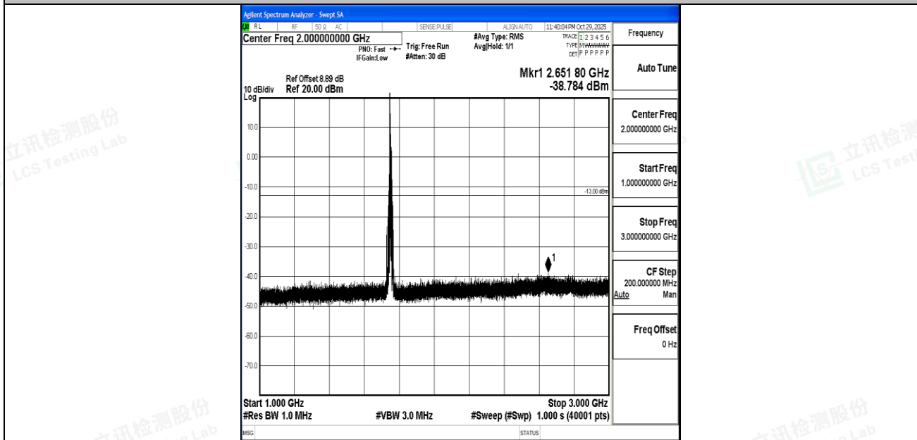
Band4_10MHz_QPSK_20350_1RB#0_1000~3000_1000~3000
