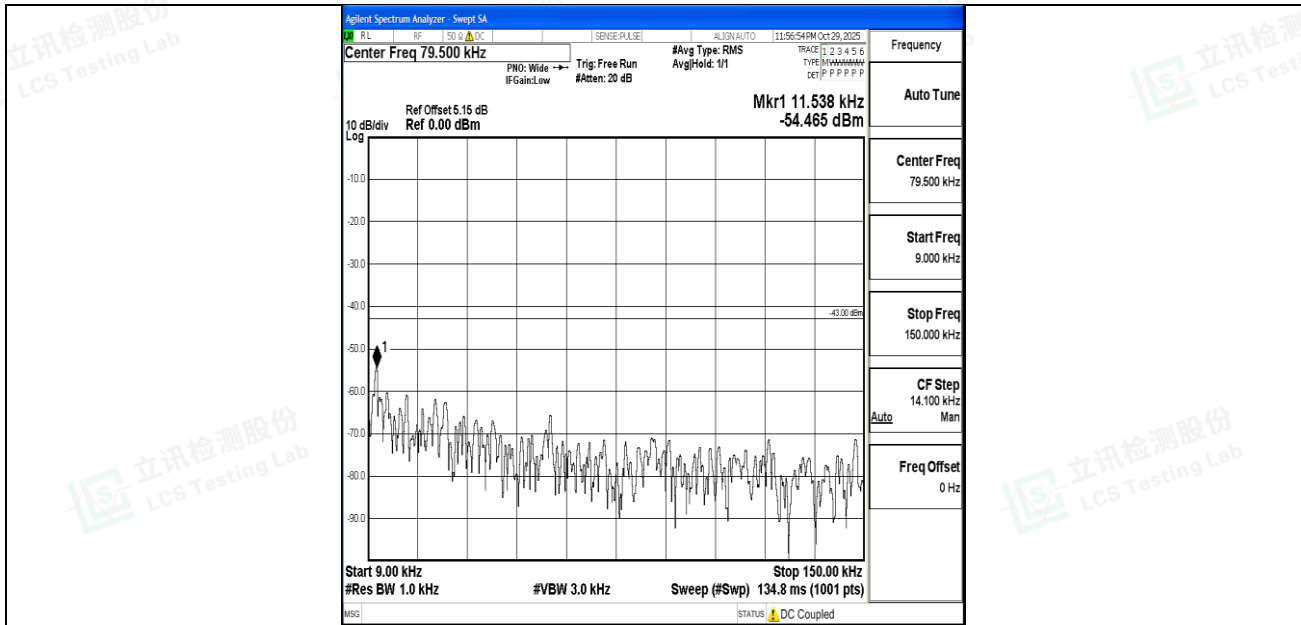
Band4_15MHz_QPSK_20325_1RB#0_0.009~0.15_0.009~0.15
