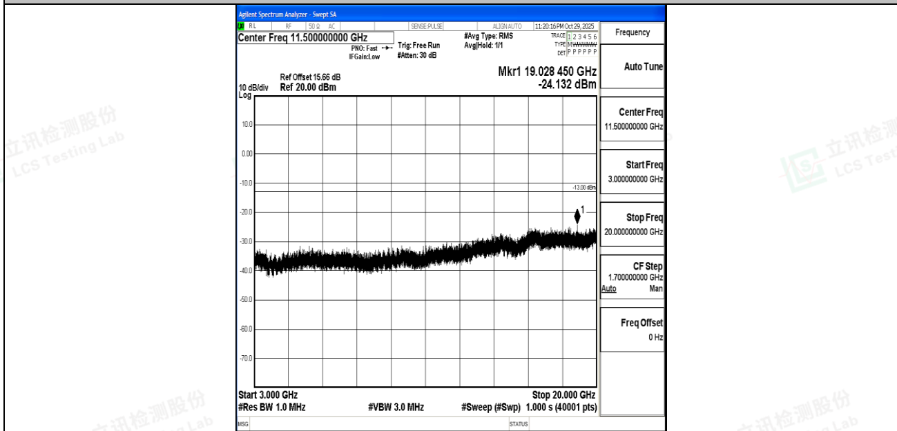
Band4_5MHz_16QAM_19975_1RB#0_3000~20000_3000~20000
