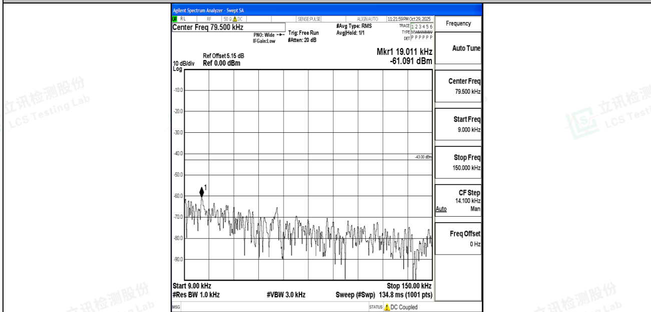
Band4_5MHz_16QAM_20375_1RB#0_0.009~0.15_0.009~0.15
