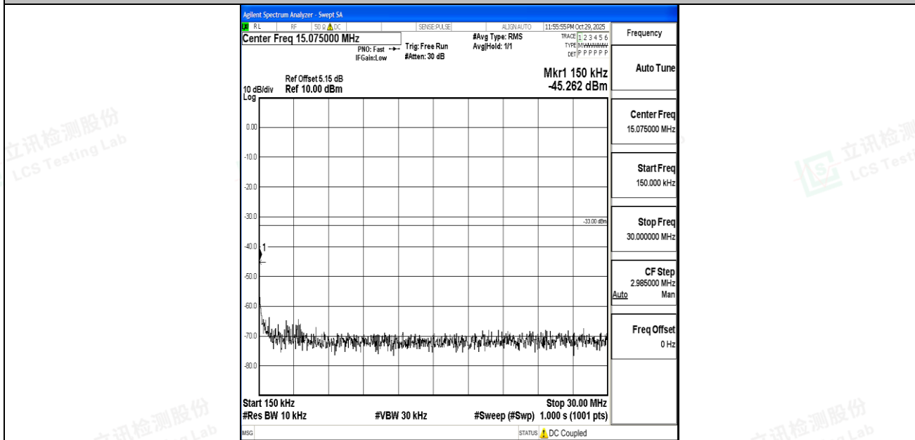
Band4_15MHz_QPSK_20175_1RB#0_0.15~30_0.15~30
