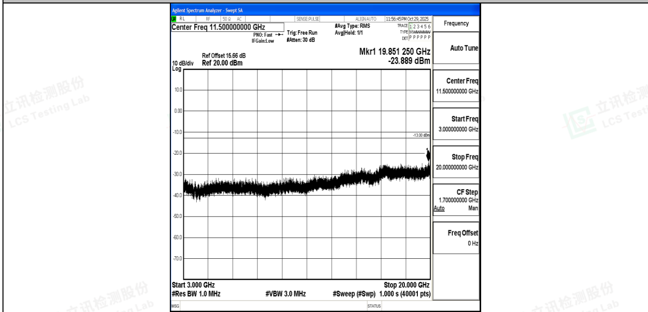
Band4_15MHz_16QAM_20175_1RB#0_3000~20000_3000~20000
