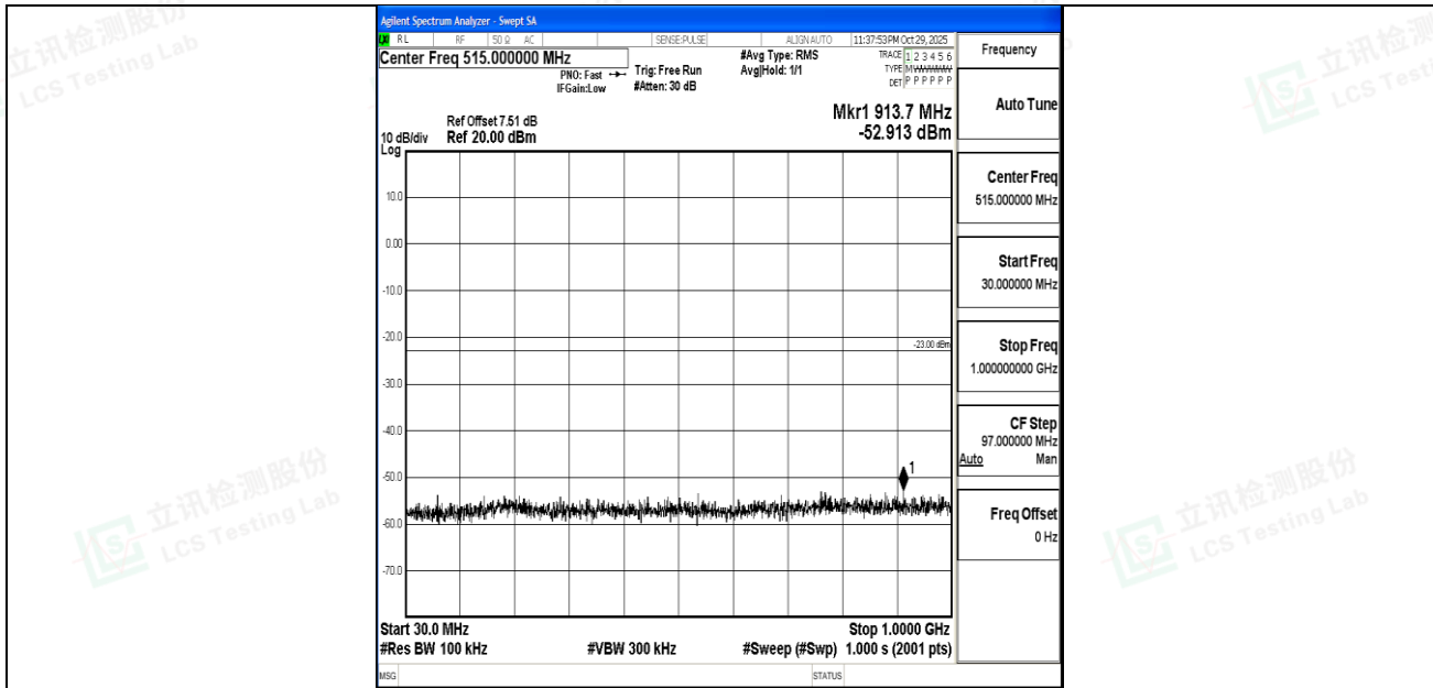
Band4_10MHz_QPSK_20000_1RB#0_30~1000_30~1000
