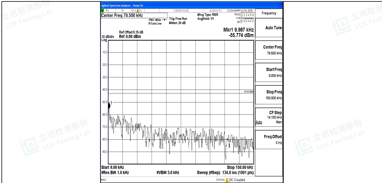
Band4_15MHz_QPSK_20025_1RB#0_0.009~0.15_0.009~0.15
