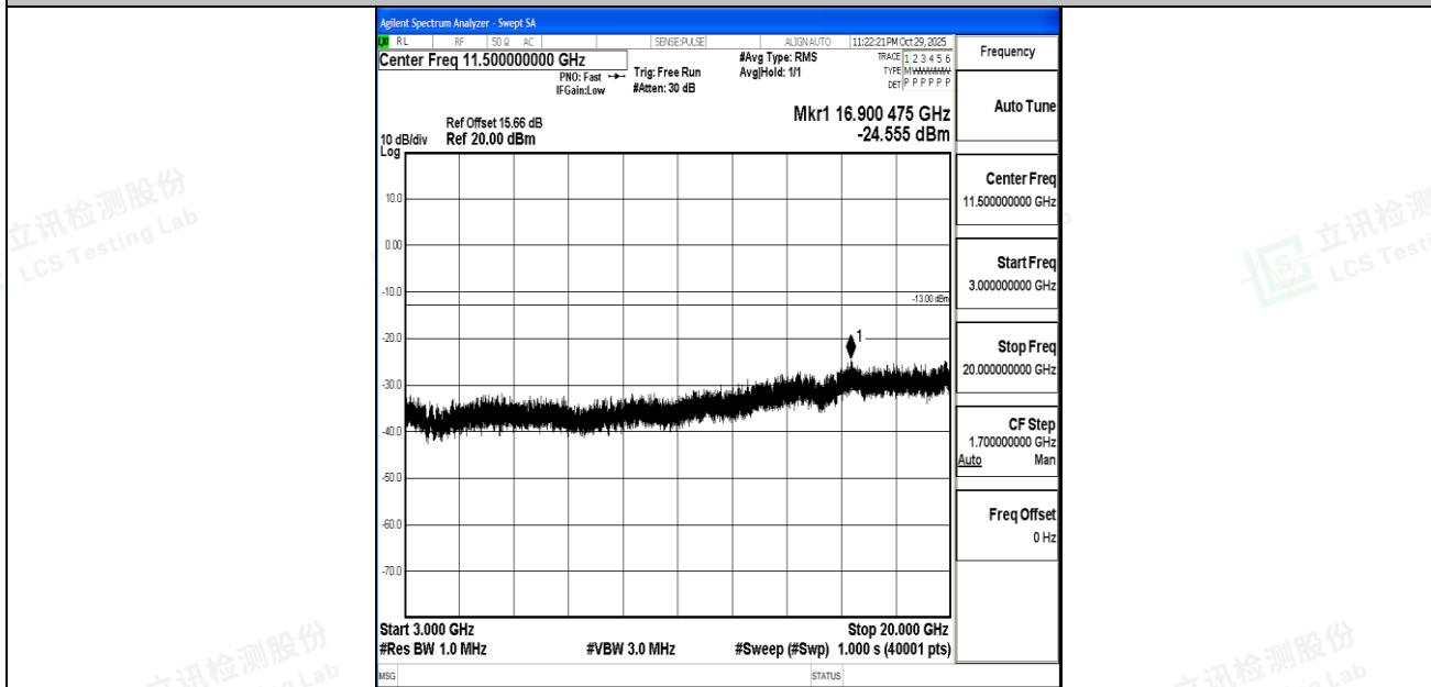
Band4_5MHz_16QAM_20375_1RB#0_3000~20000_3000~20000
