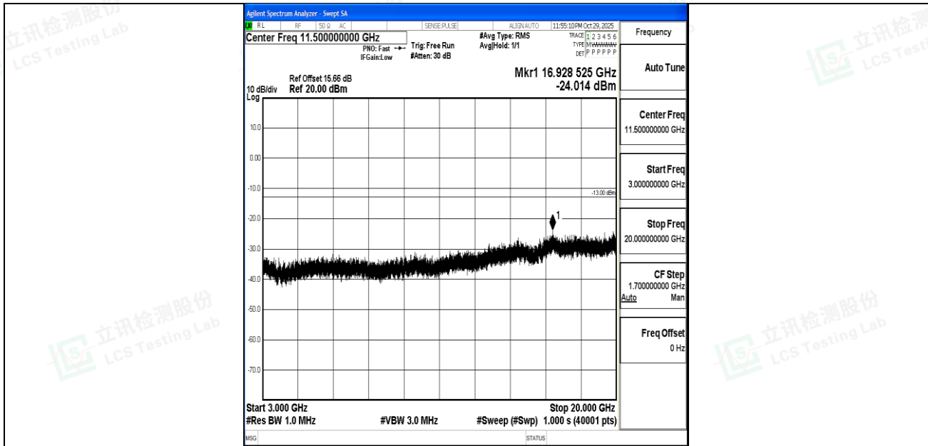
Band4_15MHz_QPSK_20025_1RB#0_3000~20000_3000~20000
