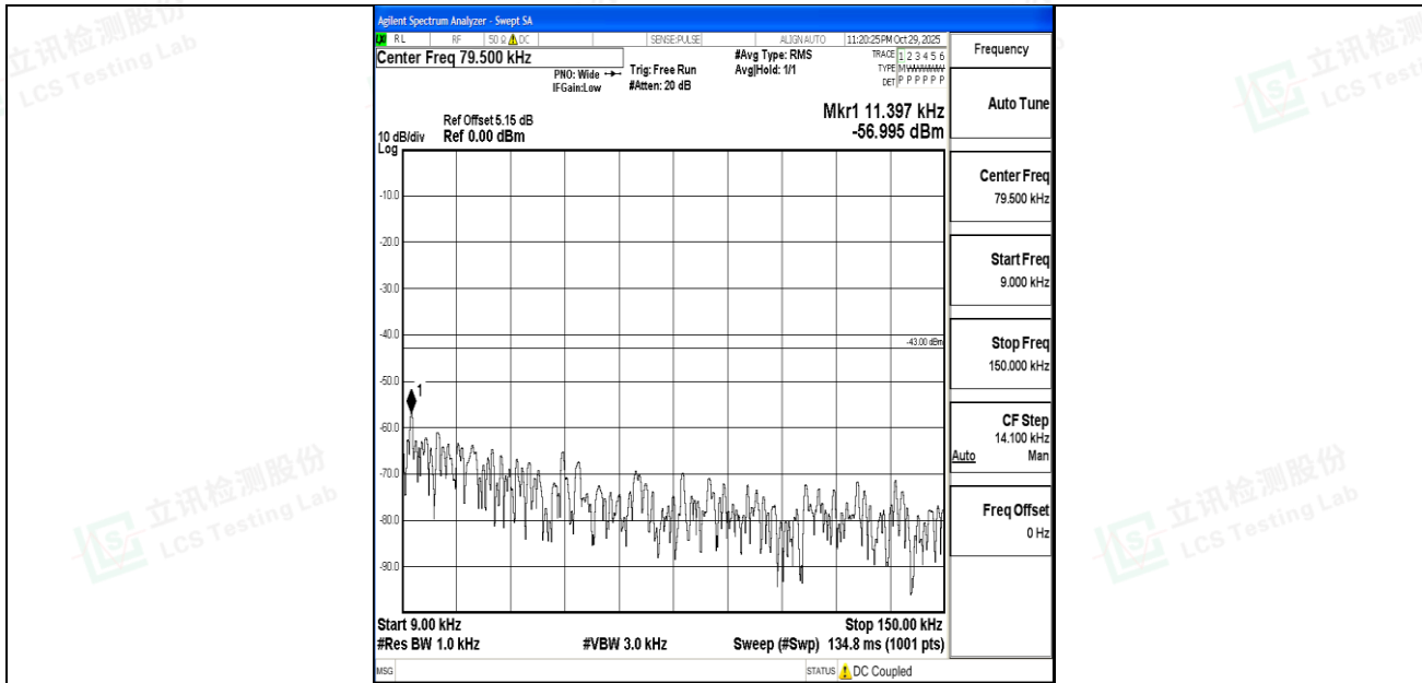
Band4_5MHz_QPSK_20175_1RB#0_0.009~0.15_0.009~0.15
