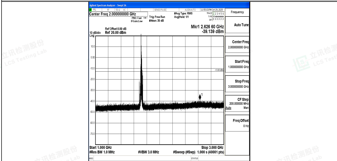
Band4_15MHz_QPSK_20025_1RB#0_1000~3000_1000~3000
