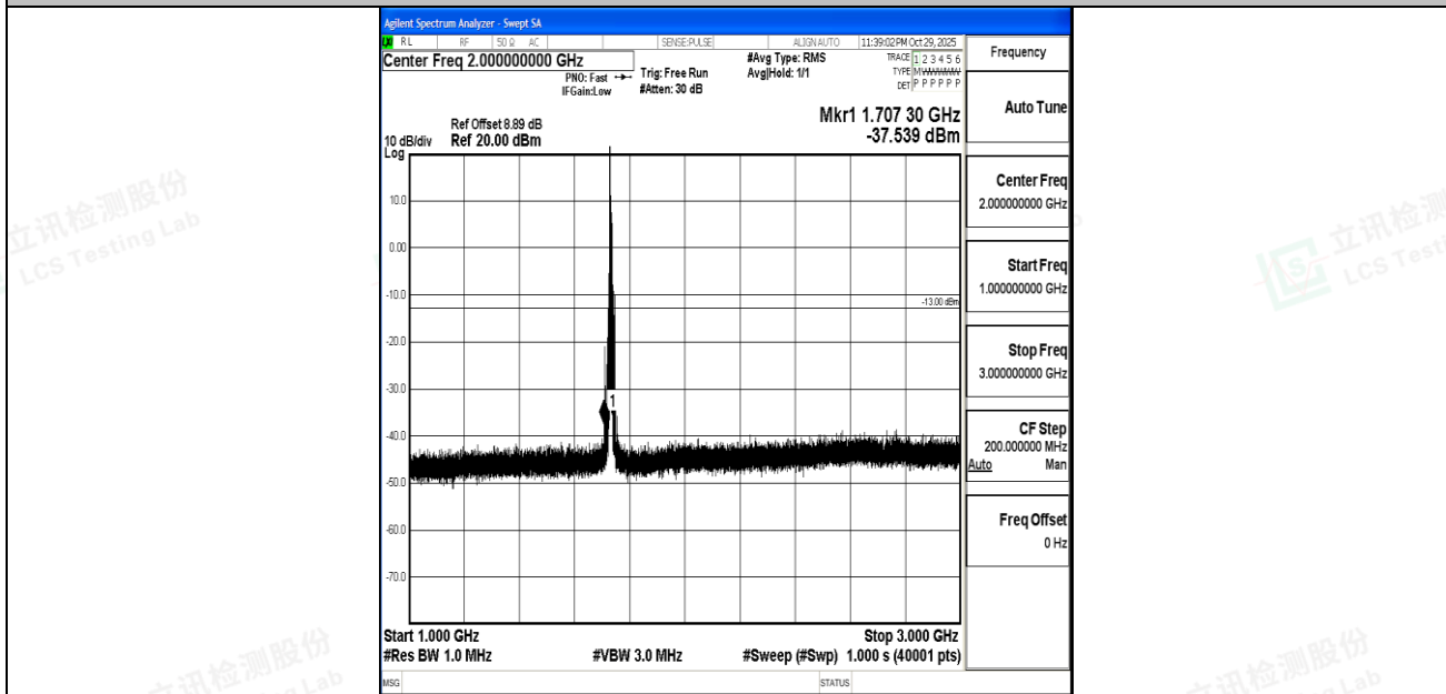
Band4_10MHz_QPSK_20175_1RB#0_1000~3000_1000~3000
