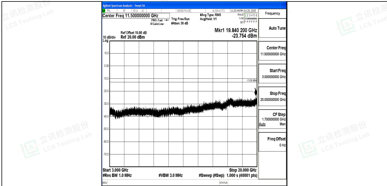
Band4_5MHz_QPSK_20175_1RB#0_3000~20000_3000~20000
