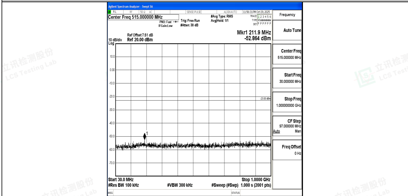
Band4_15MHz_16QAM_20175_1RB#0_30~1000_30~1000
