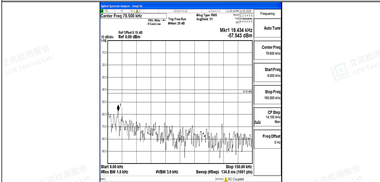
Band4_10MHz_16QAM_20175_1RB#0_0.009~0.15_0.009~0.15
