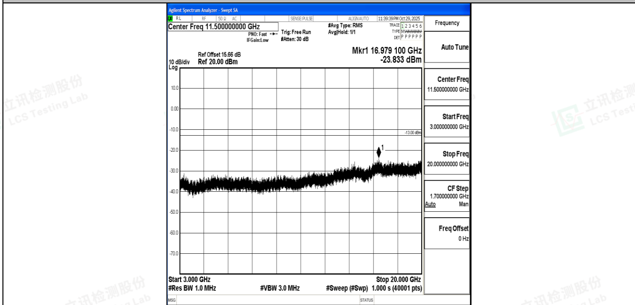
Band4_10MHz_16QAM_20175_1RB#0_3000~20000_3000~20000
