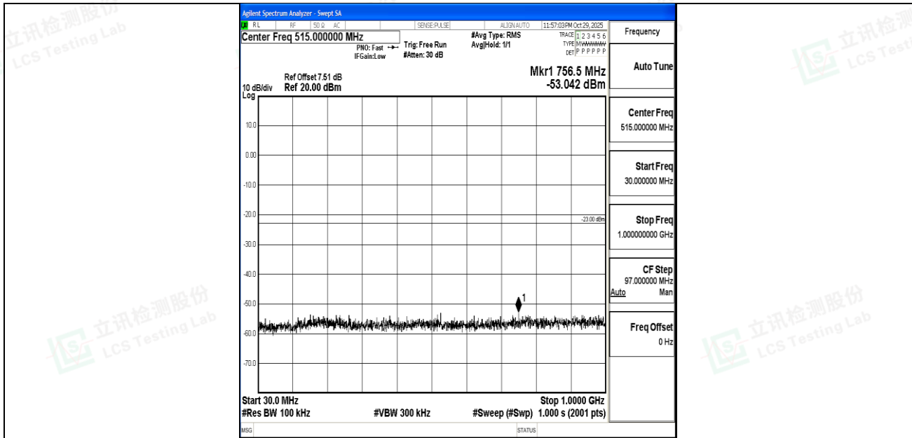
Band4_15MHz_QPSK_20325_1RB#0_30~1000_30~1000
