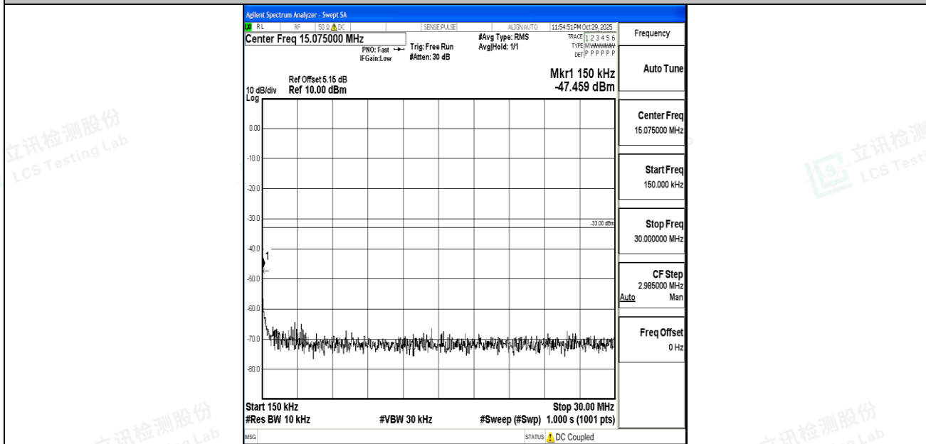
Band4_15MHz_QPSK_20025_1RB#0_0.15~30_0.15~30
