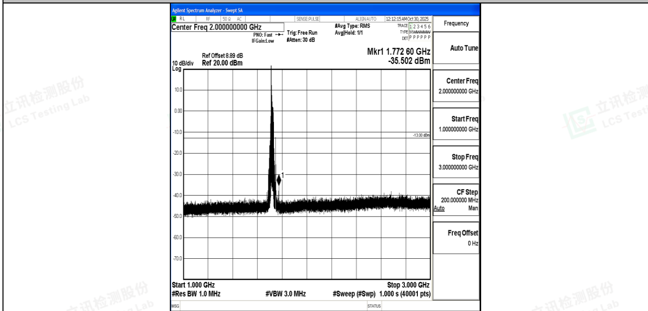
Band4_20MHz_QPSK_20050_1RB#0_1000~3000_1000~3000
