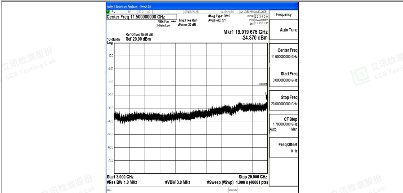
Band4_20MHz_16QAM_20050_1RB#0_3000~20000_3000~20000
