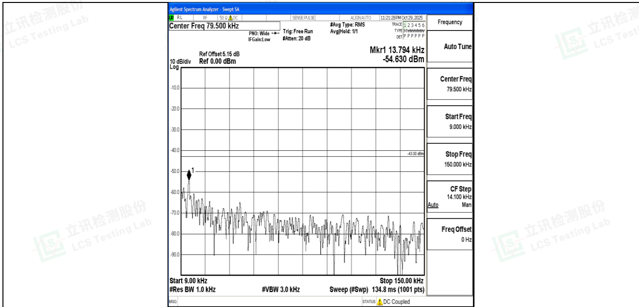
Band4_5MHz_QPSK_20375_1RB#0_0.009~0.15_0.009~0.15
