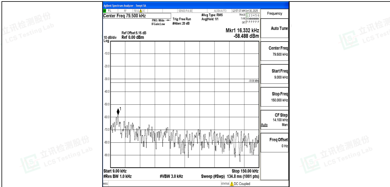
Band5_3MHz_QPSK_20635_1RB#0_0.009~0.15_0.009~0.15
