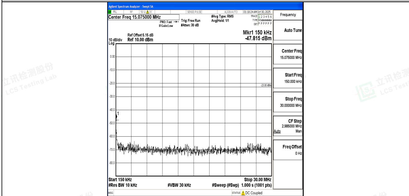
Band5_5MHz_QPSK_20625_1RB#0_0.15~30_0.15~30
