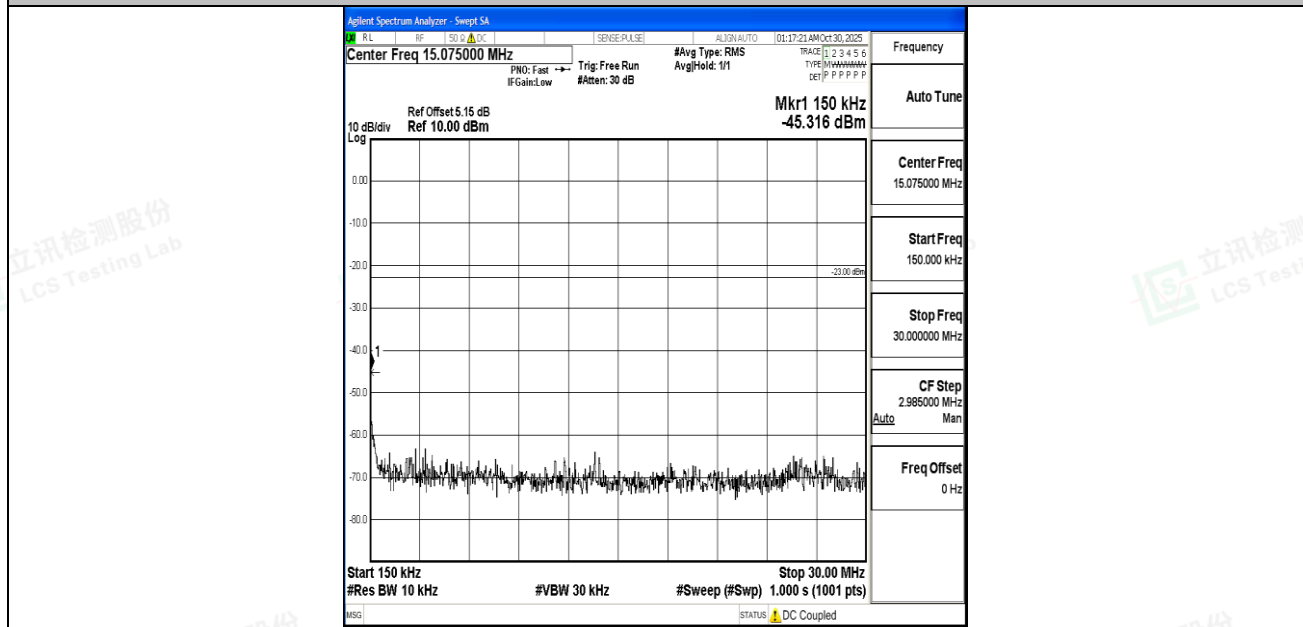
Band5_5MHz_QPSK_20525_1RB#0_0.15~30_0.15~30
