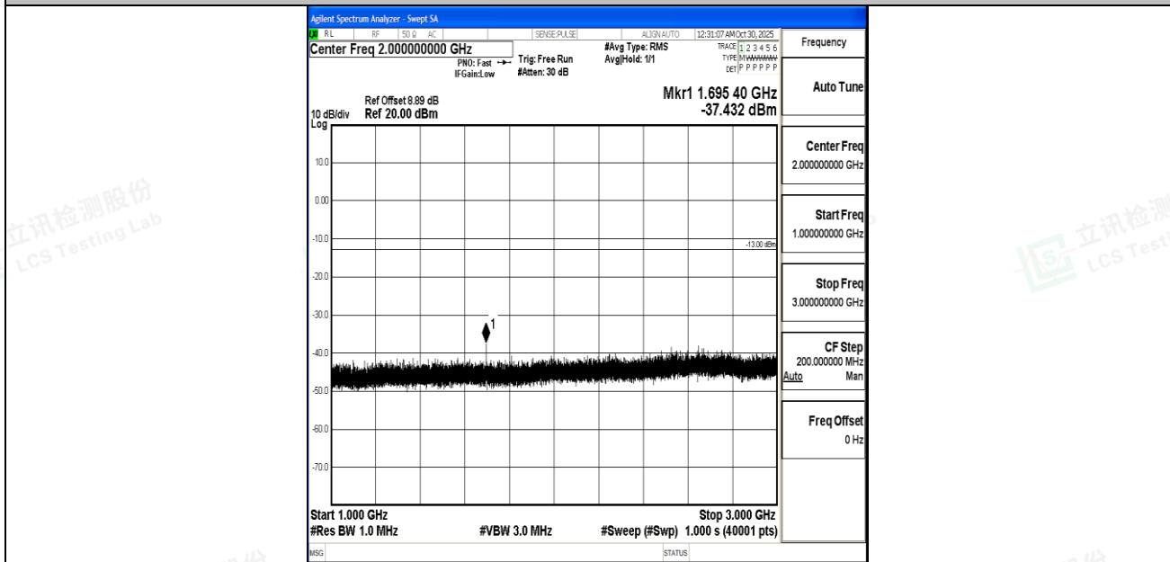
Band5_1.4MHz_QPSK_20643_1RB#0_1000~3000_1000~3000
