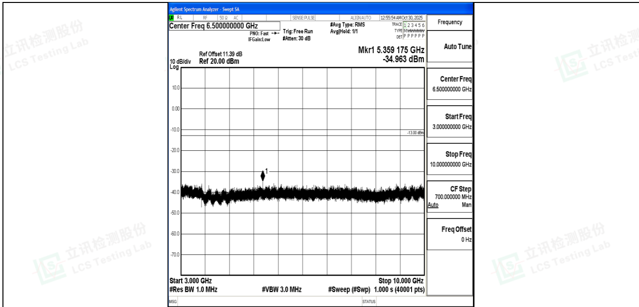
Band5_3MHz_QPSK_20415_1RB#0_3000~10000_3000~10000
