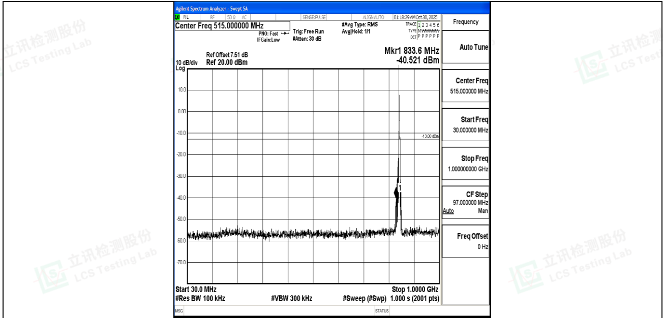
Band5_5MHz_QPSK_20625_1RB#0_30~1000_30~1000
