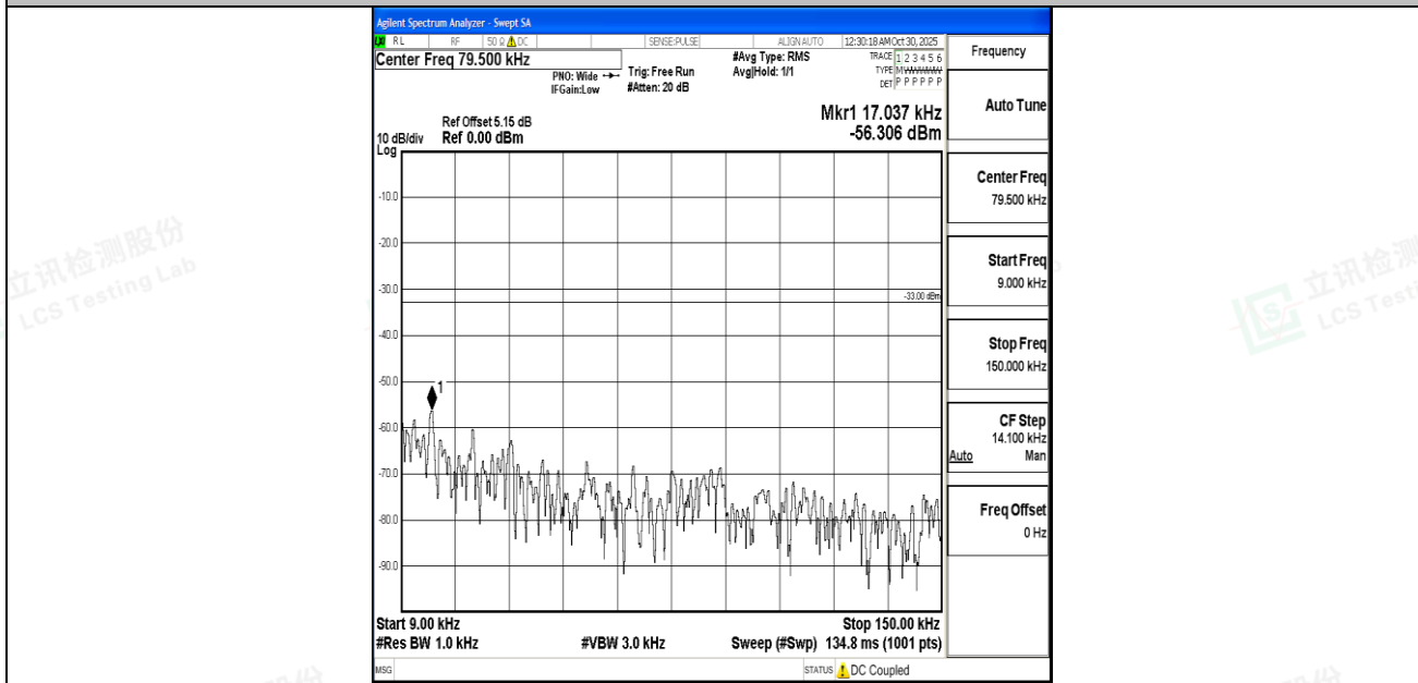
Band5_1.4MHz_16QAM_20525_1RB#0_0.009~0.15_0.009~0.15
