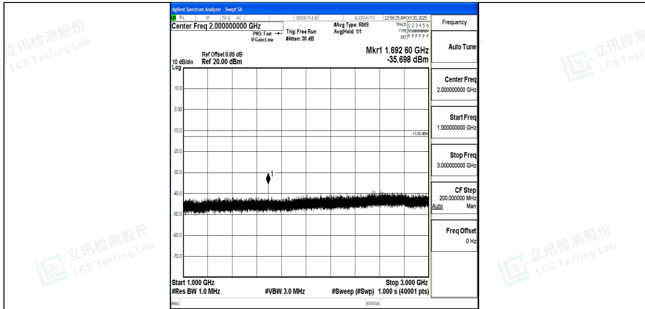
Band5_3MHz_16QAM_20635_1RB#0_1000~3000_1000~3000
