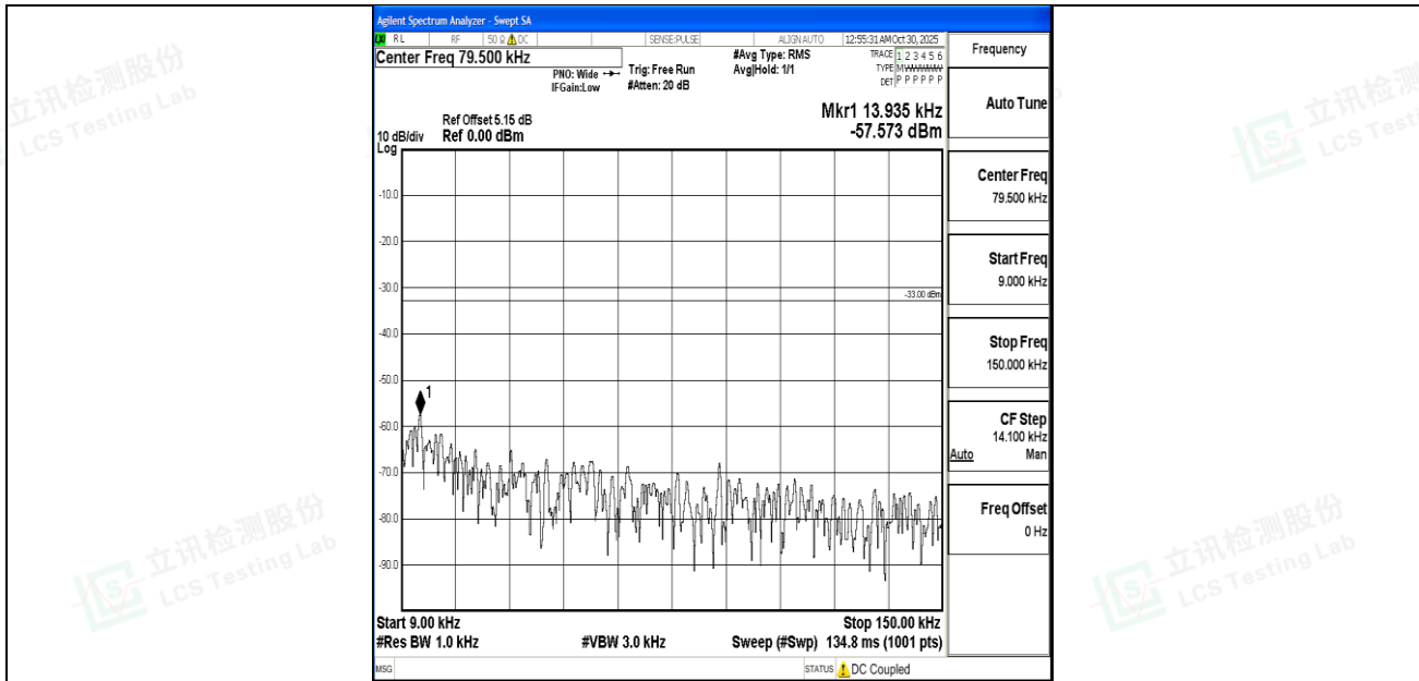
Band5_3MHz_QPSK_20415_1RB#0_0.009~0.15_0.009~0.15
