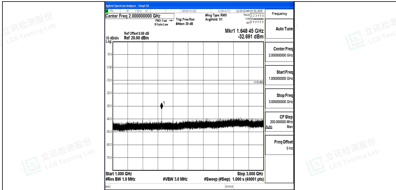
Band5_1.4MHz_16QAM_20407_1RB#0_1000~3000_1000~3000
