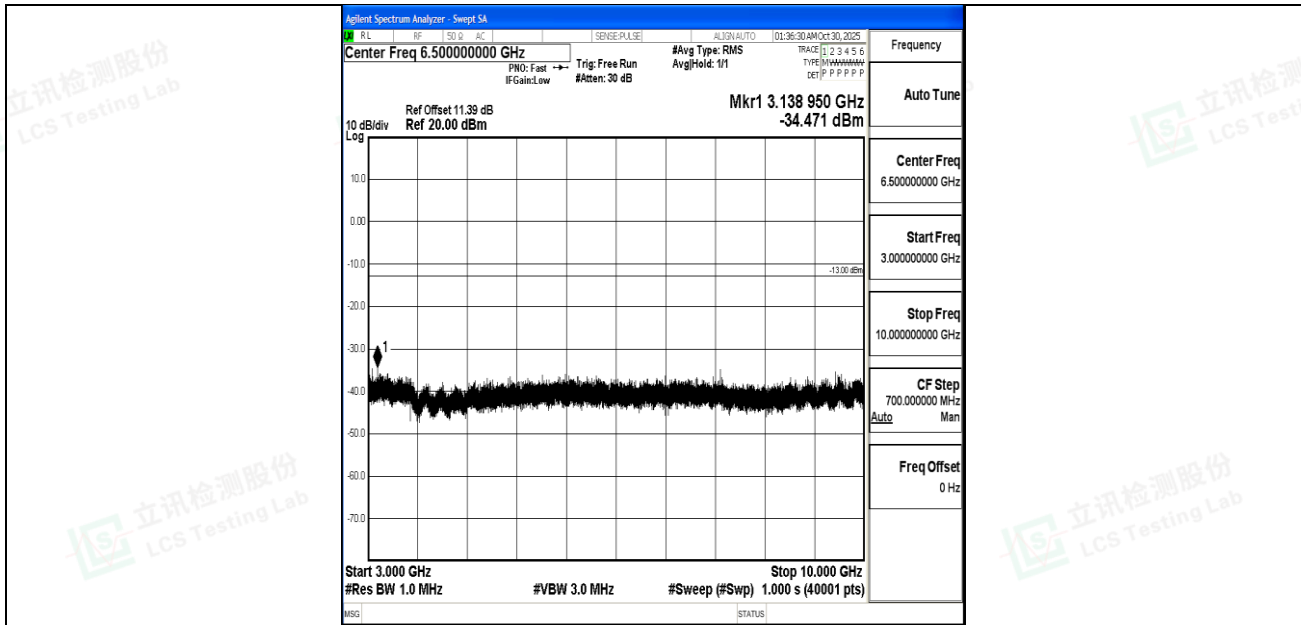
Band5_10MHz_QPSK_20450_1RB#0_3000~10000_3000~10000
