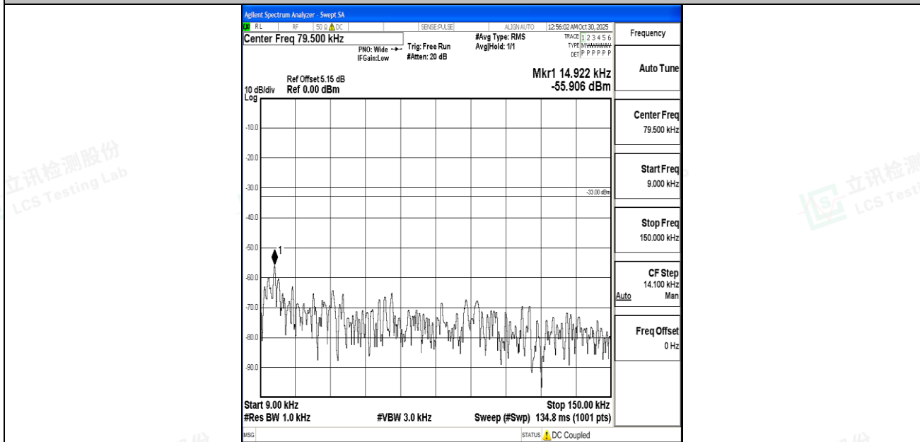
Band5_3MHz_16QAM_20415_1RB#0_0.009~0.15_0.009~0.15
