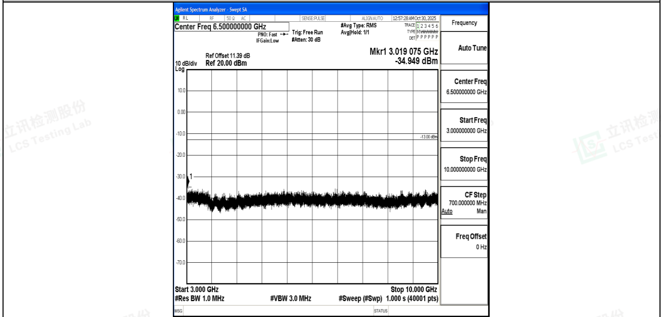
Band5_3MHz_16QAM_20525_1RB#0_3000~10000_3000~10000
