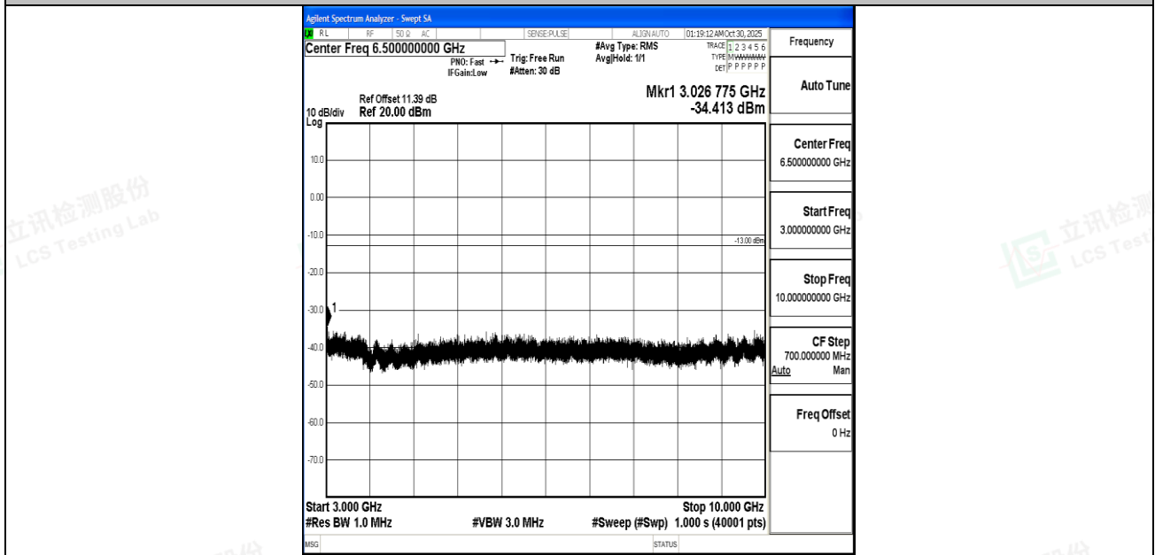
Band5_5MHz_16QAM_20625_1RB#0_3000~10000_3000~10000
