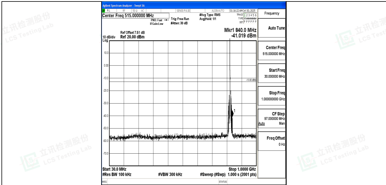
Band5_5MHz_QPSK_20425_1RB#0_30~1000_30~1000
