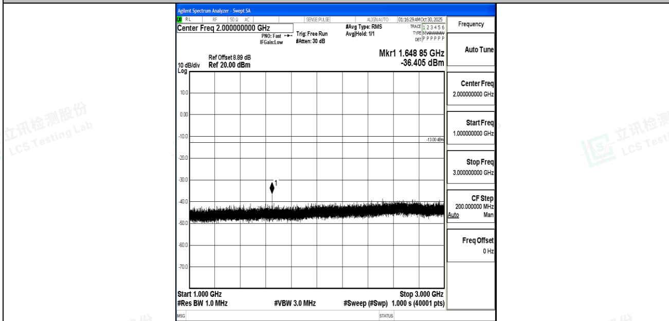
Band5_5MHz_QPSK_20425_1RB#0_1000~3000_1000~3000
