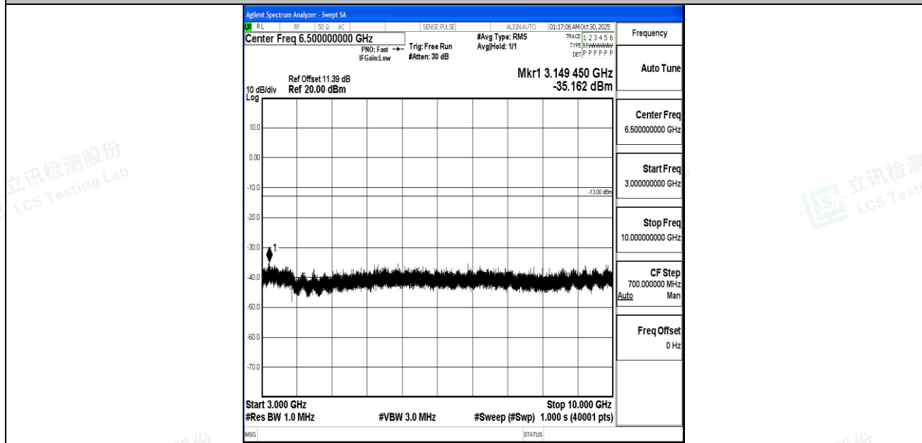
Band5_5MHz_16QAM_20425_1RB#0_3000~10000_3000~10000
