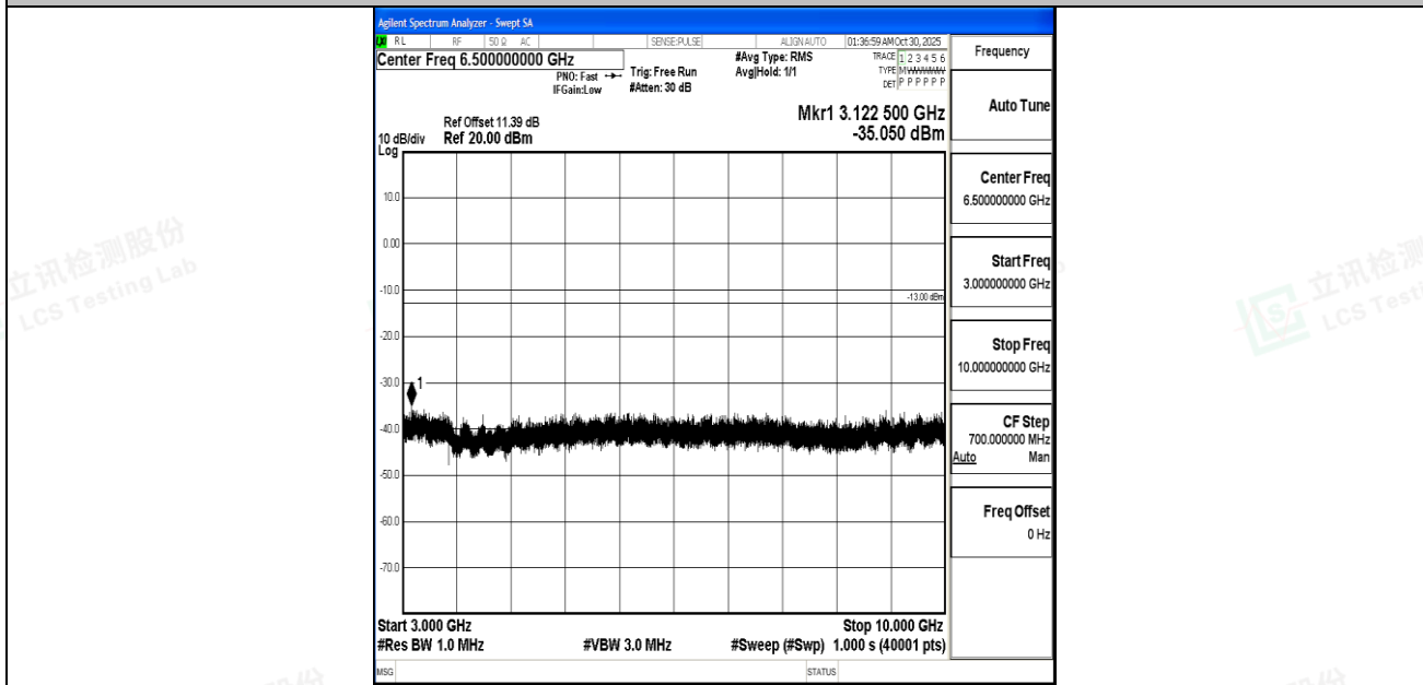
Band5_10MHz_16QAM_20450_1RB#0_3000~10000_3000~10000
