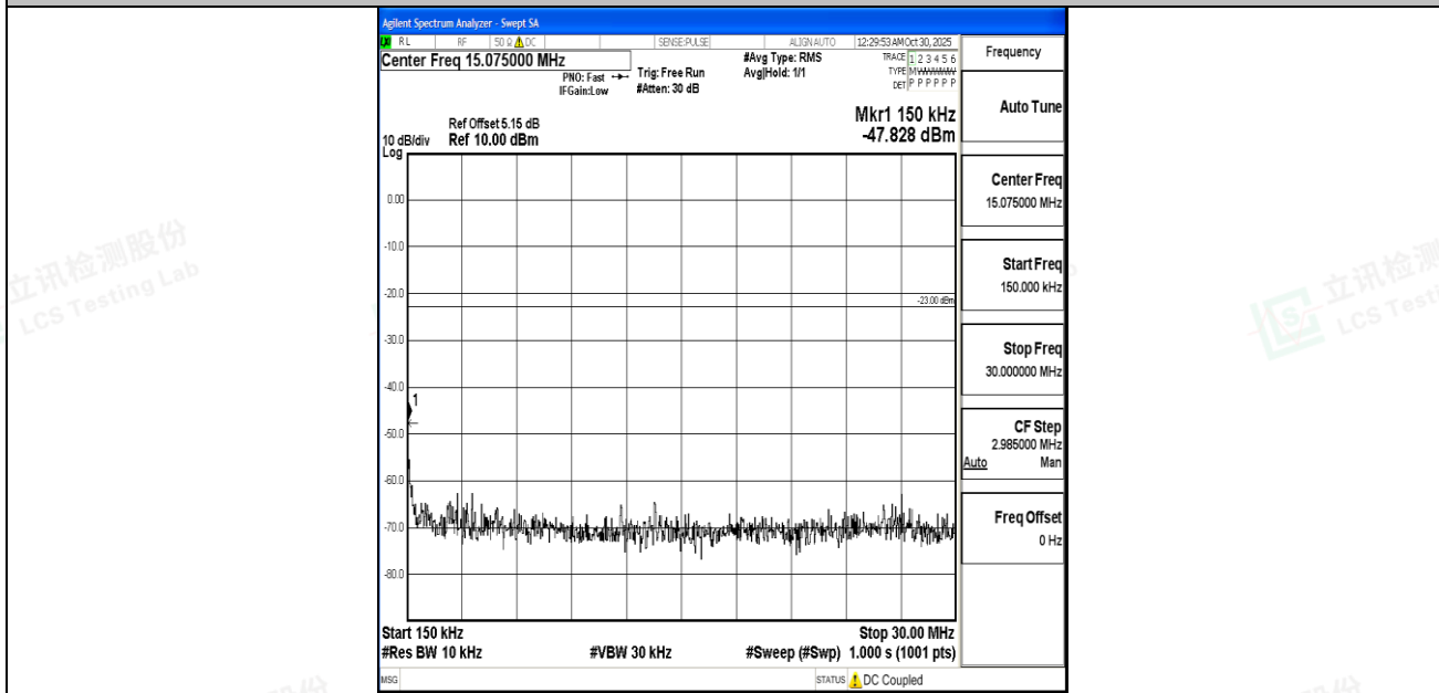
Band5_1.4MHz_QPSK_20525_1RB#0_0.15~30_0.15~30
