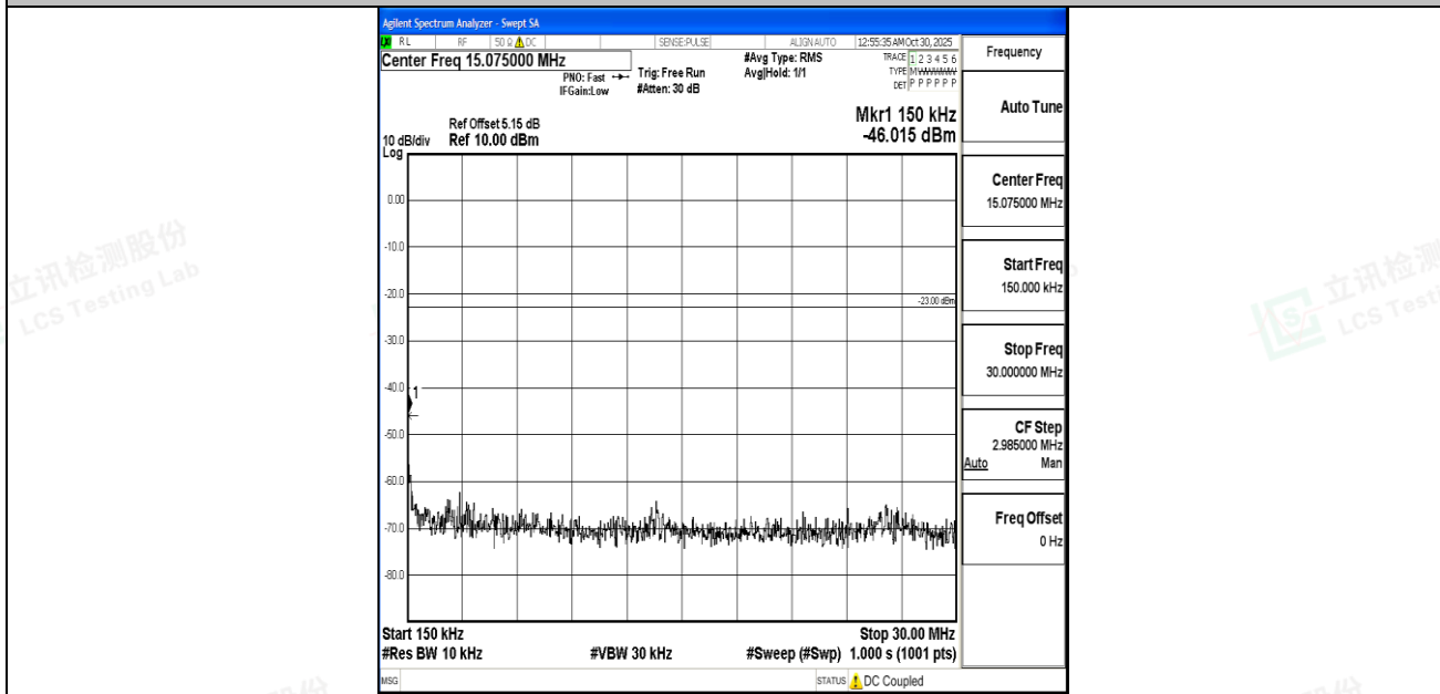
Band5_3MHz_QPSK_20415_1RB#0_0.15~30_0.15~30
