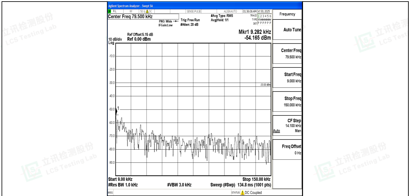
Band5_10MHz_QPSK_20450_1RB#0_0.009~0.15_0.009~0.15
