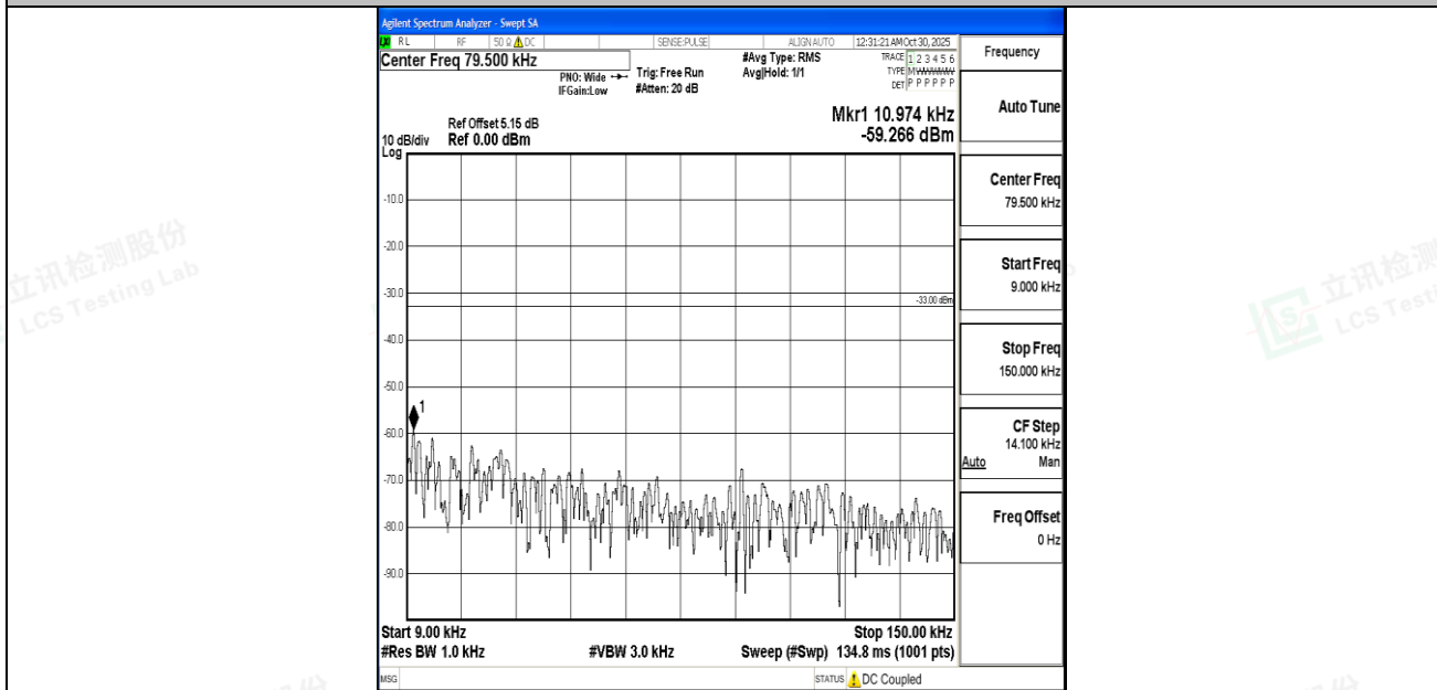
Band5_1.4MHz_16QAM_20643_1RB#0_0.009~0.15_0.009~0.15
