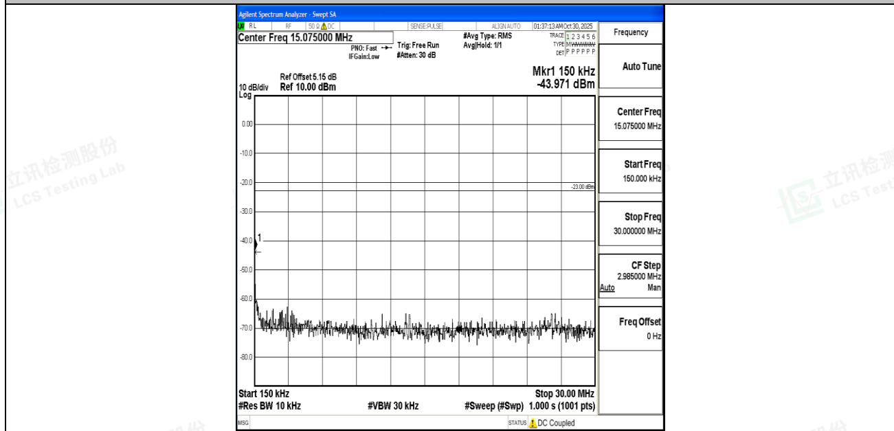
Band5_10MHz_QPSK_20525_1RB#0_0.15~30_0.15~30
