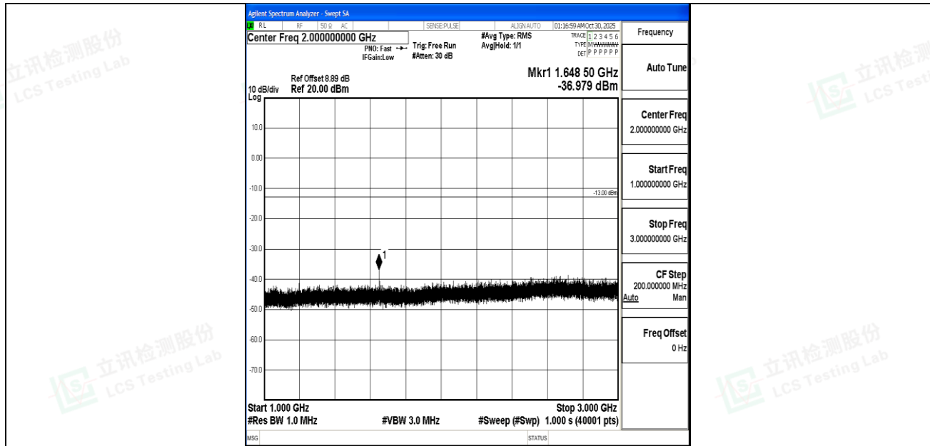
Band5_5MHz_16QAM_20425_1RB#0_1000~3000_1000~3000
