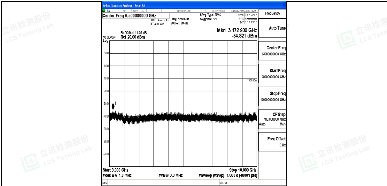
Band5_1.4MHz_QPSK_20643_1RB#0_3000~10000_3000~10000
