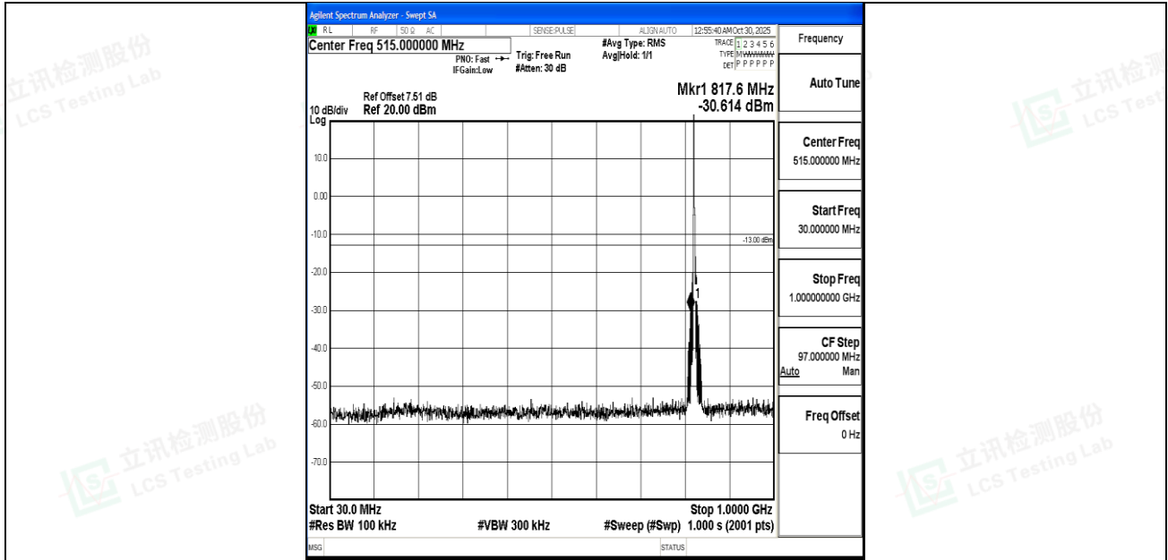
Band5_3MHz_QPSK_20415_1RB#0_30~1000_30~1000
