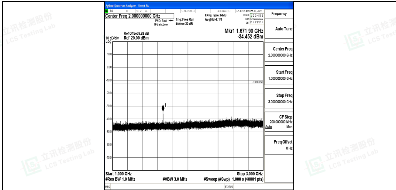
Band5_1.4MHz_16QAM_20525_1RB#0_1000~3000_1000~3000
