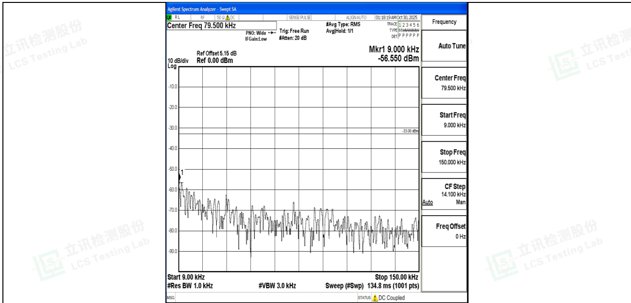
Band5_5MHz_QPSK_20625_1RB#0_0.009~0.15_0.009~0.15
