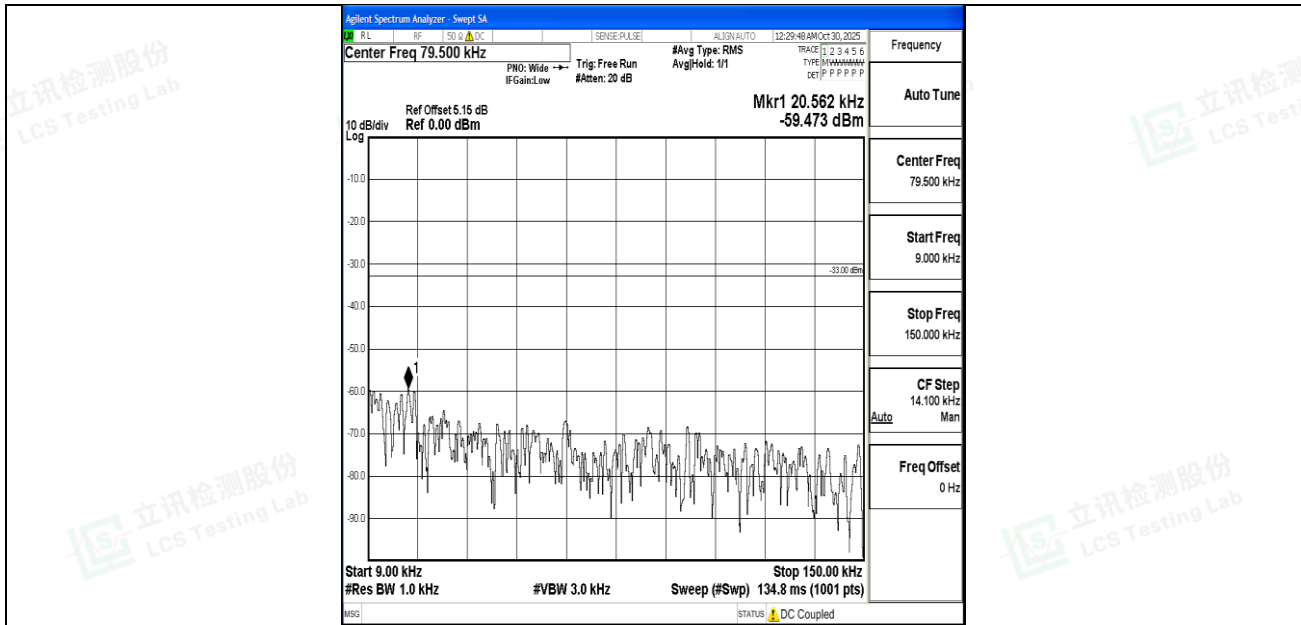
Band5_1.4MHz_QPSK_20525_1RB#0_0.009~0.15_0.009~0.15
