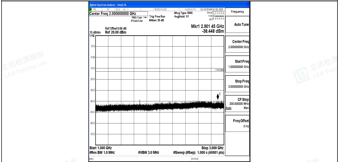
Band5_5MHz_QPSK_20625_1RB#0_1000~3000_1000~3000
