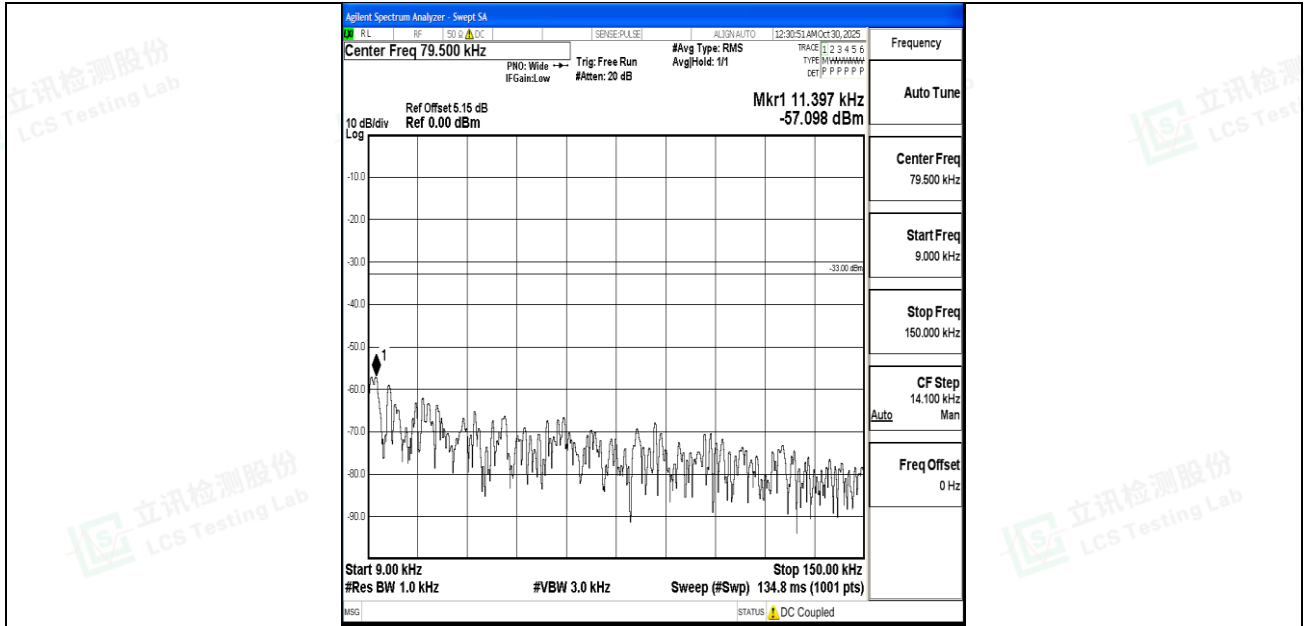
Band5_1.4MHz_QPSK_20643_1RB#0_0.009~0.15_0.009~0.15
