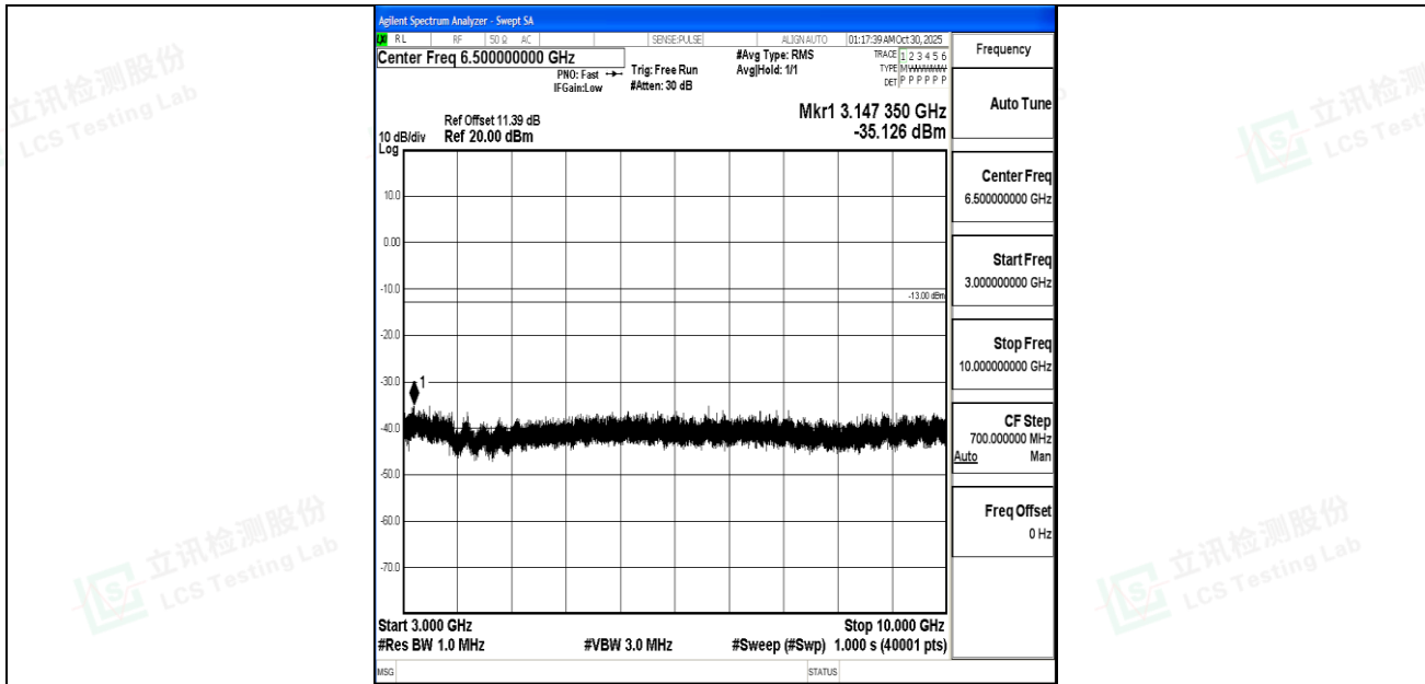
Band5_5MHz_QPSK_20525_1RB#0_3000~10000_3000~10000
