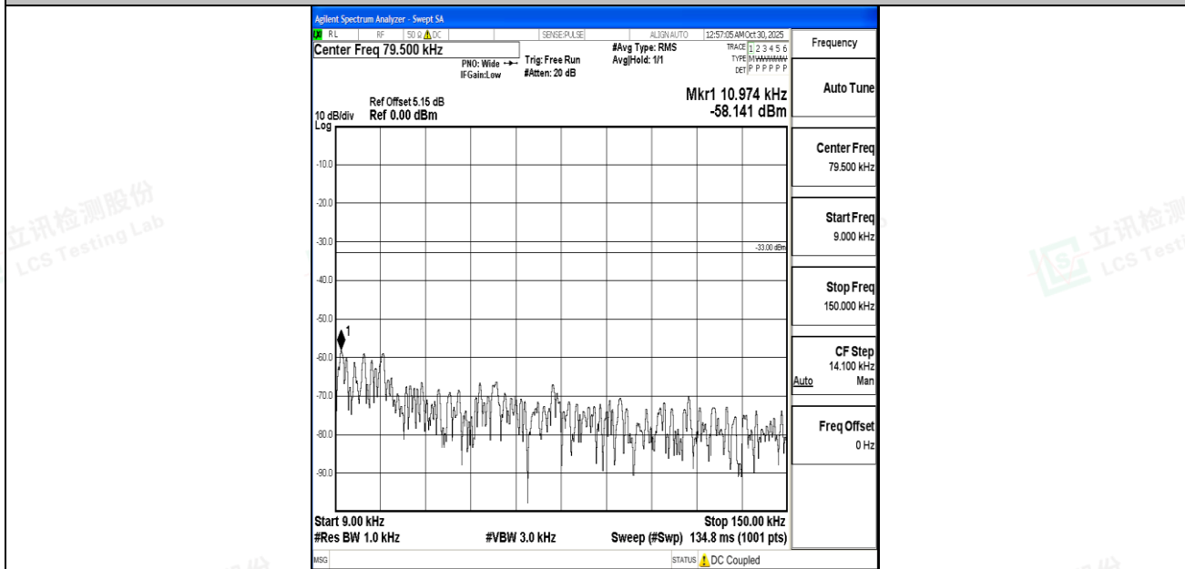
Band5_3MHz_16QAM_20525_1RB#0_0.009~0.15_0.009~0.15
