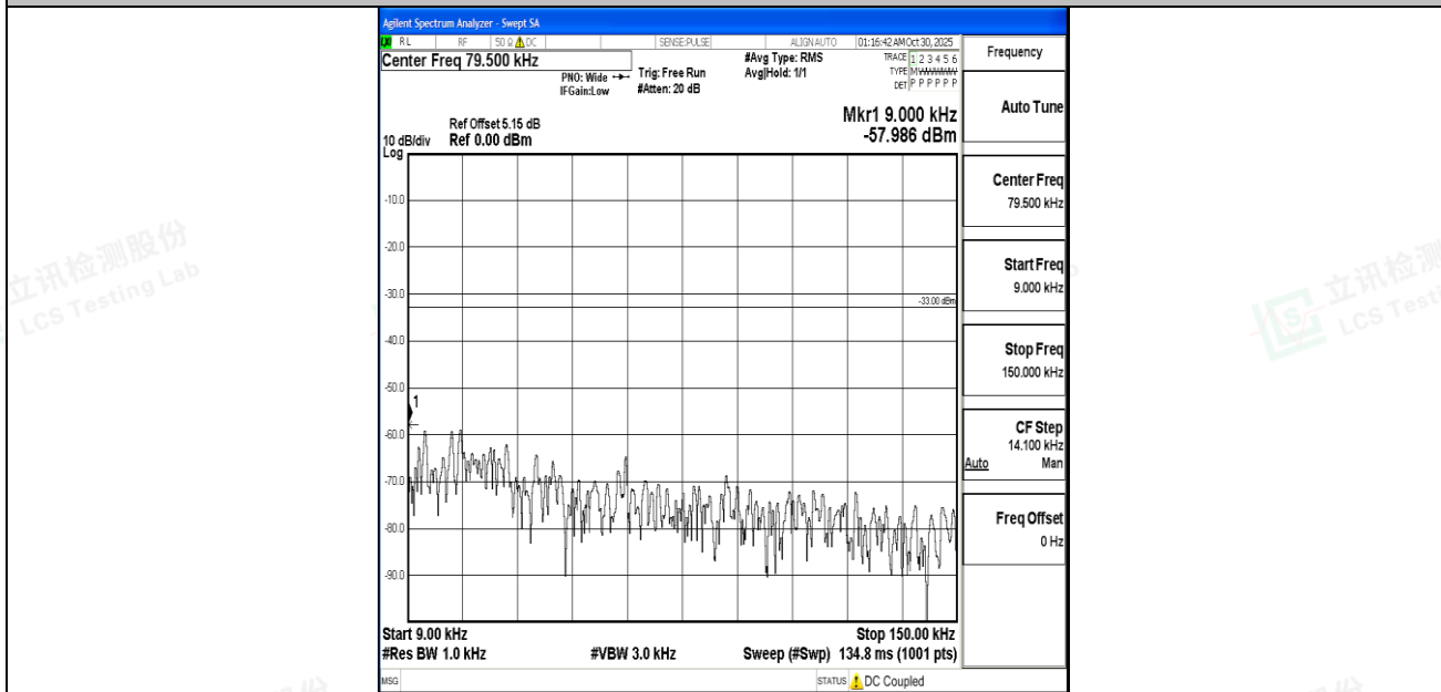
Band5_5MHz_16QAM_20425_1RB#0_0.009~0.15_0.009~0.15
