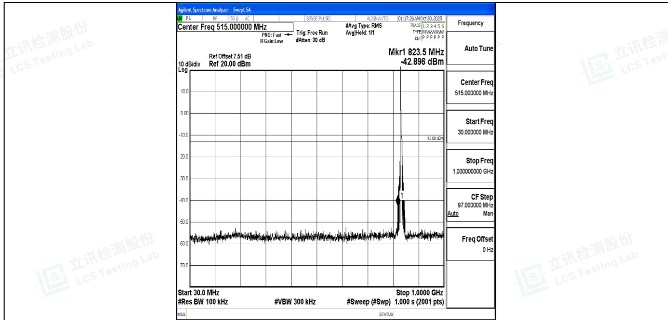
Band5_5MHz_QPSK_20525_1RB#0_30~1000_30~1000
