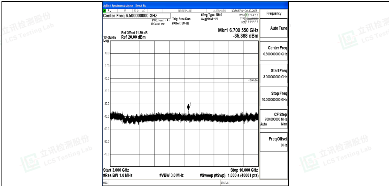
Band5_3MHz_QPSK_20525_1RB#0_3000~10000_3000~10000
