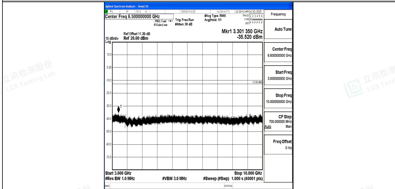
Band5_1.4MHz_16QAM_20525_1RB#0_3000~10000_3000~10000
