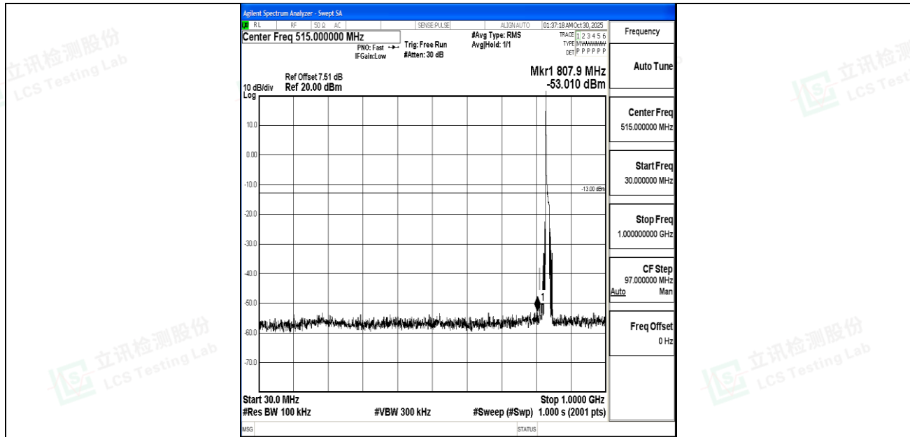
Band5_10MHz_QPSK_20525_1RB#0_30~1000_30~1000
