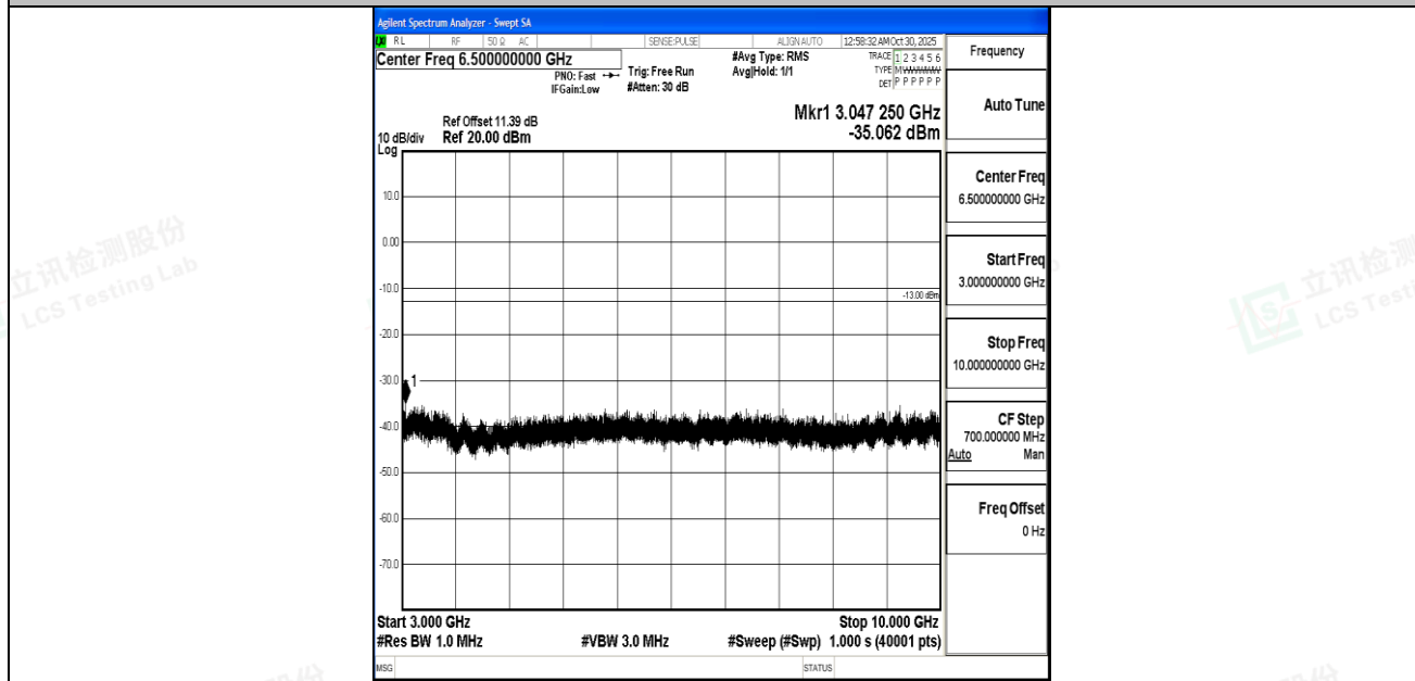
Band5_3MHz_16QAM_20635_1RB#0_3000~10000_3000~10000
