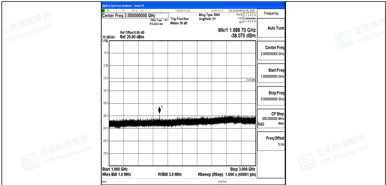
Band5_5MHz_16QAM_20625_1RB#0_1000~3000_1000~3000
