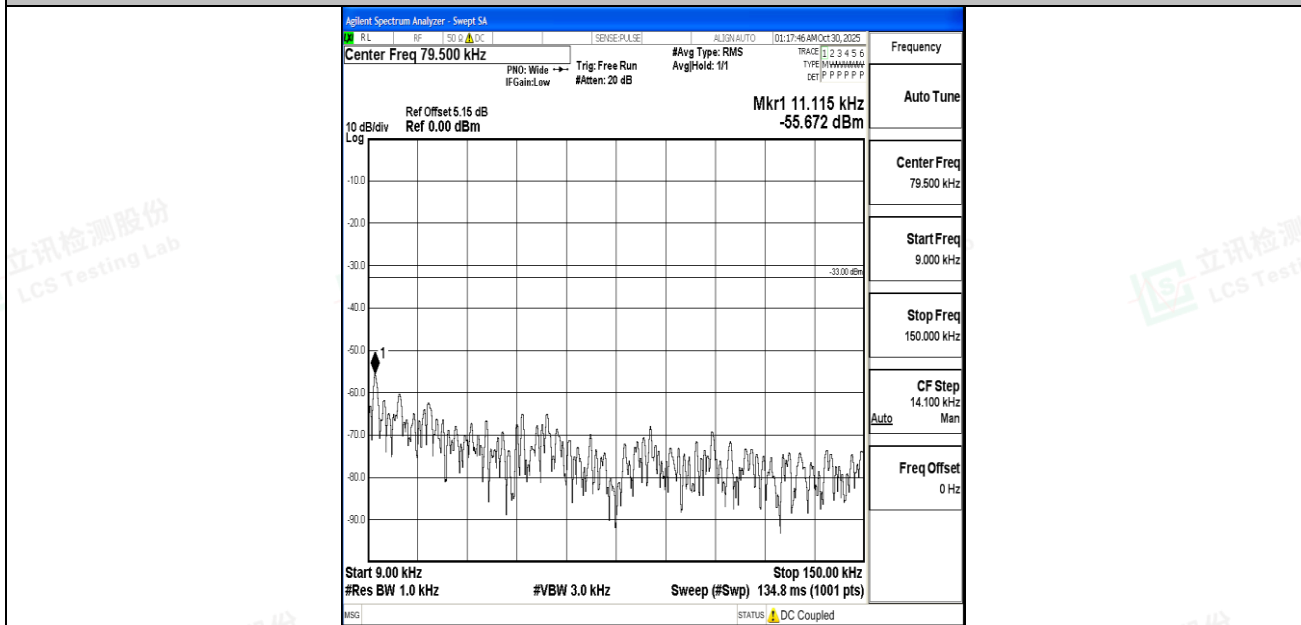
Band5_5MHz_16QAM_20525_1RB#0_0.009~0.15_0.009~0.15
