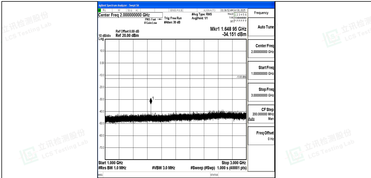
Band5_10MHz_16QAM_20450_1RB#0_1000~3000_1000~3000
