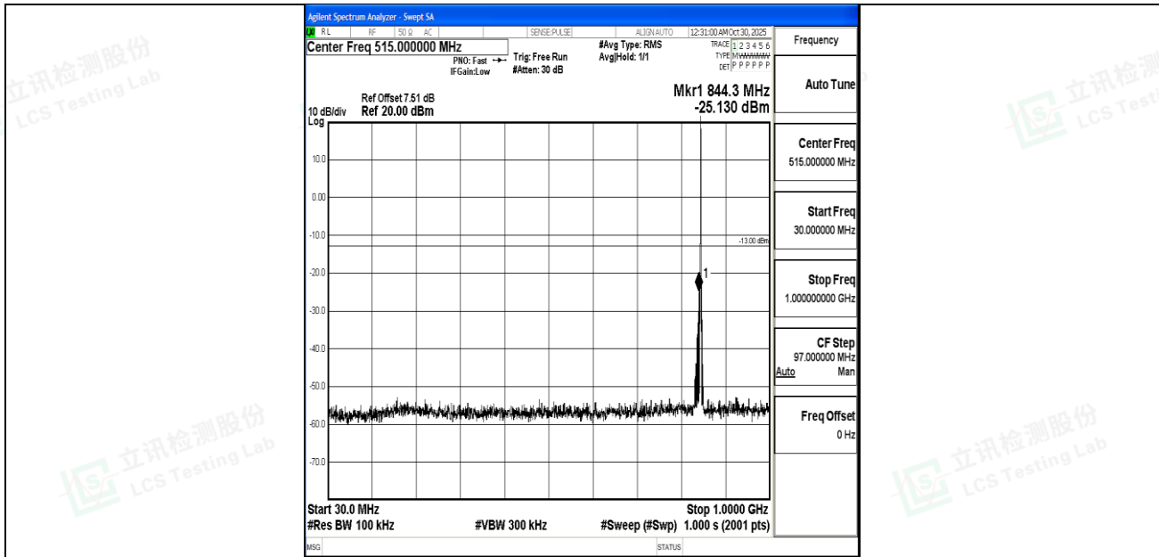
Band5_1.4MHz_QPSK_20643_1RB#0_30~1000_30~1000
