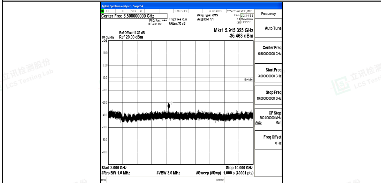
Band5_3MHz_16QAM_20415_1RB#0_3000~10000_3000~10000
