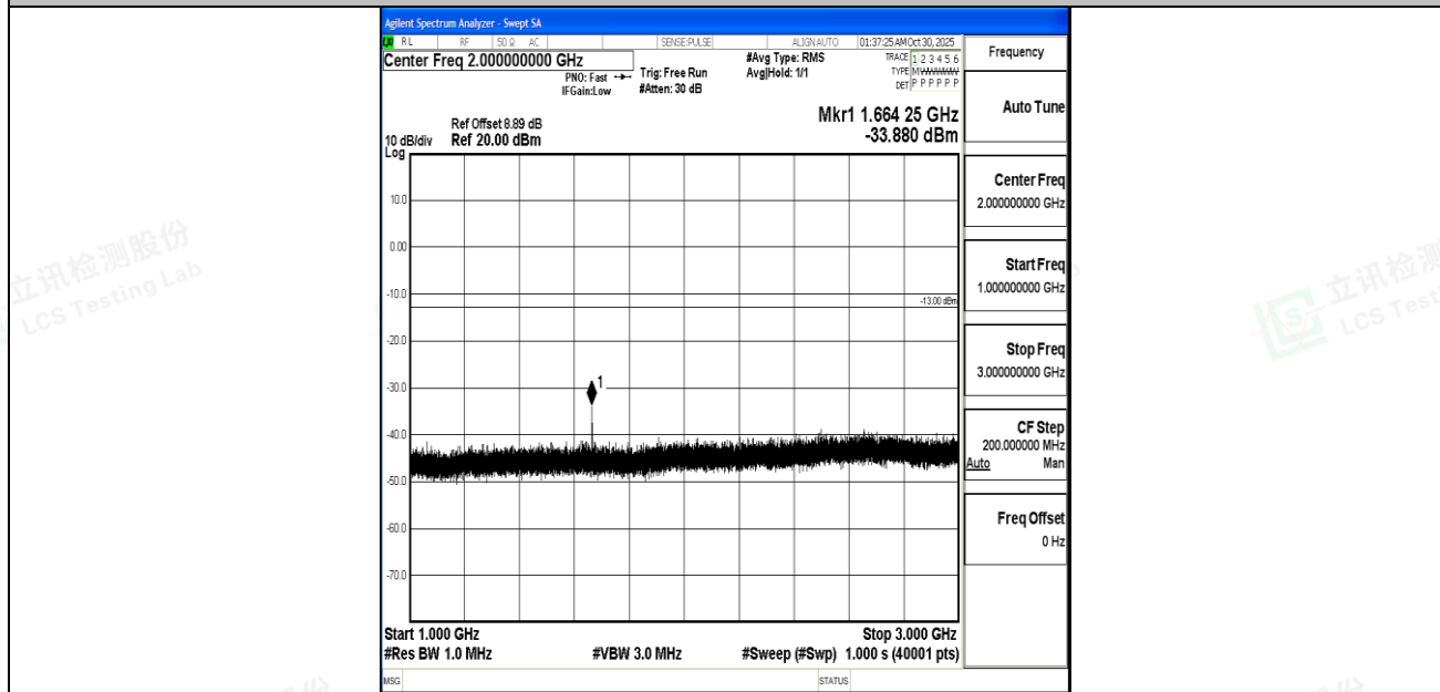
Band5_10MHz_QPSK_20525_1RB#0_1000~3000_1000~3000
