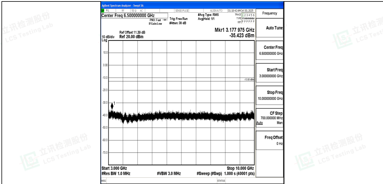
Band5_5MHz_QPSK_20625_1RB#0_3000~10000_3000~10000
