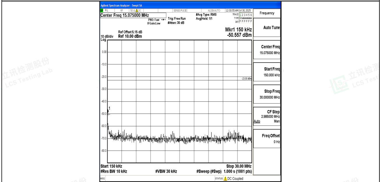
Band5_1.4MHz_QPSK_20643_1RB#0_0.15~30_0.15~30
