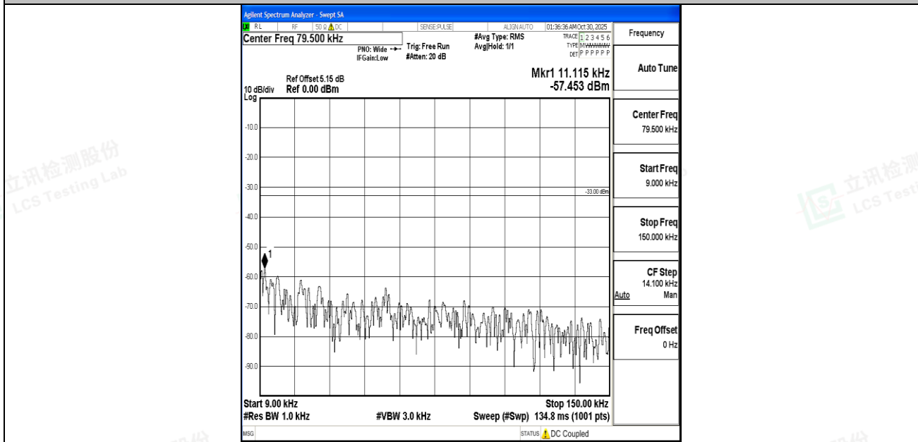
Band5_10MHz_16QAM_20450_1RB#0_0.009~0.15_0.009~0.15
