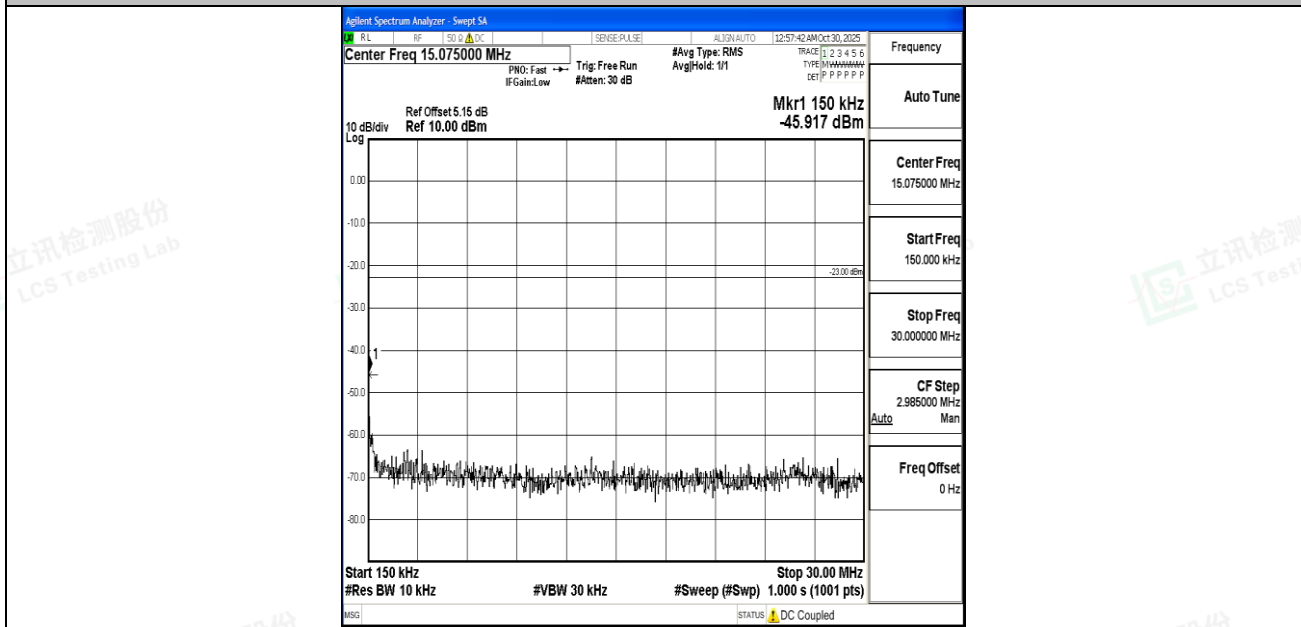
Band5_3MHz_QPSK_20635_1RB#0_0.15~30_0.15~30
