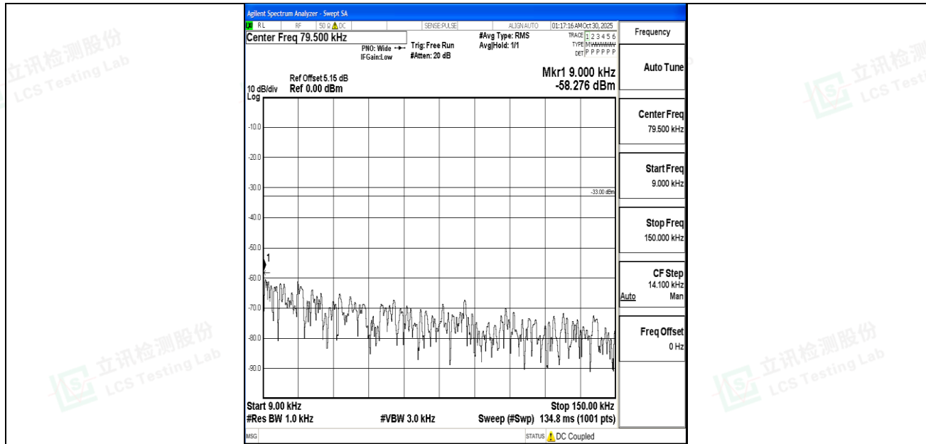
Band5_5MHz_QPSK_20525_1RB#0_0.009~0.15_0.009~0.15
