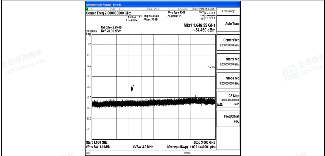
Band5_3MHz_QPSK_20415_1RB#0_1000~3000_1000~3000
