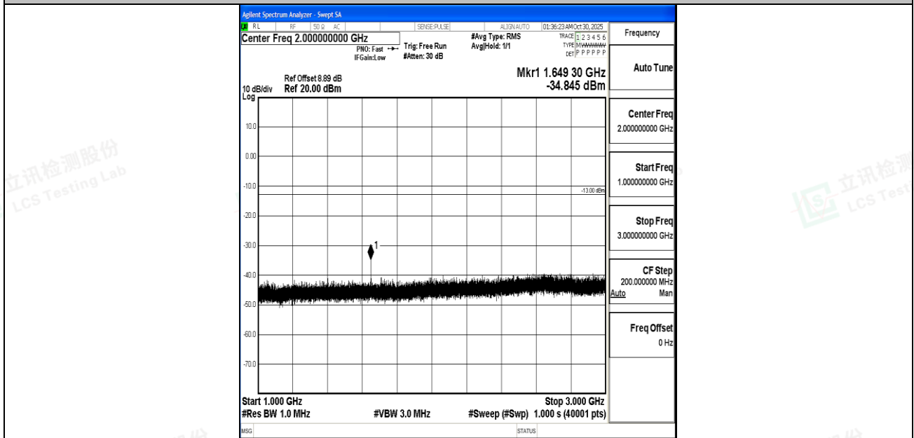
Band5_10MHz_QPSK_20450_1RB#0_1000~3000_1000~3000
