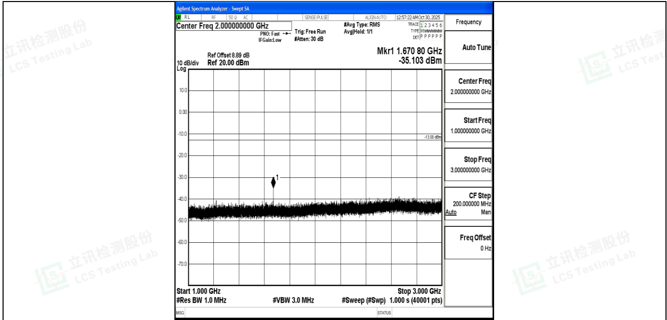
Band5_3MHz_16QAM_20525_1RB#0_1000~3000_1000~3000
