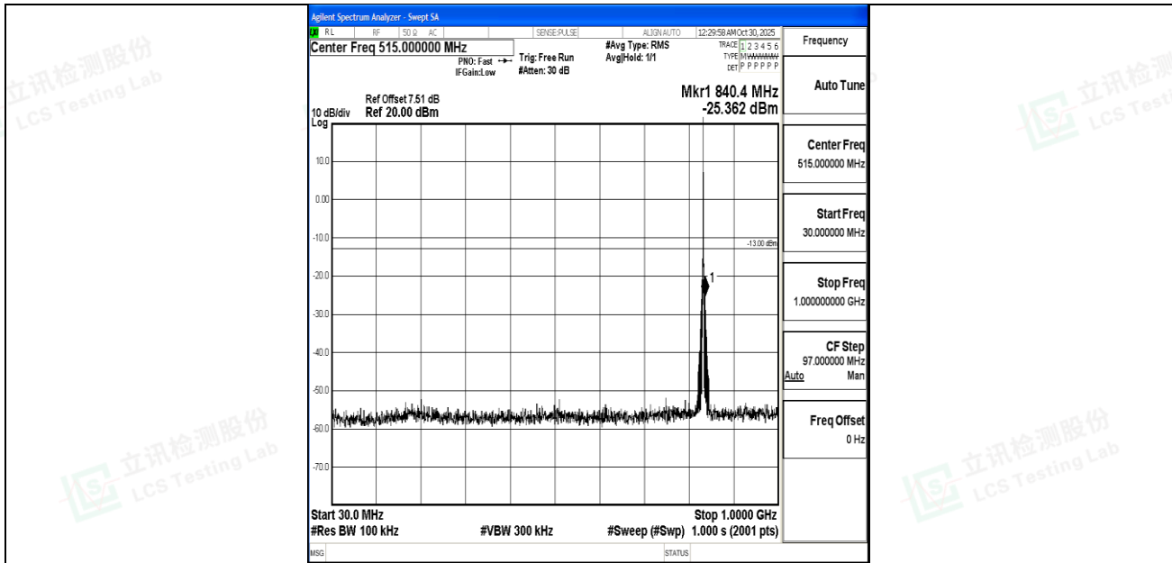
Band5_1.4MHz_QPSK_20525_1RB#0_30~1000_30~1000
