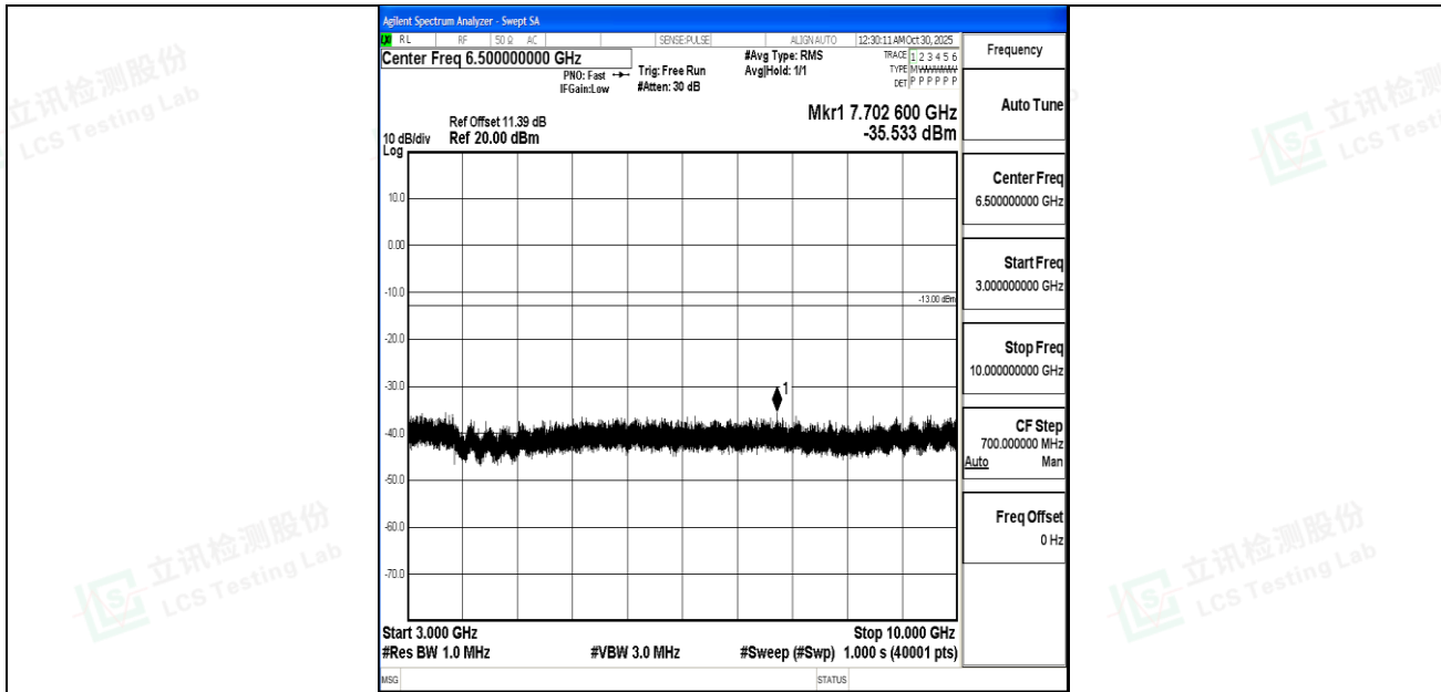
Band5_1.4MHz_QPSK_20525_1RB#0_3000~10000_3000~10000
