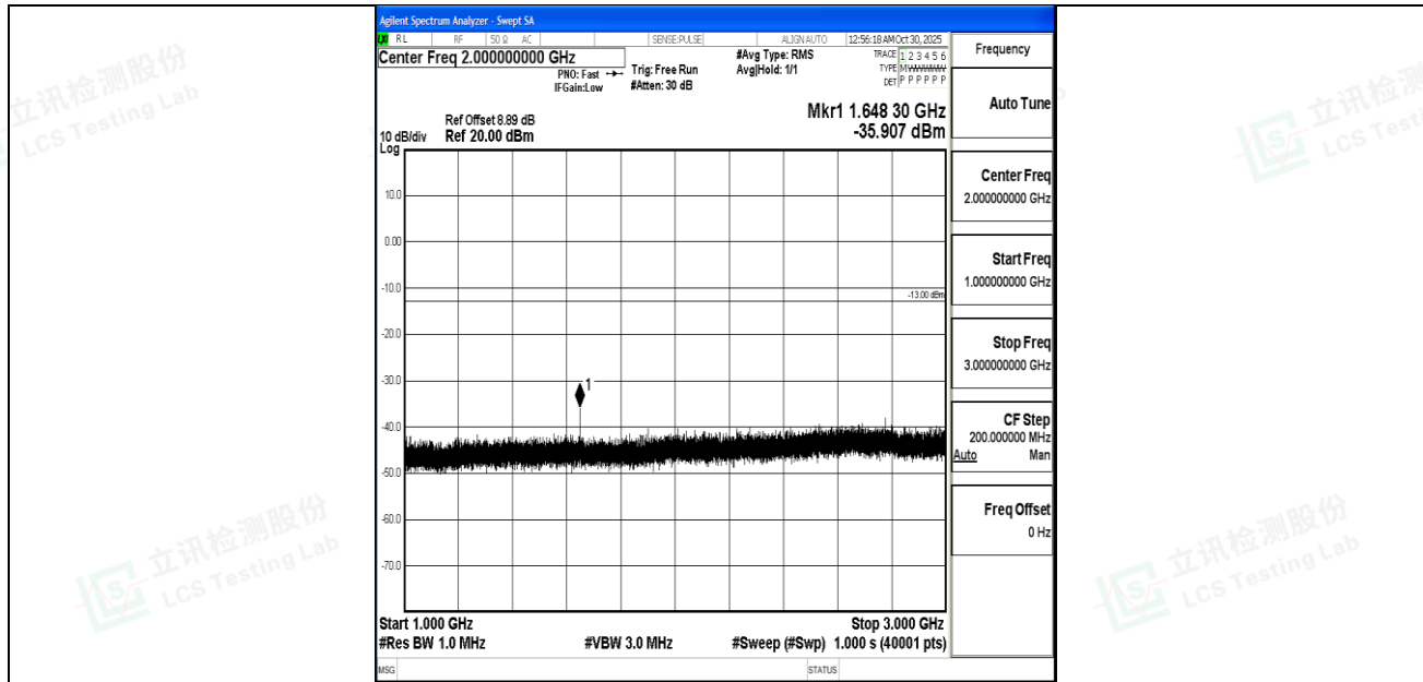
Band5_3MHz_16QAM_20415_1RB#0_1000~3000_1000~3000
