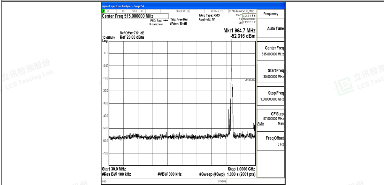
Band5_10MHz_16QAM_20600_1RB#0_30~1000_30~1000
