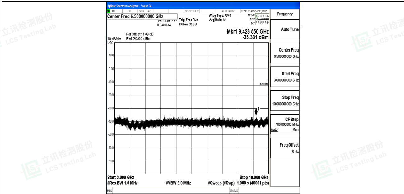
Band5_10MHz_QPSK_20600_1RB#0_3000~10000_3000~10000
