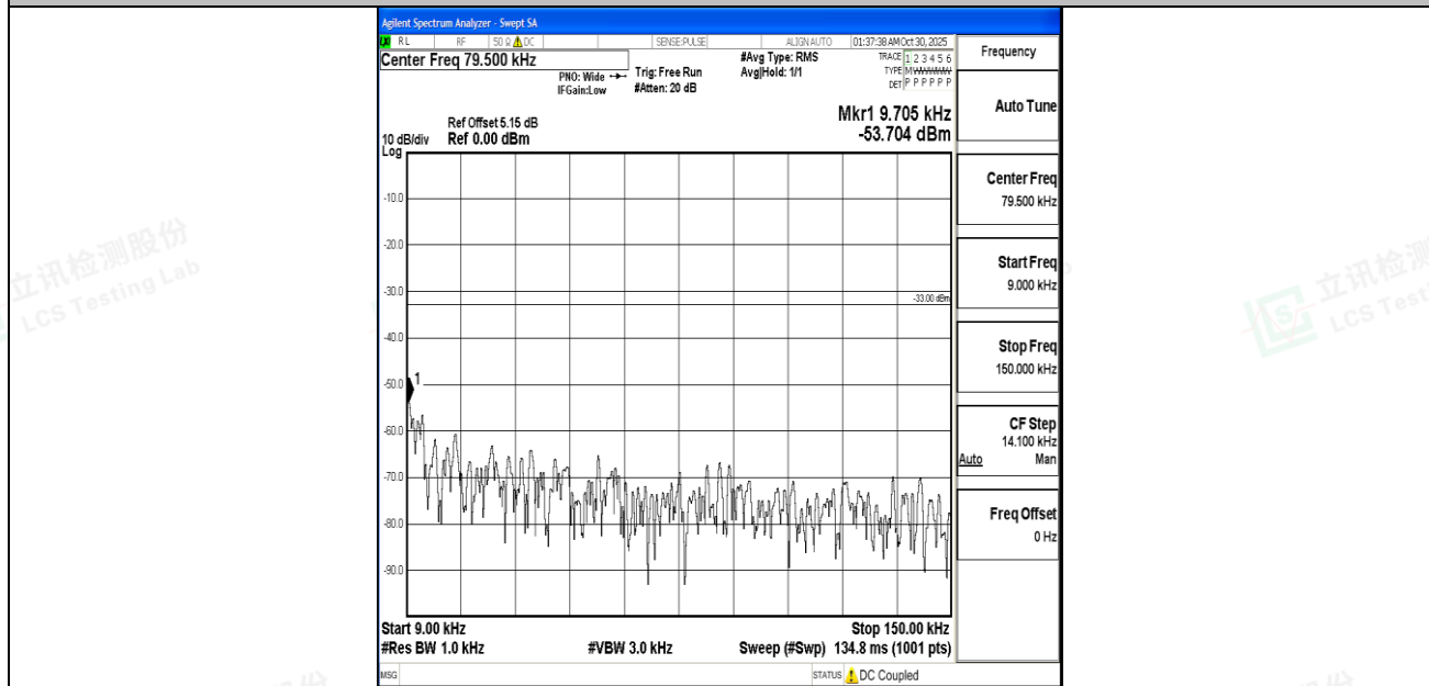
Band5_10MHz_16QAM_20525_1RB#0_0.009~0.15_0.009~0.15
