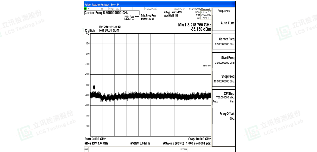
Band5_10MHz_QPSK_20525_1RB#0_3000~10000_3000~10000
