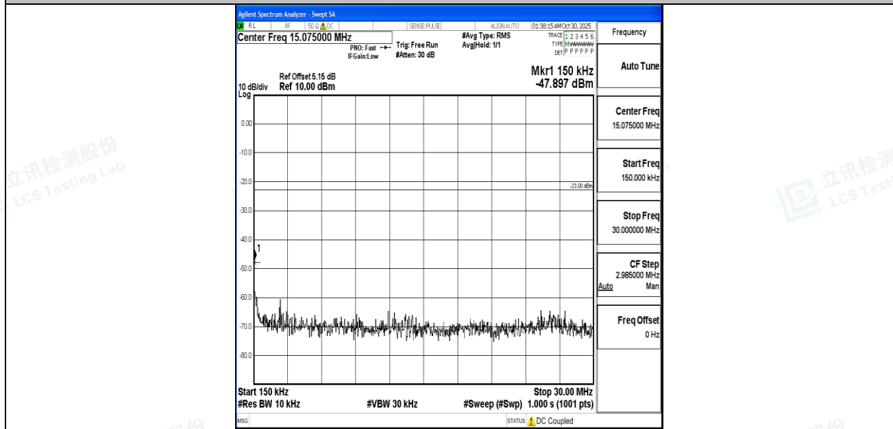
Band5_10MHz_QPSK_20600_1RB#0_0.15~30_0.15~30
