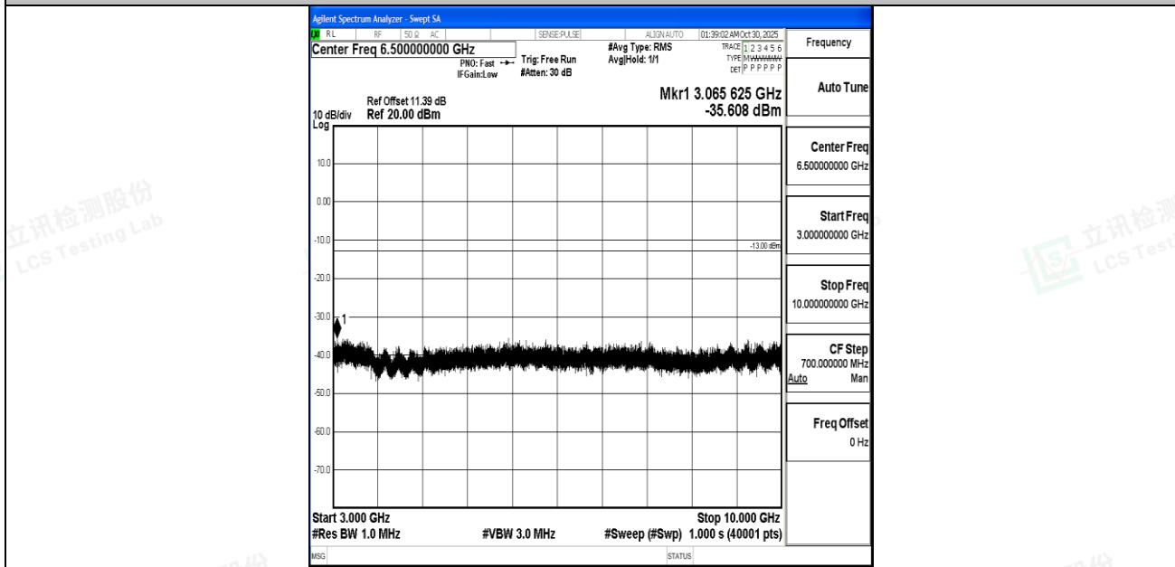
Band5_10MHz_16QAM_20600_1RB#0_3000~10000_3000~10000
