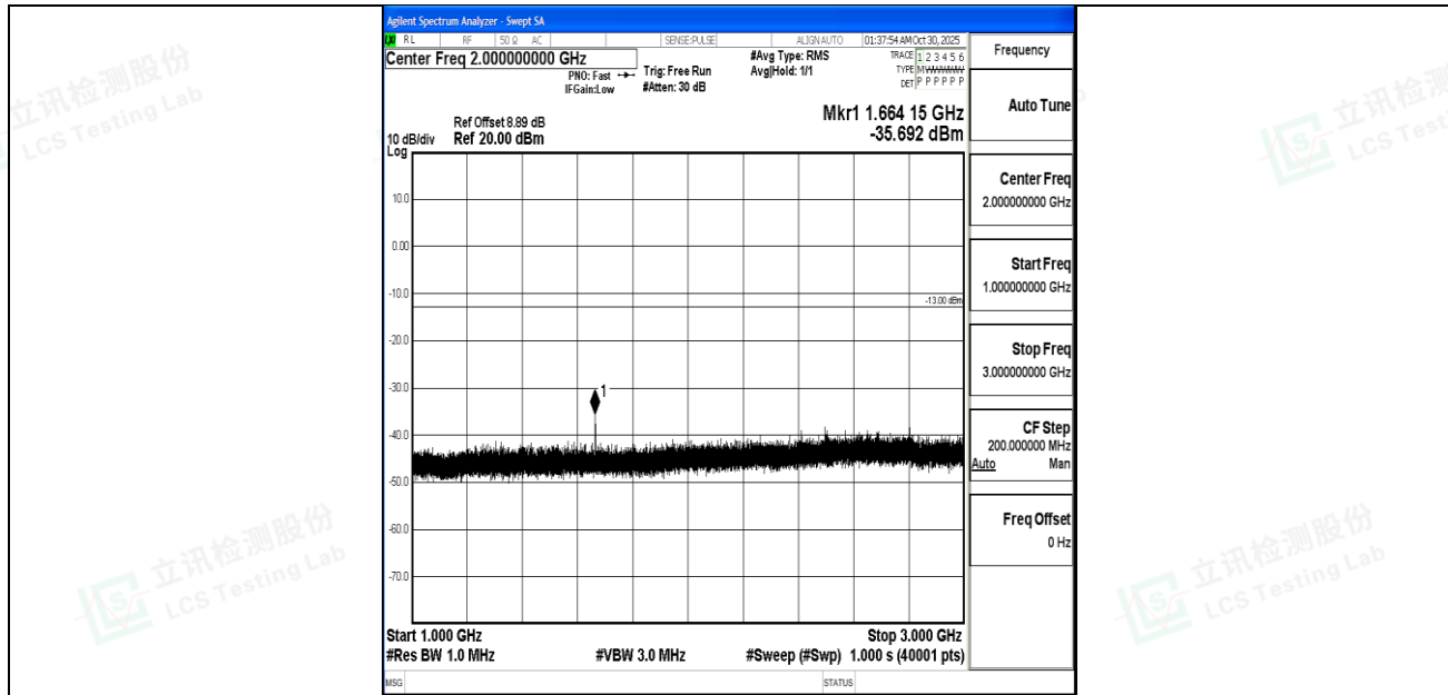
Band5_10MHz_16QAM_20525_1RB#0_1000~3000_1000~3000
