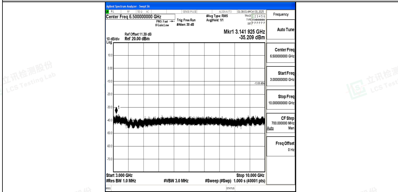
Band5_10MHz_16QAM_20525_1RB#0_3000~10000_3000~10000
