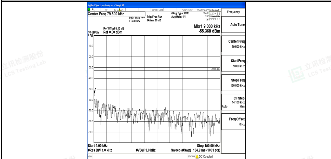
Band5_10MHz_16QAM_20600_1RB#0_0.009~0.15_0.009~0.15
