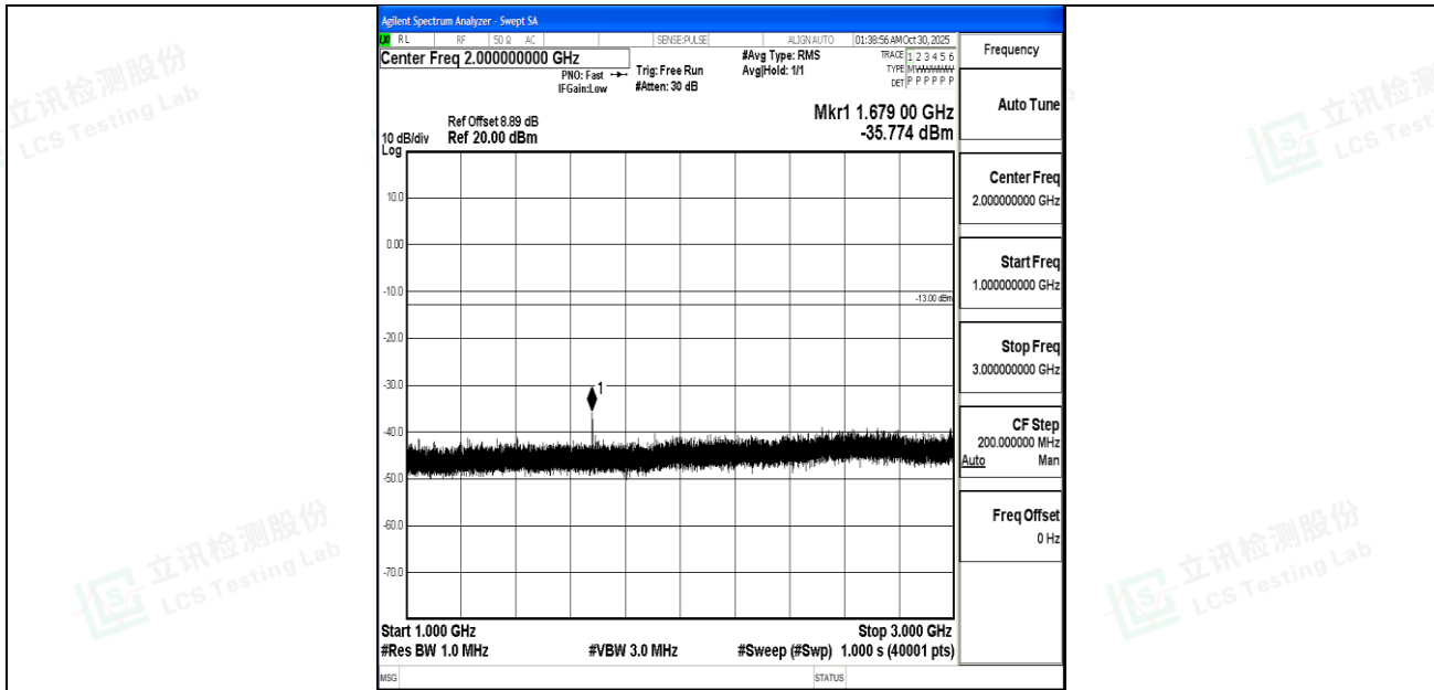
Band5_10MHz_16QAM_20600_1RB#0_1000~3000_1000~3000
