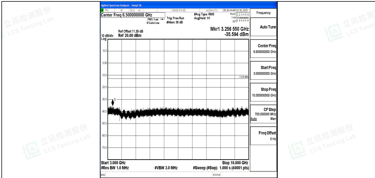
Band17_10MHz_QPSK_23800_1RB#0_3000~10000_3000~10000
