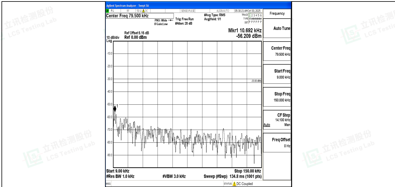
Band17_10MHz_QPSK_23800_1RB#0_0.009~0.15_0.009~0.15
