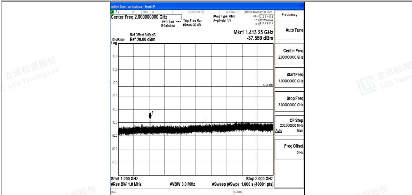
Band17_10MHz_QPSK_23800_1RB#0_1000~3000_1000~3000
