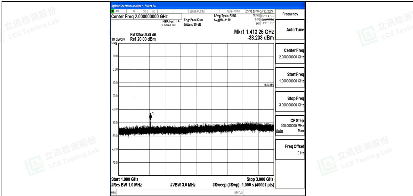
Band17_10MHz_16QAM_23800_1RB#0_1000~3000_1000~3000
