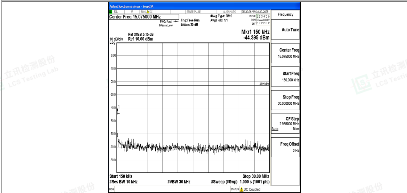
Band17_10MHz_QPSK_23800_1RB#0_0.15~30_0.15~30
