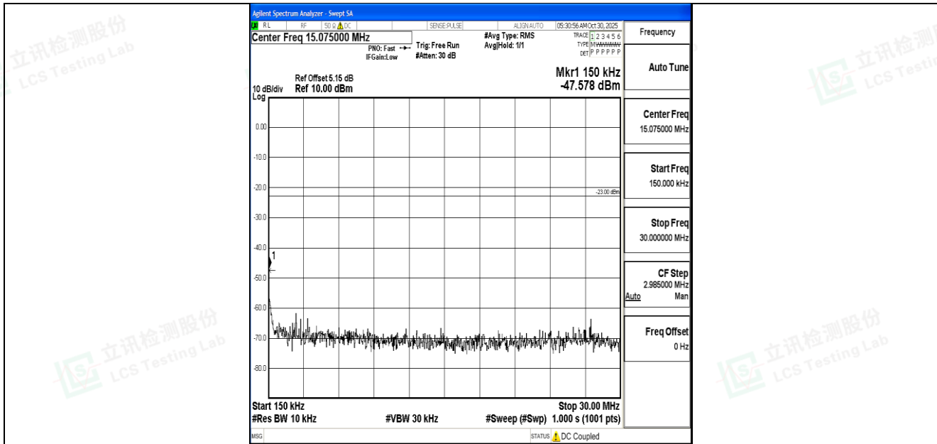
Band17_10MHz_16QAM_23800_1RB#0_0.15~30_0.15~30
