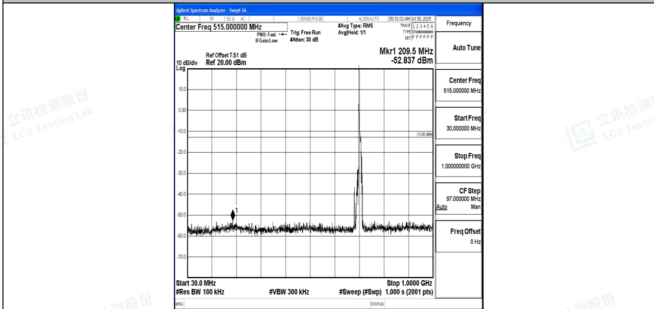
Band17_10MHz_16QAM_23800_1RB#0_30~1000_30~1000
