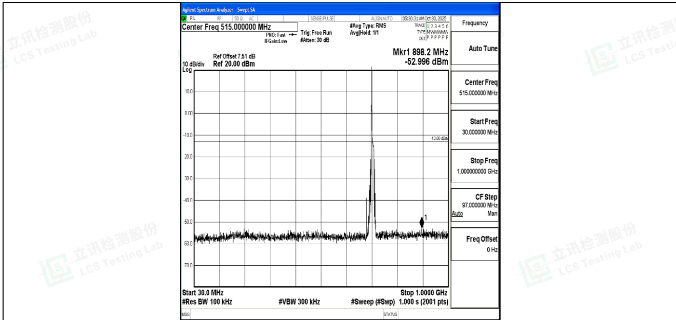
Band17_10MHz_QPSK_23800_1RB#0_30~1000_30~1000
