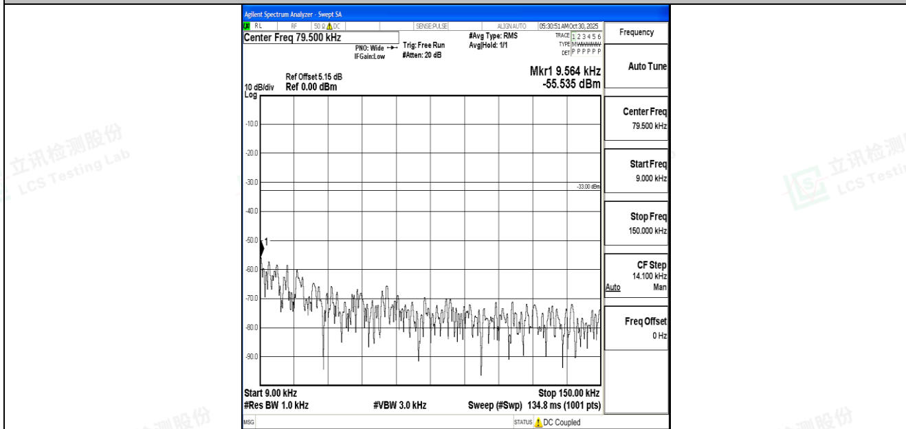
Band17_10MHz_16QAM_23800_1RB#0_0.009~0.15_0.009~0.15
