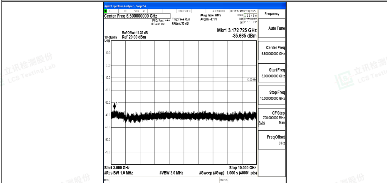
Band17_10MHz_16QAM_23800_1RB#0_3000~10000_3000~10000
