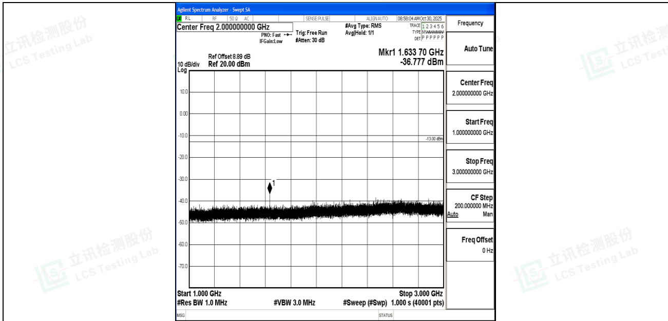
Band26_5MHz_QPSK_26740_1RB#0_1000~3000_1000~3000
