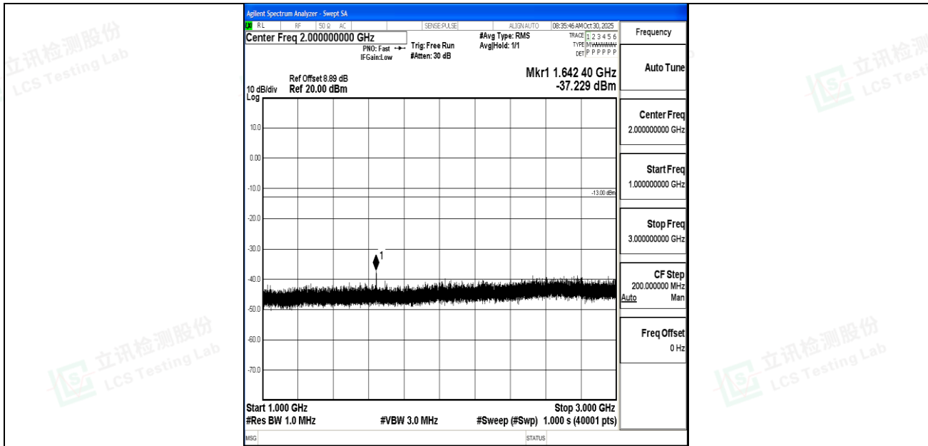
Band26_3MHz_QPSK_26775_1RB#0_1000~3000_1000~3000
