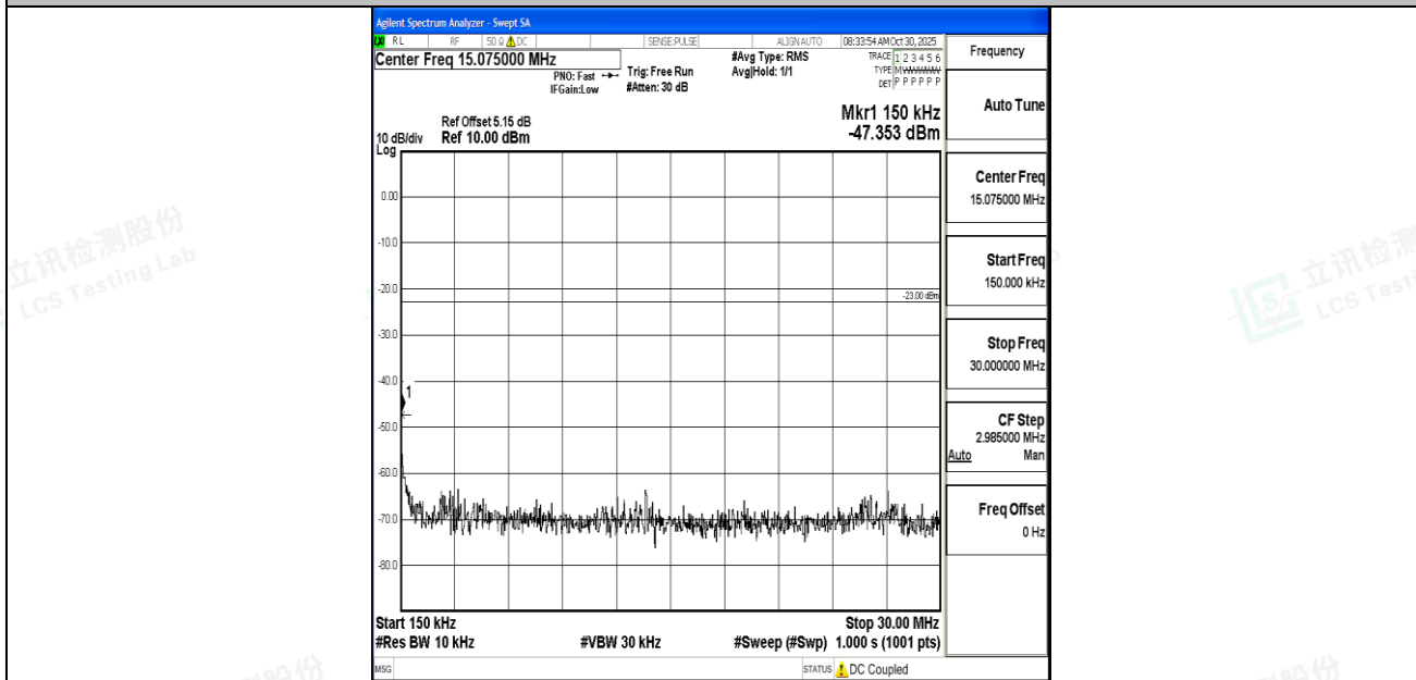
Band26_3MHz_16QAM_26705_1RB#0_0.15~30_0.15~30
