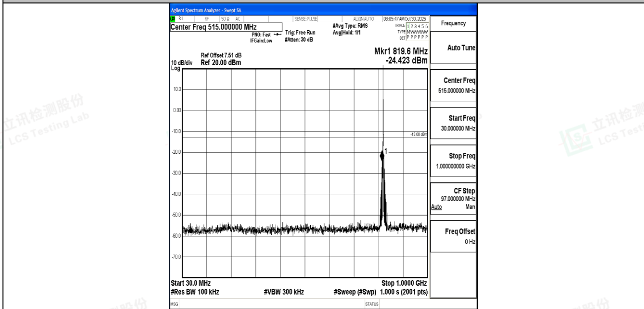
Band26_1.4MHz_QPSK_26783_1RB#0_30~1000_30~1000
