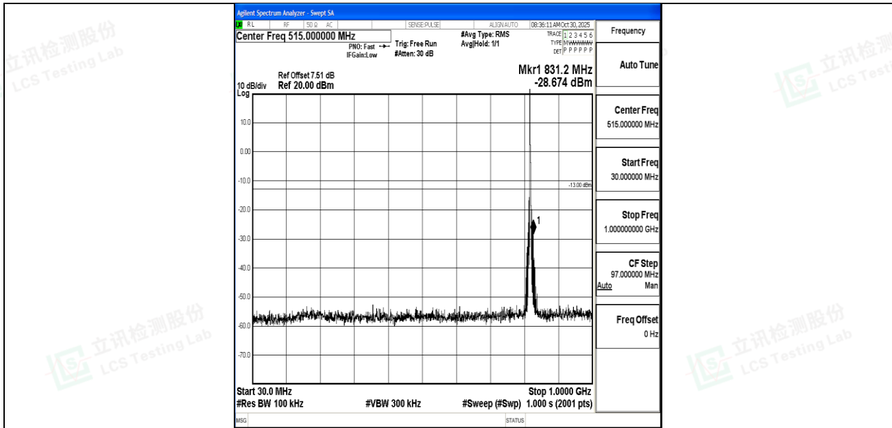
Band26_3MHz_16QAM_26775_1RB#0_30~1000_30~1000
