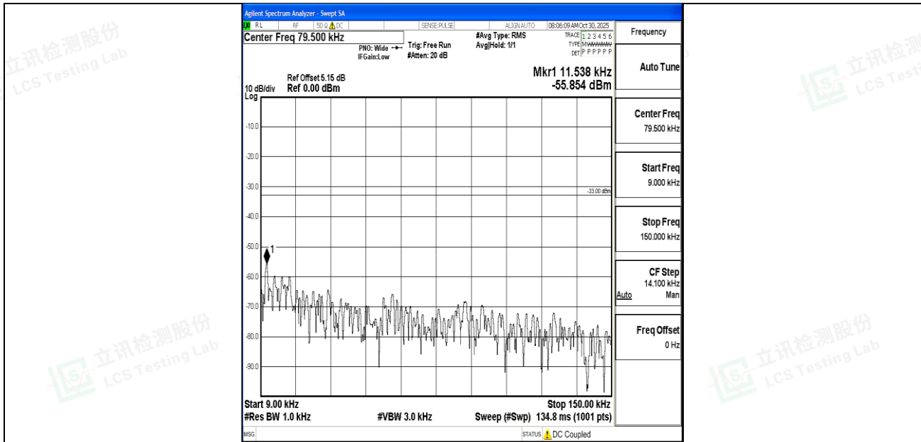
Band26_1.4MHz_16QAM_26783_1RB#0_0.009~0.15_0.009~0.15
