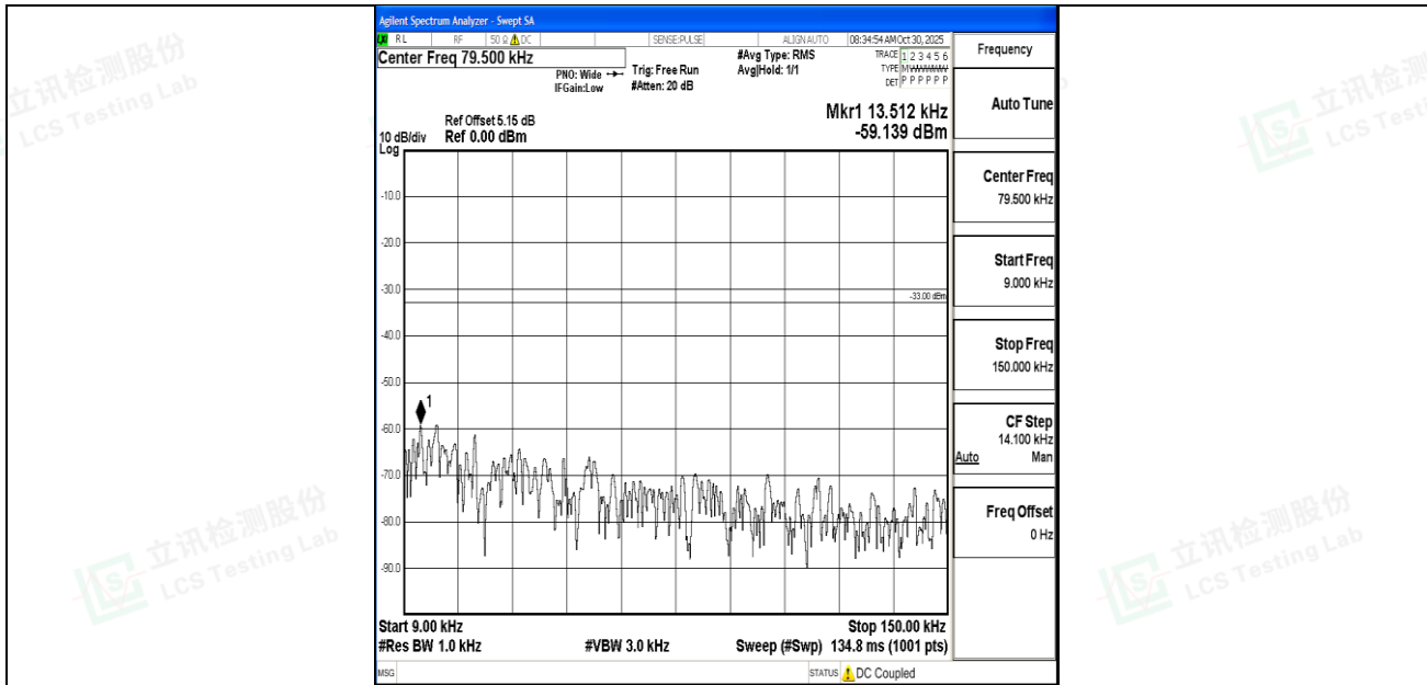
Band26_3MHz_16QAM_26740_1RB#0_0.009~0.15_0.009~0.15
