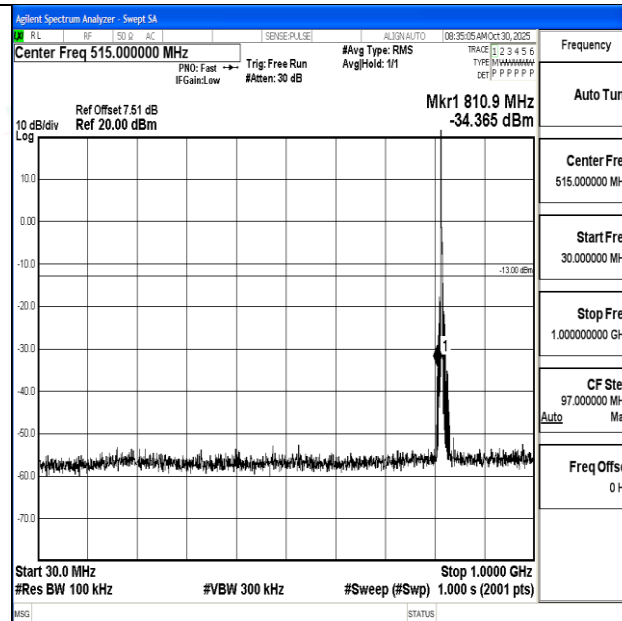
Band26_3MHz_16QAM_26740_1RB#0_30~1000_30~1000
