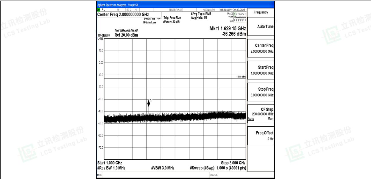
Band26_10MHz_QPSK_26740_1RB#0_1000~3000_1000~3000
