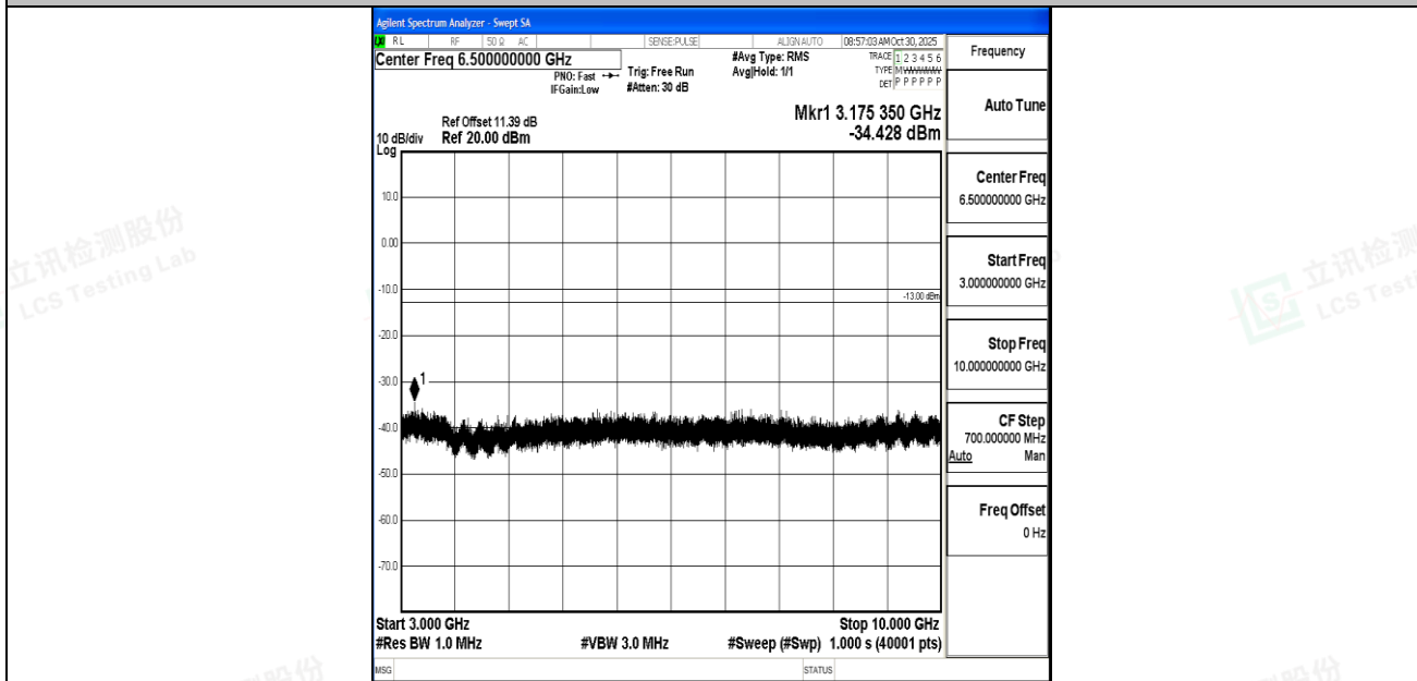
Band26_5MHz_QPSK_26715_1RB#0_3000~10000_3000~10000
