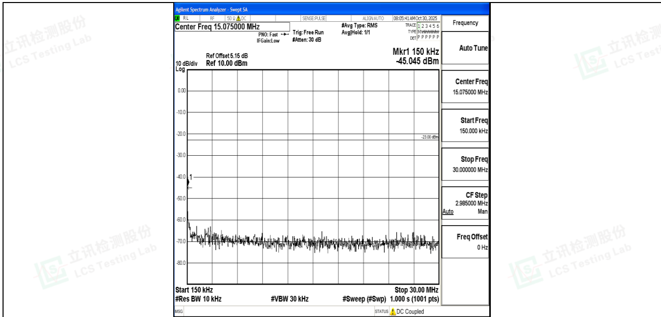
Band26_1.4MHz_QPSK_26783_1RB#0_0.15~30_0.15~30
