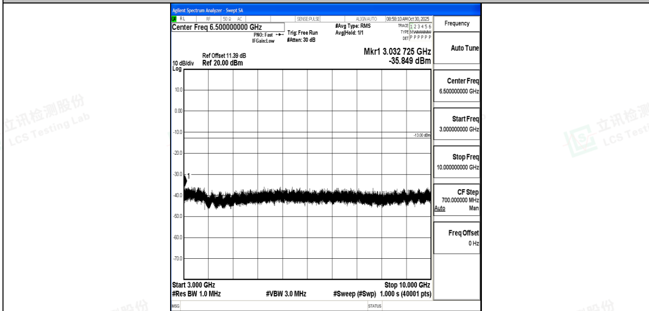
Band26_5MHz_QPSK_26740_1RB#0_3000~10000_3000~10000
