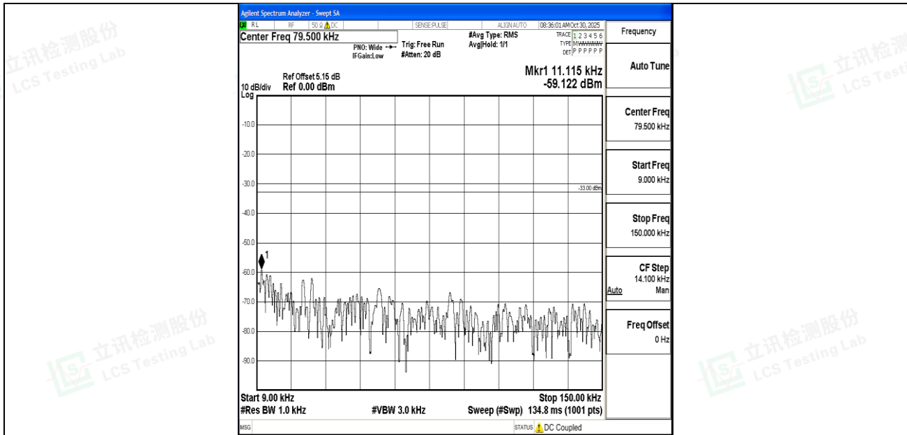
Band26_3MHz_16QAM_26775_1RB#0_0.009~0.15_0.009~0.15
