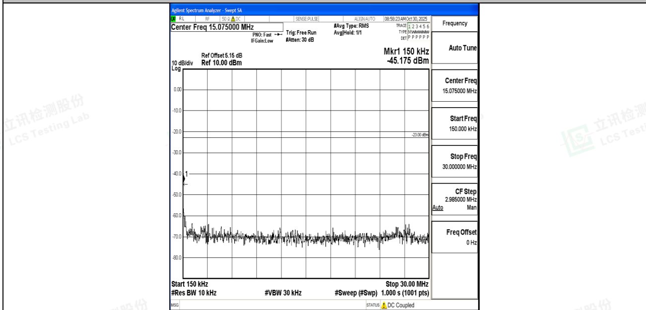
Band26_5MHz_16QAM_26740_1RB#0_0.15~30_0.15~30
