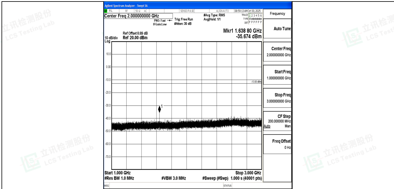
Band26_5MHz_QPSK_26765_1RB#0_1000~3000_1000~3000
