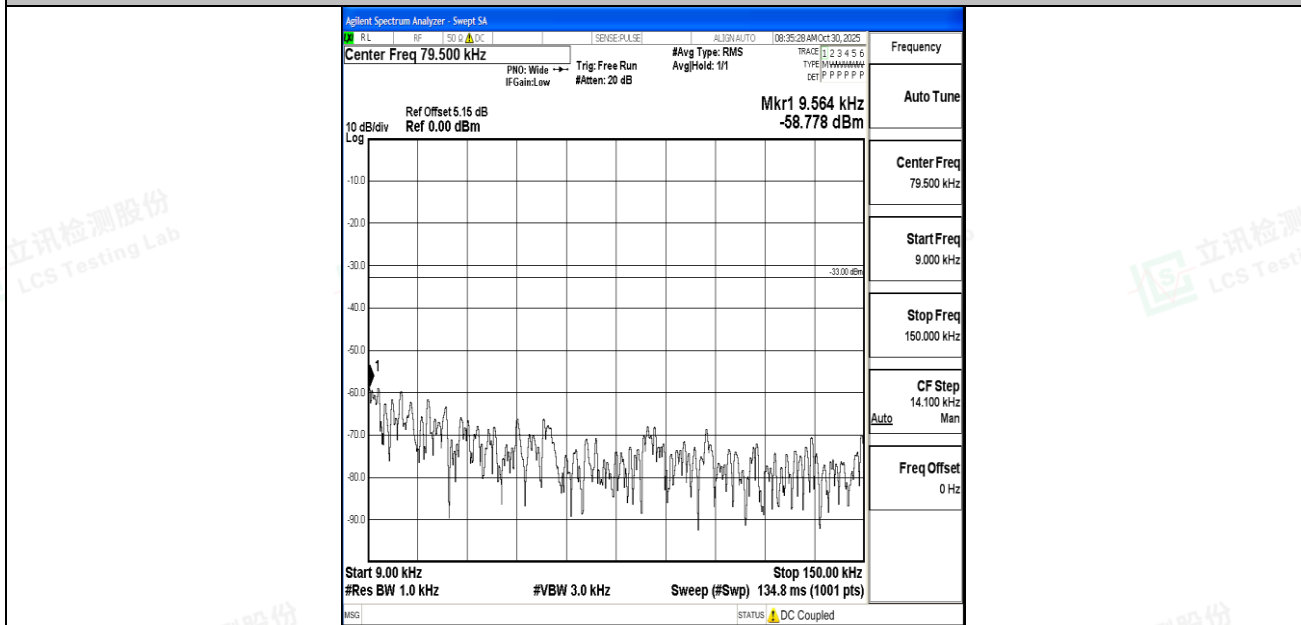
Band26_3MHz_QPSK_26775_1RB#0_0.009~0.15_0.009~0.15
