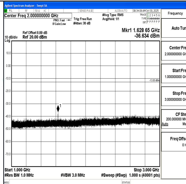
Band26_3MHz_16QAM_26705_1RB#0_1000~3000_1000~3000
