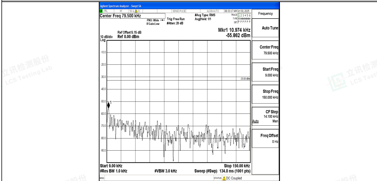
Band26_3MHz_QPSK_26705_1RB#0_0.009~0.15_0.009~0.15
