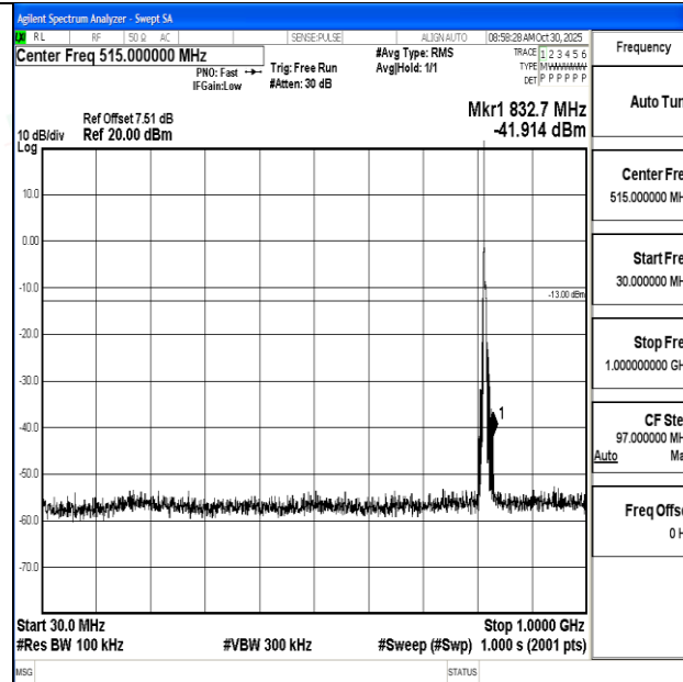
Band26_5MHz_16QAM_26740_1RB#0_30~1000_30~1000
