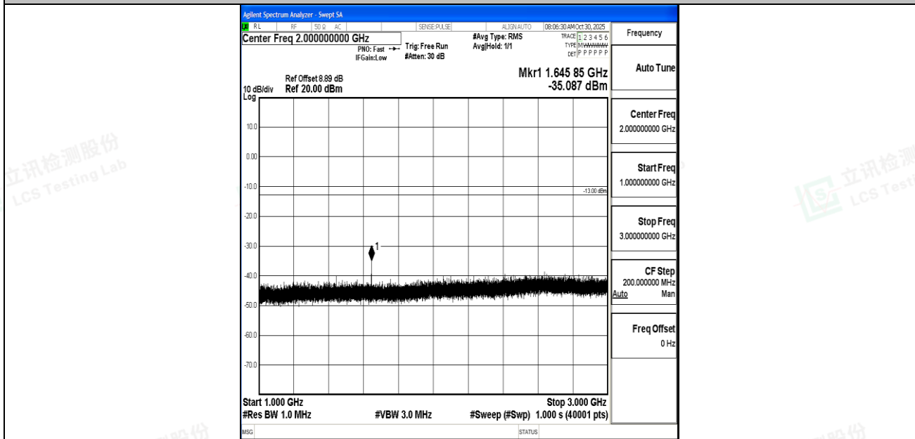
Band26_1.4MHz_16QAM_26783_1RB#0_1000~3000_1000~3000
