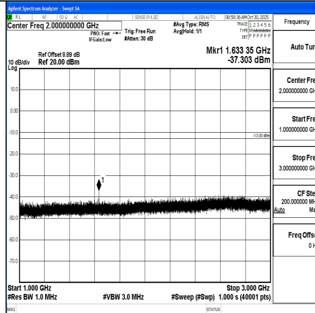
Band26_5MHz_16QAM_26740_1RB#0_1000~3000_1000~3000
