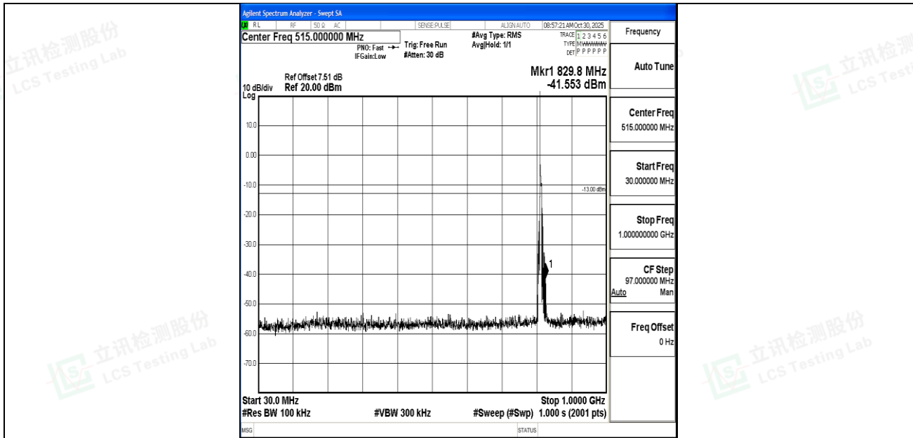
Band26_5MHz_16QAM_26715_1RB#0_30~1000_30~1000
