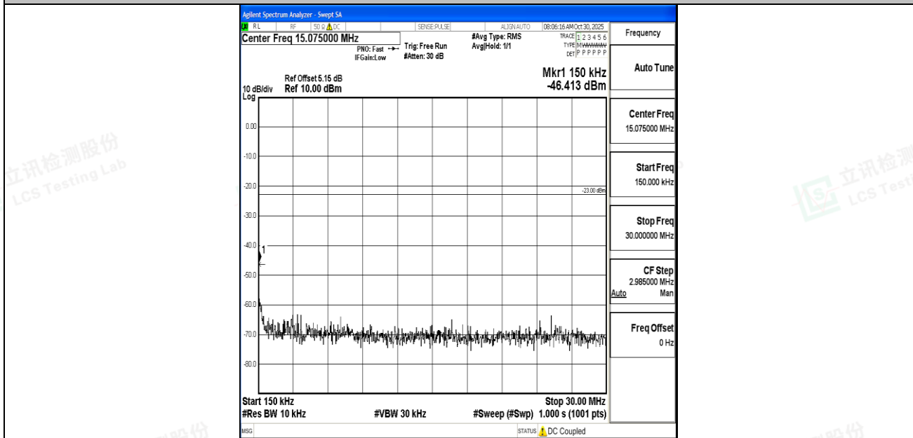
Band26_1.4MHz_16QAM_26783_1RB#0_0.15~30_0.15~30
