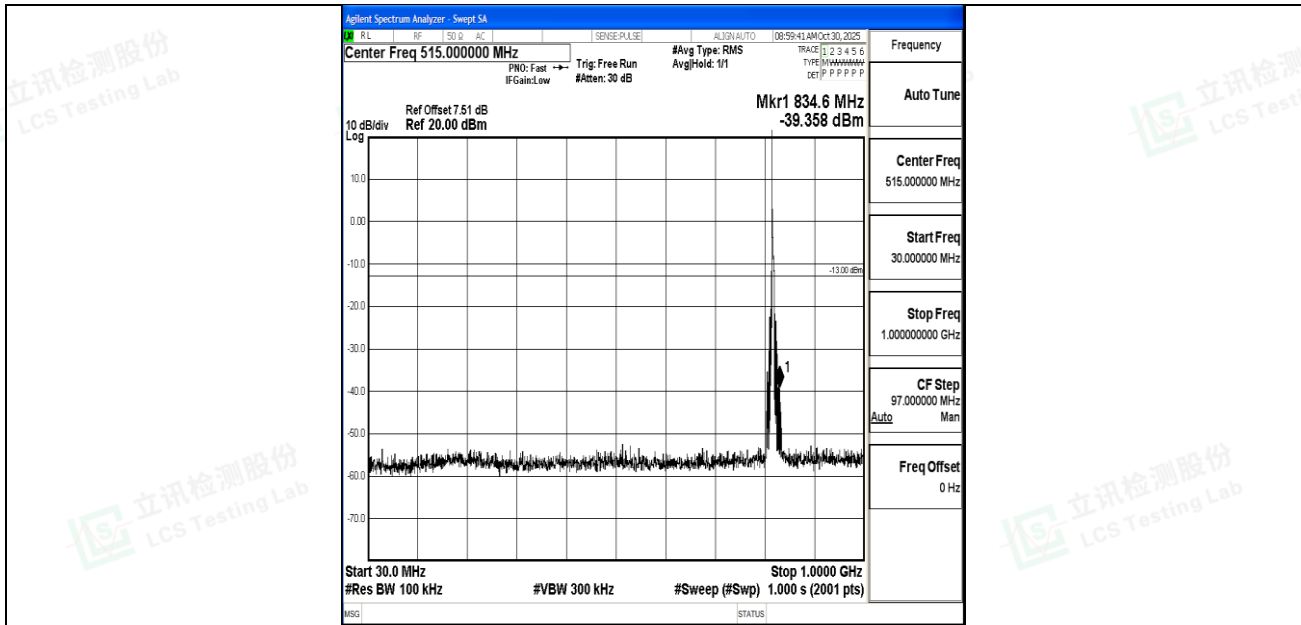
Band26_5MHz_16QAM_26765_1RB#0_30~1000_30~1000
