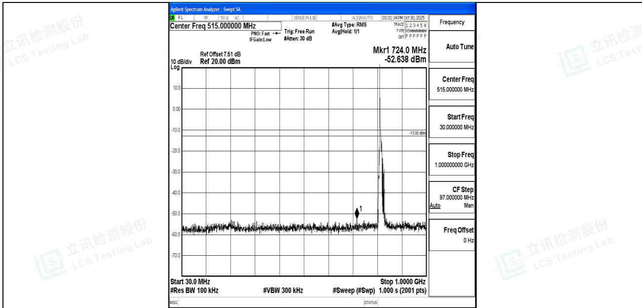
Band26_10MHz_16QAM_26740_1RB#0_30~1000_30~1000
