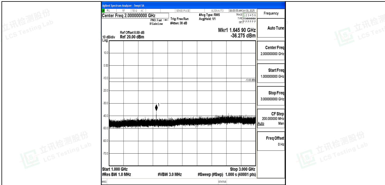
Band26_1.4MHz_QPSK_26783_1RB#0_1000~3000_1000~3000
