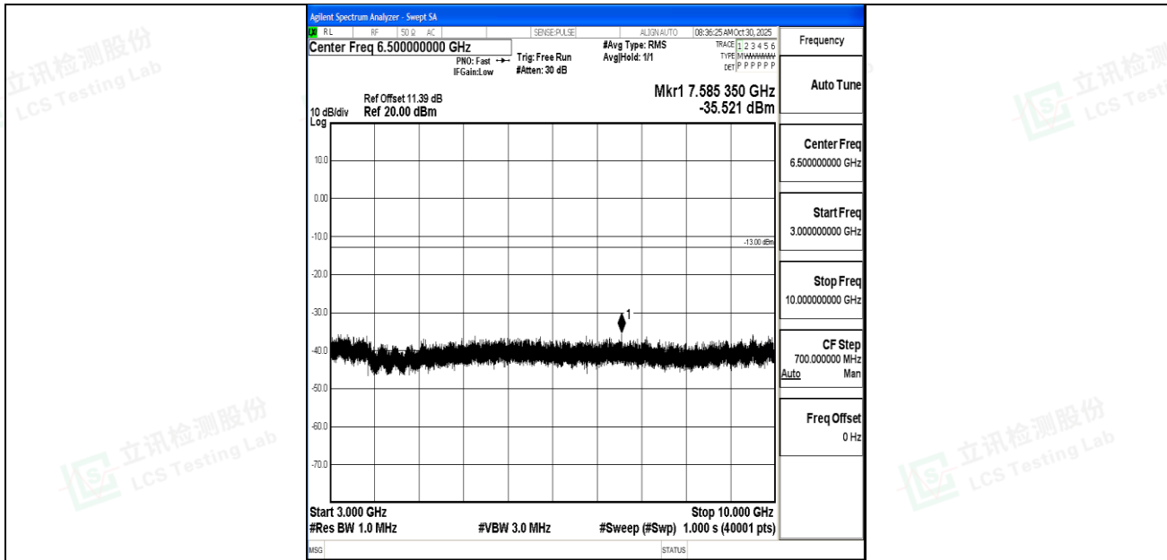
Band26_3MHz_16QAM_26775_1RB#0_3000~10000_3000~10000
