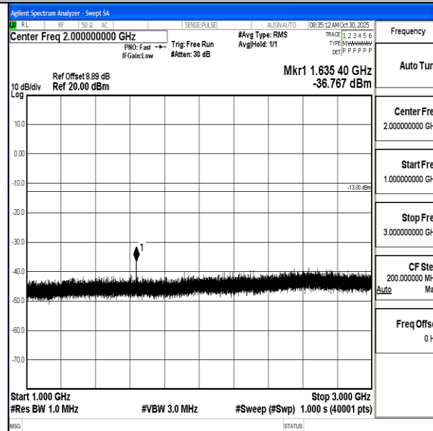
Band26_3MHz_16QAM_26740_1RB#0_1000~3000_1000~3000
