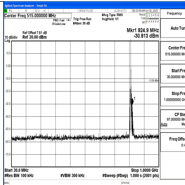
Band26_3MHz_16QAM_26705_1RB#0_30~1000_30~1000
