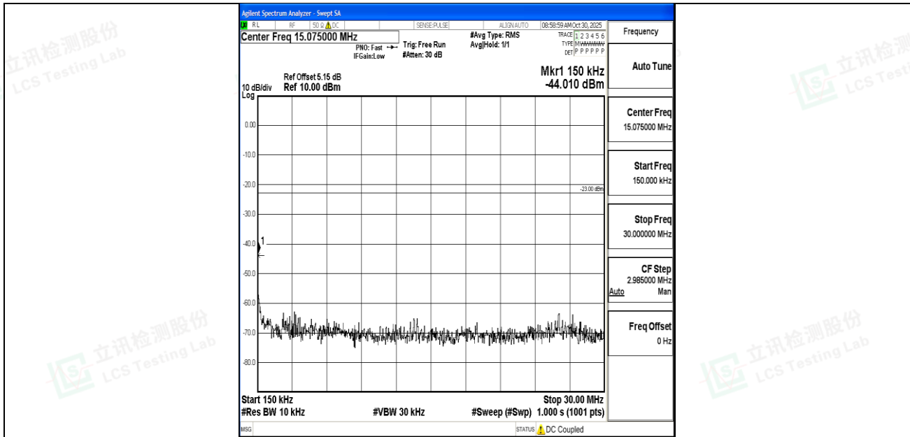
Band26_5MHz_QPSK_26765_1RB#0_0.15~30_0.15~30
