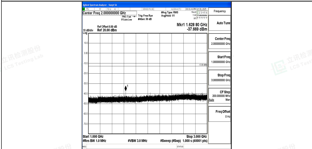
Band26_10MHz_16QAM_26740_1RB#0_1000~3000_1000~3000
