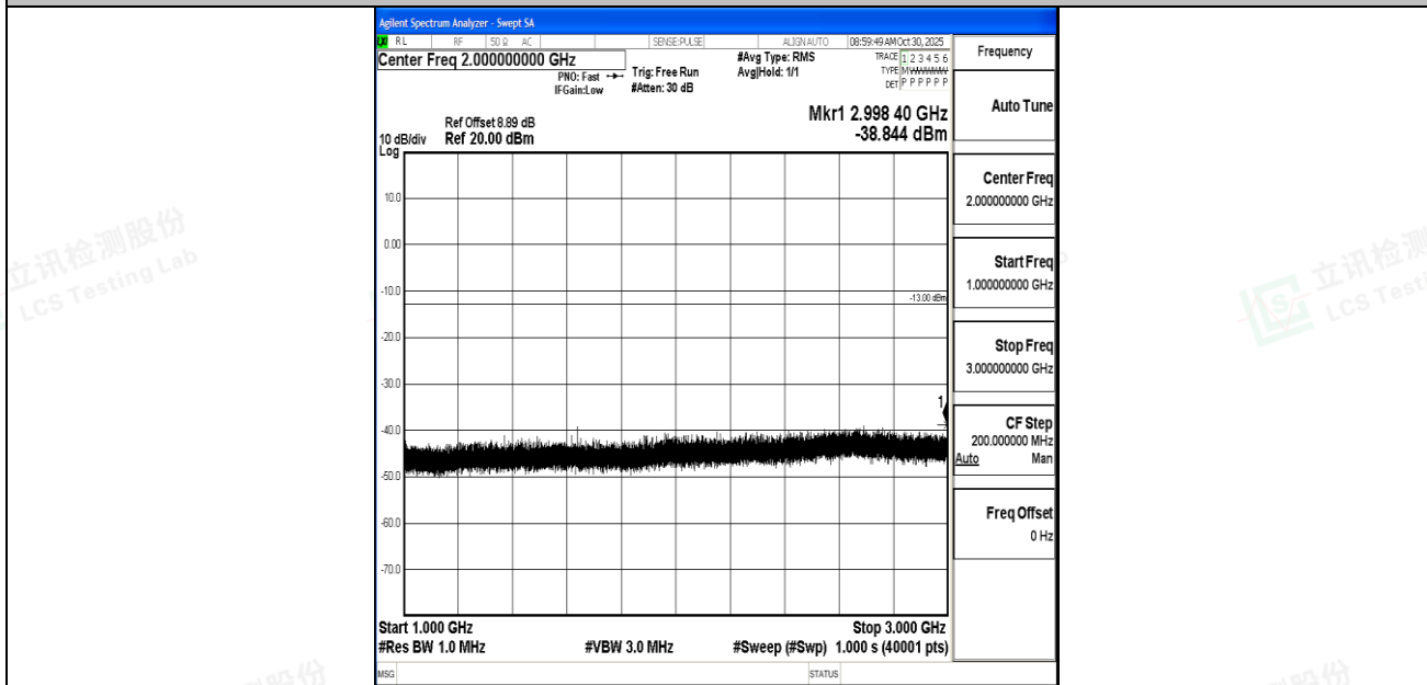
Band26_5MHz_16QAM_26765_1RB#0_1000~3000_1000~3000
