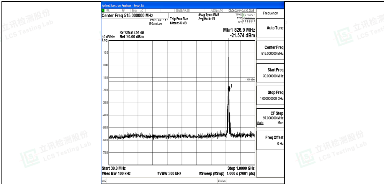
Band26_1.4MHz_16QAM_26783_1RB#0_30~1000_30~1000
