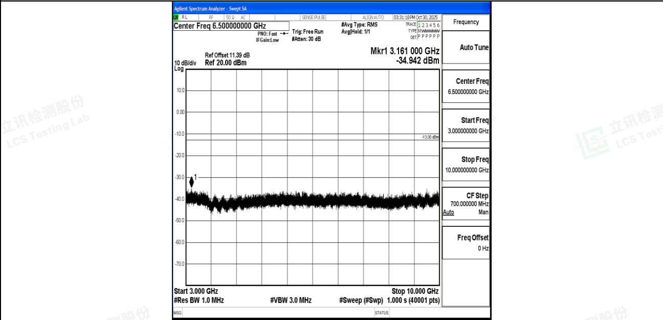
Band26_10MHz_QPSK_26740_1RB#0_3000~10000_3000~10000
