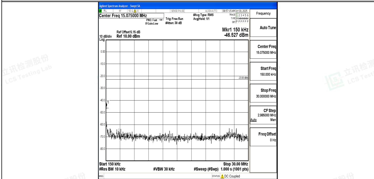
Band26_5MHz_16QAM_26715_1RB#0_0.15~30_0.15~30
