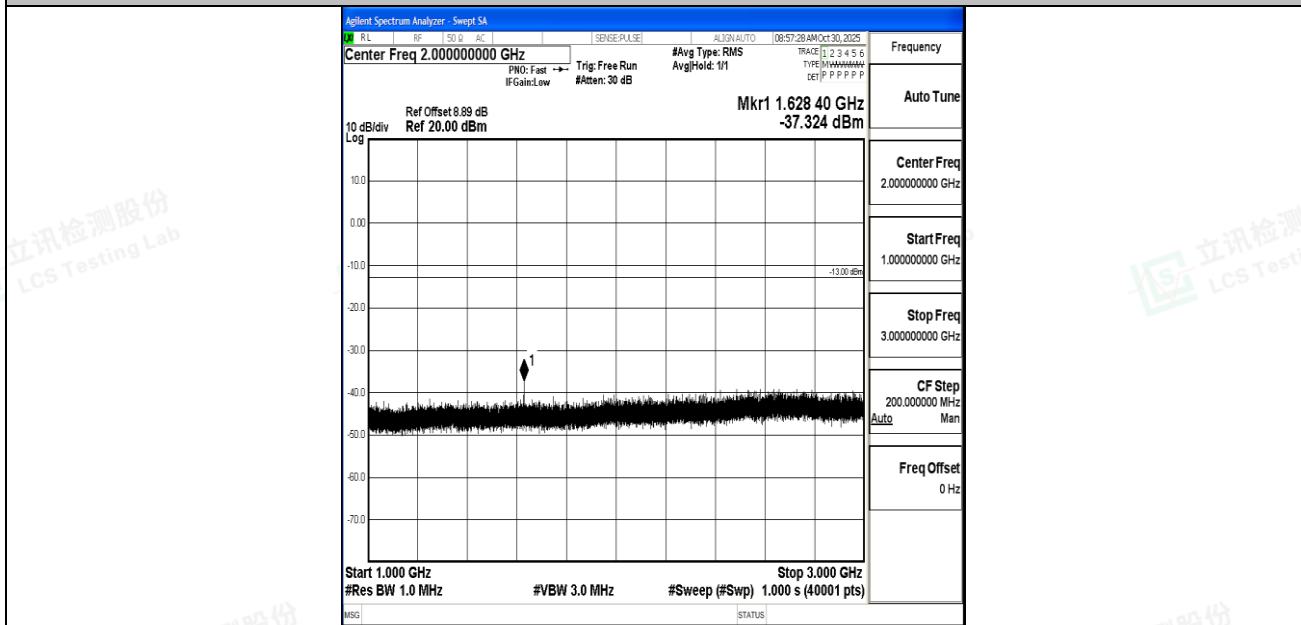
Band26_5MHz_16QAM_26715_1RB#0_1000~3000_1000~3000
