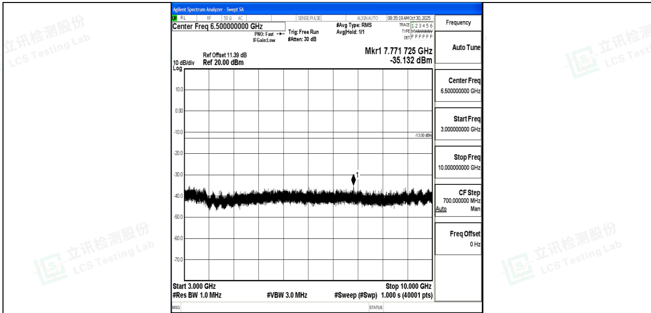
Band26_3MHz_16QAM_26740_1RB#0_3000~10000_3000~10000
