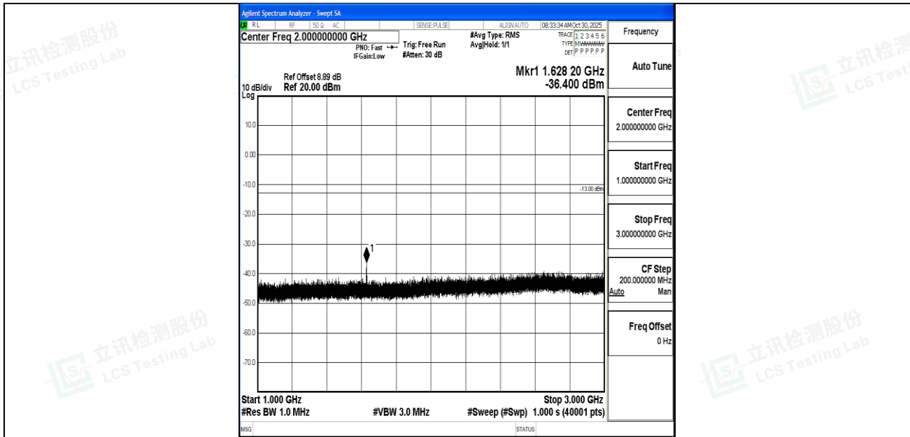
Band26_3MHz_QPSK_26705_1RB#0_1000~3000_1000~3000
