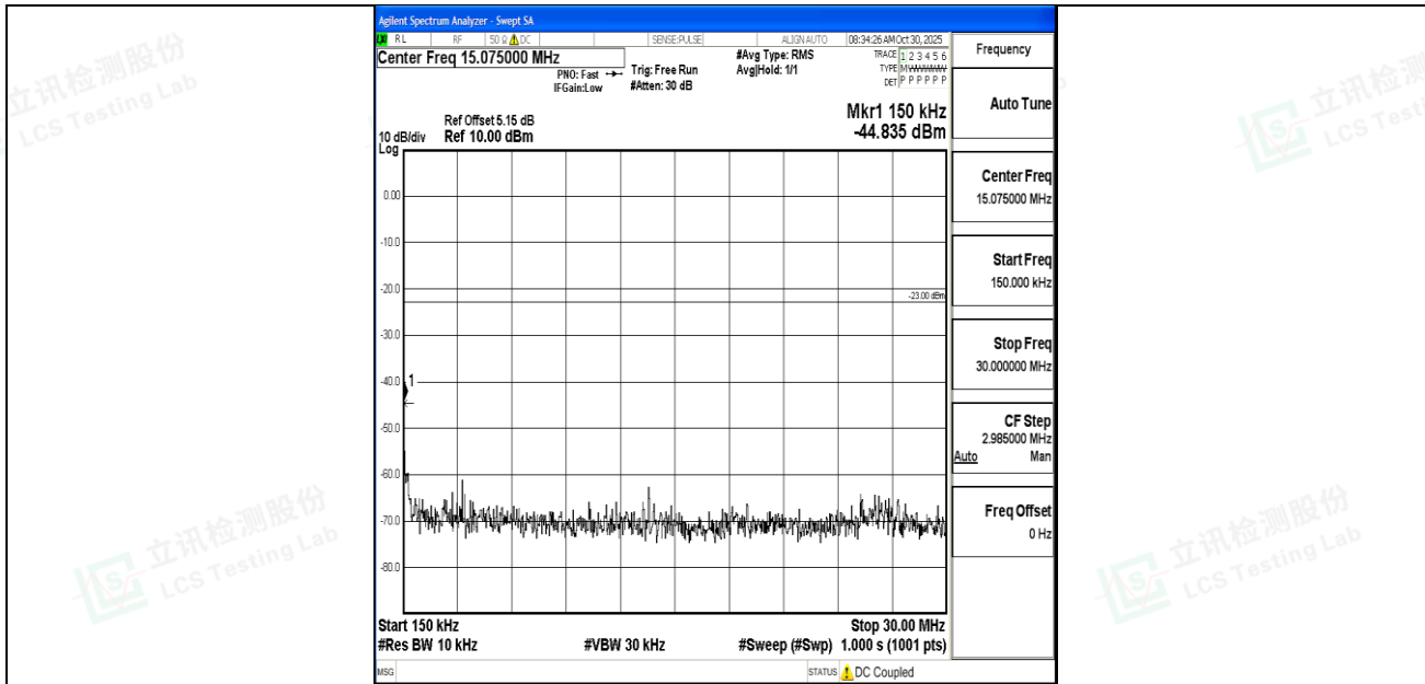
Band26_3MHz_QPSK_26740_1RB#0_0.15~30_0.15~30
