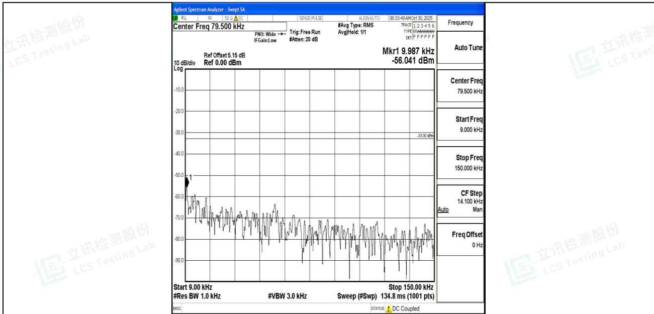
Band26_3MHz_16QAM_26705_1RB#0_0.009~0.15_0.009~0.15
