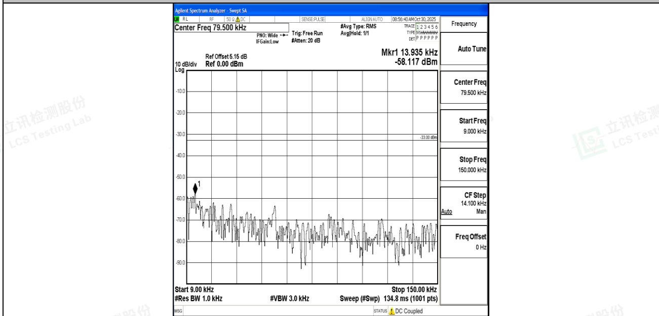
Band26_5MHz_QPSK_26715_1RB#0_0.009~0.15_0.009~0.15
