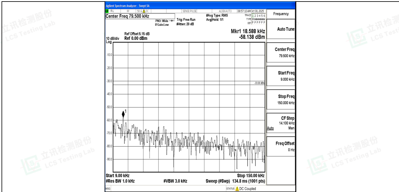
Band26_5MHz_16QAM_26715_1RB#0_0.009~0.15_0.009~0.15
