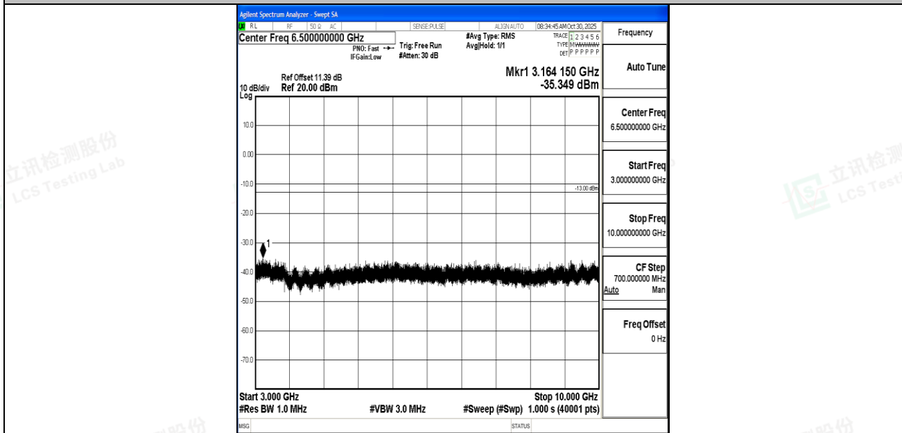
Band26_3MHz_QPSK_26740_1RB#0_3000~10000_3000~10000
