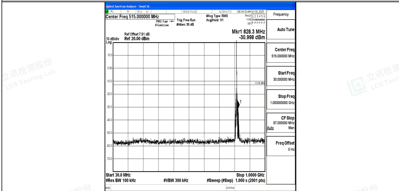
Band26_3MHz_QPSK_26740_1RB#0_30~1000_30~1000
