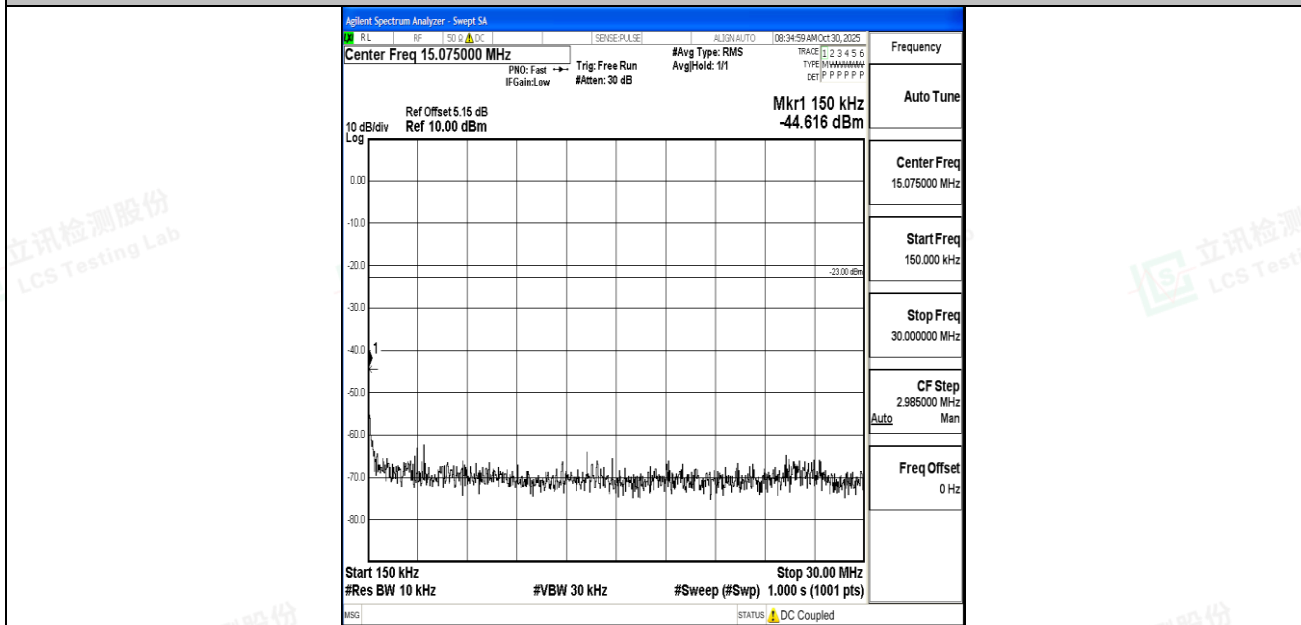
Band26_3MHz_16QAM_26740_1RB#0_0.15~30_0.15~30
