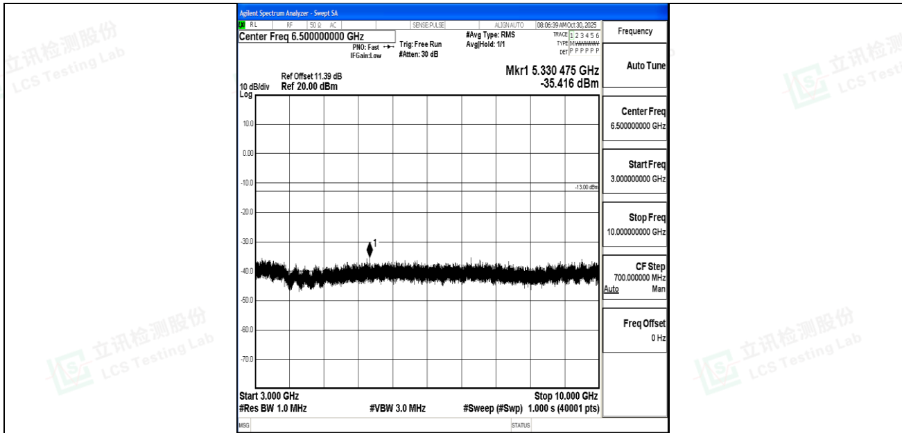
Band26_1.4MHz_16QAM_26783_1RB#0_3000~10000_3000~10000
