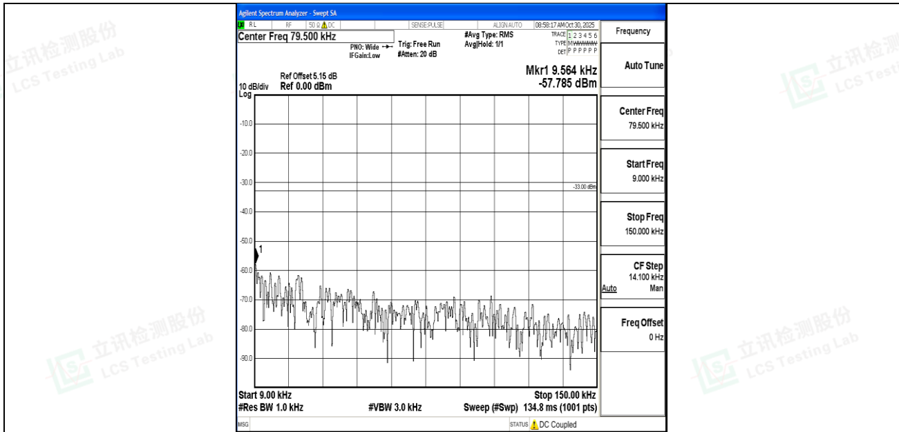
Band26_5MHz_16QAM_26740_1RB#0_0.009~0.15_0.009~0.15
