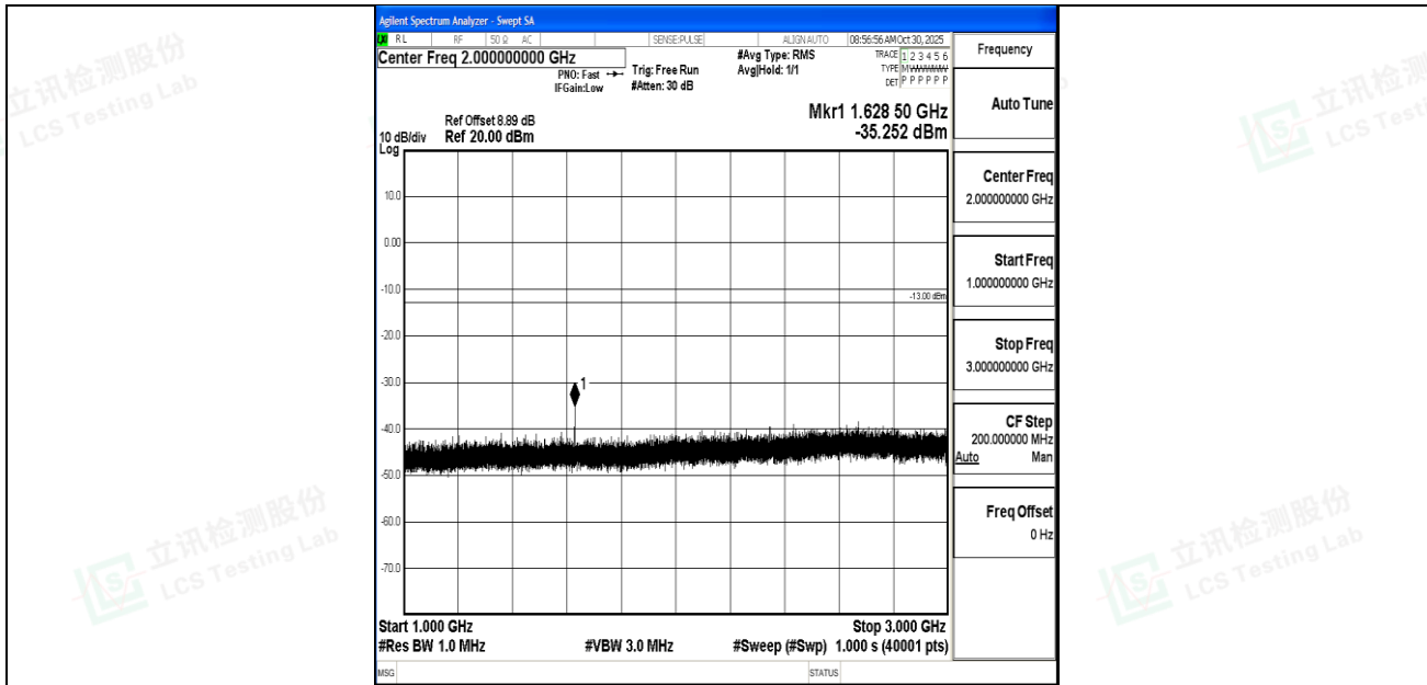
Band26_5MHz_QPSK_26715_1RB#0_1000~3000_1000~3000
