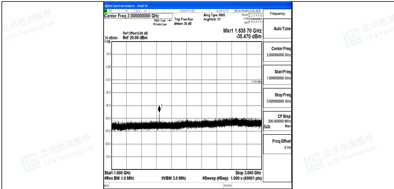
Band26_3MHz_QPSK_26740_1RB#0_1000~3000_1000~3000
