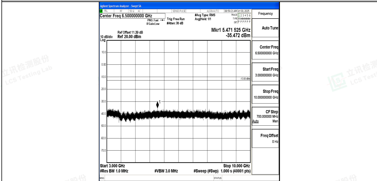
Band26_5MHz_QPSK_26765_1RB#0_3000~10000_3000~10000
