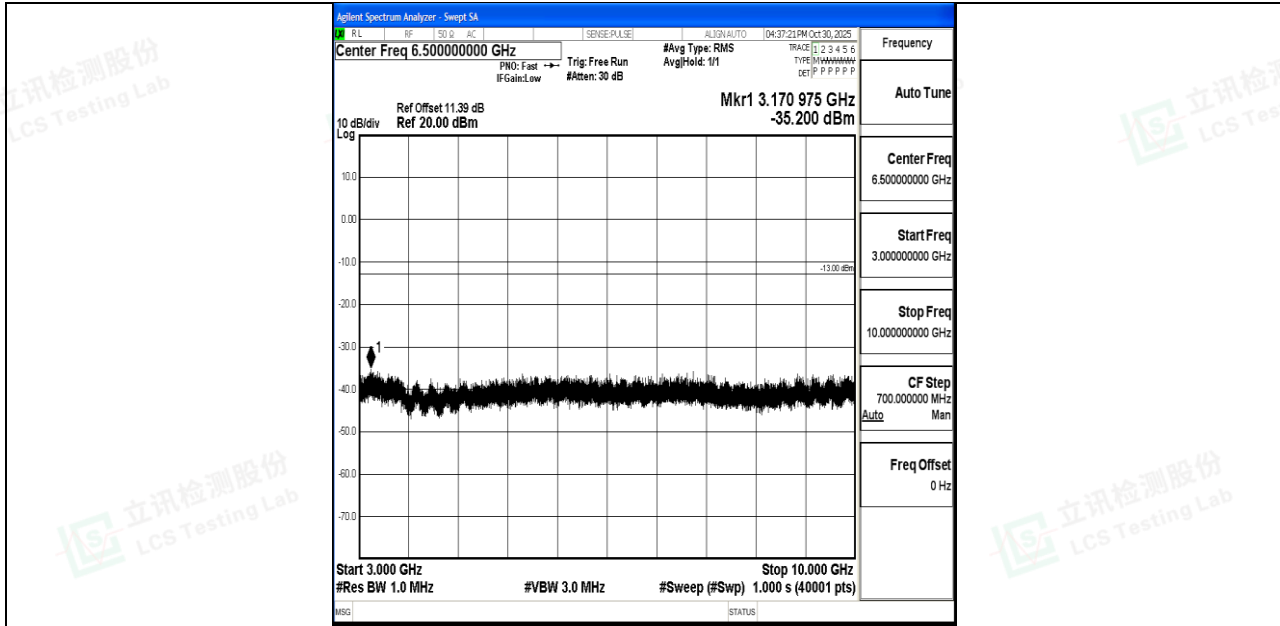
Band26_5MHz_QPSK_26915_1RB#0_3000~10000_3000~10000
