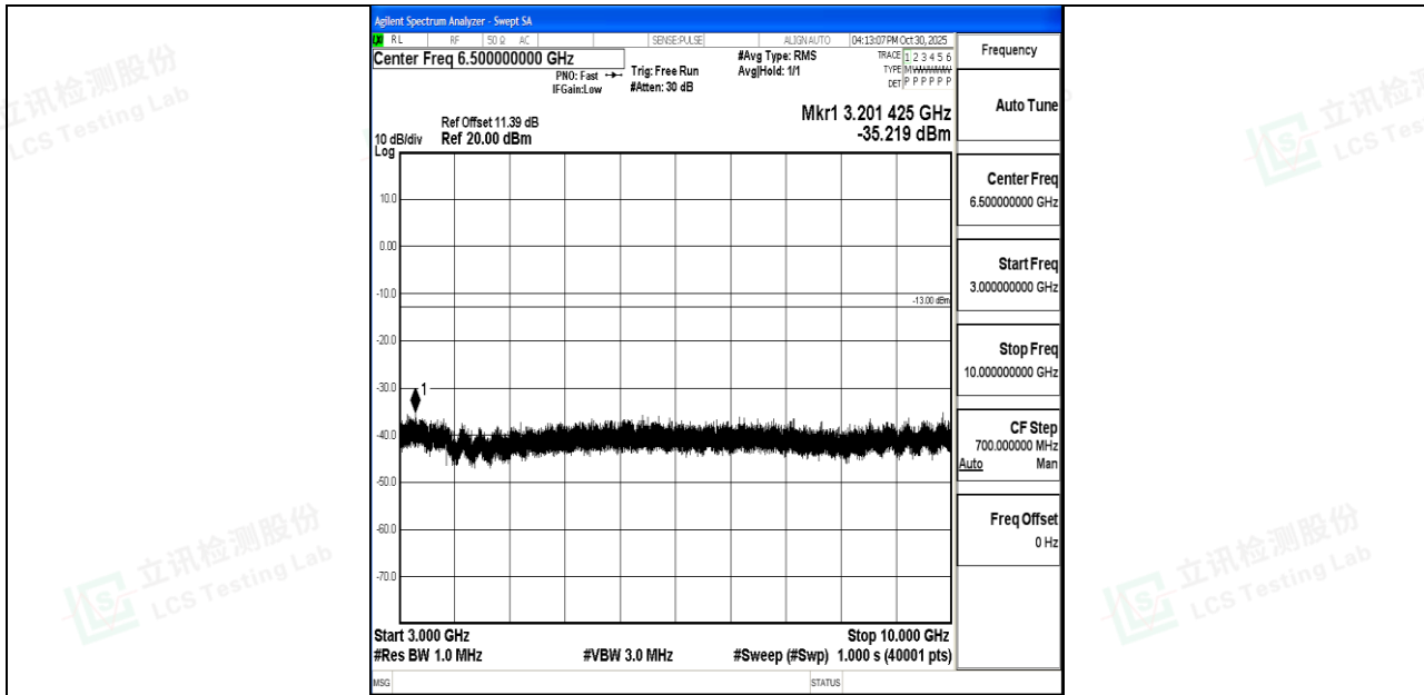
Band26_3MHz_QPSK_26915_1RB#0_3000~10000_3000~10000
