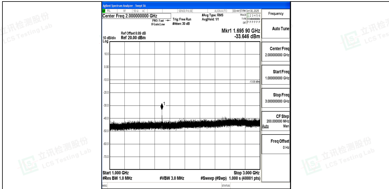
Band26_1.4MHz_16QAM_27033_1RB#0_1000~3000_1000~3000
