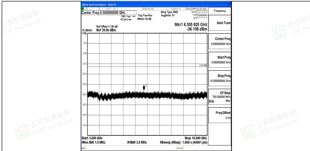
Band26_1.4MHz_QPSK_26797_1RB#0_3000~10000_3000~10000
