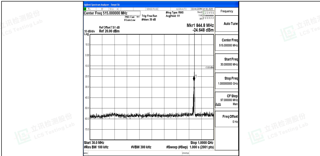
Band26_1.4MHz_QPSK_27033_1RB#0_30~1000_30~1000
