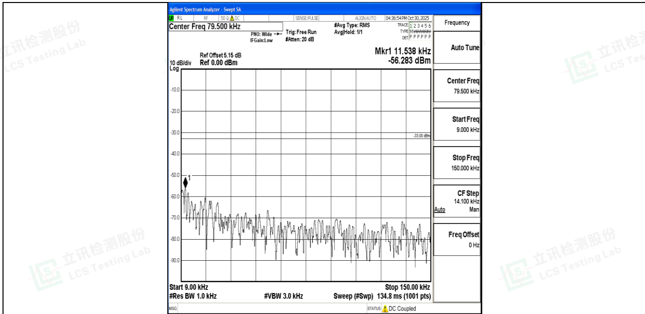
Band26_5MHz_QPSK_26915_1RB#0_0.009~0.15_0.009~0.15
