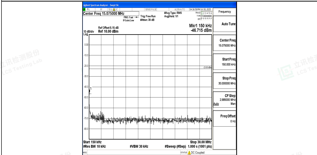
Band26_5MHz_QPSK_26915_1RB#0_0.15~30_0.15~30
