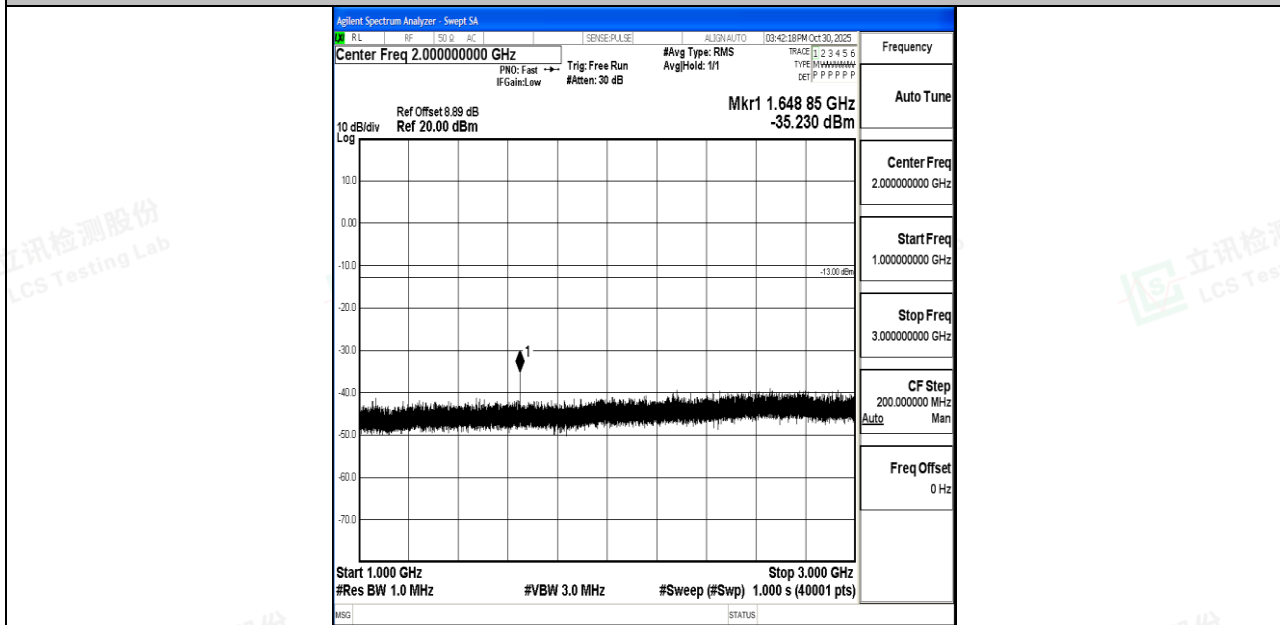
Band26_1.4MHz_QPSK_26797_1RB#0_1000~3000_1000~3000
