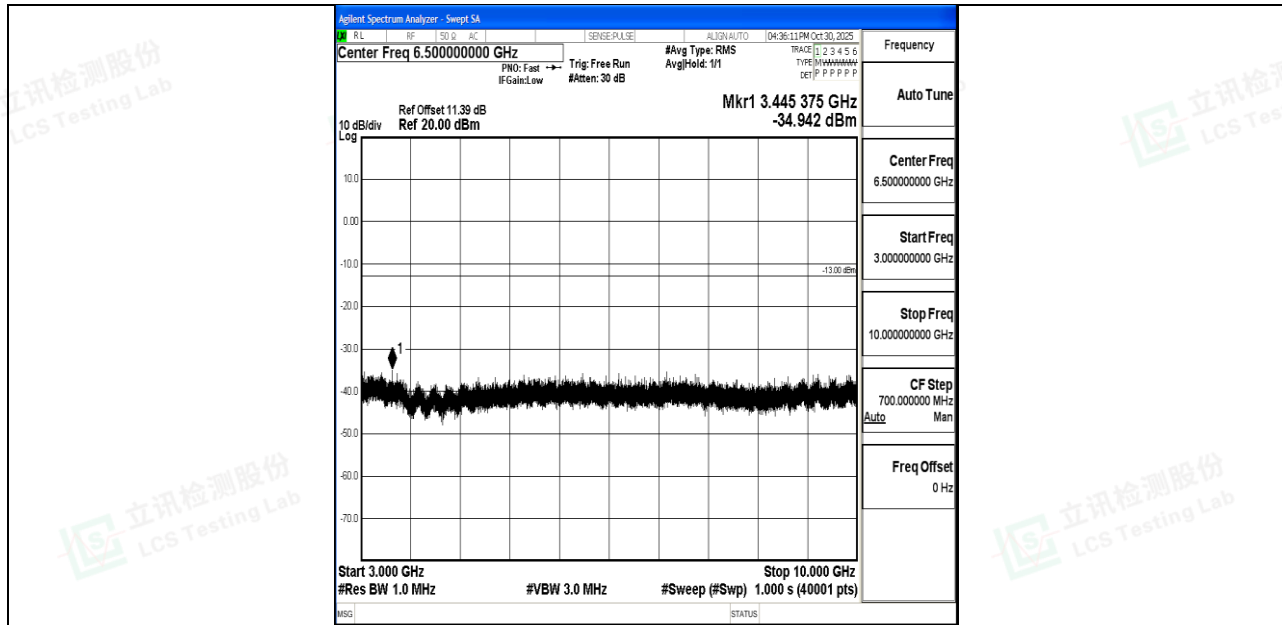
Band26_5MHz_QPSK_26815_1RB#0_3000~10000_3000~10000
