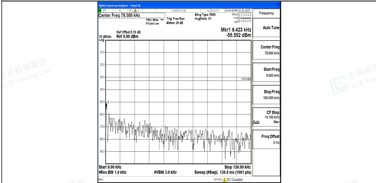
Band26_1.4MHz_16QAM_27033_1RB#0_0.009~0.15_0.009~0.15
