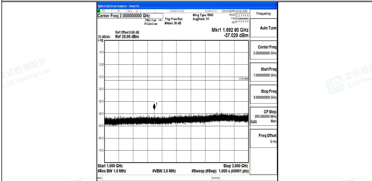
Band26_3MHz_QPSK_27025_1RB#0_1000~3000_1000~3000
