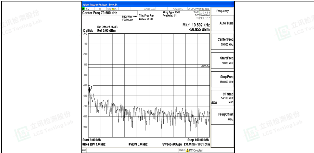
Band26_3MHz_QPSK_26915_1RB#0_0.009~0.15_0.009~0.15
