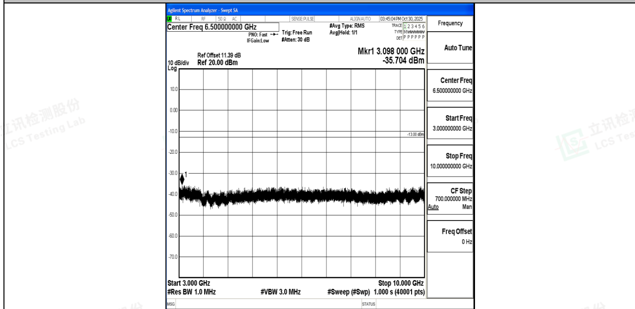
Band26_1.4MHz_16QAM_27033_1RB#0_3000~10000_3000~10000
