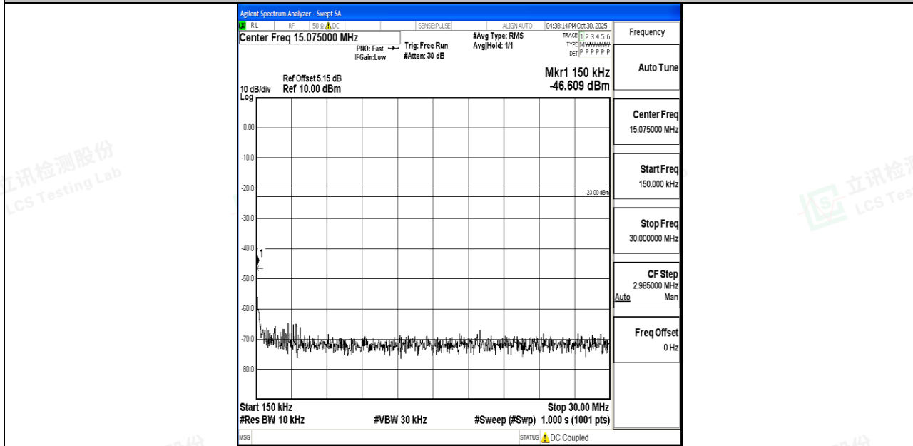
Band26_5MHz_QPSK_27015_1RB#0_0.15~30_0.15~30
