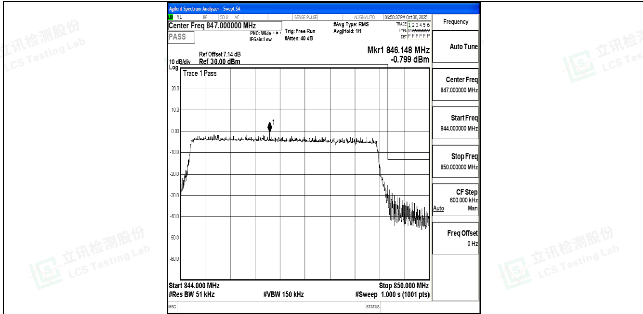
Band26_5MHz_QPSK_27015_25RB#0
