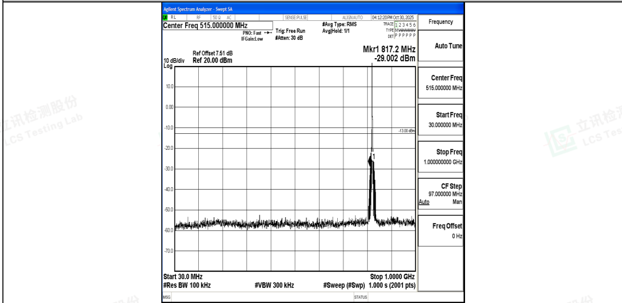
Band26_3MHz_16QAM_26805_1RB#0_30~1000_30~1000
