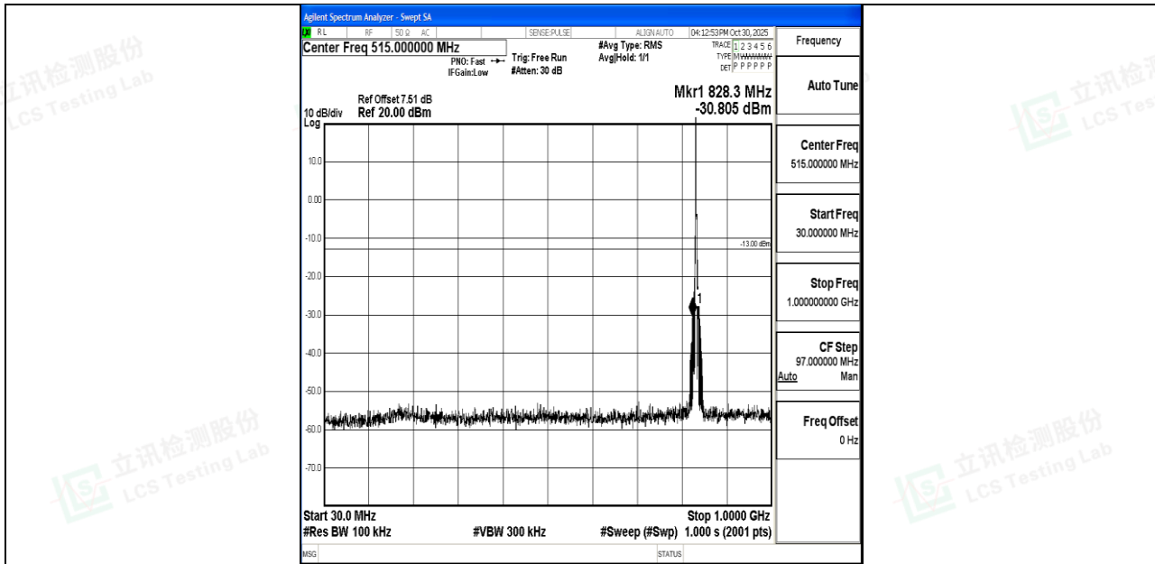
Band26_3MHz_QPSK_26915_1RB#0_30~1000_30~1000
