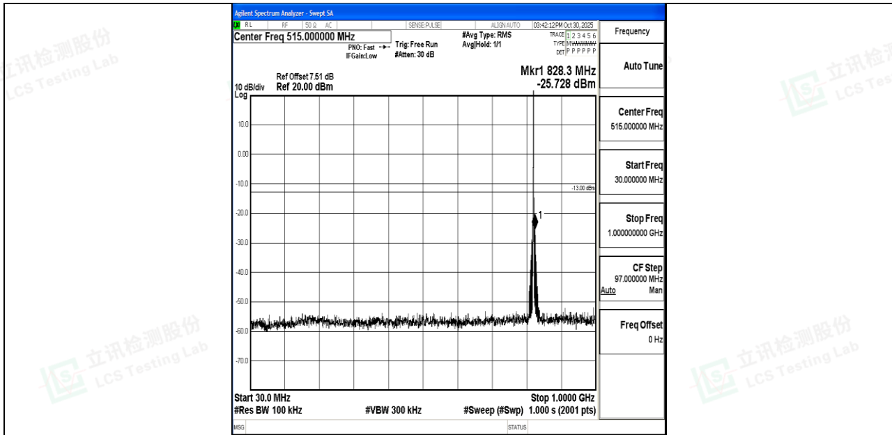
Band26_1.4MHz_QPSK_26797_1RB#0_30~1000_30~1000
