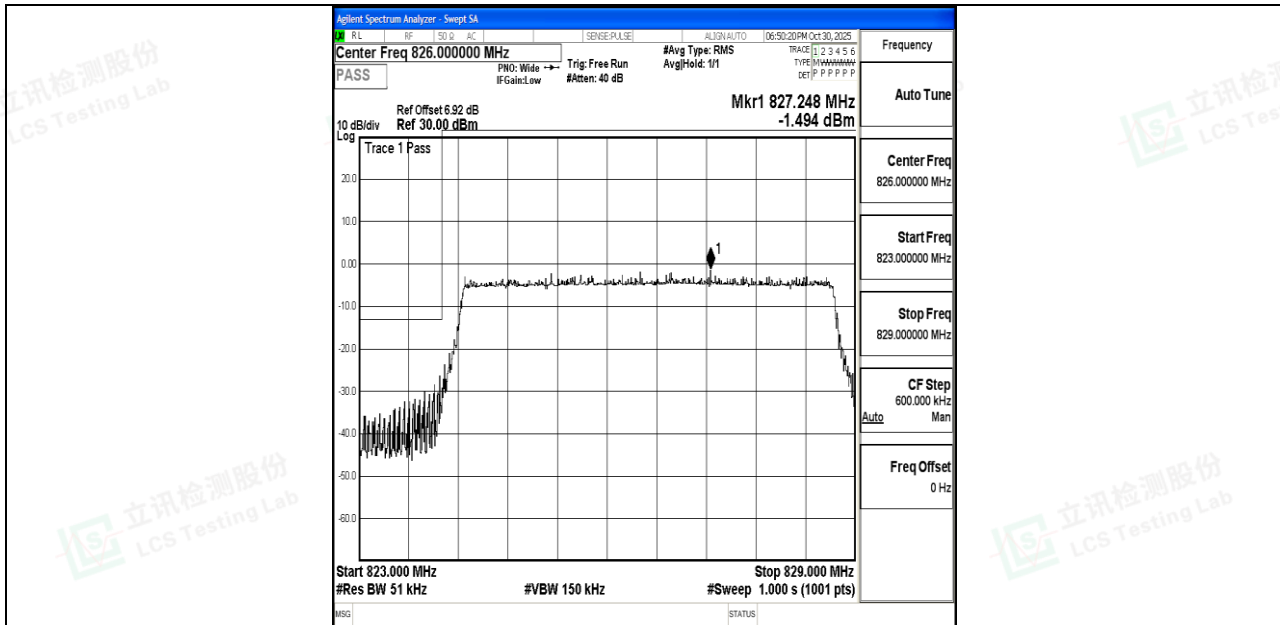
Band26_5MHz_QPSK_26815_25RB#0
