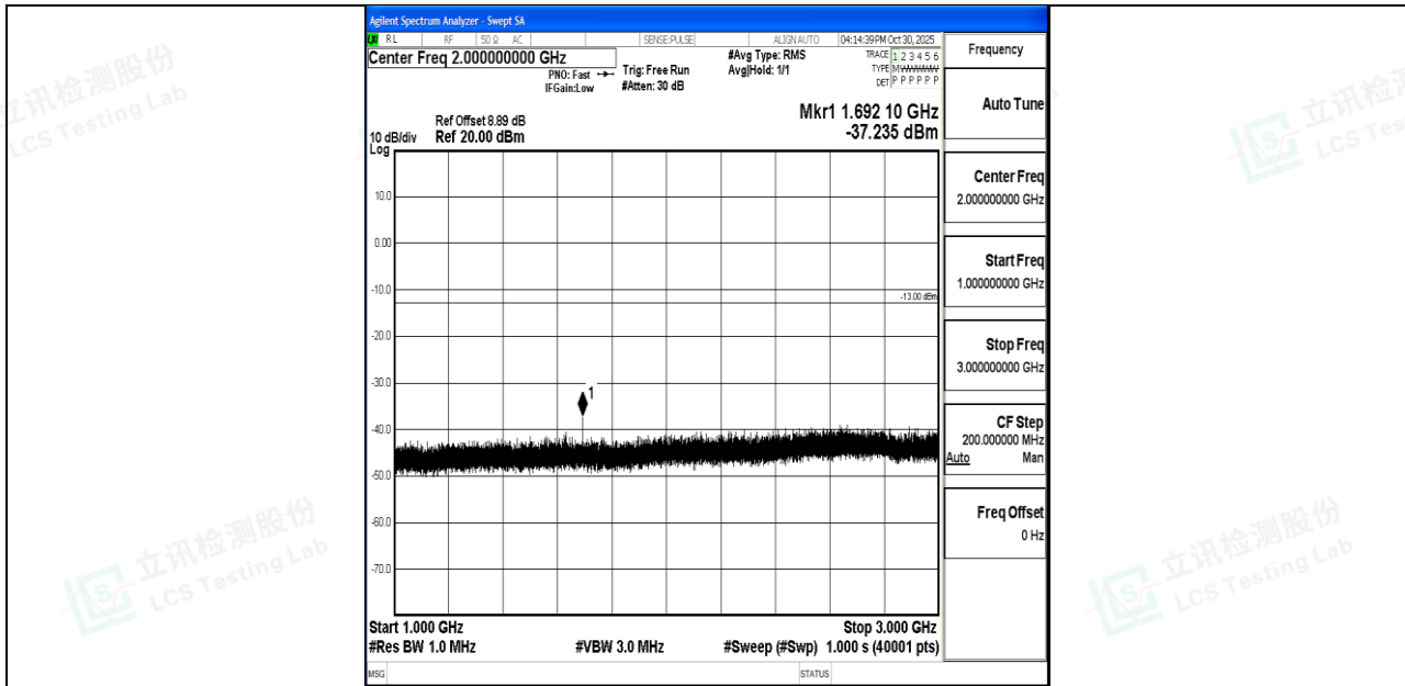
Band26_3MHz_16QAM_27025_1RB#0_1000~3000_1000~3000
