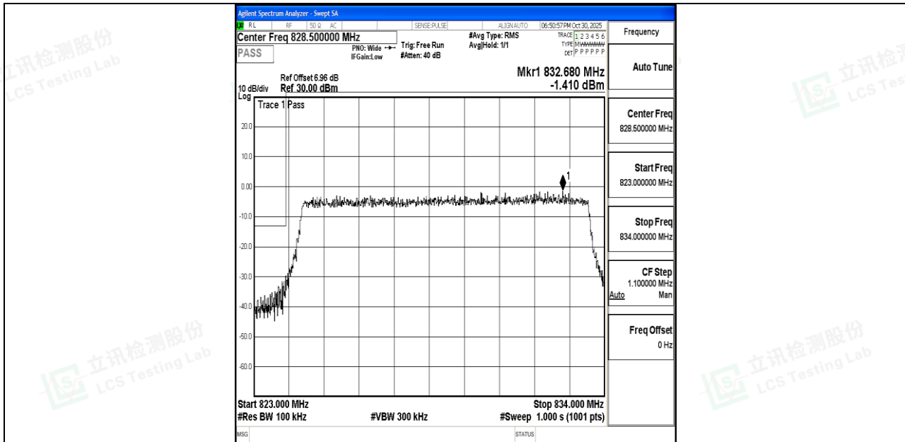
Band26_10MHz_QPSK_26840_50RB#0
