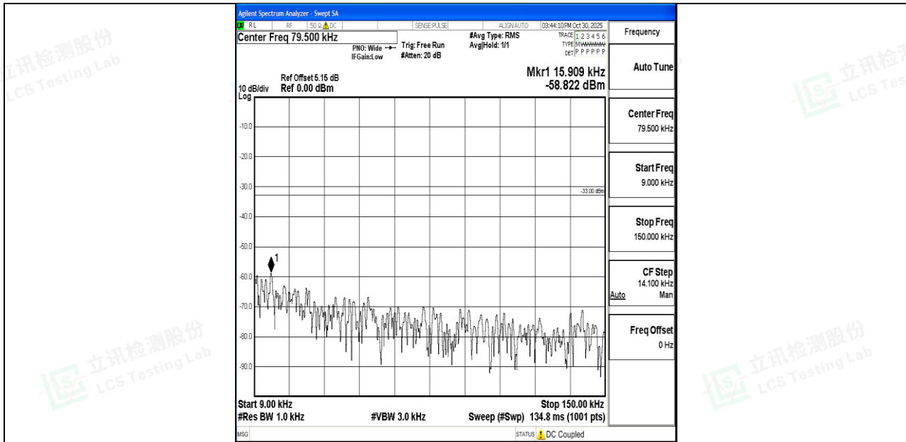
Band26_1.4MHz_QPSK_27033_1RB#0_0.009~0.15_0.009~0.15
