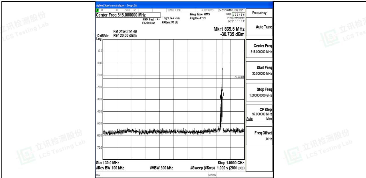
Band26_3MHz_QPSK_27025_1RB#0_30~1000_30~1000
