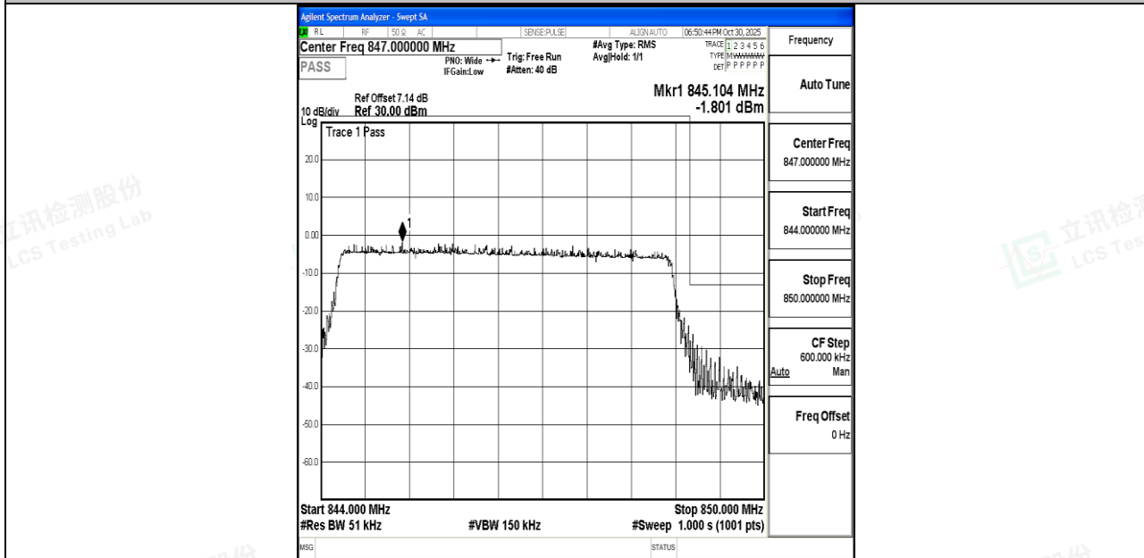
Band26_5MHz_16QAM_27015_25RB#0
