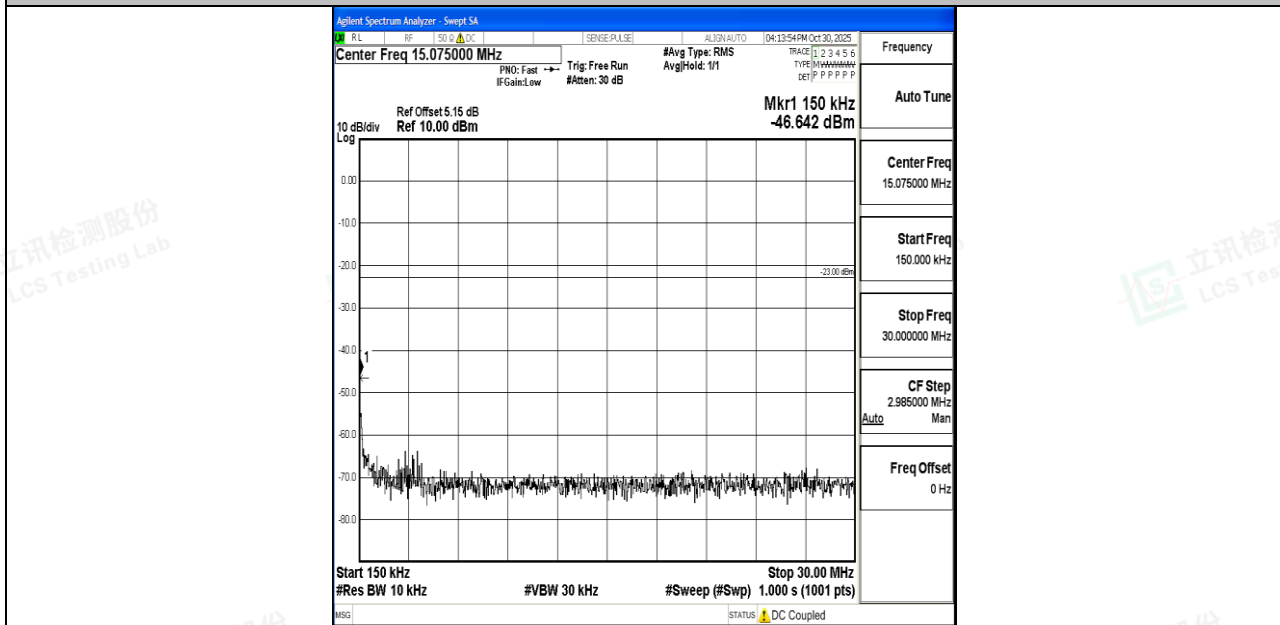
Band26_3MHz_QPSK_27025_1RB#0_0.15~30_0.15~30
