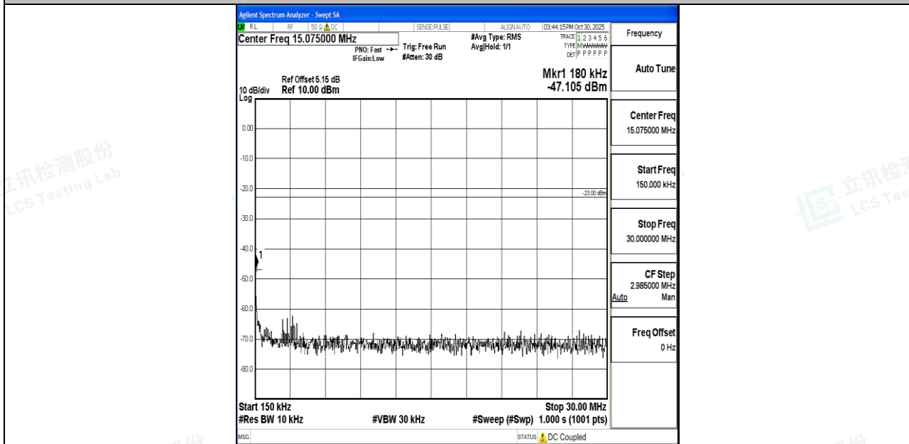
Band26_1.4MHz_QPSK_27033_1RB#0_0.15~30_0.15~30
