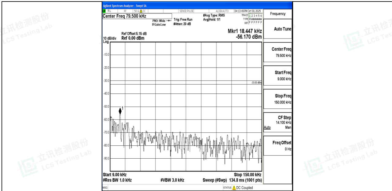
Band26_3MHz_QPSK_27025_1RB#0_0.009~0.15_0.009~0.15
