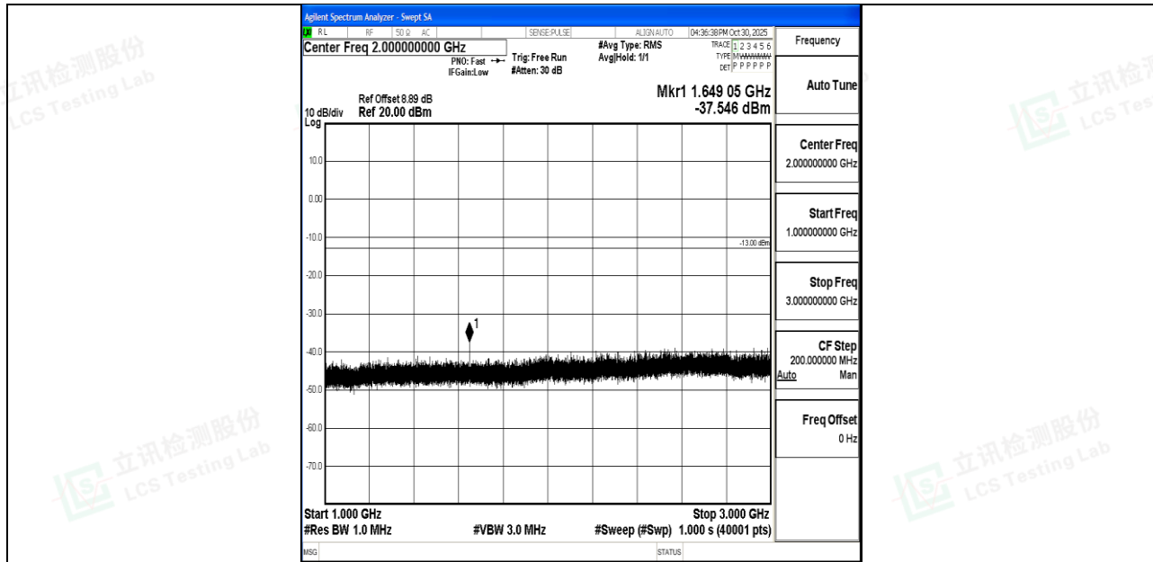
Band26_5MHz_16QAM_26815_1RB#0_1000~3000_1000~3000
