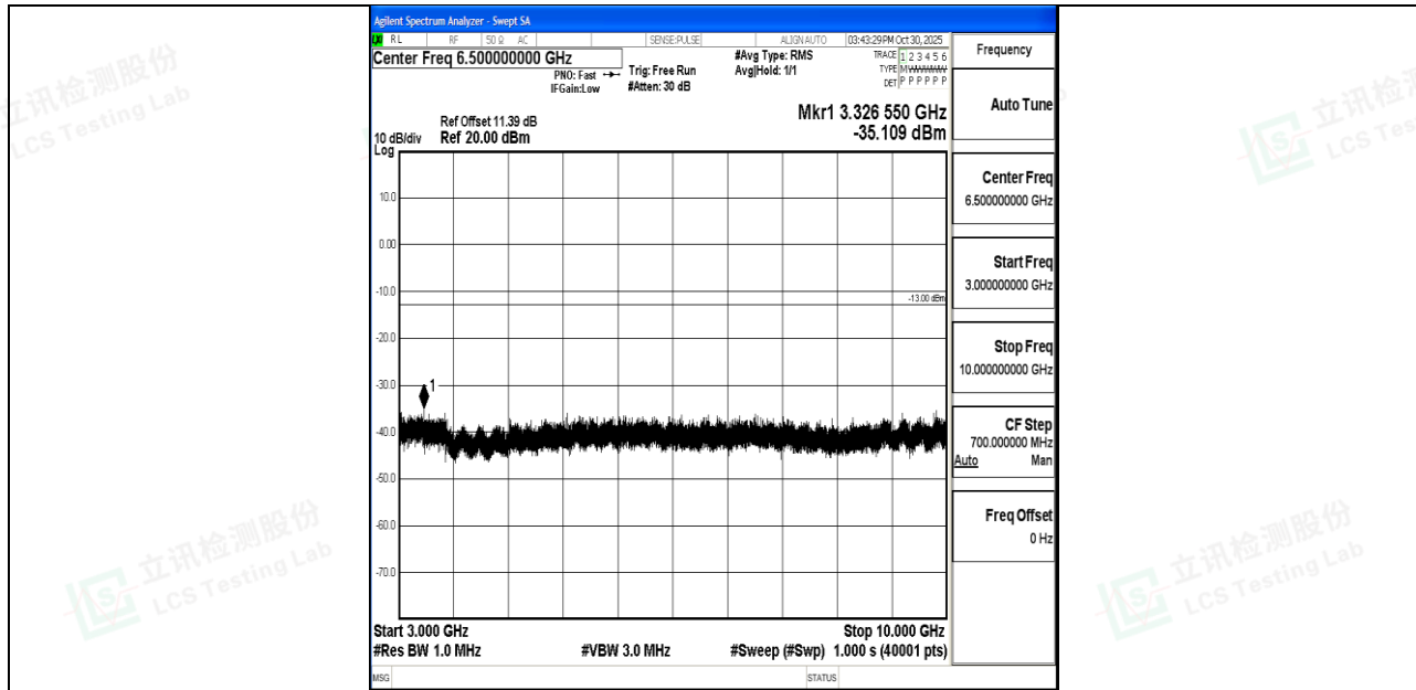
Band26_1.4MHz_QPSK_26915_1RB#0_3000~10000_3000~10000
