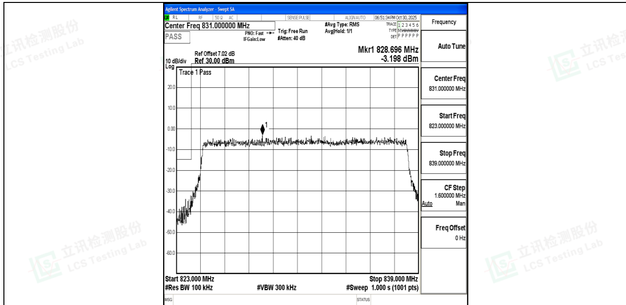
Band26_15MHz_QPSK_26865_75RB#0
