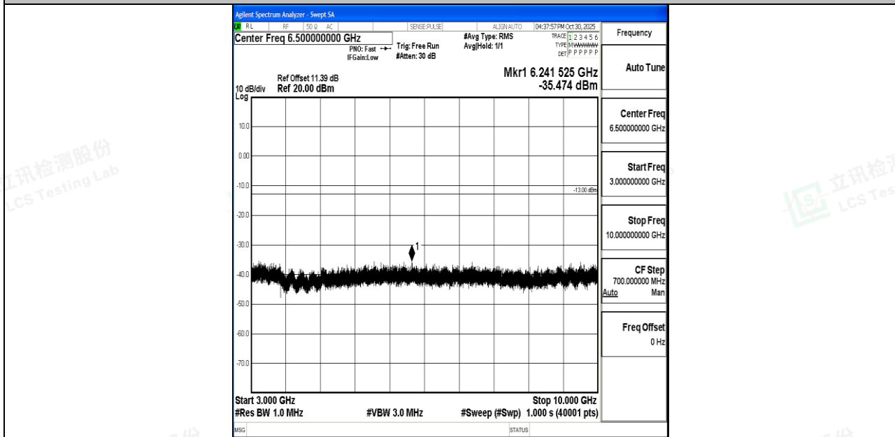
Band26_5MHz_16QAM_26915_1RB#0_3000~10000_3000~10000
