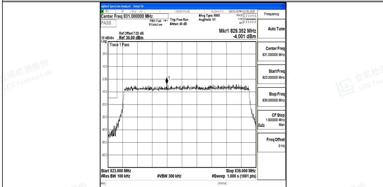
Band26_15MHz_16QAM_26865_75RB#0
