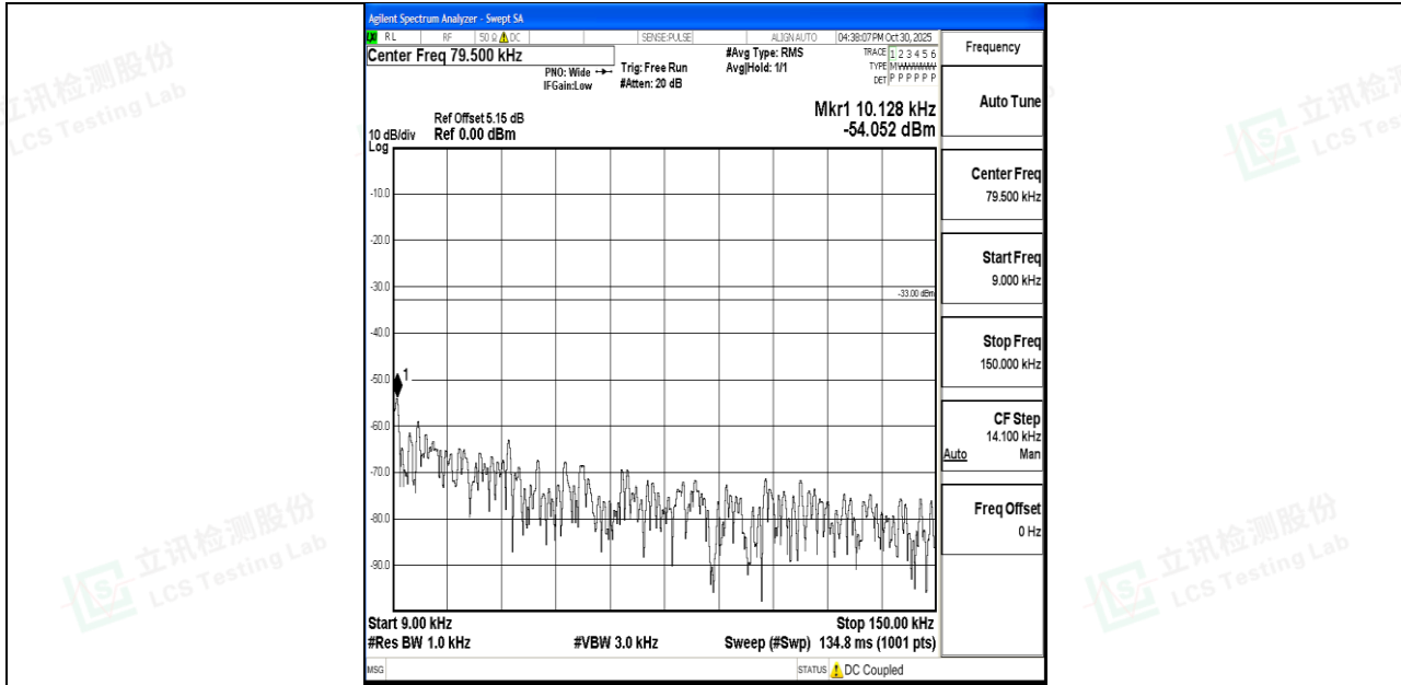
Band26_5MHz_QPSK_27015_1RB#0_0.009~0.15_0.009~0.15
