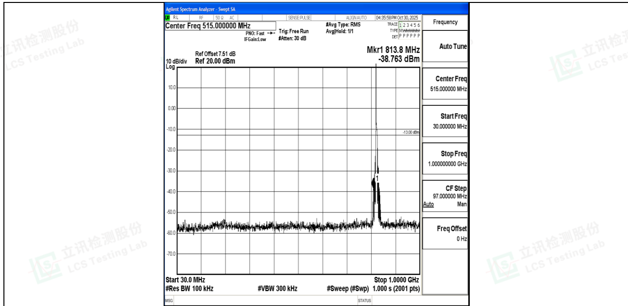
Band26_5MHz_QPSK_26815_1RB#0_30~1000_30~1000
