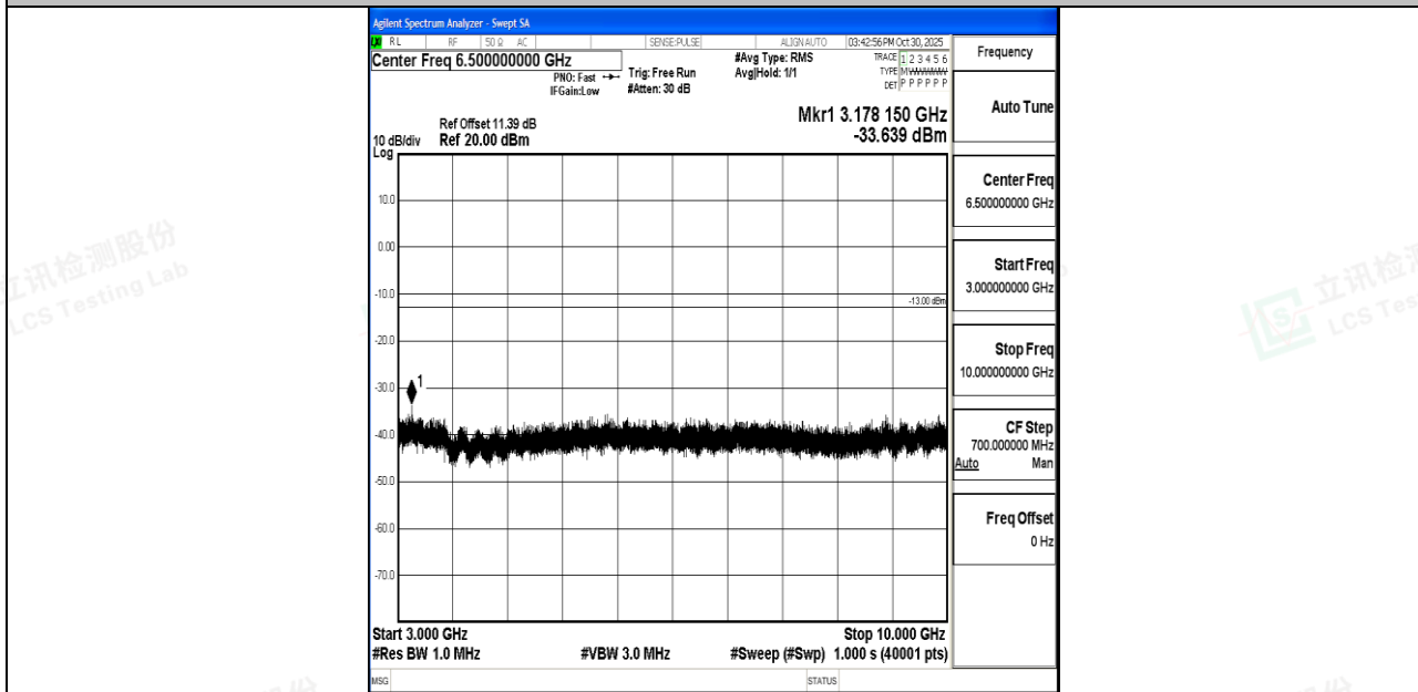
Band26_1.4MHz_16QAM_26797_1RB#0_3000~10000_3000~10000
