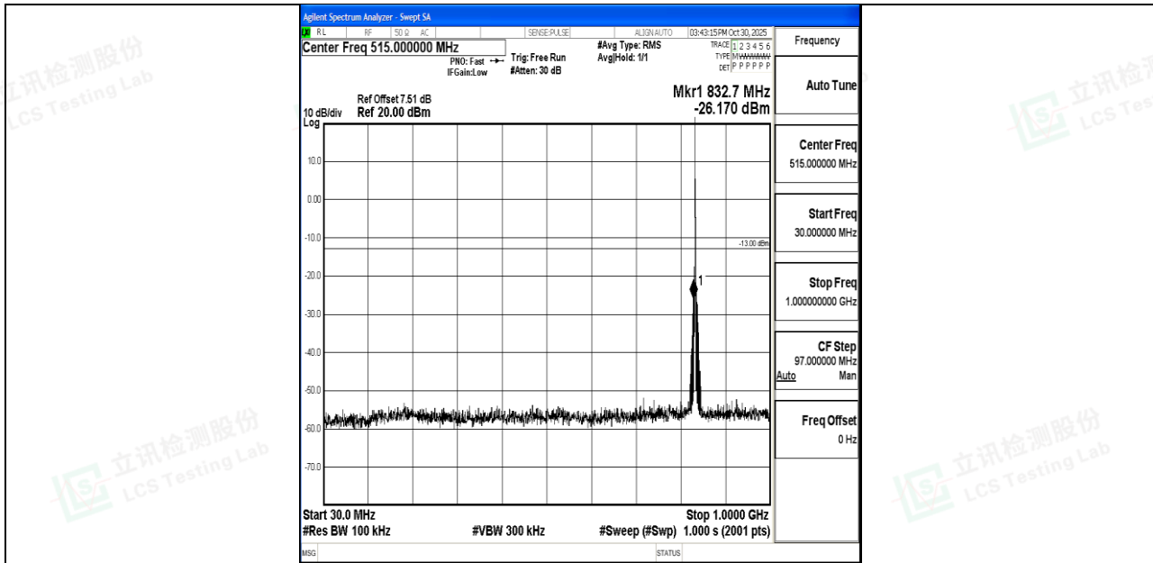
Band26_1.4MHz_QPSK_26915_1RB#0_30~1000_30~1000
