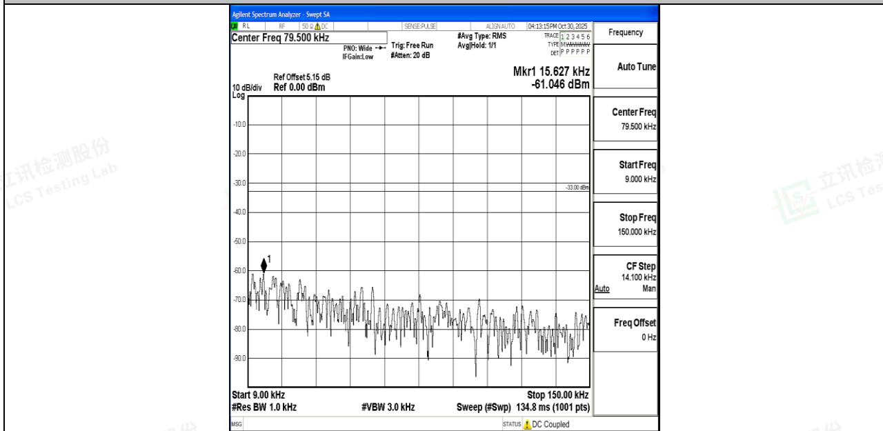
Band26_3MHz_16QAM_26915_1RB#0_0.009~0.15_0.009~0.15
