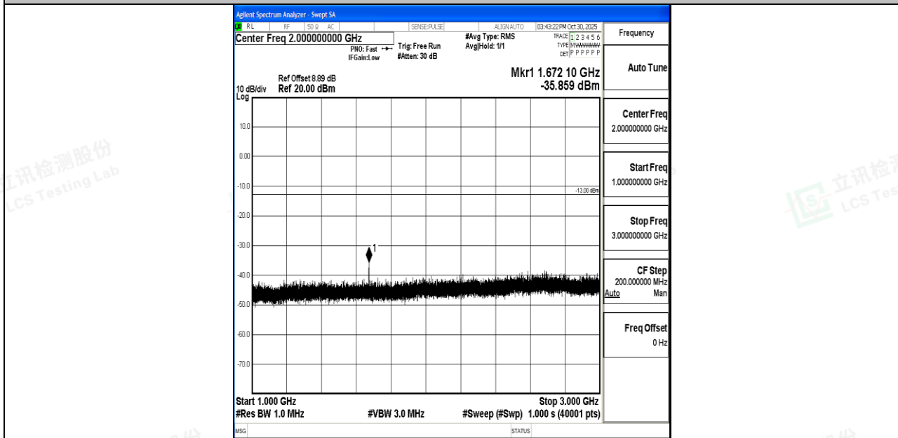
Band26_1.4MHz_QPSK_26915_1RB#0_1000~3000_1000~3000
