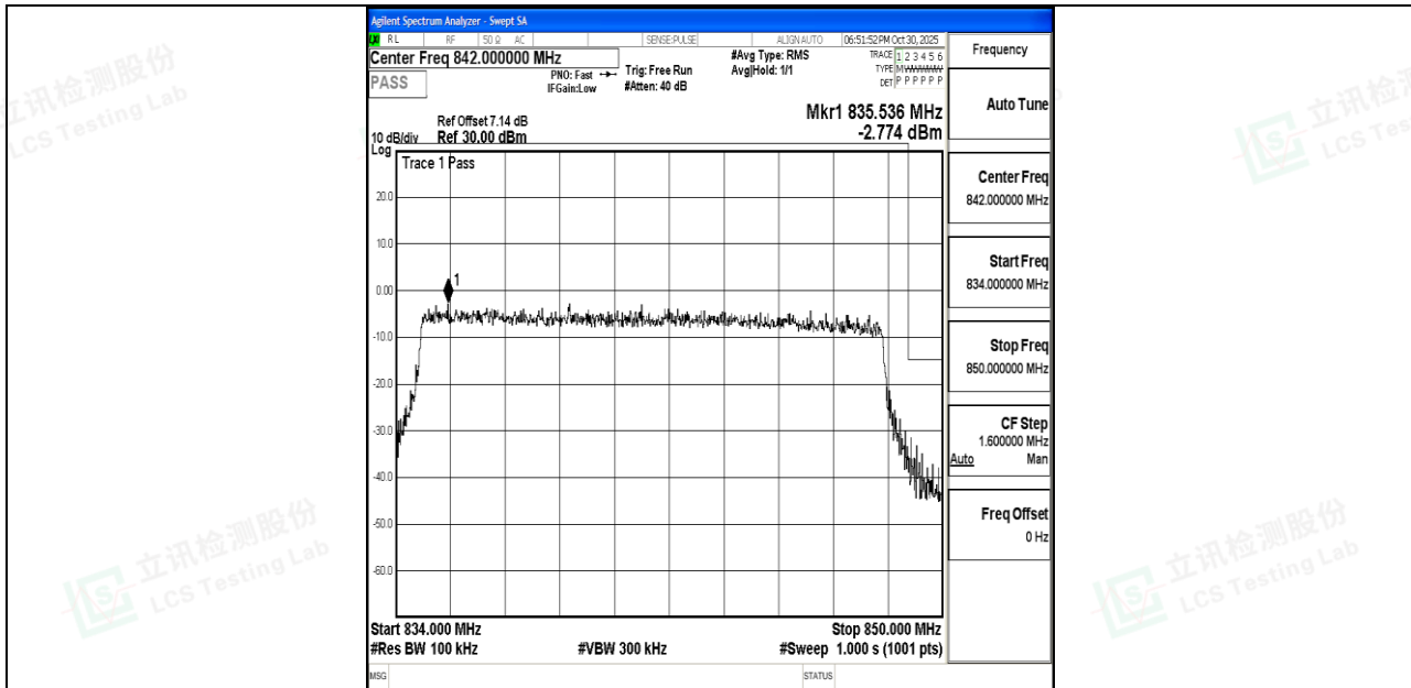
Band26_15MHz_QPSK_26965_75RB#0
