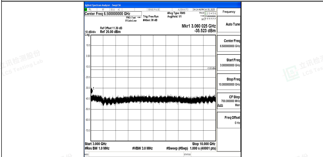
Band26_3MHz_16QAM_27025_1RB#0_3000~10000_3000~10000
