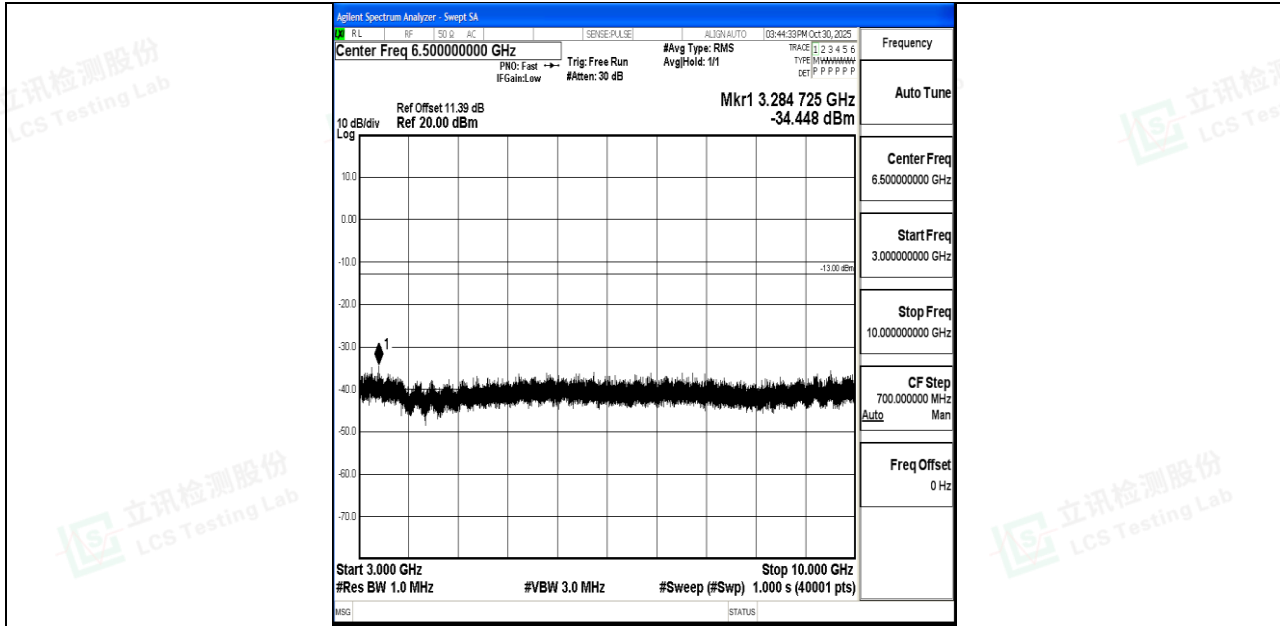
Band26_1.4MHz_QPSK_27033_1RB#0_3000~10000_3000~10000
