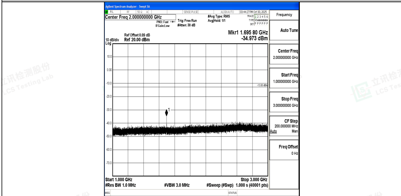
Band26_1.4MHz_QPSK_27033_1RB#0_1000~3000_1000~3000
