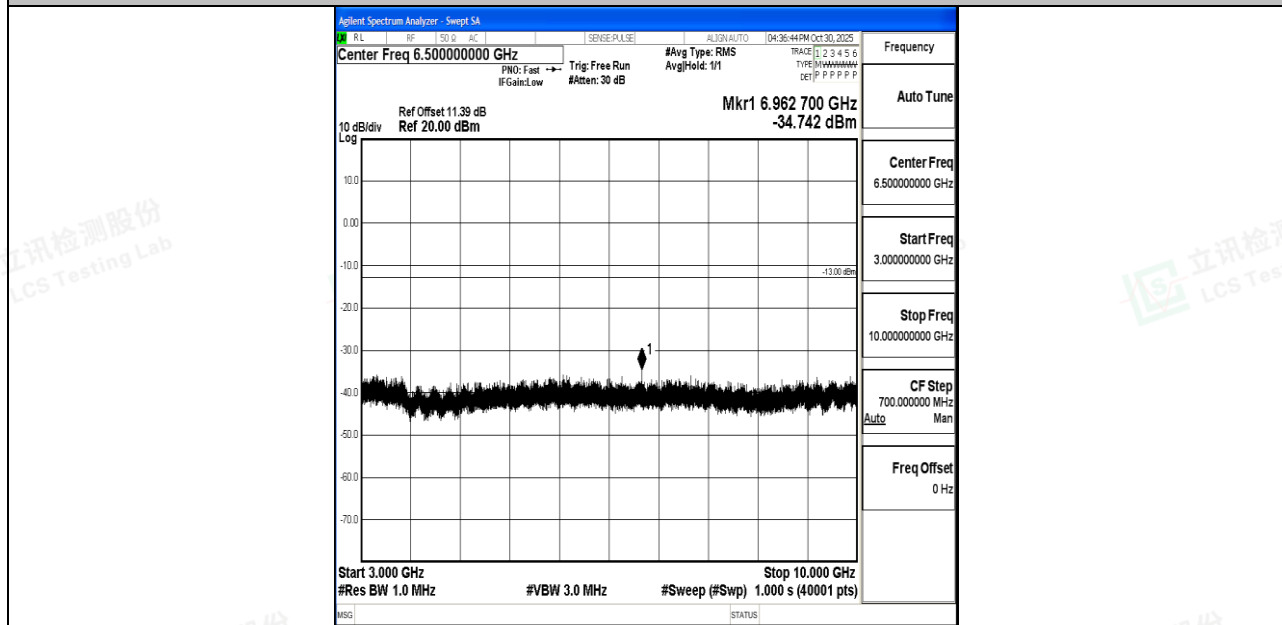
Band26_5MHz_16QAM_26815_1RB#0_3000~10000_3000~10000
