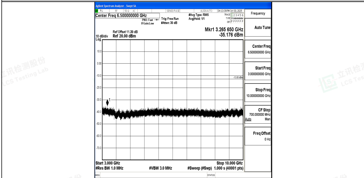
Band26_3MHz_16QAM_26915_1RB#0_3000~10000_3000~10000
