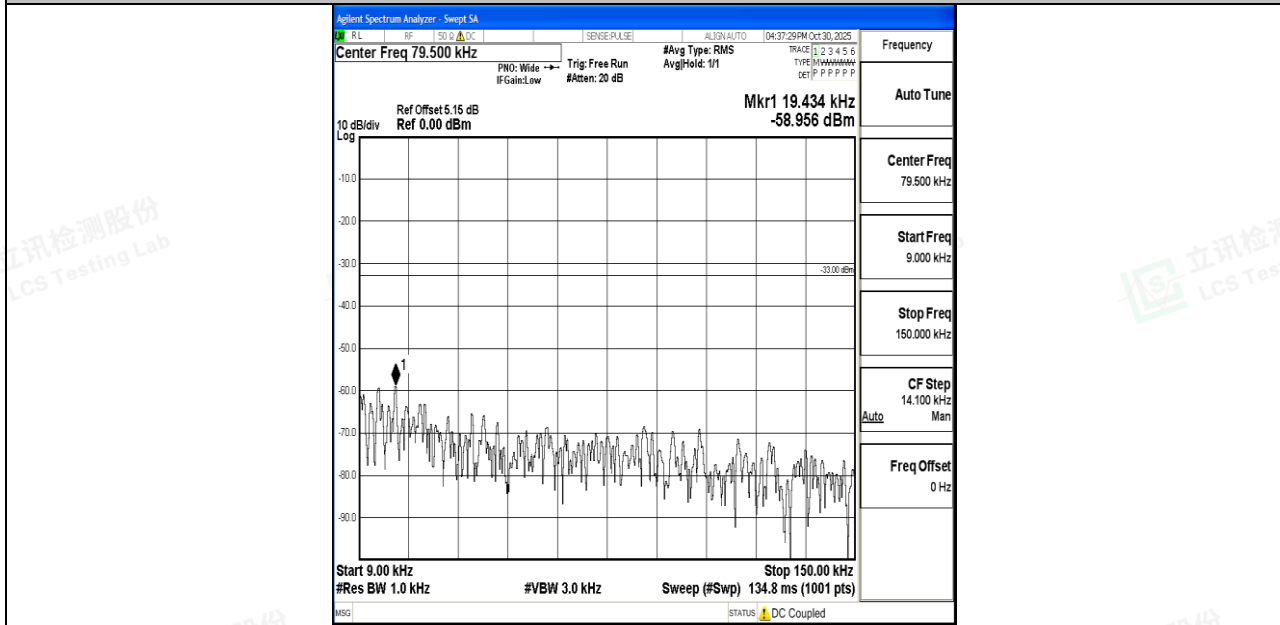
Band26_5MHz_16QAM_26915_1RB#0_0.009~0.15_0.009~0.15
