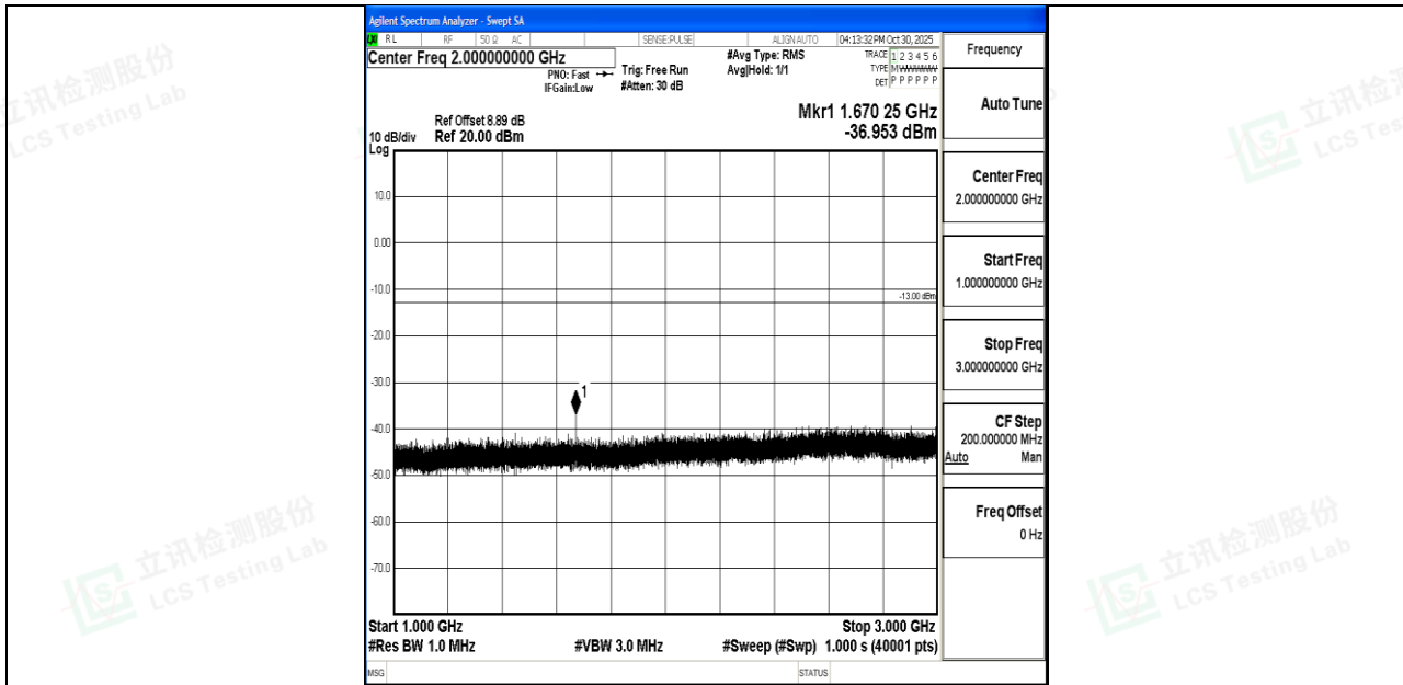
Band26_3MHz_16QAM_26915_1RB#0_1000~3000_1000~3000
