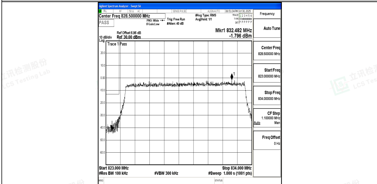
Band26_10MHz_16QAM_26840_50RB#0
