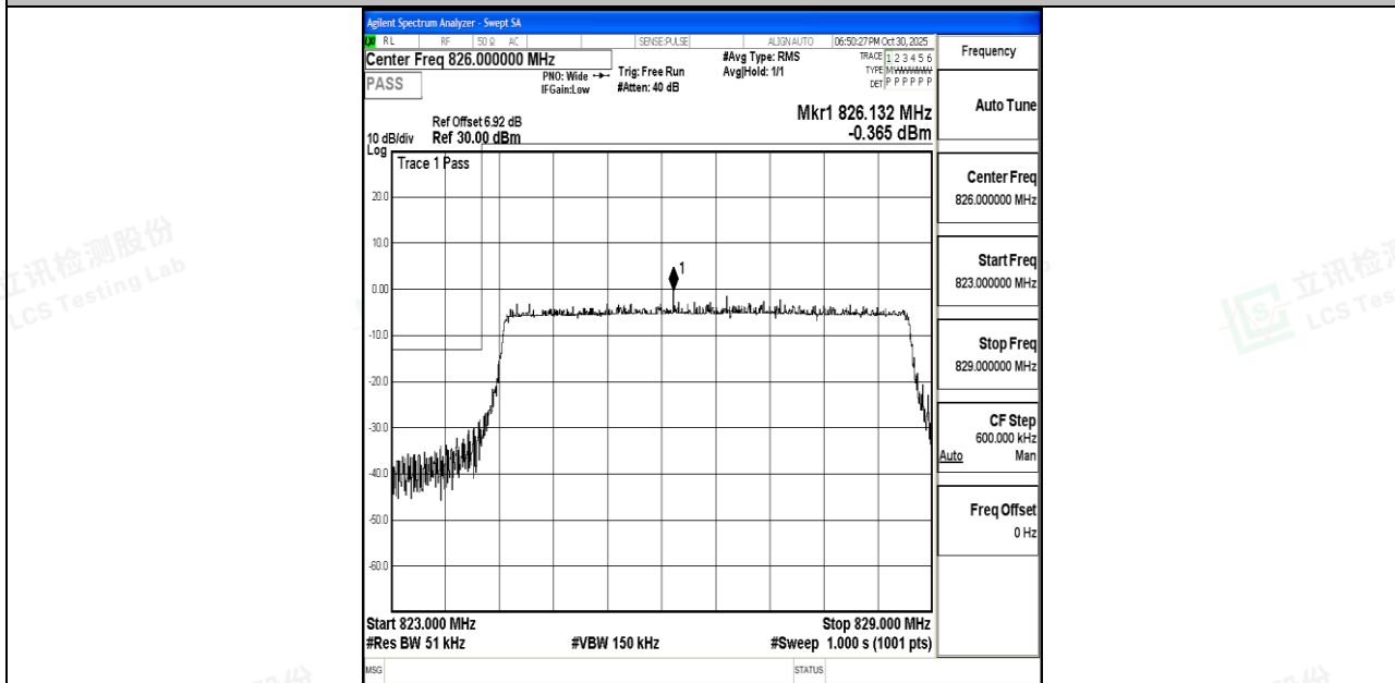
Band26_5MHz_16QAM_26815_25RB#0
