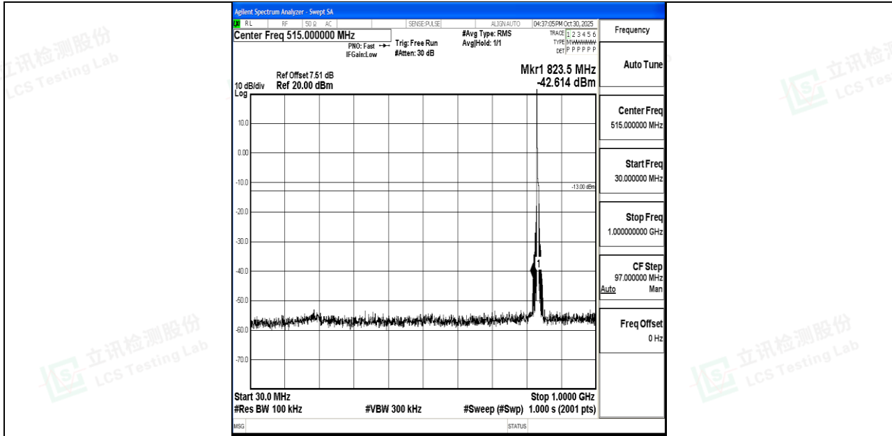
Band26_5MHz_QPSK_26915_1RB#0_30~1000_30~1000
