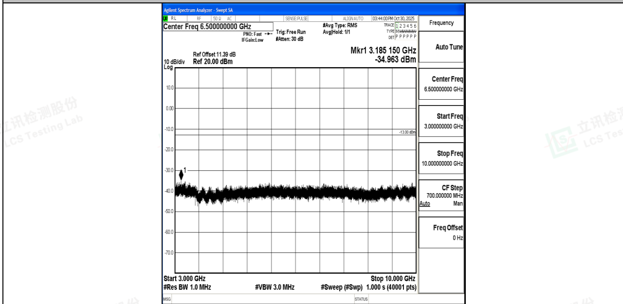
Band26_1.4MHz_16QAM_26915_1RB#0_3000~10000_3000~10000
