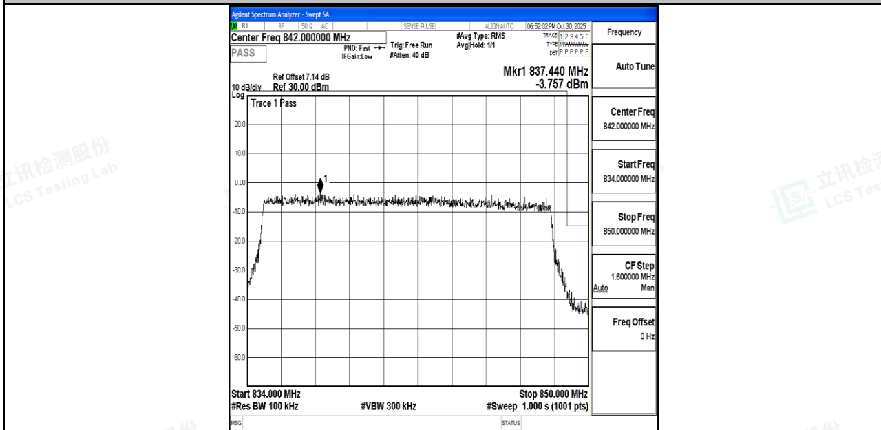
Band26_15MHz_16QAM_26965_75RB#0
