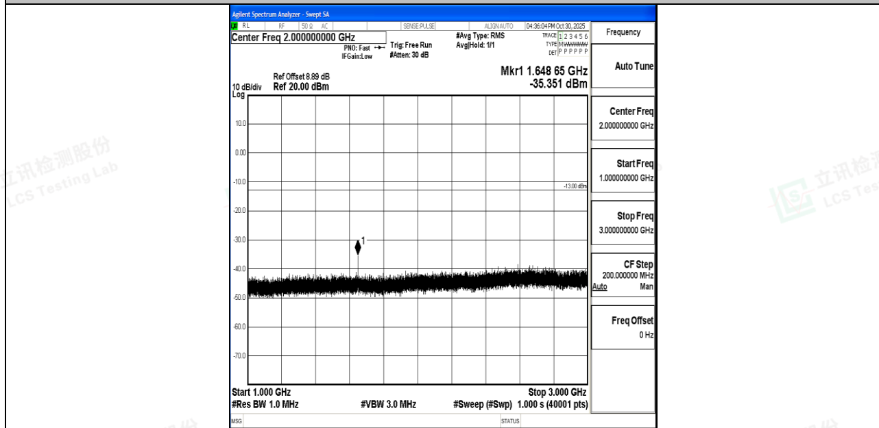
Band26_5MHz_QPSK_26815_1RB#0_1000~3000_1000~3000
