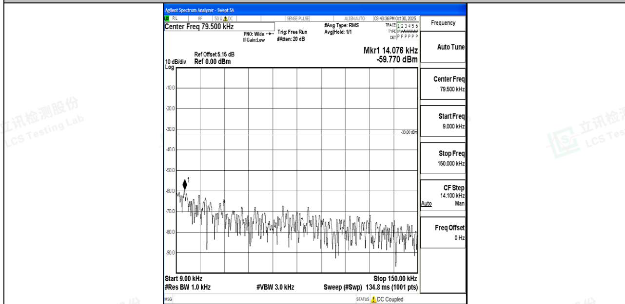
Band26_1.4MHz_16QAM_26915_1RB#0_0.009~0.15_0.009~0.15
