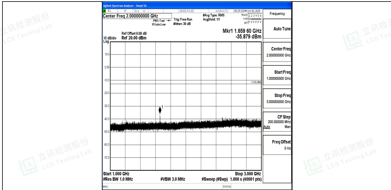
Band26_15MHz_16QAM_26915_1RB#0_1000~3000_1000~3000
