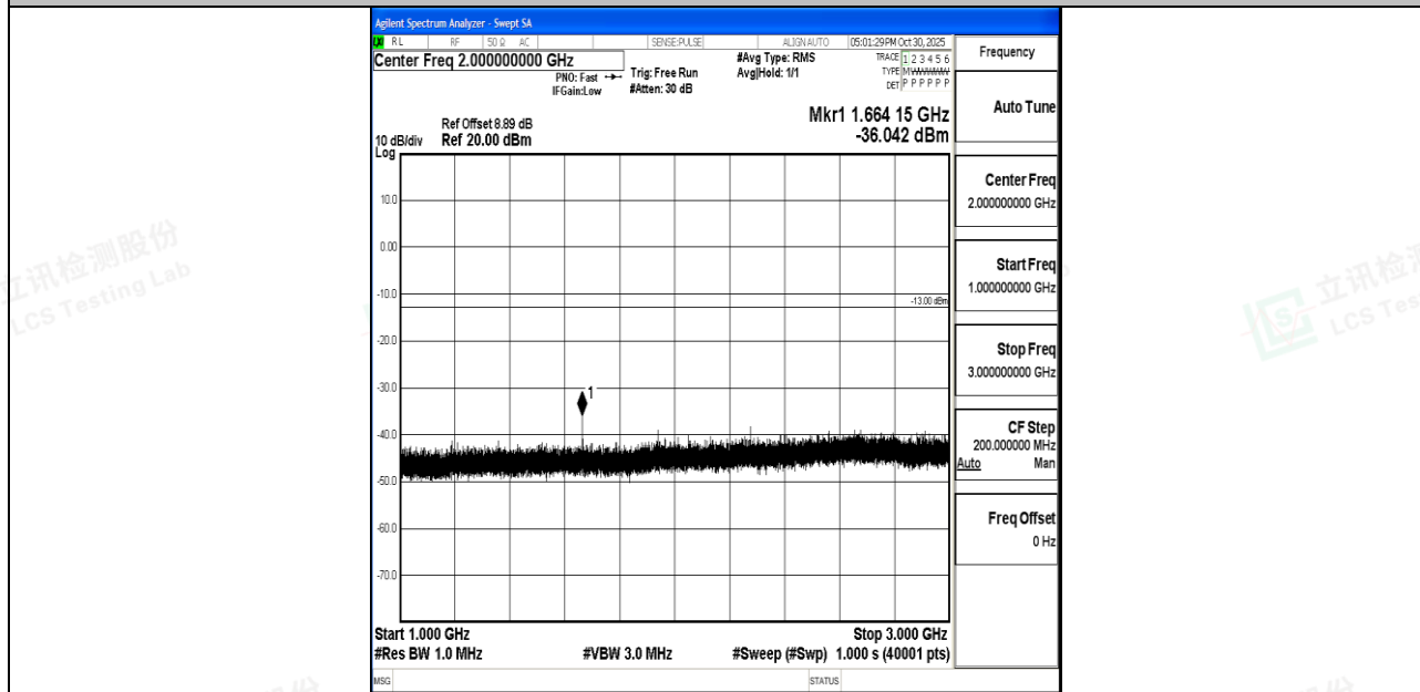
Band26_10MHz_QPSK_26915_1RB#0_1000~3000_1000~3000
