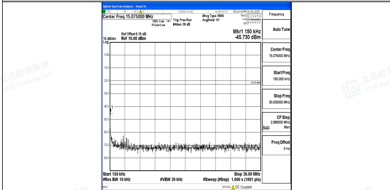
Band26_15MHz_QPSK_26915_1RB#0_0.15~30_0.15~30
