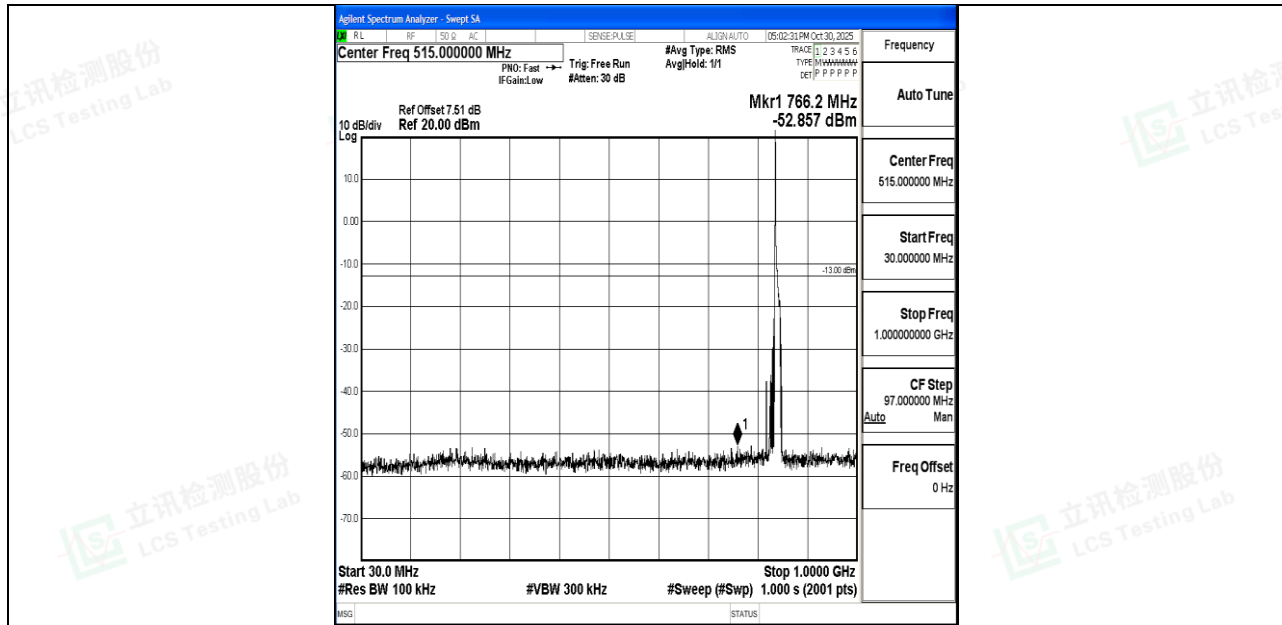
Band26_10MHz_QPSK_26990_1RB#0_30~1000_30~1000
