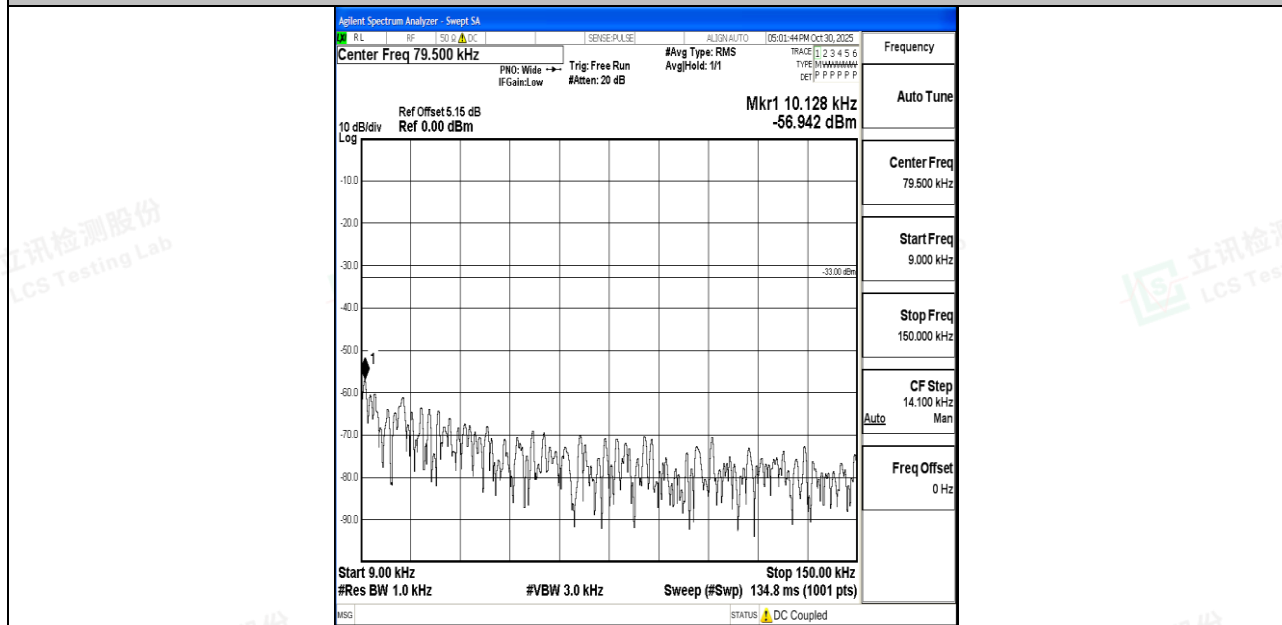
Band26_10MHz_16QAM_26915_1RB#0_0.009~0.15_0.009~0.15
