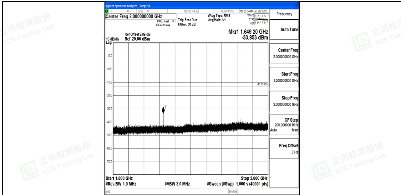
Band26_10MHz_16QAM_26840_1RB#0_1000~3000_1000~3000
