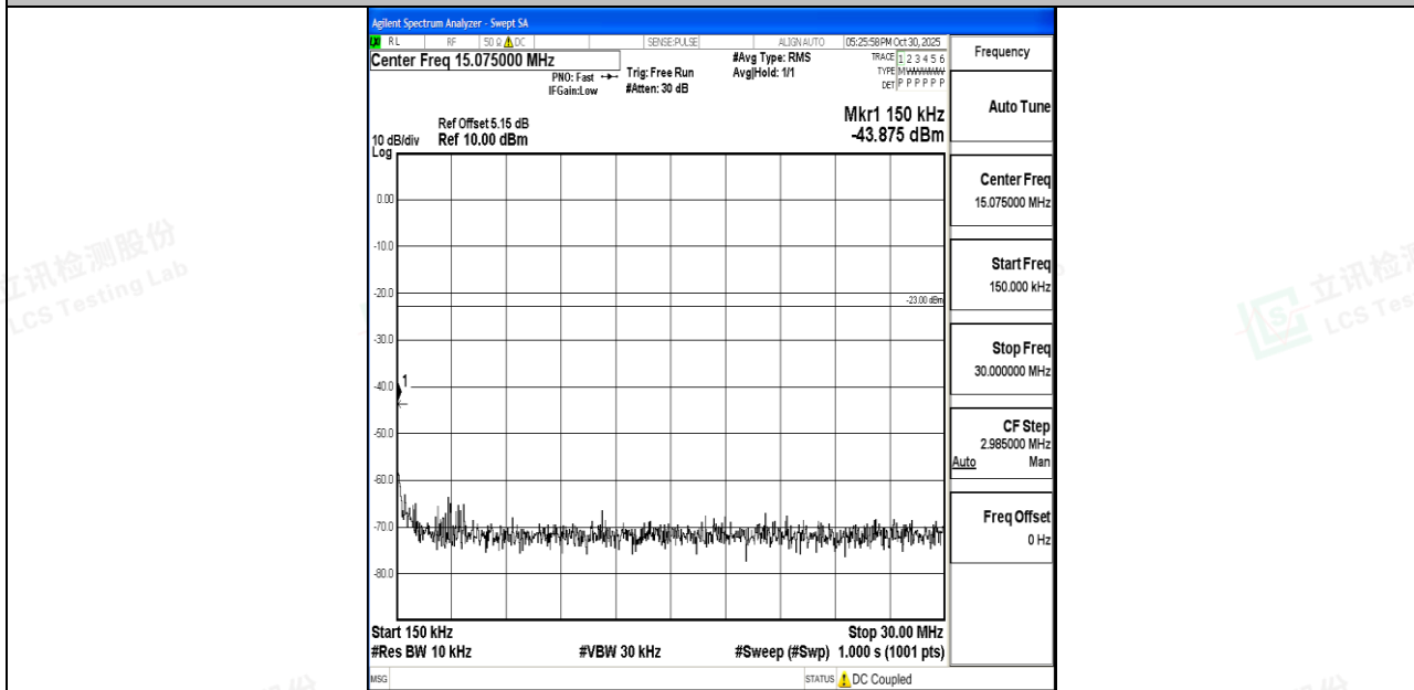
Band26_15MHz_QPSK_26965_1RB#0_0.15~30_0.15~30
