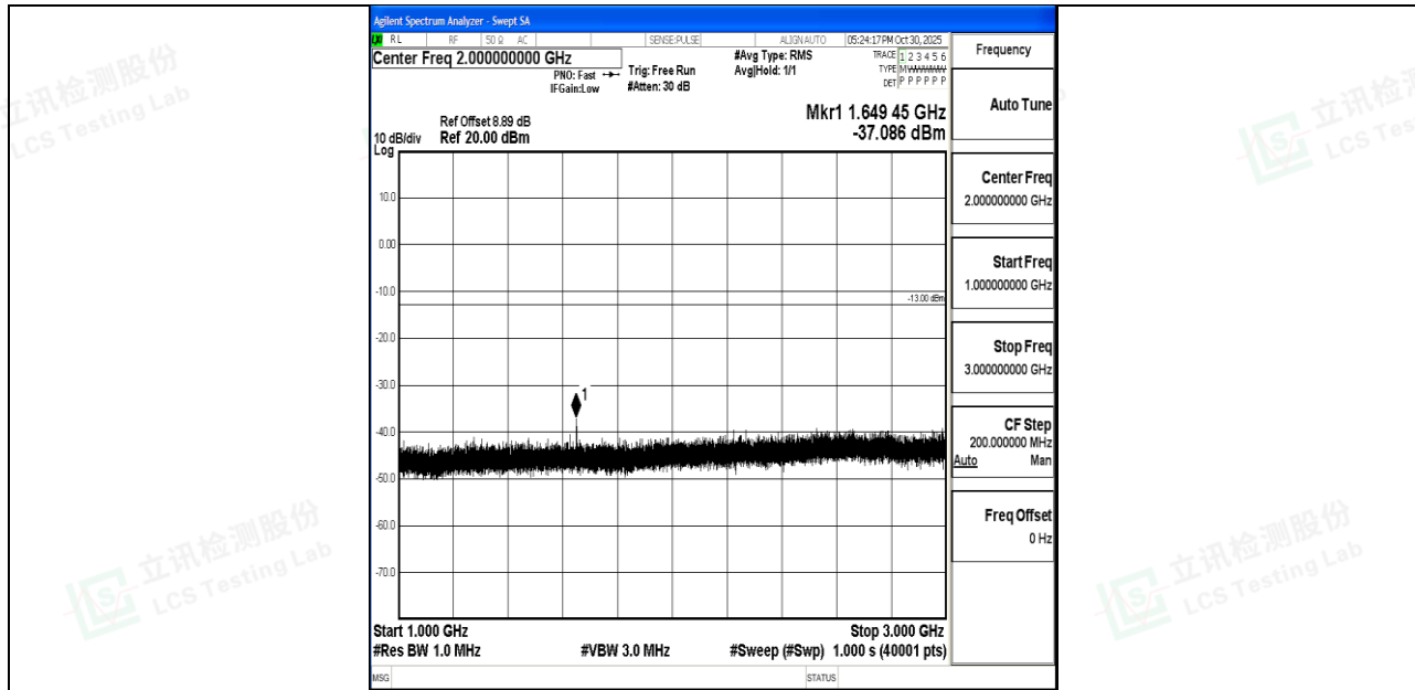
Band26_15MHz_16QAM_26865_1RB#0_1000~3000_1000~3000
