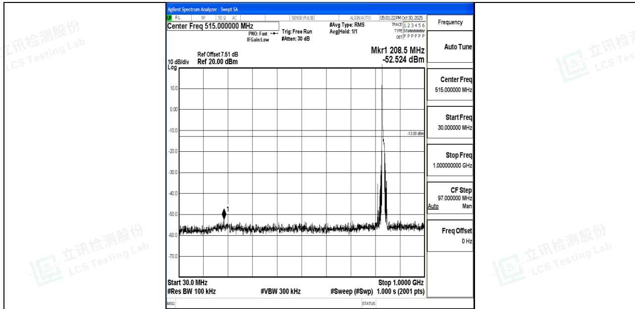
Band26_10MHz_QPSK_26915_1RB#0_30~1000_30~1000
