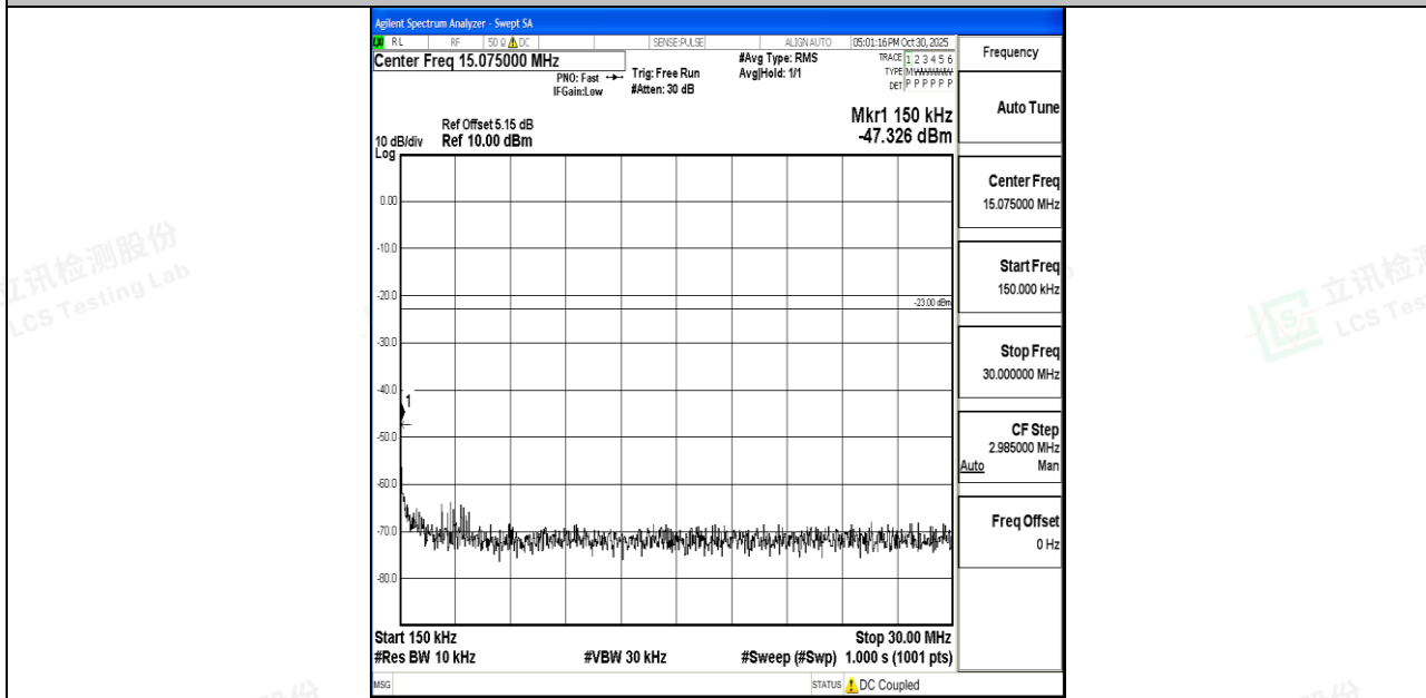
Band26_10MHz_QPSK_26915_1RB#0_0.15~30_0.15~30
