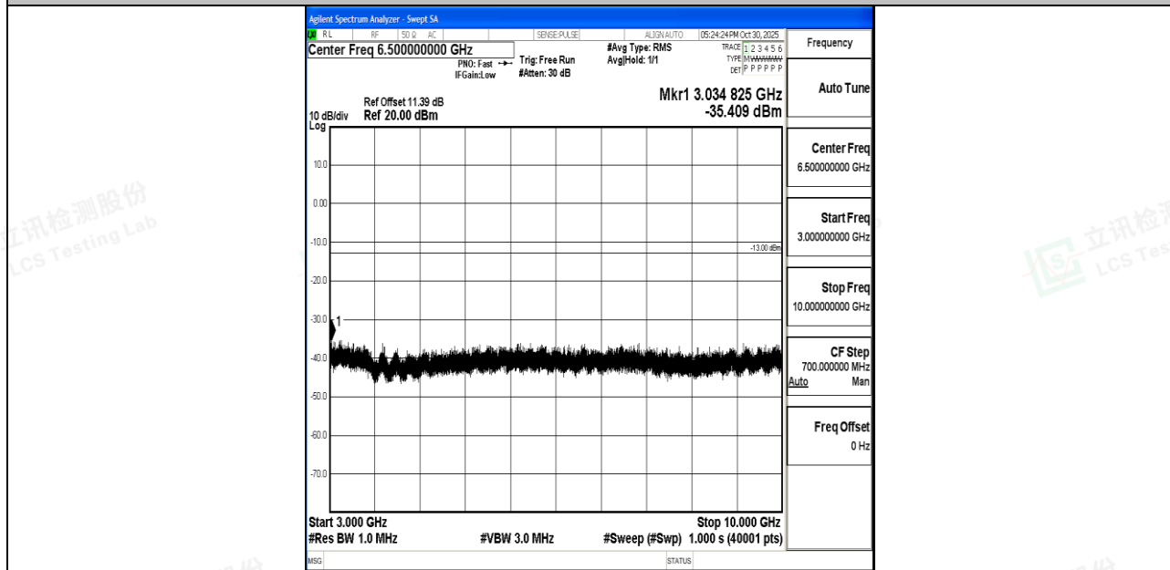
Band26_15MHz_16QAM_26865_1RB#0_3000~10000_3000~10000
