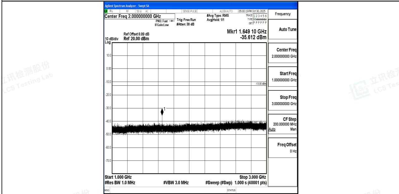
Band26_10MHz_QPSK_26840_1RB#0_1000~3000_1000~3000
