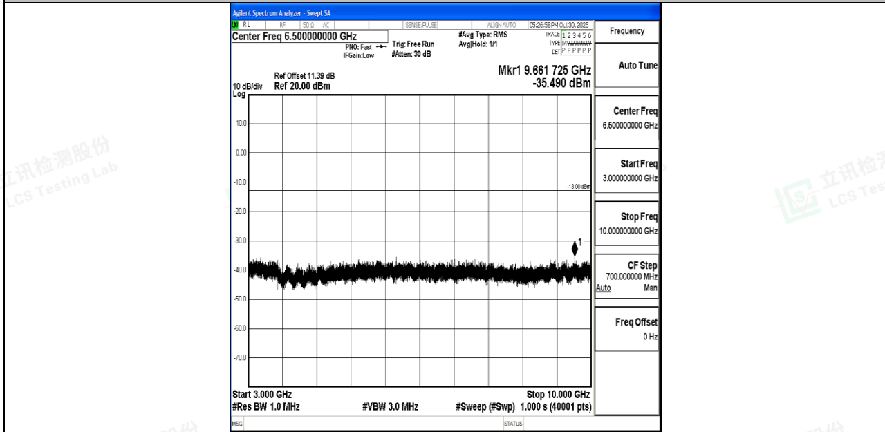
Band26_15MHz_16QAM_26965_1RB#0_3000~10000_3000~10000
