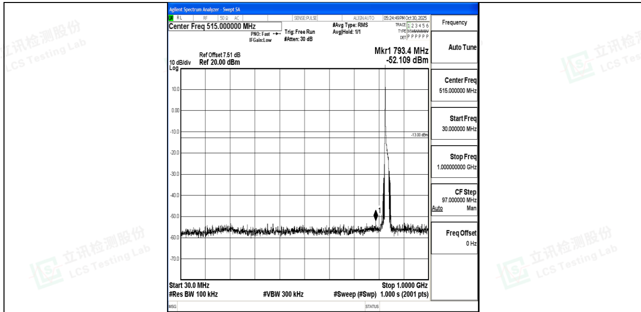
Band26_15MHz_QPSK_26915_1RB#0_30~1000_30~1000
