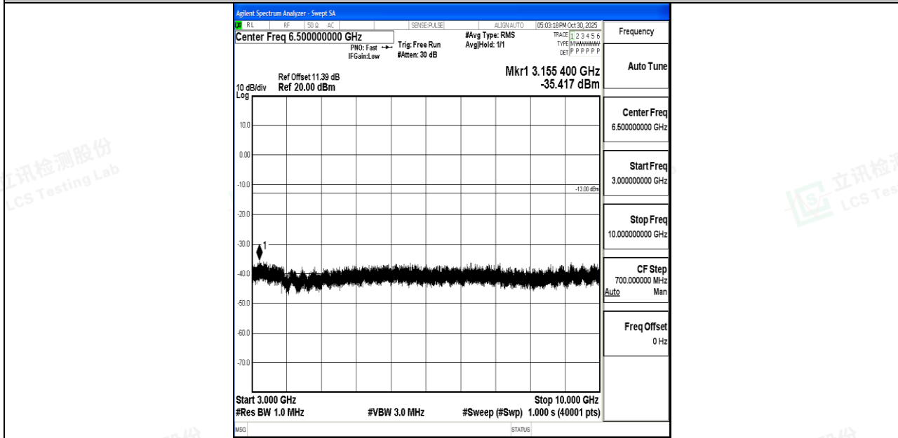
Band26_10MHz_16QAM_26990_1RB#0_3000~10000_3000~10000
