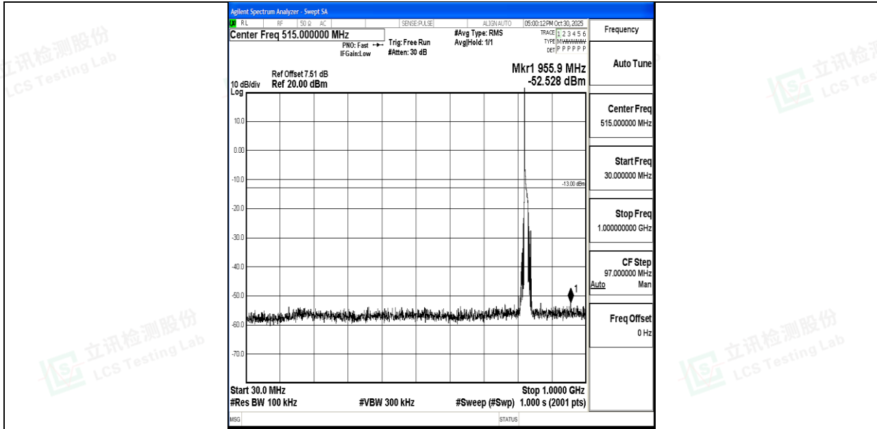
Band26_10MHz_QPSK_26840_1RB#0_30~1000_30~1000
