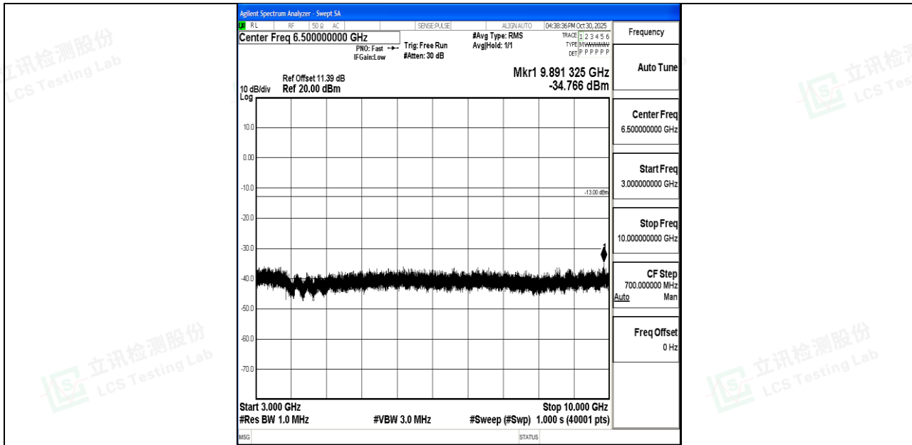
Band26_5MHz_QPSK_27015_1RB#0_3000~10000_3000~10000
