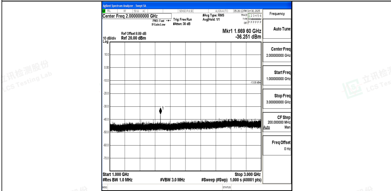
Band26_15MHz_QPSK_26965_1RB#0_1000~3000_1000~3000
