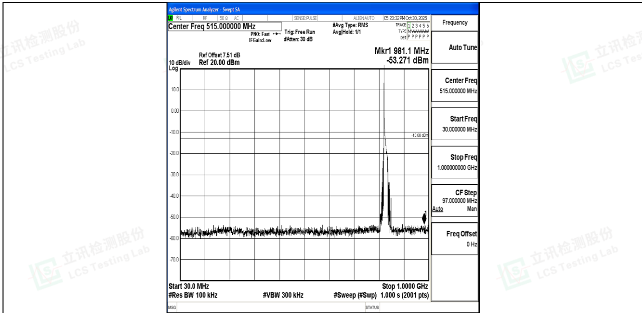
Band26_15MHz_QPSK_26865_1RB#0_30~1000_30~1000
