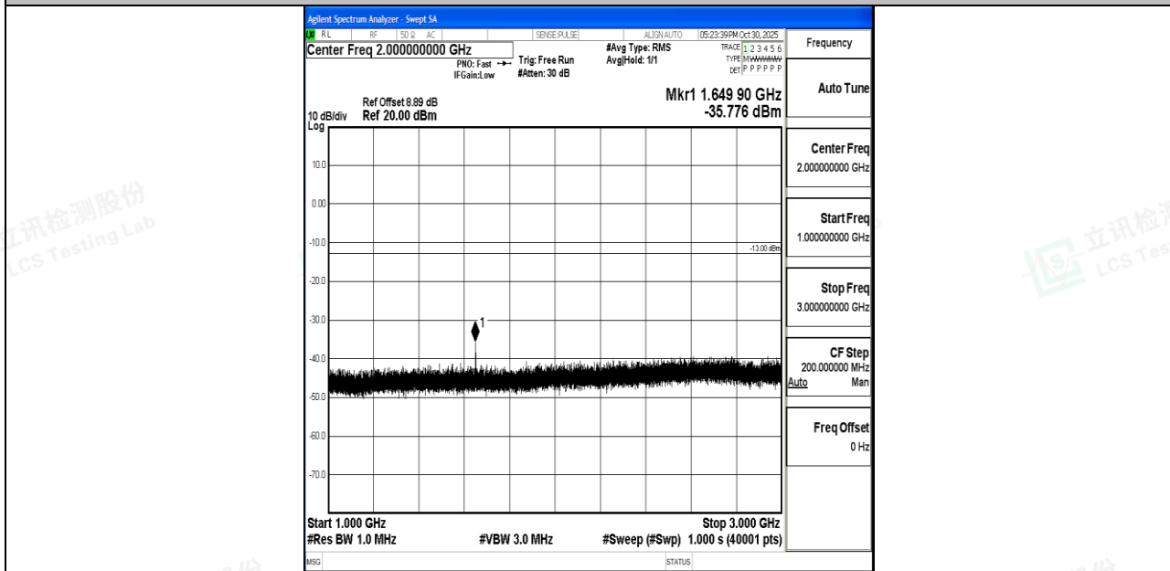
Band26_15MHz_QPSK_26865_1RB#0_1000~3000_1000~3000
