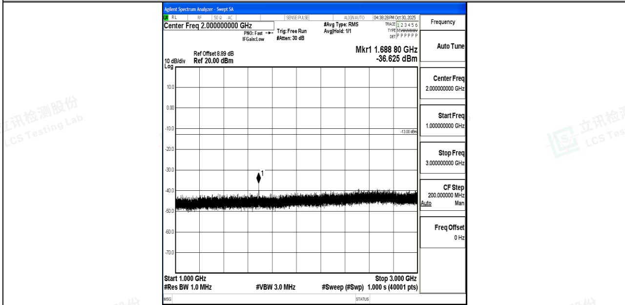
Band26_5MHz_QPSK_27015_1RB#0_1000~3000_1000~3000
