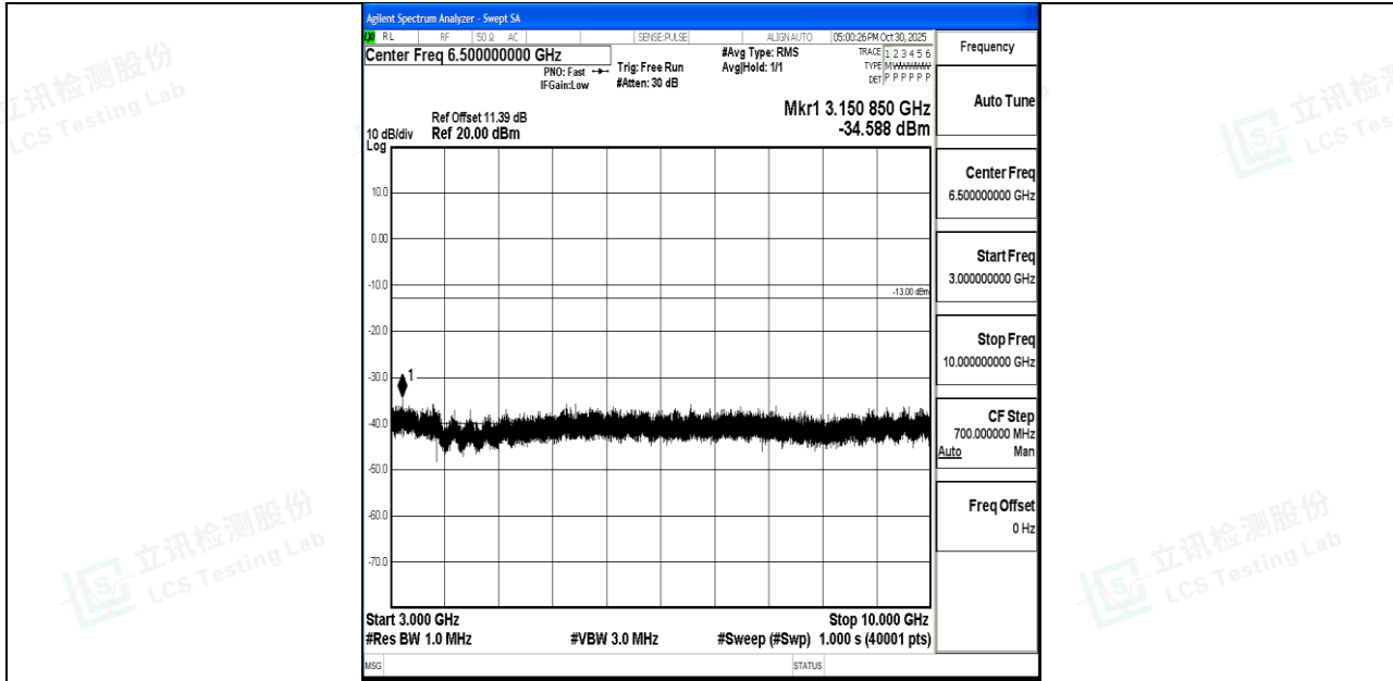
Band26_10MHz_QPSK_26840_1RB#0_3000~10000_3000~10000
