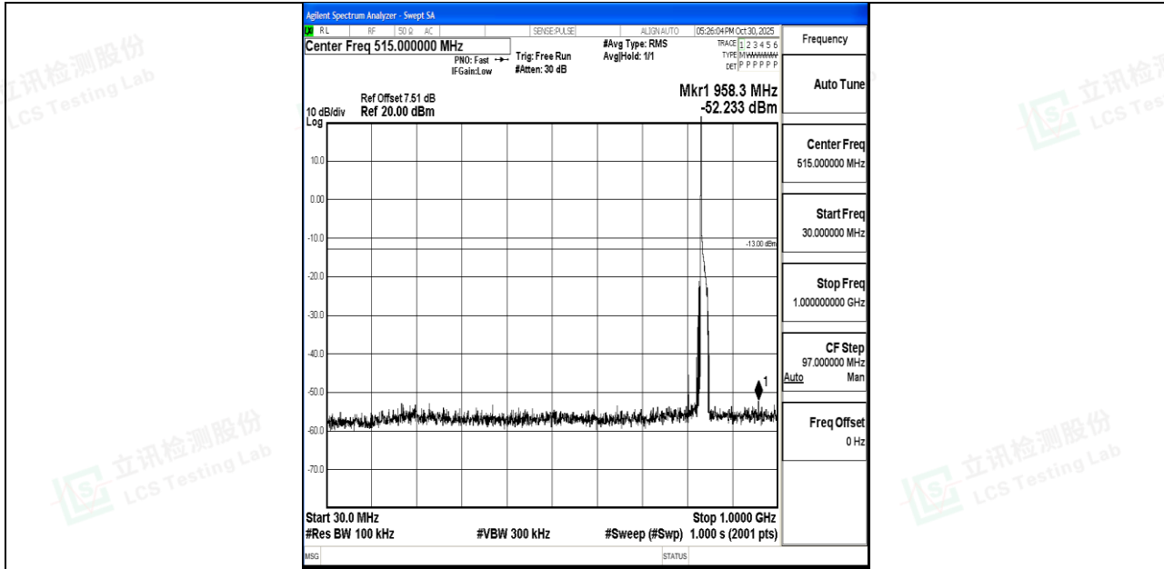
Band26_15MHz_QPSK_26965_1RB#0_30~1000_30~1000
