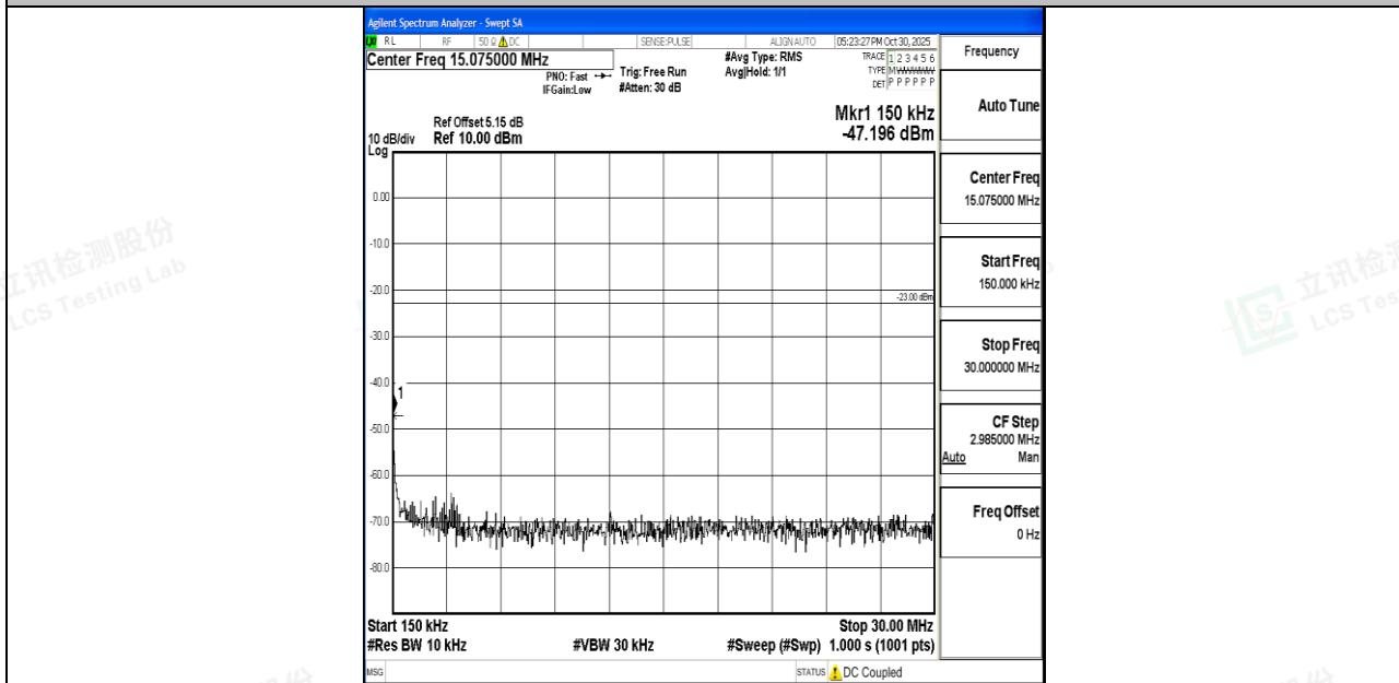
Band26_15MHz_QPSK_26865_1RB#0_0.15~30_0.15~30
