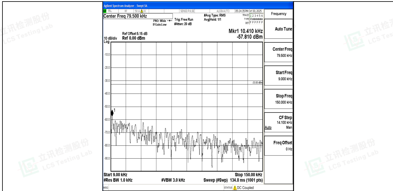
Band26_15MHz_QPSK_26915_1RB#0_0.009~0.15_0.009~0.15
