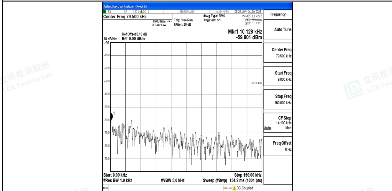
Band26_15MHz_16QAM_26915_1RB#0_0.009~0.15_0.009~0.15
