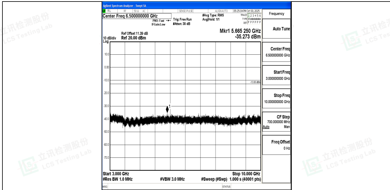
Band26_15MHz_QPSK_26915_1RB#0_3000~10000_3000~10000
