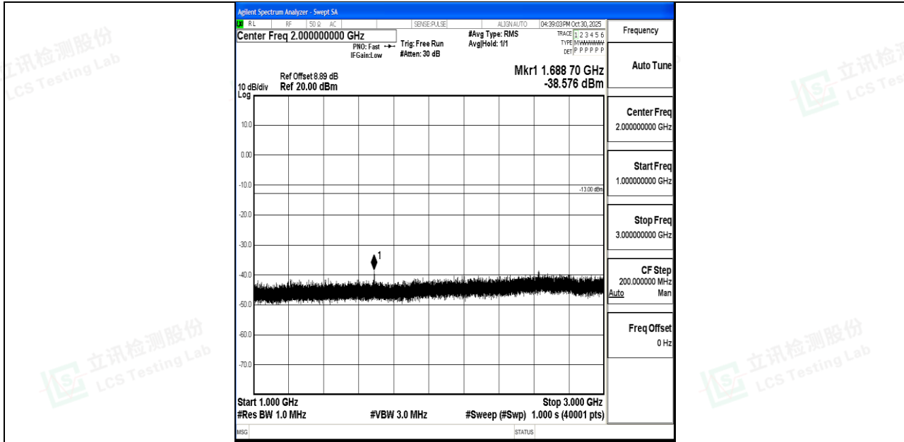
Band26_5MHz_16QAM_27015_1RB#0_1000~3000_1000~3000
