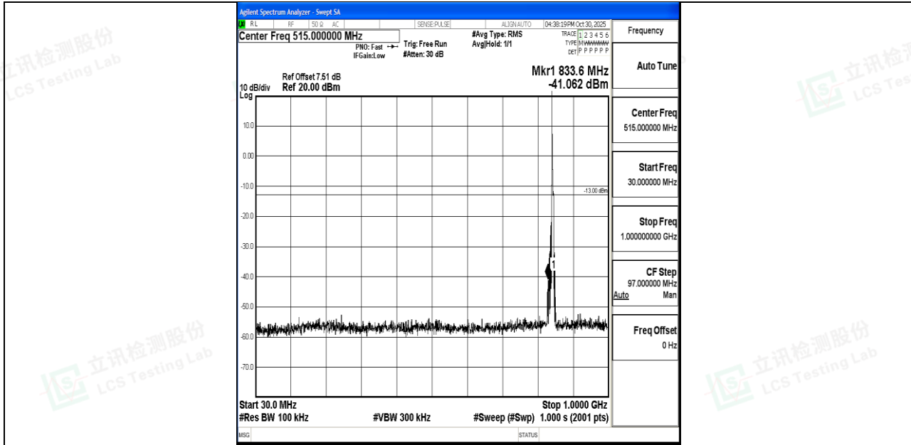
Band26_5MHz_QPSK_27015_1RB#0_30~1000_30~1000
