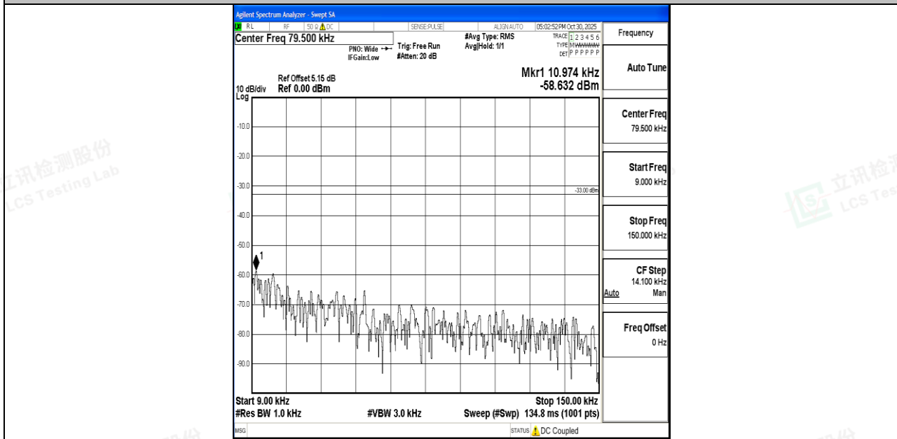
Band26_10MHz_16QAM_26990_1RB#0_0.009~0.15_0.009~0.15
