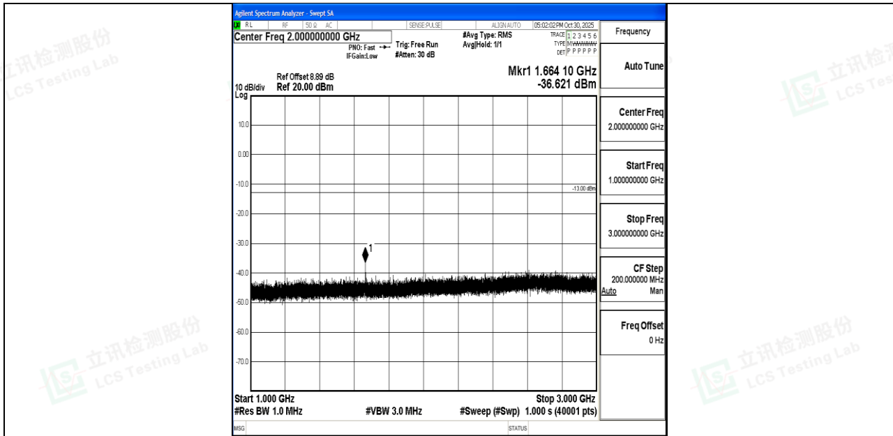
Band26_10MHz_16QAM_26915_1RB#0_1000~3000_1000~3000
