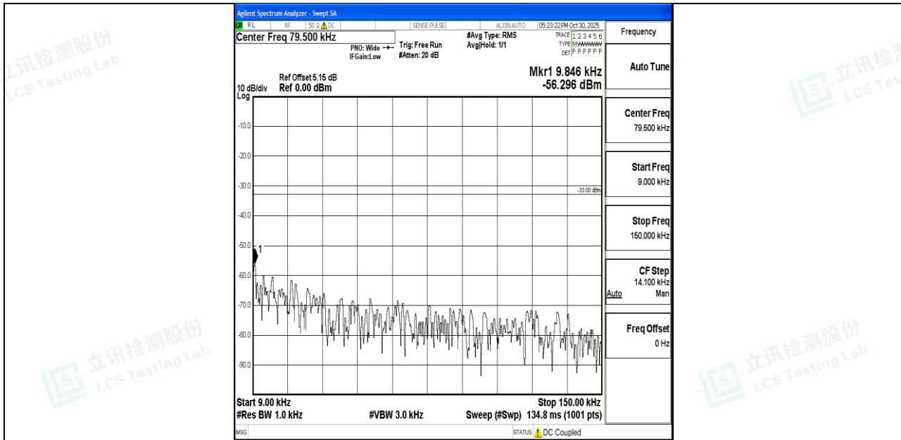
Band26_15MHz_QPSK_26865_1RB#0_0.009~0.15_0.009~0.15
