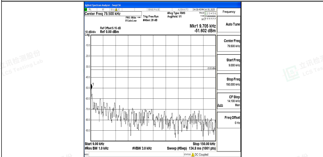
Band26_5MHz_16QAM_27015_1RB#0_0.009~0.15_0.009~0.15
