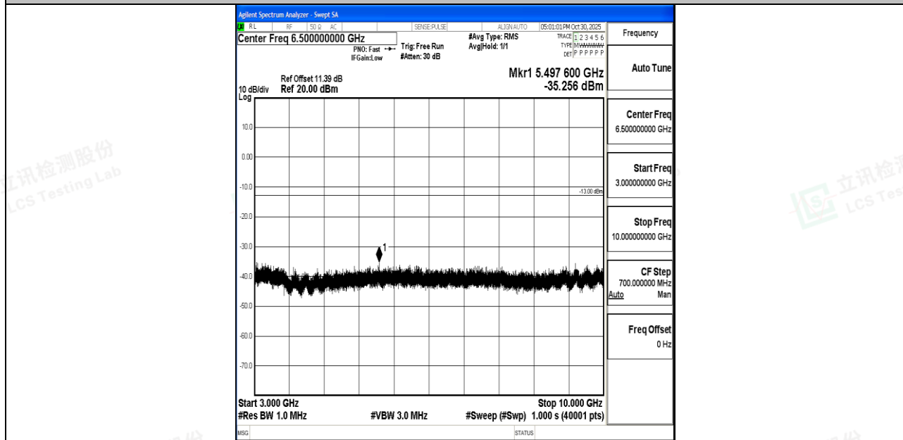
Band26_10MHz_16QAM_26840_1RB#0_3000~10000_3000~10000
