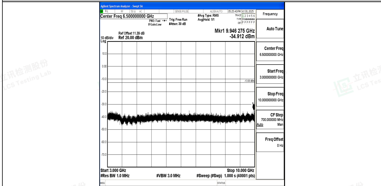
Band26_15MHz_16QAM_26915_1RB#0_3000~10000_3000~10000
