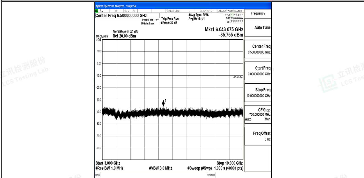
Band26_10MHz_16QAM_26915_1RB#0_3000~10000_3000~10000
