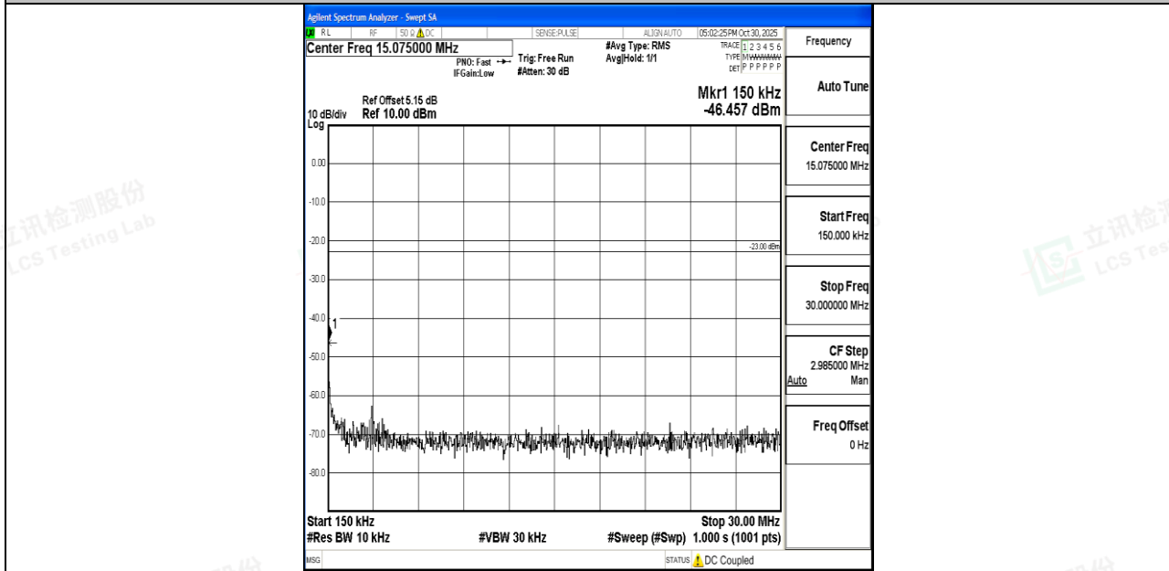
Band26_10MHz_QPSK_26990_1RB#0_0.15~30_0.15~30
