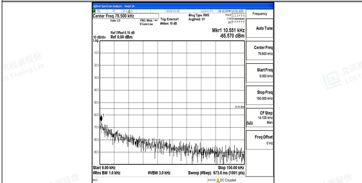
Band38_20MHz_16QAM_37850_1RB#0_0.009~0.15_0.009~0.15
