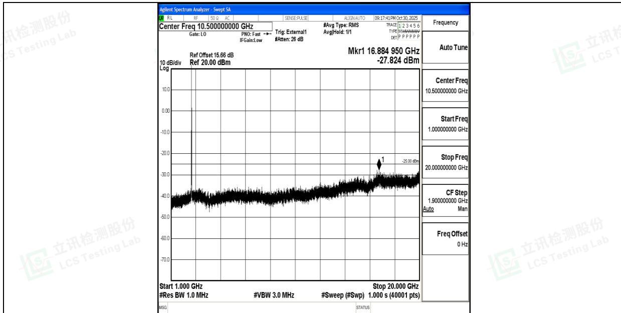
Band38_20MHz_16QAM_37850_1RB#0_1000~20000_1000~20000
