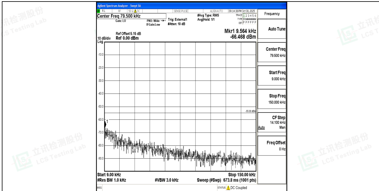
Band38_20MHz_QPSK_37850_1RB#0_0.009~0.15_0.009~0.15
