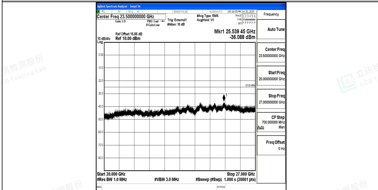
Band38_20MHz_16QAM_37850_1RB#0_20000~27000_20000~27000
