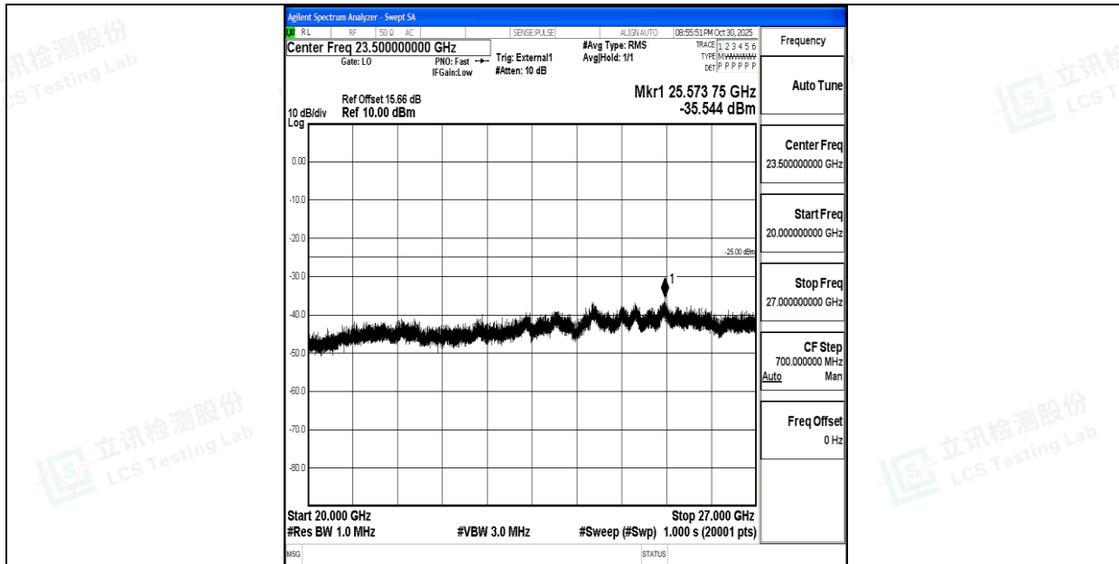
Band38_15MHz_QPSK_38175_1RB#0_20000~27000_20000~27000
