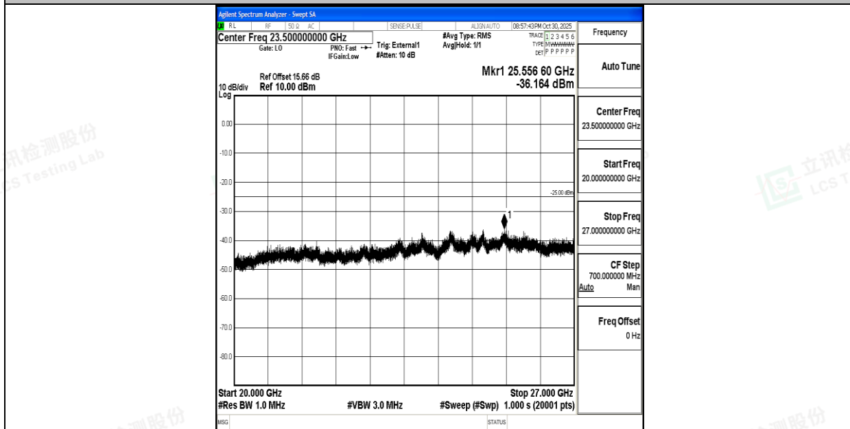
Band38_15MHz_16QAM_38175_1RB#0_20000~27000_20000~27000
