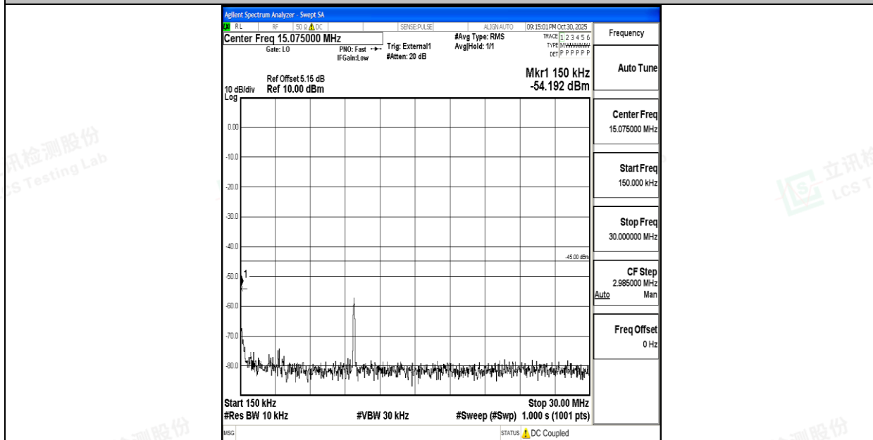
Band38_20MHz_QPSK_37850_1RB#0_0.15~30_0.15~30
