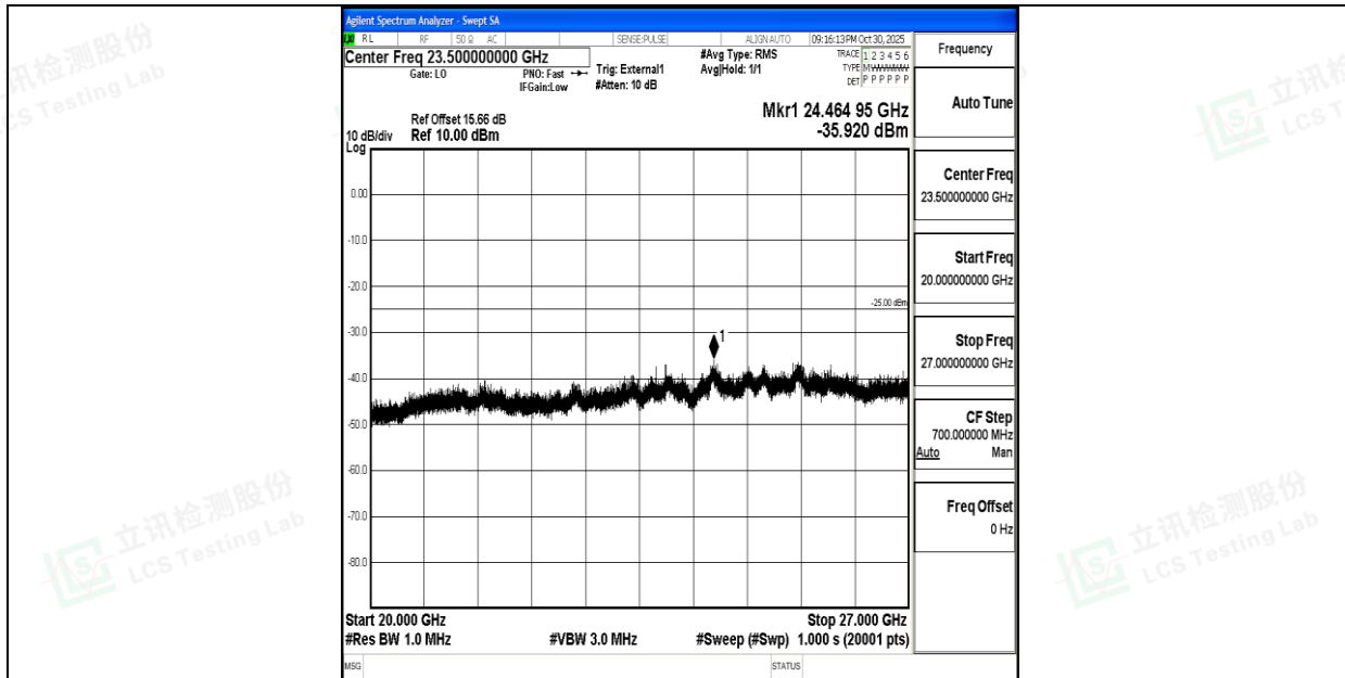
Band38_20MHz_QPSK_37850_1RB#0_20000~27000_20000~27000
