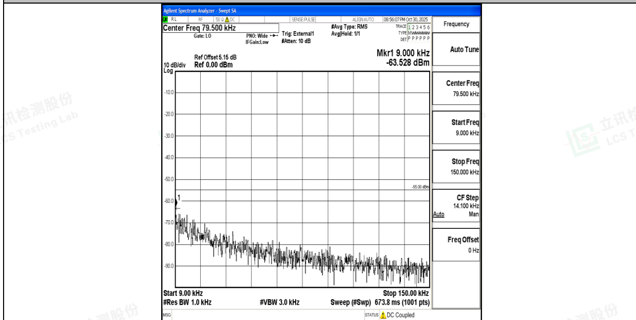
Band38_15MHz_16QAM_38175_1RB#0_0.009~0.15_0.009~0.15
