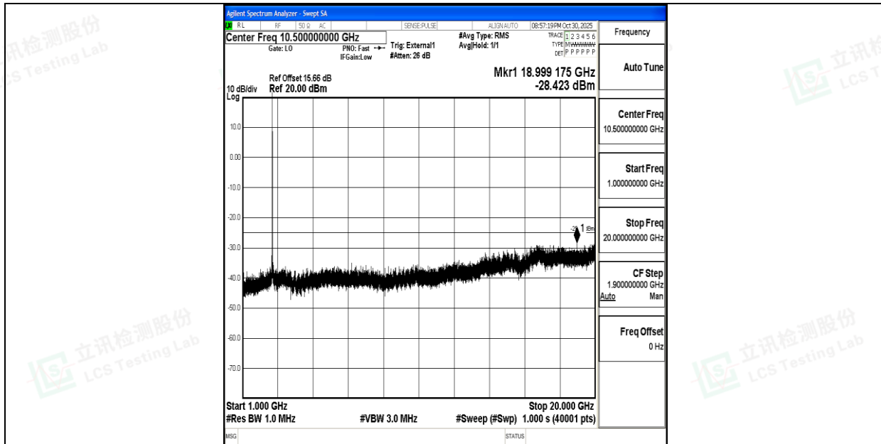
Band38_15MHz_16QAM_38175_1RB#0_1000~20000_1000~20000
