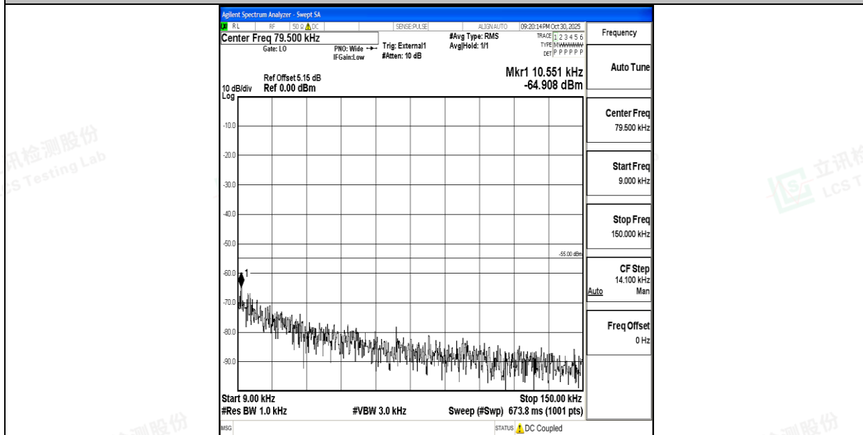
Band38_20MHz_16QAM_38000_1RB#0_0.009~0.15_0.009~0.15
