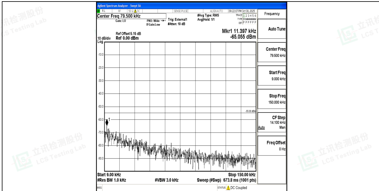
Band38_20MHz_QPSK_38150_1RB#0_0.009~0.15_0.009~0.15
