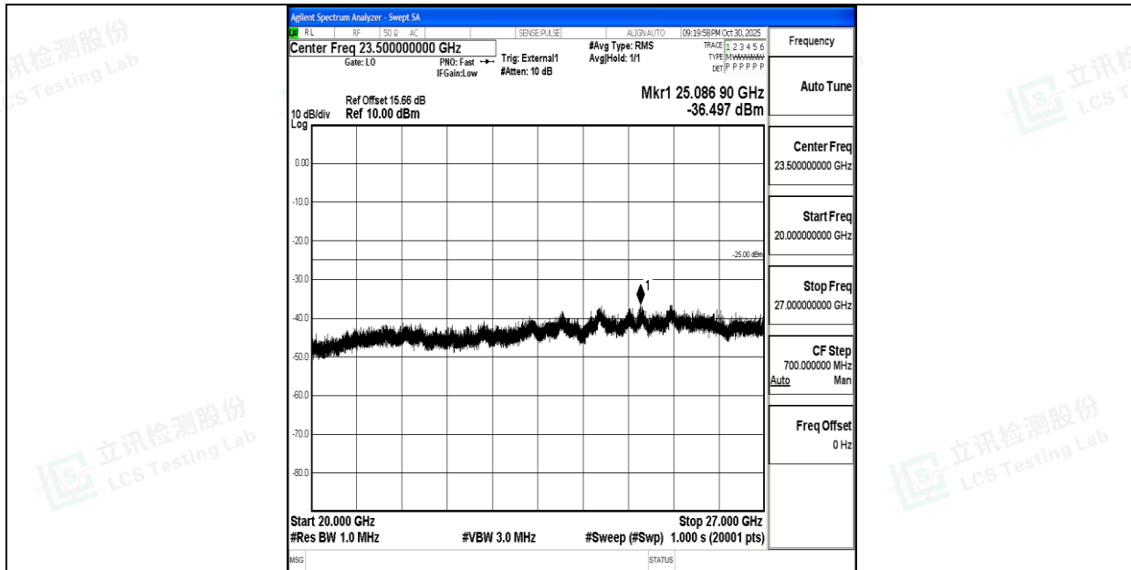
Band38_20MHz_QPSK_38000_1RB#0_20000~27000_20000~27000
