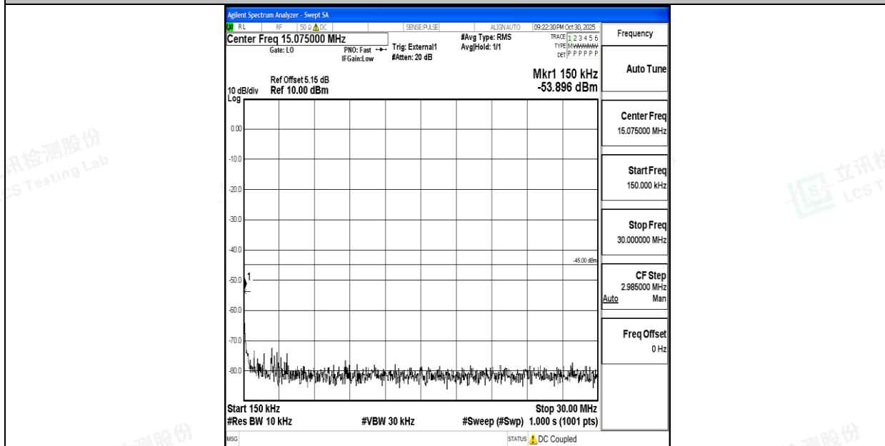
Band38_20MHz_QPSK_38150_1RB#0_0.15~30_0.15~30
