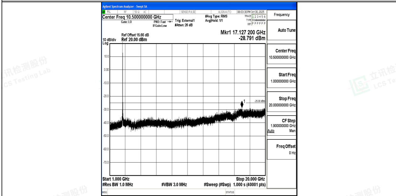
Band41_20MHz_QPSK_40620_1RB#0_1000~20000_1000~20000
