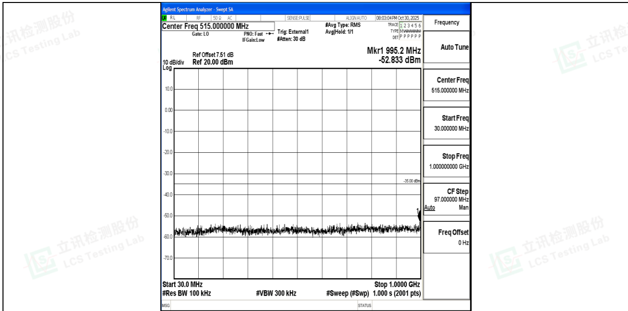
Band41_20MHz_QPSK_40620_1RB#0_30~1000_30~1000
