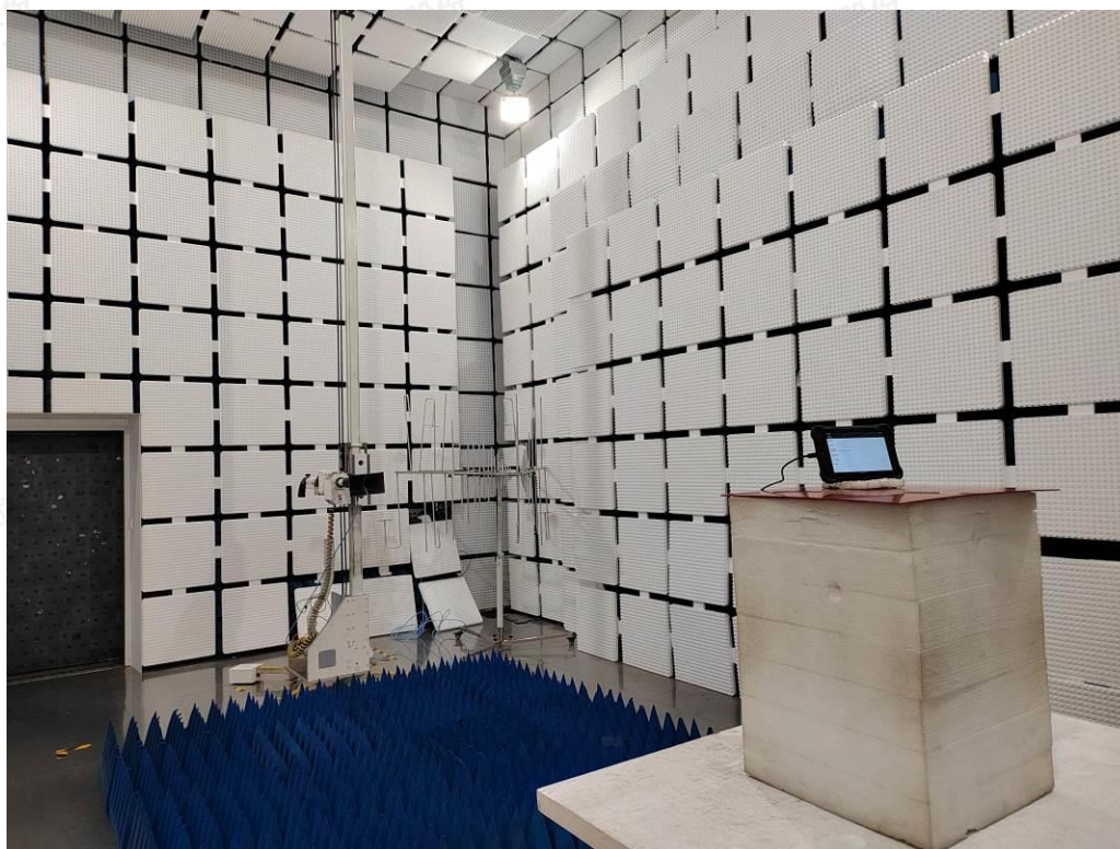
Fig. 3 Test Setup Photo(s) of Conducted Emissions Measurement
