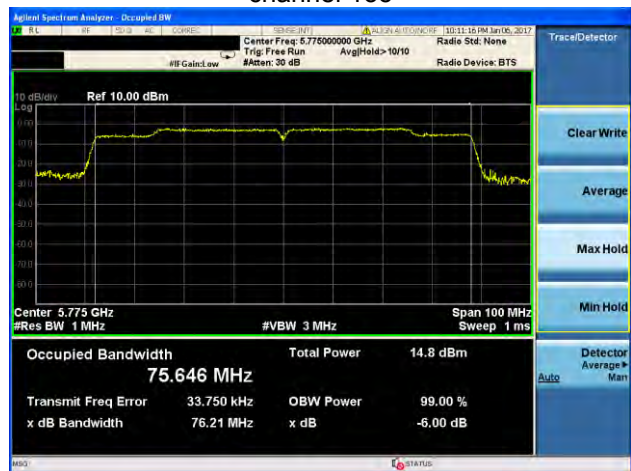
(802.11ac80) -6dB Bandwidth plot on channel 155
