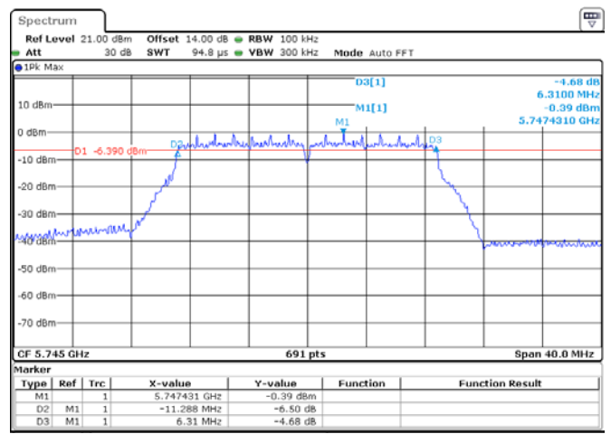
ANT 2(802.11N20)
