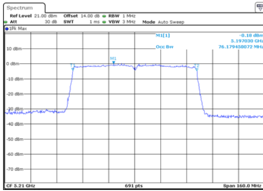
ANT 1(11AC80)
