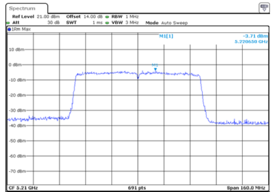
ANT 2(11AC80)
