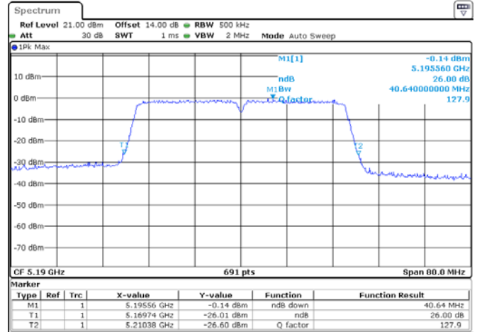
ANT 2(802.11n40)
