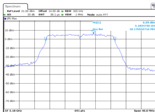
ANT 2(11N20)
