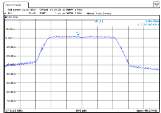
ANT 2(11N20)
