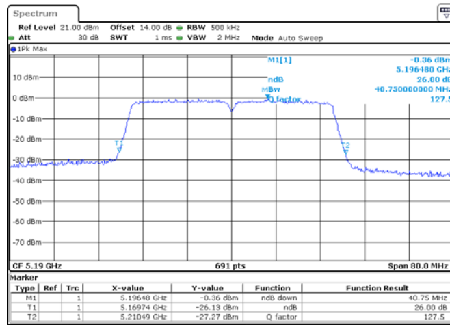
ANT 2(802.11ac40)
