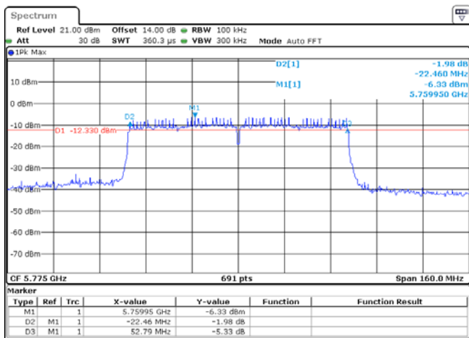
ANT 1(802.11ac80)
