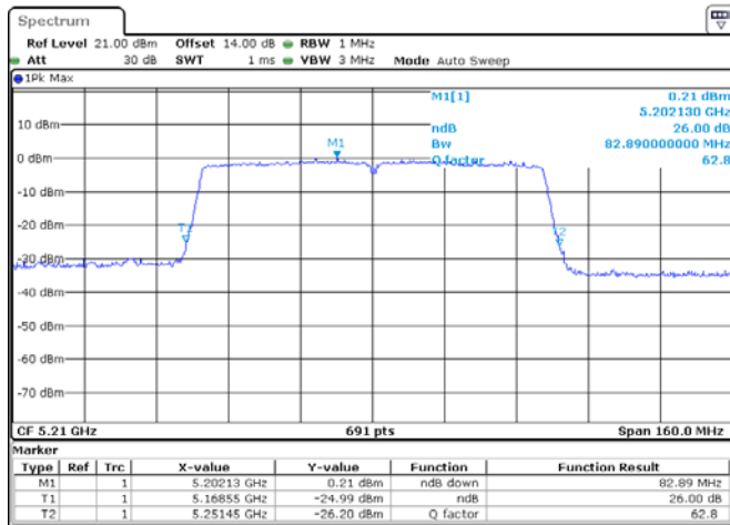
ANT 1(802.11ac80)
