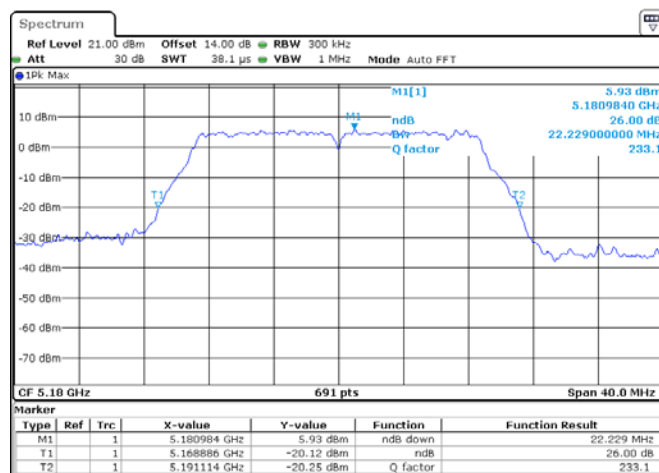
ANT 2(11N20)
