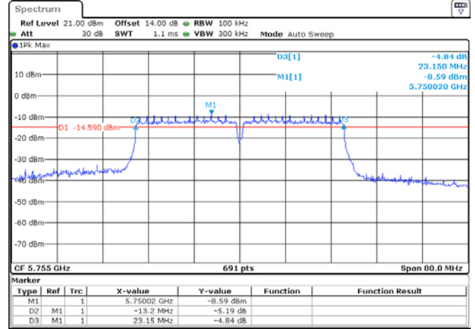
ANT 2(802.11N40)
