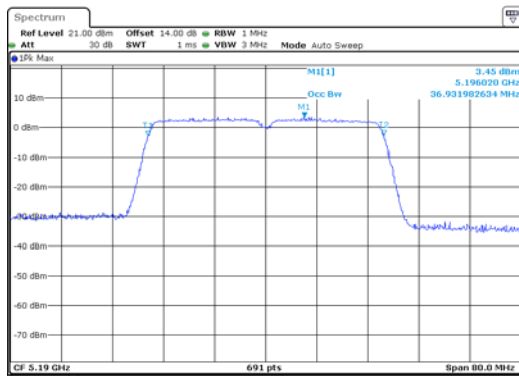
ANT 1(11AC40)
