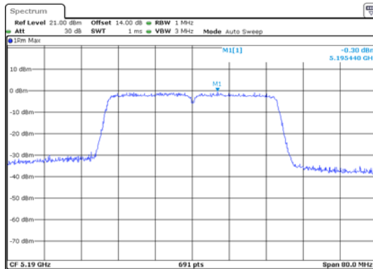
ANT 2(11N40)
