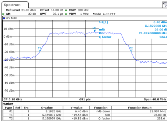
ANT 1(802.11ac20)
