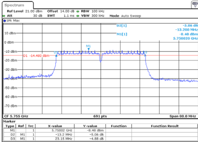
ANT 1(802.11ac40)
