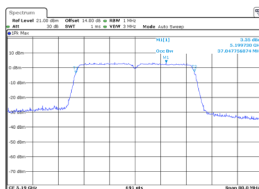
ANT 2(11N40)
