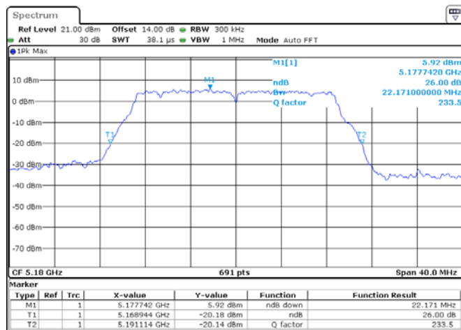
ANT 1(11N20)
