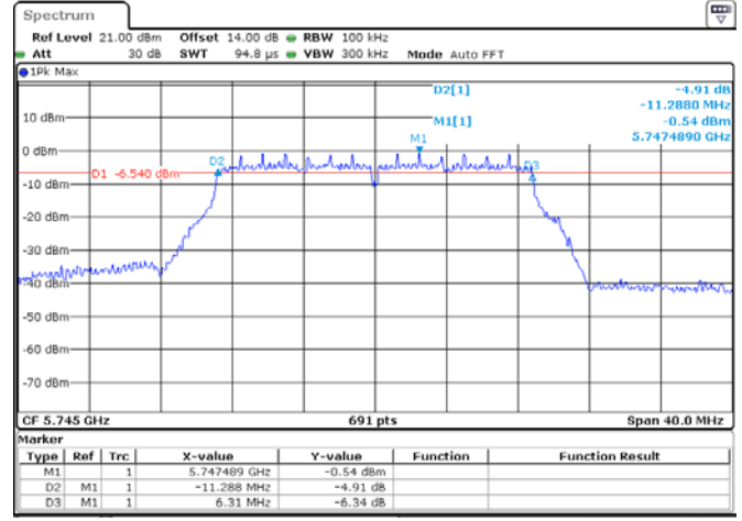
ANT 2(802.11ac20)
