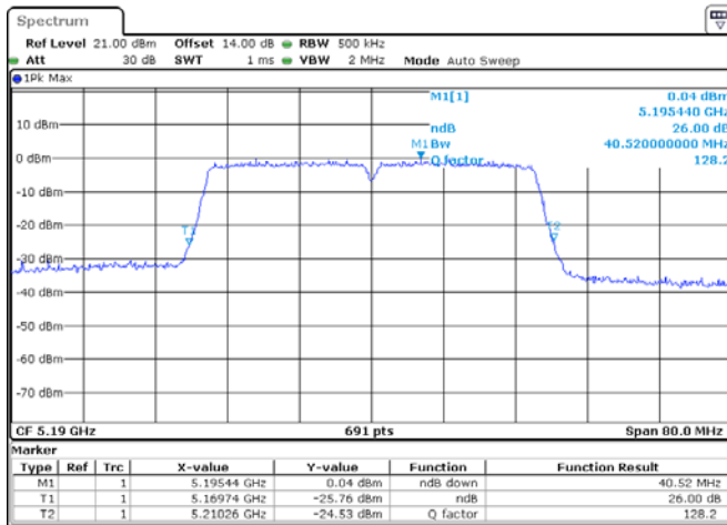
ANT 1(802.11n40)
