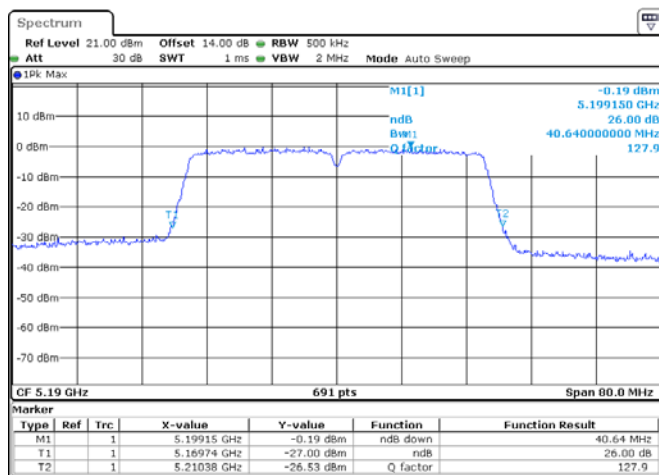
ANT 1(802.11ac40)
