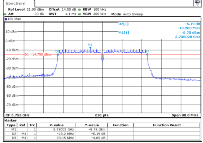
ANT 2(802.11ac40)
