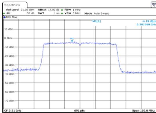
ANT 1(11AC80)
