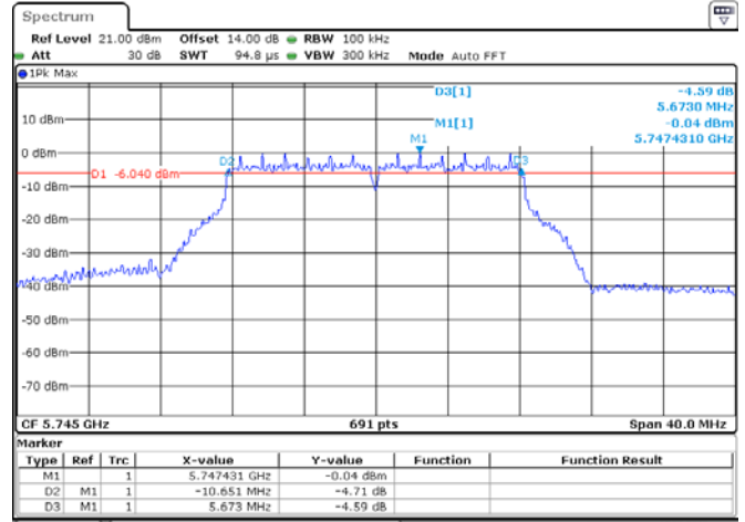
ANT 2(802.11A)
