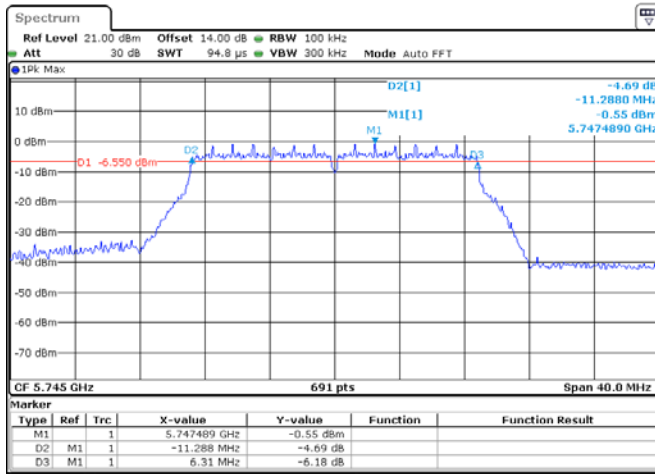
ANT 1(802.11ac20)
