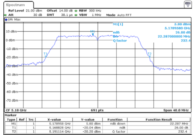
ANT 2(802.11ac20)
