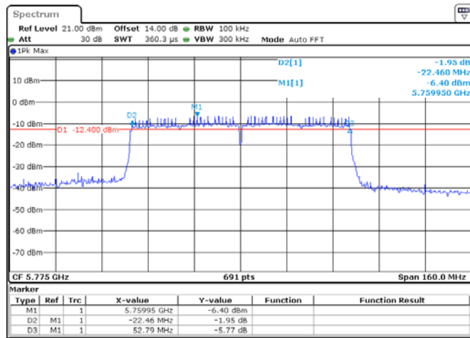
ANT 2(802.11ac80)
