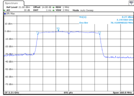
ANT 2(11AC80)
