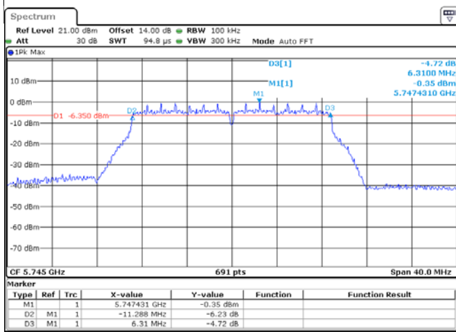
ANT 1(802.11N20)
