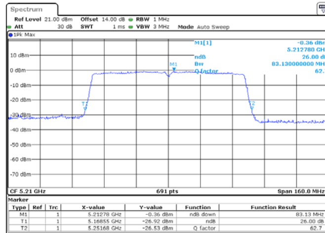
ANT 2(802.11ac80)
