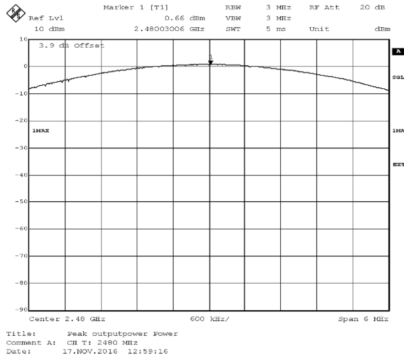
Setup S01_AD01, BT + WLAN module
