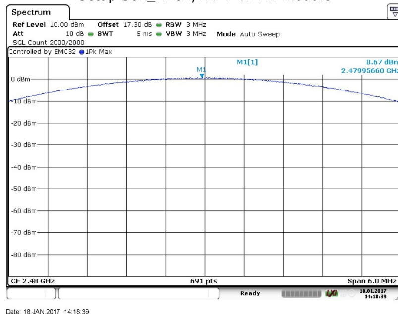
Setup S01_A001, BT + WLAN module
