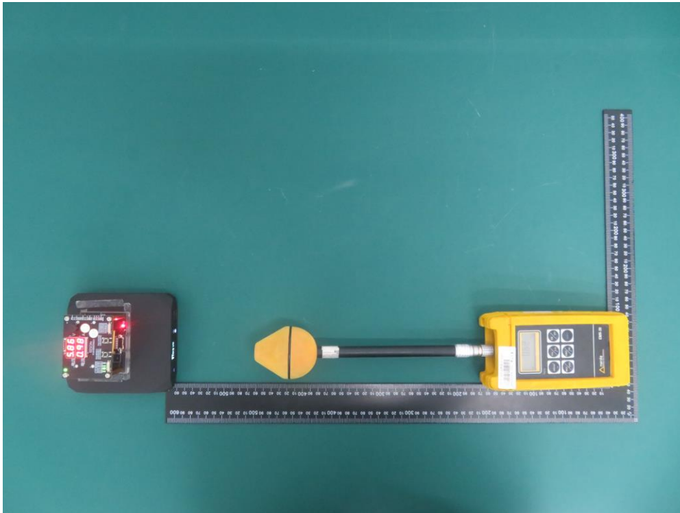
Description: RF Exposure Setup (15cm)
