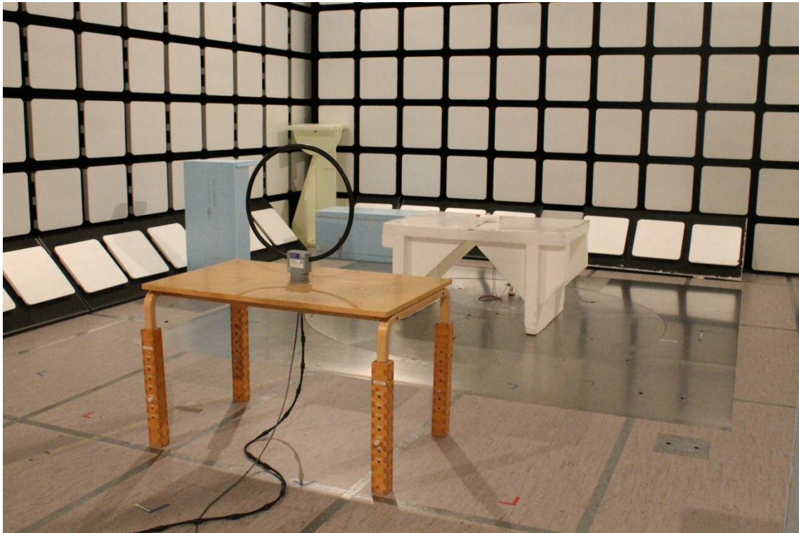
Photograph 1. Radiated Spurious Emissions 9 kHz – 30 MHz
