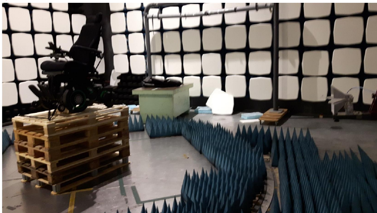
Test set up radiated emission > 1GHz
