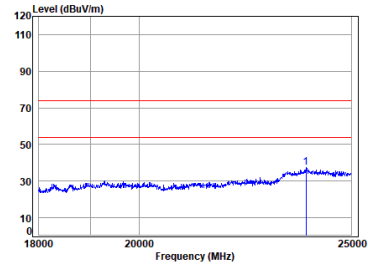
2.4G WIFI_TX_CH_M_Vertical
