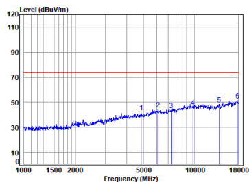
11g_TX_CH_06_Vertical-Peak
