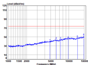
11g_TX_CH_06_Horizontal-Peak
