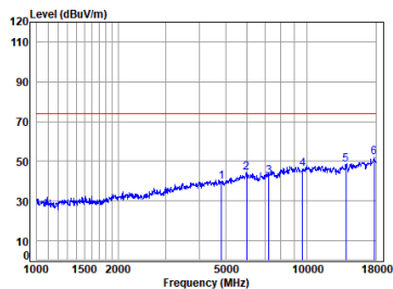
11g_TX_CH_01_Vertical-Peak
