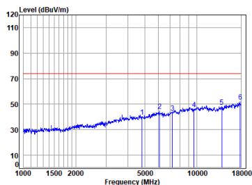
11g_TX_CH_01_Horizontal-Peak
