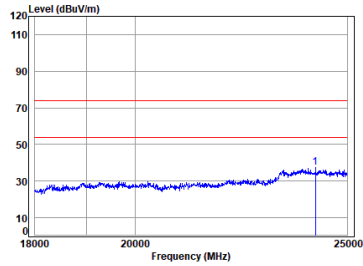
2.4G WIFI_TX_CH_M_Horizontal
