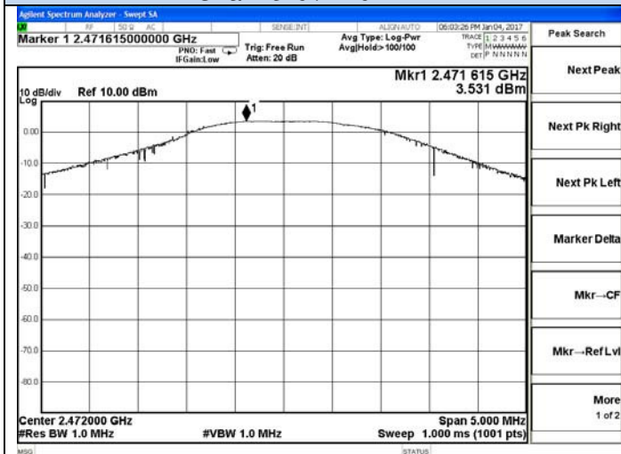
Channel 15/ 2472 MHz
