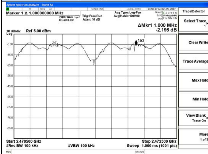
Channel 15 / 2472 MHz
