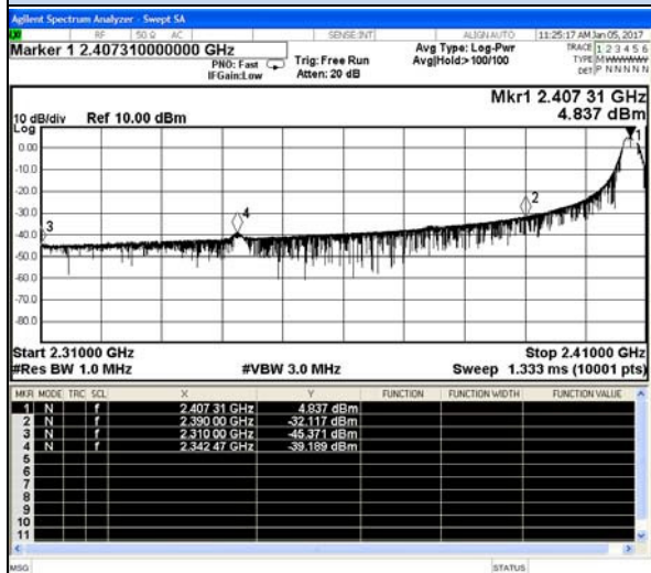
Channel 0 / 2407 MHz- Peak
