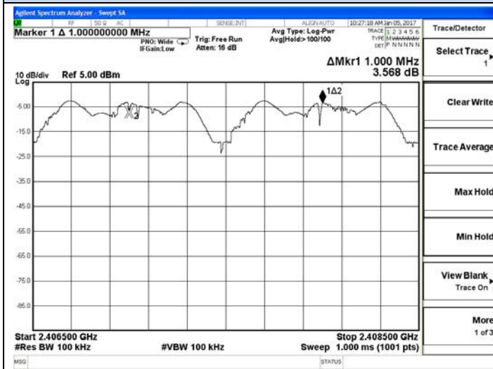
Channel 0 / 2407 MHz
