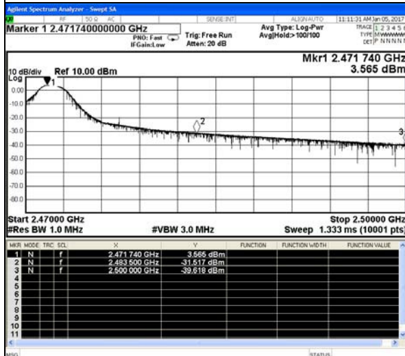
Channel 16 / 2472 MHz- Peak
