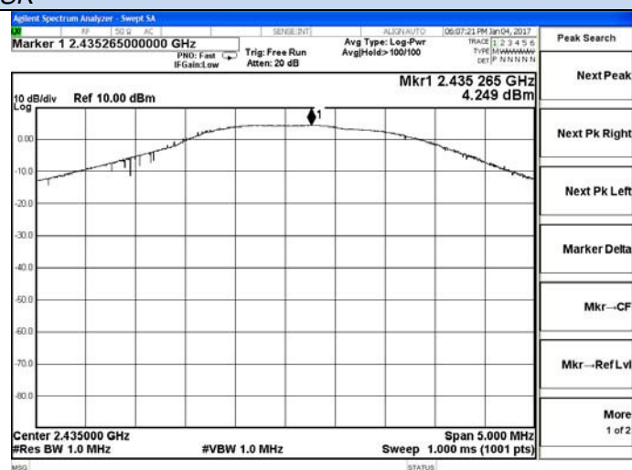
Channel 5 / 2435 MHz
