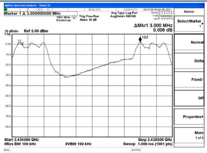
Channel 5 / 2435 MHz
