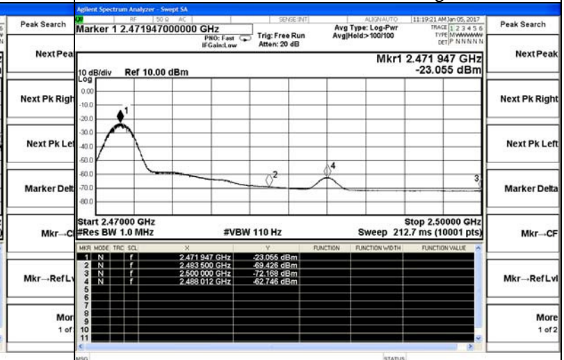
Channel 16 / 2472 MHz-Average
