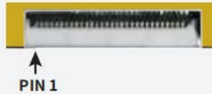
FPC connector (30Pin , Space between PINs 0.5mm)
