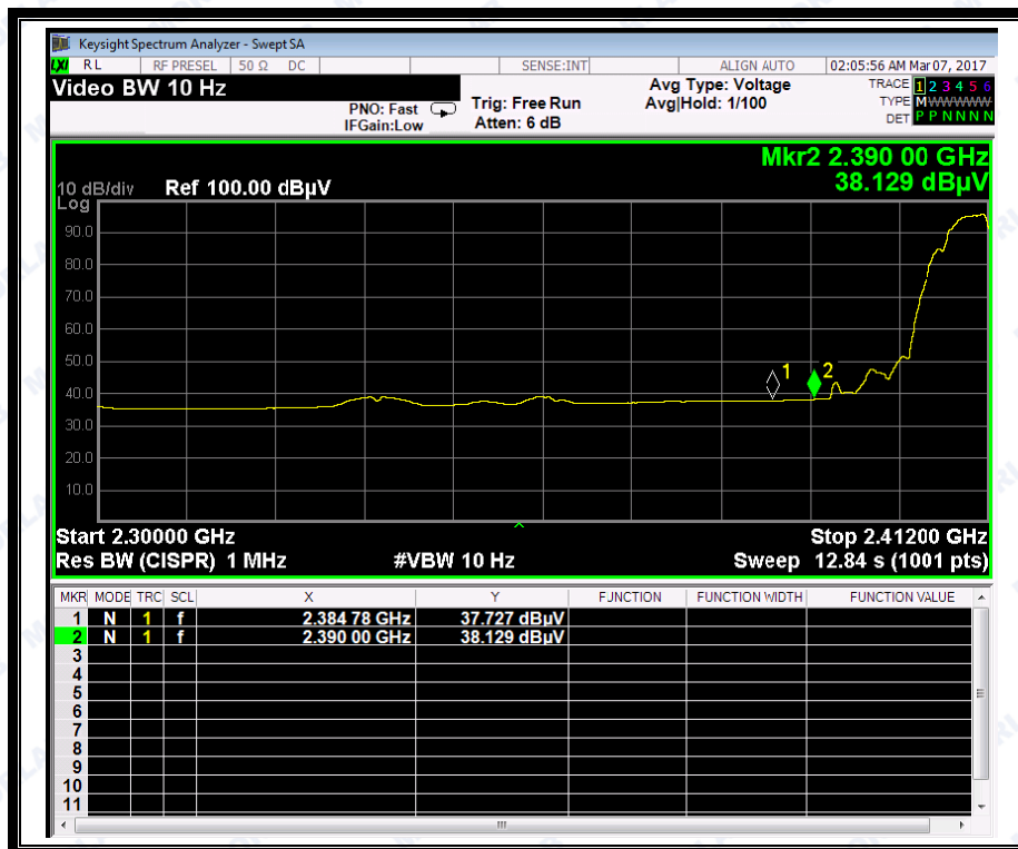
(Plot A2: Channel = 1 AVG @ 802.11b)
