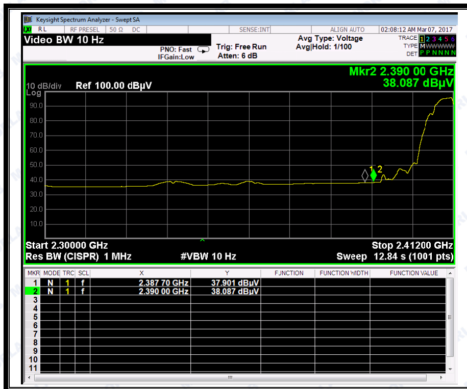
(Plot E2: Channel = 1 AVG @ 802.11n-20)
