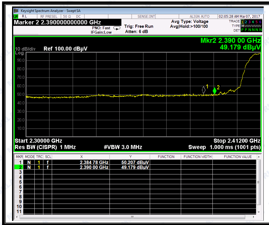
(Plot A1: Channel = 1 PEAK @ 802.11b)
