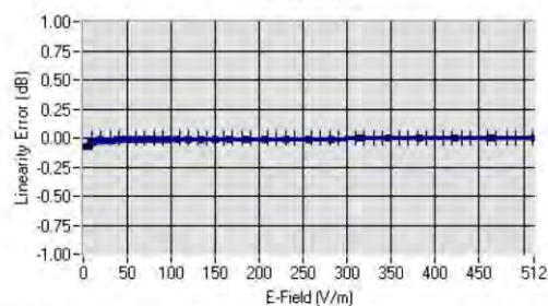
Linearity
