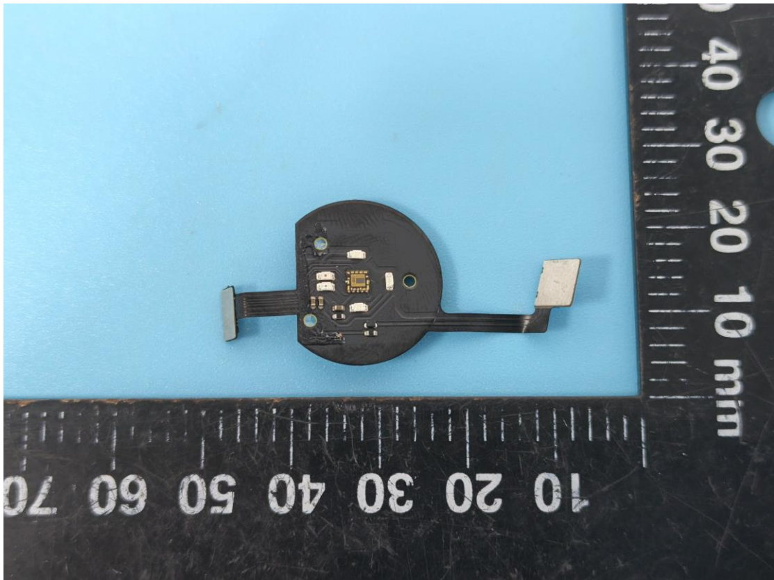
Bluetooth Antenna
