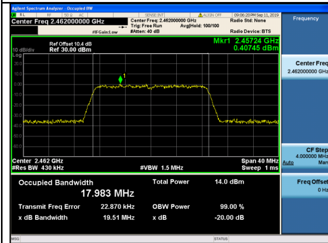
802.11n20 99% Bandwidth - High CH 2462
