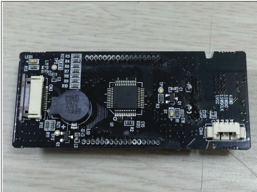
Bottom view of LCD PCB
