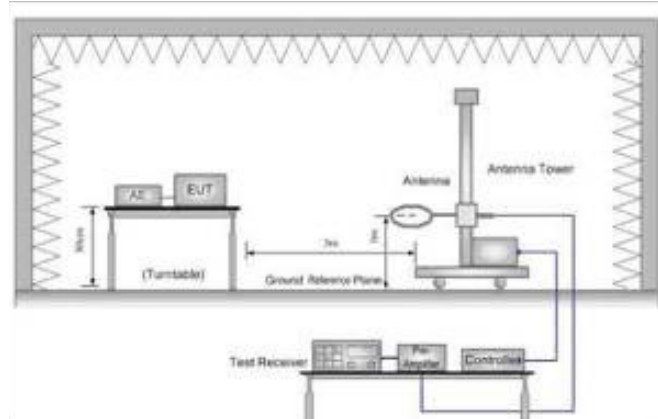
Figure 1. Below 30MHz
