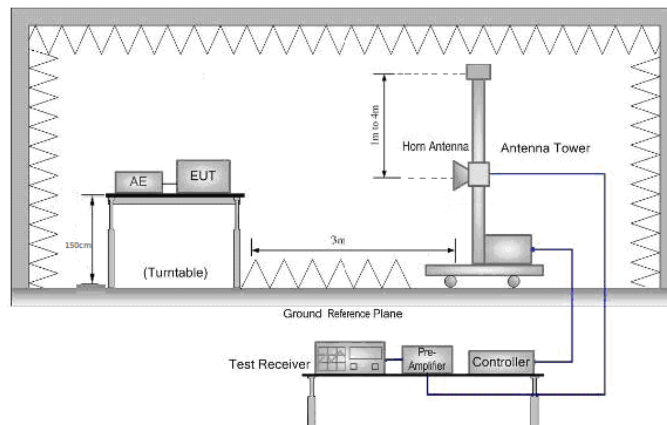
Figure 3. Above 1 GHz
