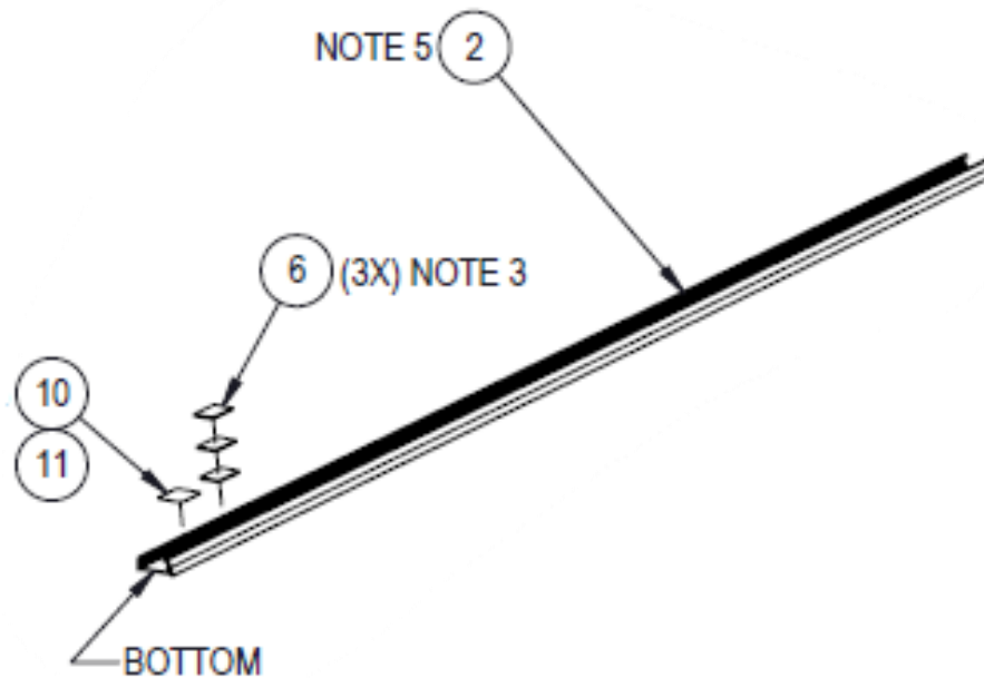
Figure 2. Placement of identification label (Item #10) on inside of 3600 FMD Archway's bottom channel of the AF3601 master and AF3601S slave rail assemblies.
