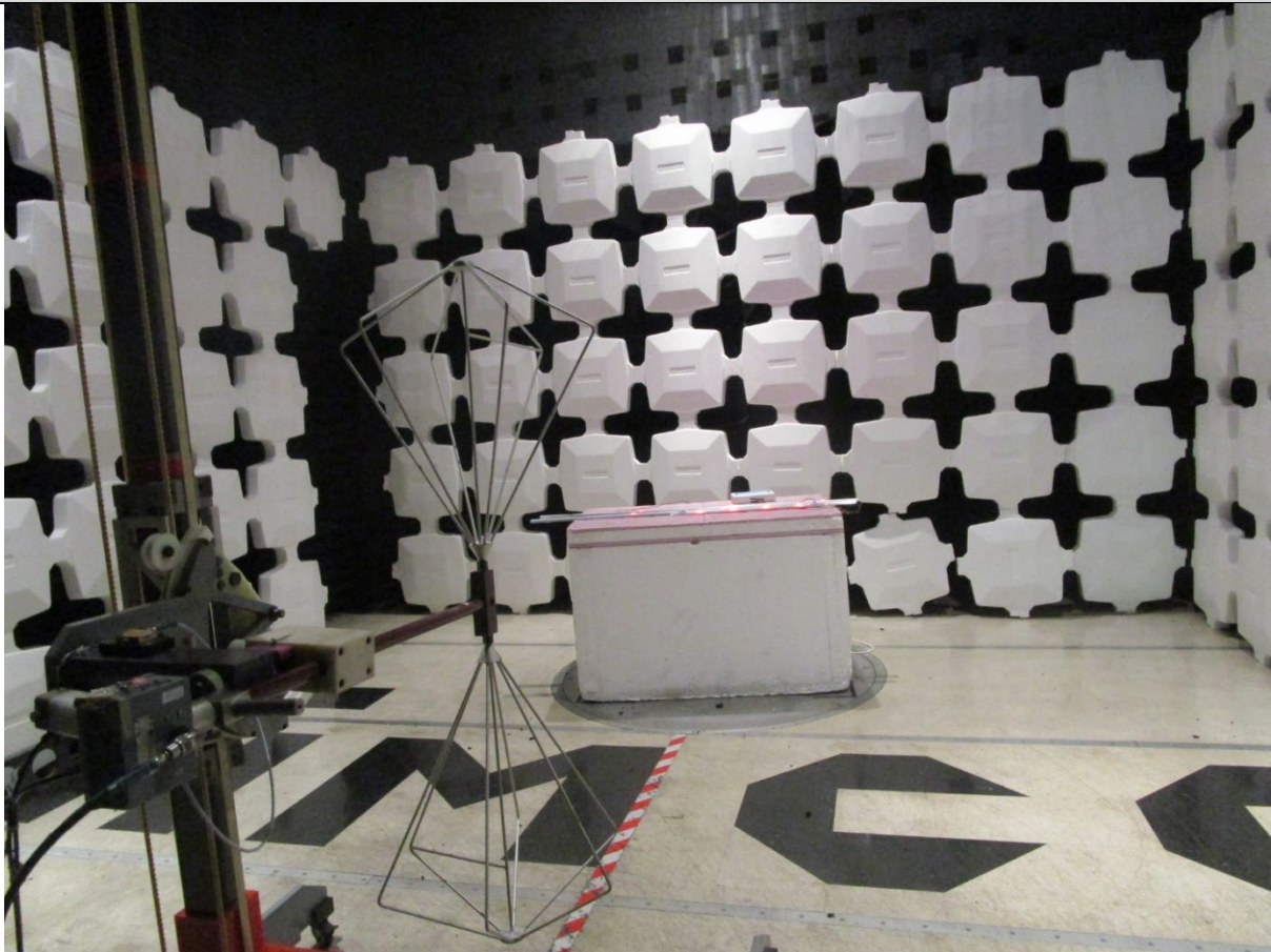
Radiated Testing, Below 1 GHz
