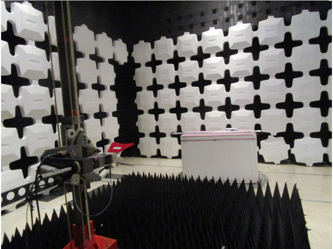
Radiated Testing, Above 1 GHz
