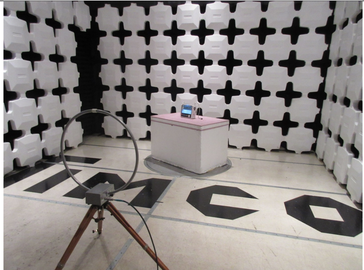
Radiated Emissions Below 30 MHz Setup
