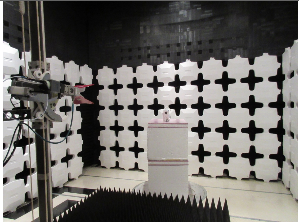
Radiated Emissions Above 1 GHz Setup
