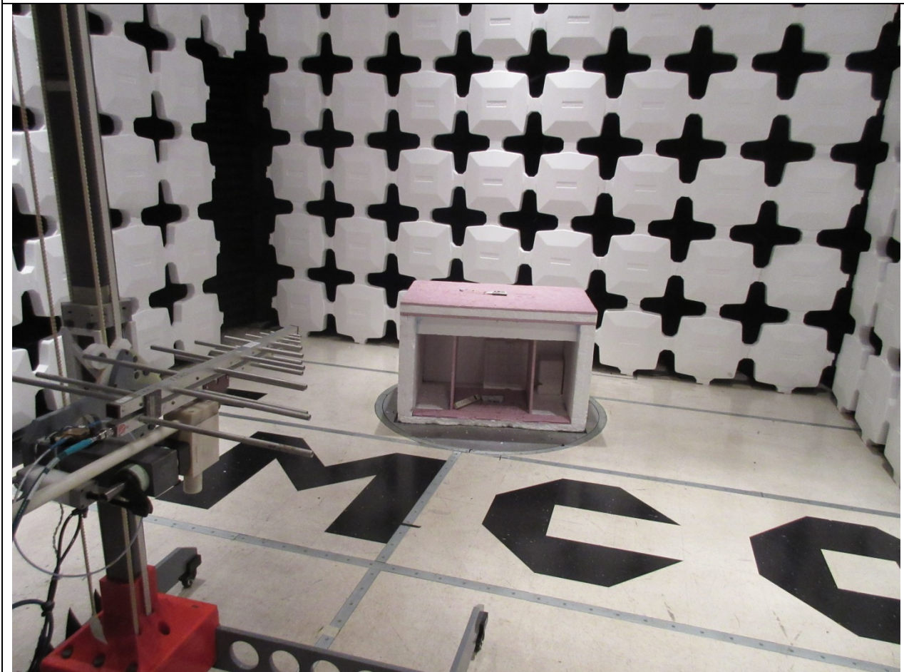
Radiated Emissions Below 1 GHz Setup
