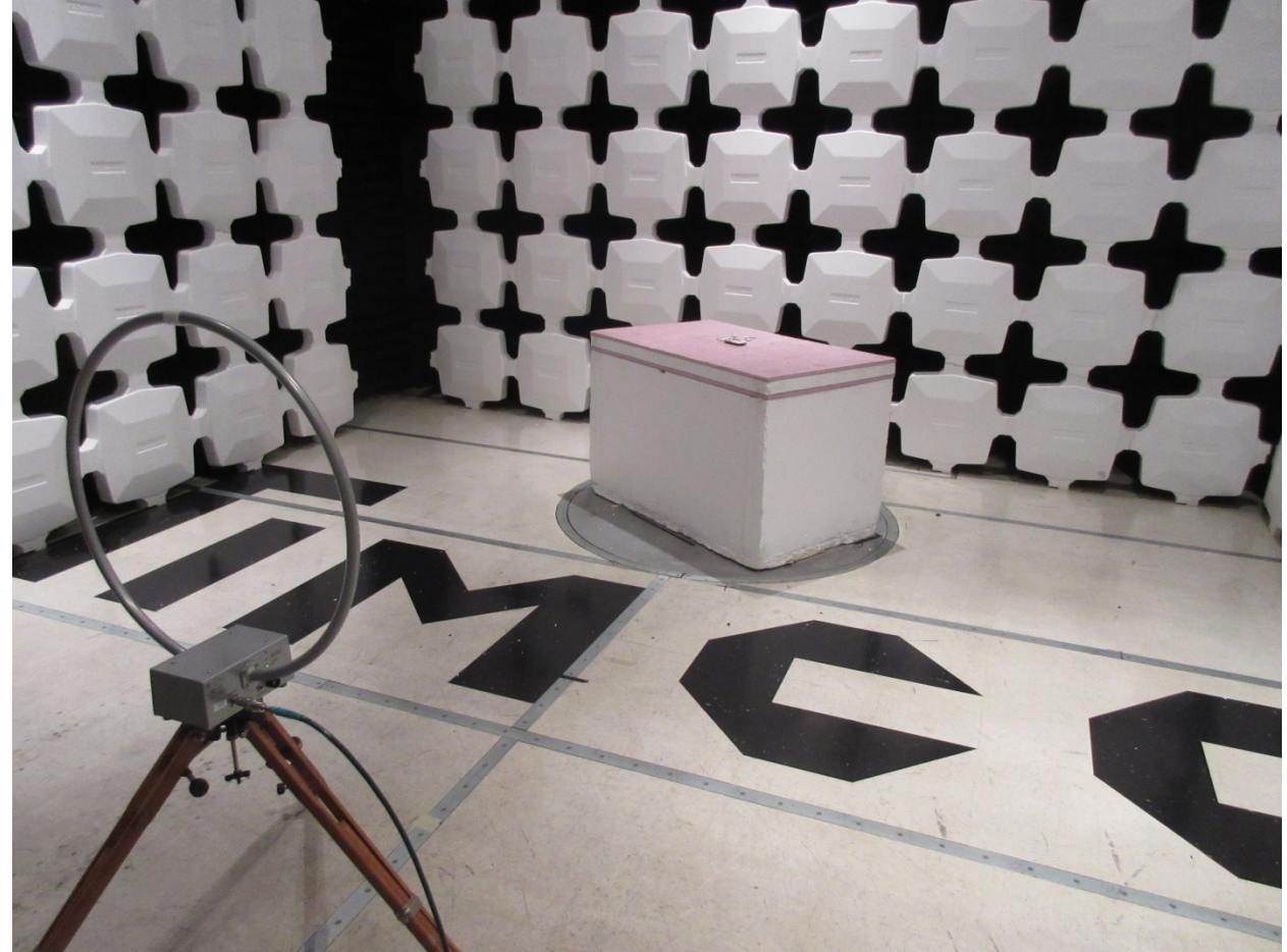
Radiated Emissions Below 30 MHz Setup
