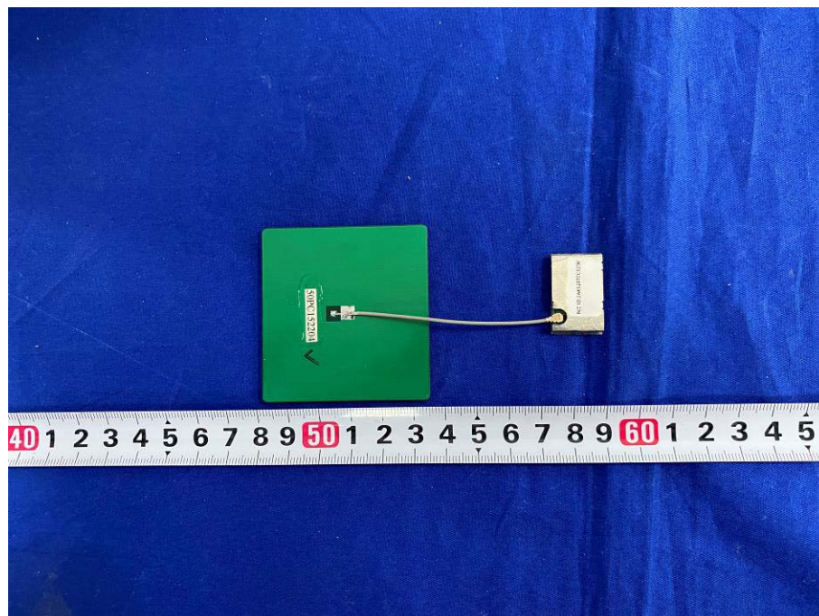
EUT with Antenna - Top View
