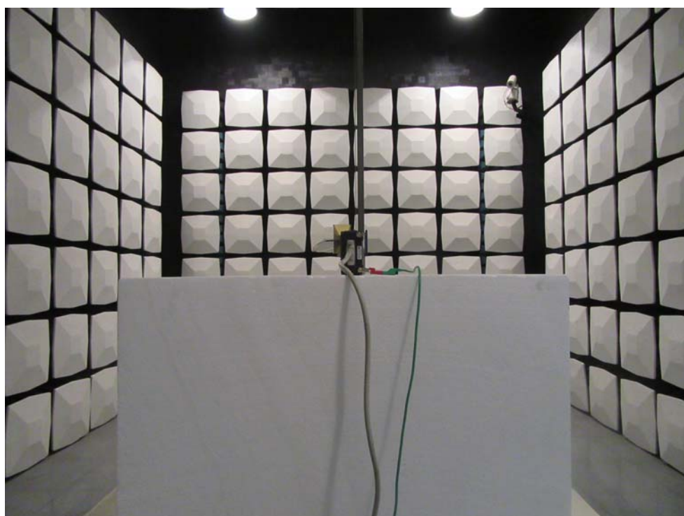
Radiated Disturbance Test Setup View-Above 1GHz
