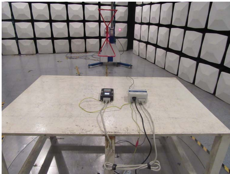
Radiated Disturbance Test Setup View-Below 1GHz
