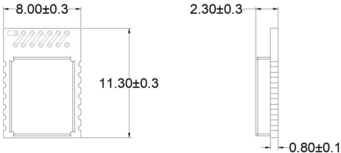
Figure 14: Module top and side dimension drawing
