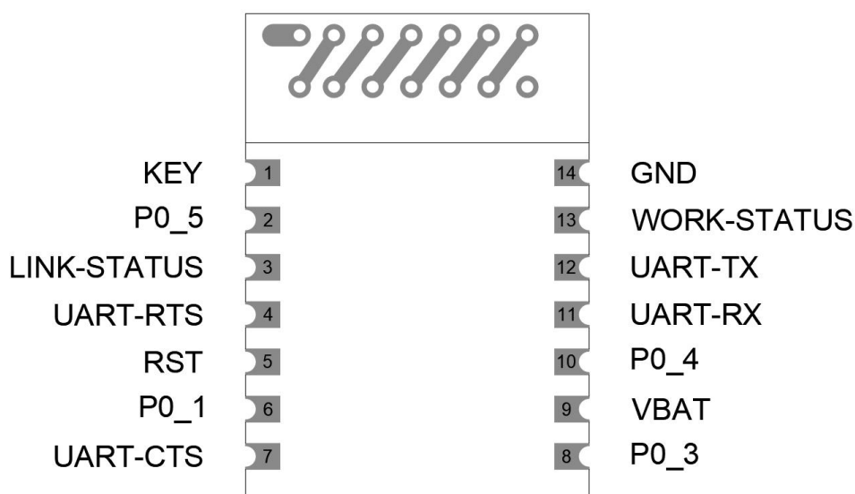
Figure 2: Module pin definition
