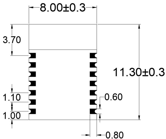
Figure 15: Bottom view size of the module
