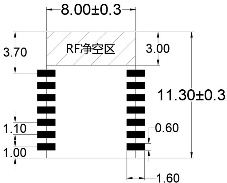
Figure 16: Recommended package dimensions
